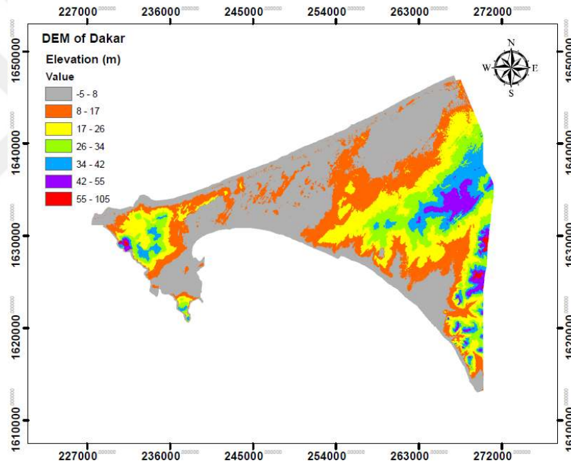
Figure 3. 7 Digital Elevation Model (DEM) of Dakar.
