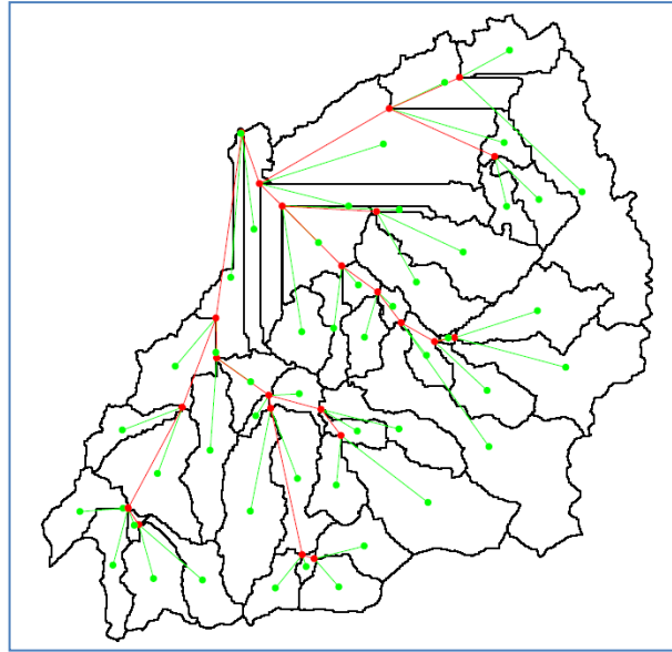
Figure 4.22 HMS Schematic
