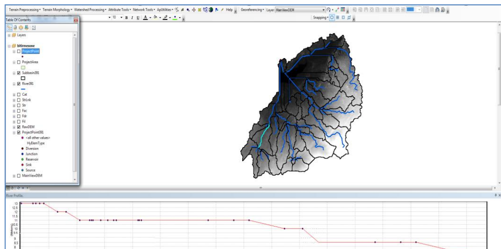
Figure 4. 18 River profile
