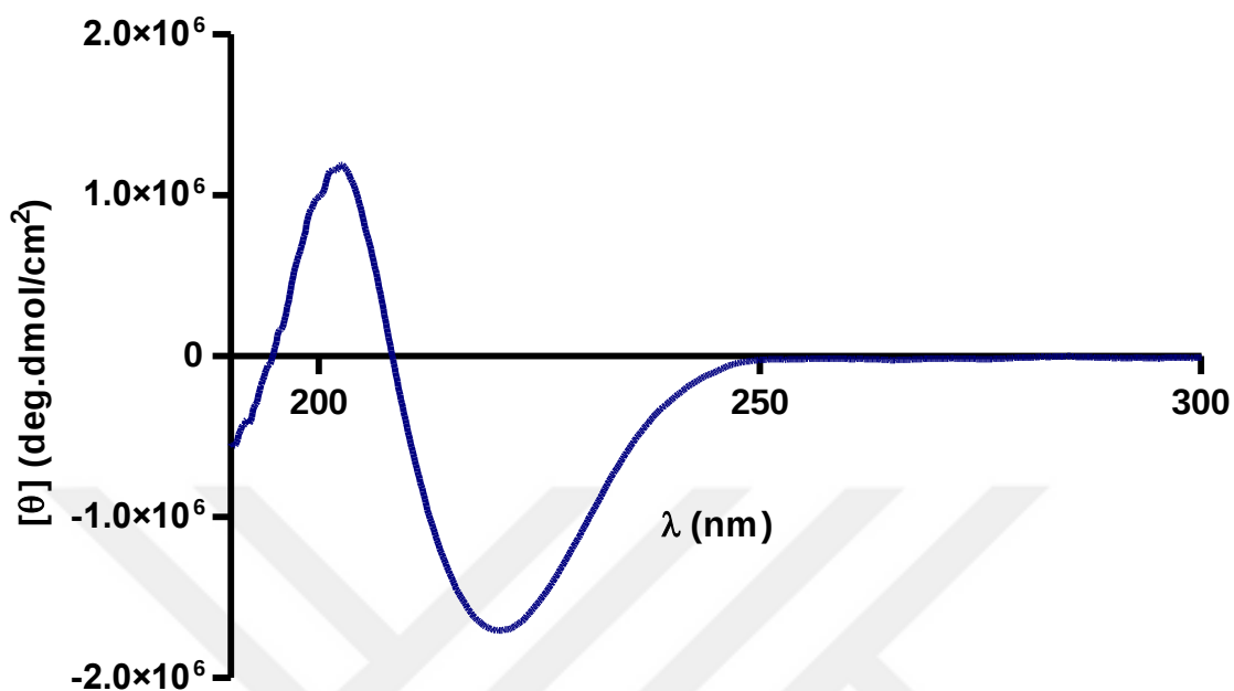
Figure 3.2 CD spectra of peptide amphiphile.
