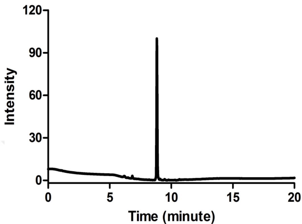
Figure 2.13 Liquid chromatogram of nPC molecule.
