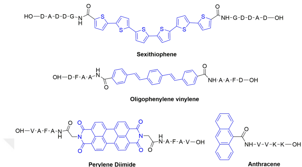
Figure 1.11 Semiconducting oligomers conjugated to peptide molecules.
