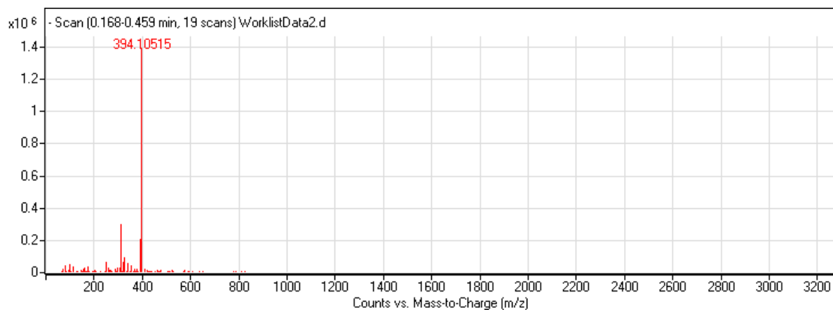
Figure 2.7 Mass spectrum of n-Bu-NTA- \beta alanine
