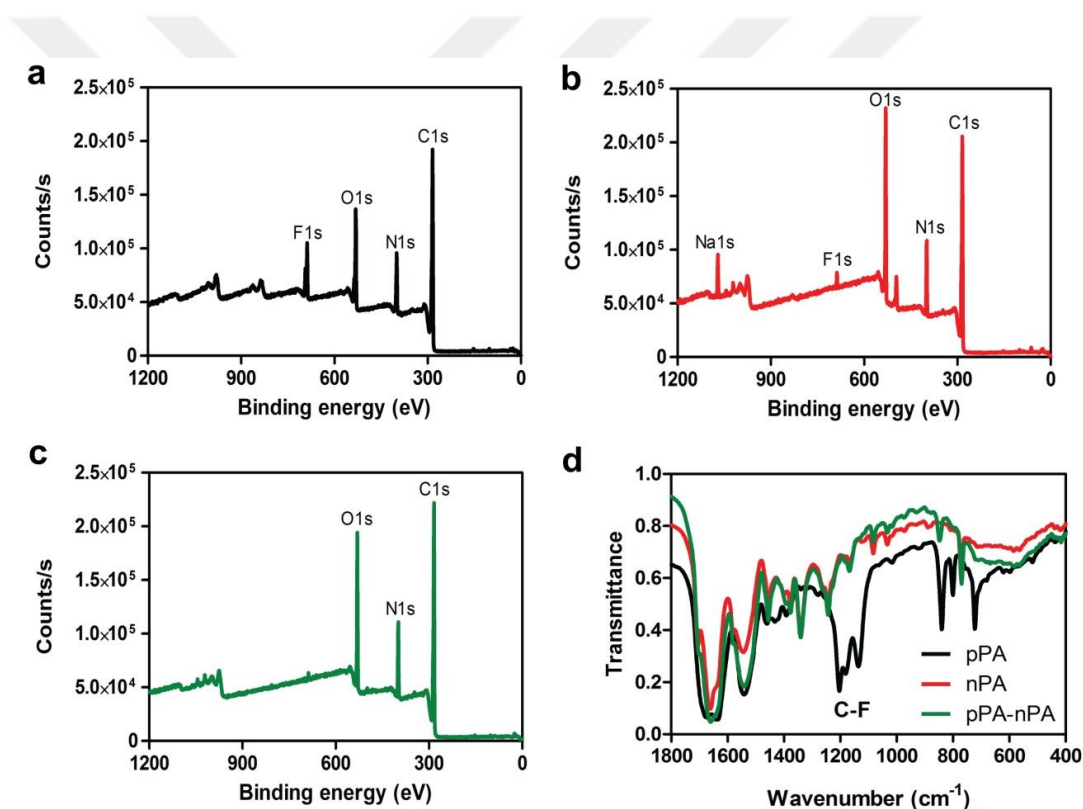
Figure 2.19 XPS analysis of pPC (a), nPC (b), and pPC-nPC (c) powders. FT-IR analysis (d).
