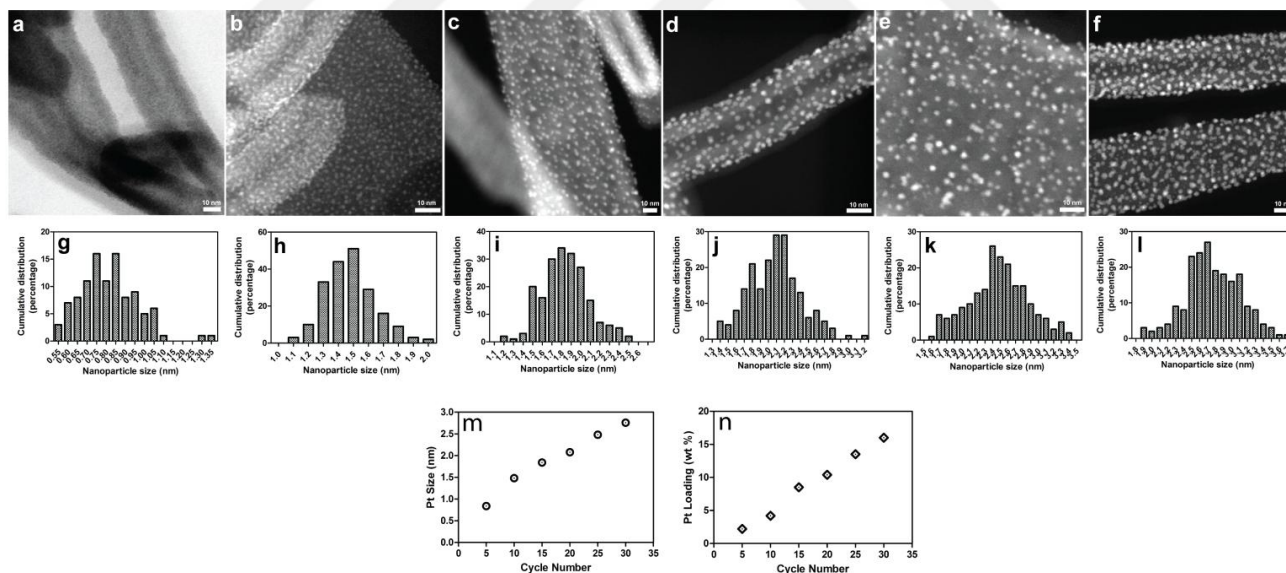
Figure 5.7 STEM images and size distribution of Pt5@TiO 2 (a, g), Pt10@TiO 2 (b, h), Pt15@TiO 2 (c, i), Pt20@TiO 2 (d, j), Pt25@TiO 2 (e, k) and Pt30@TiO 2 (f, l). Effect of Pt cycle on Pt nanoparticle size (m) and Pt loading (n). Histograms of particle size distribution were constructed by counting 100 nanoparticles for 5 cycle and 200 nanoparticles for the rest of cycles.
