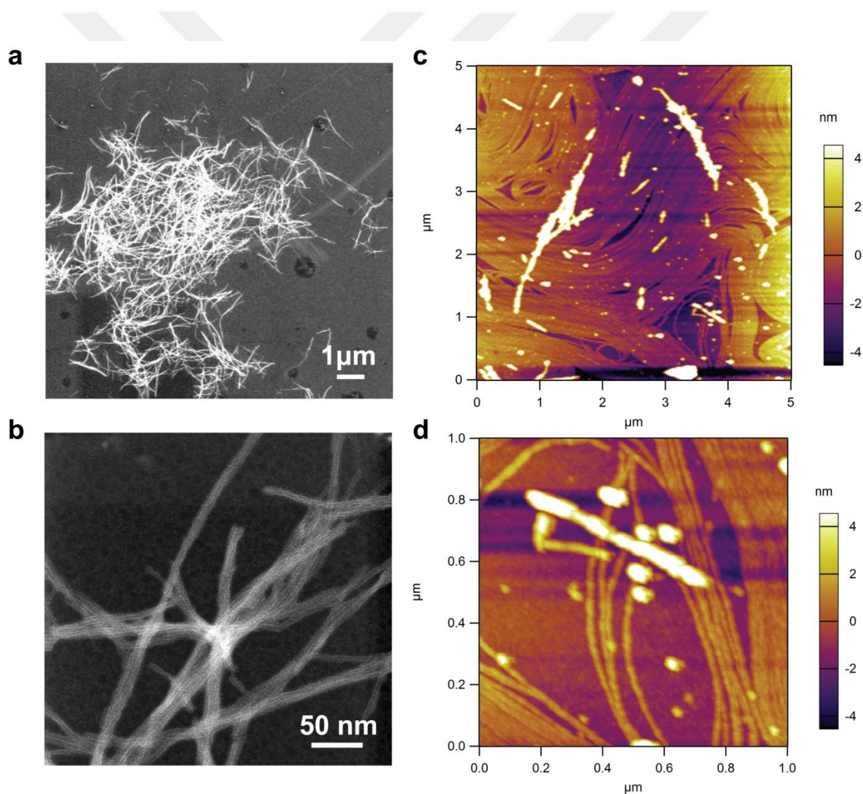
Figure 2.18 Imaging of pPC-nPC CT complex nanowires. STEM images (a and b) and AFM images (c and d) of n/p-coassembled supramolecular nanowires.
