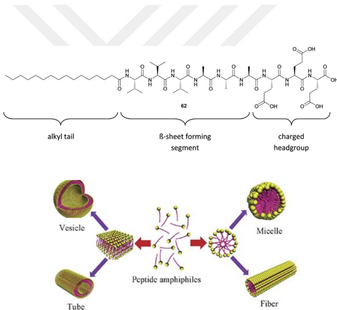
Figure 1.7 Typical chemical structure of peptide amphiphile and its self-assembly into various supramolecular nanostructures.
