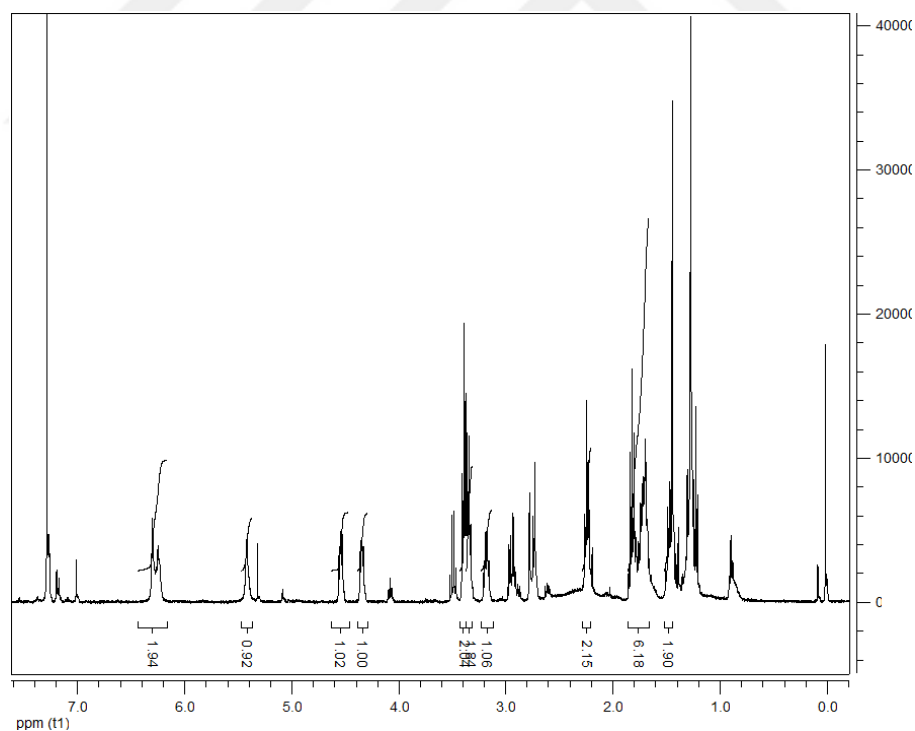
Figure 4.7 1 H NMR of Biotin-azide
