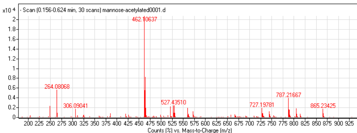
Figure 4.12 HRMS of \text{Ac}_4\text{ManNAI}
