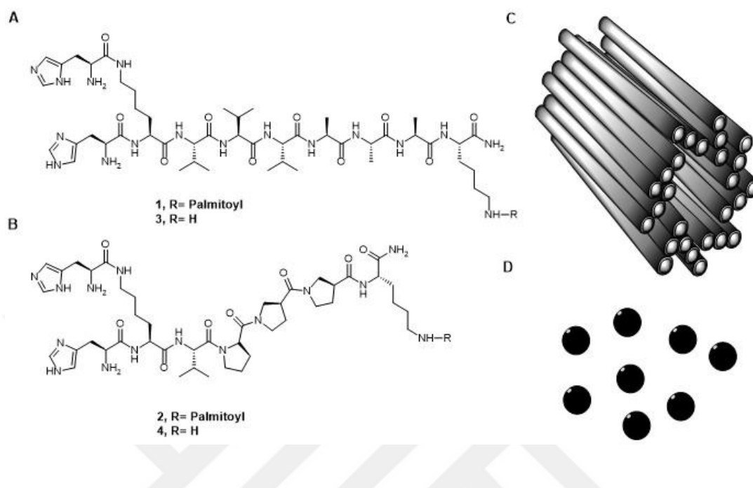
Figure 1.9 Chemical structures of peptide molecules (A and B), schematic representation of self-assembled nanofibers (C) and spherical aggregates (D).
