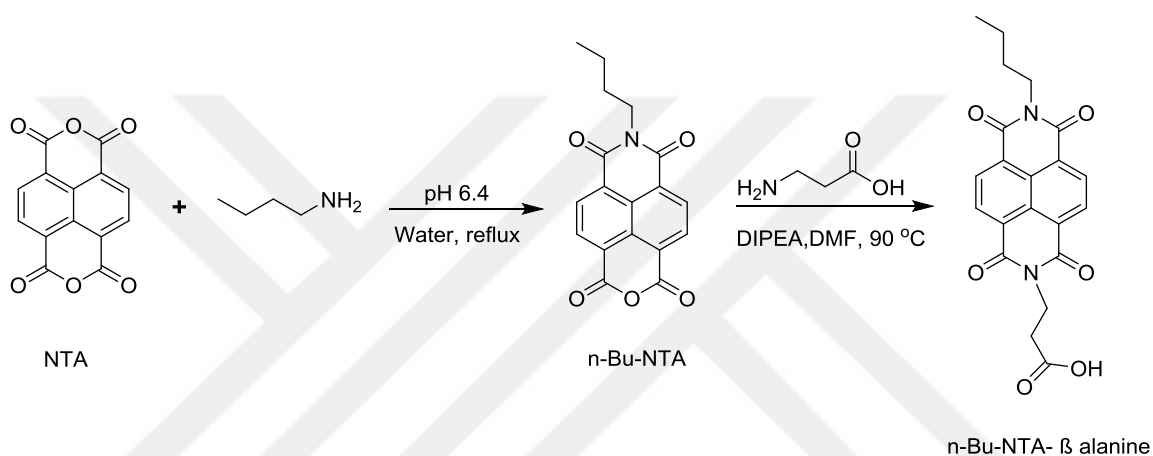
Figure 2.2 Schematic presentation of synthesis of n-Bu-NTA- β alanine
