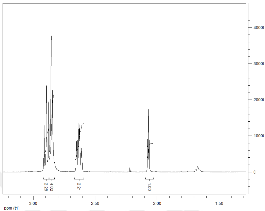
Figure 4.9 1 H NMR of N-succinimidyl-4-pentynoate
