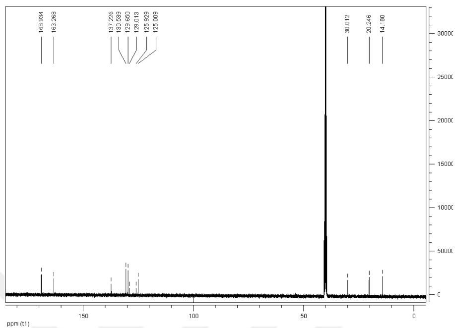
Figure 2.4 13 C NMR of n-Bu-NTA
