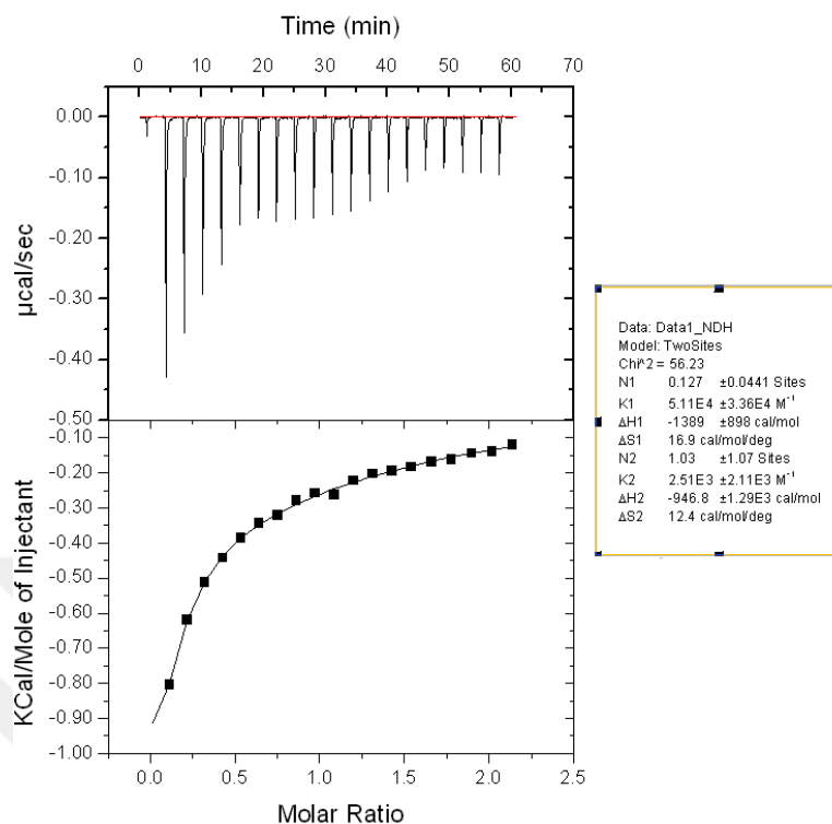
Figure 4.27 Isothermal titration calorimetry of Ac-HH-Am by CuSO 4 solution.
