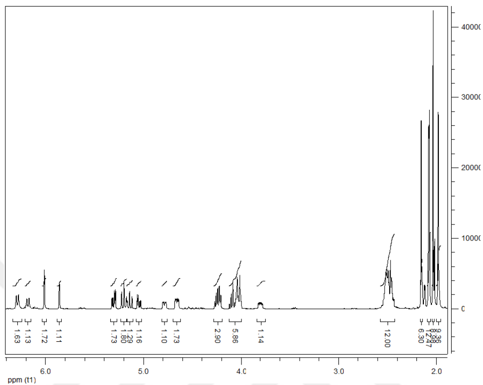
Figure 4.13 1 H spectrum of Ac 4 ManNAI
