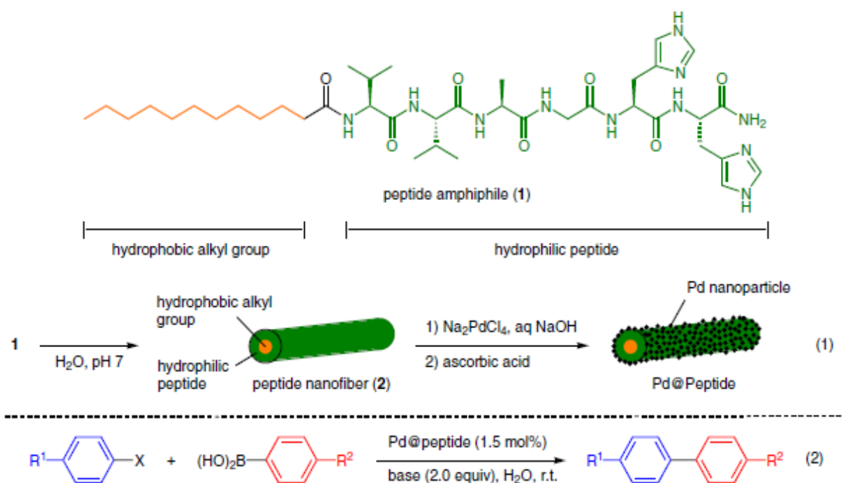
Scheme 2. Self-assembly of peptide amphiphile molecules generates nanofibers with 10 nm in diameter (1). Seeding and reduction of Pd II ions on the surface of peptide nanofibers form hybrid peptide and Pd 0 nanostructures (Pd@Peptide). Pd@Peptide nanostructures can be used as catalyst in C-C coupling reactions (2).
