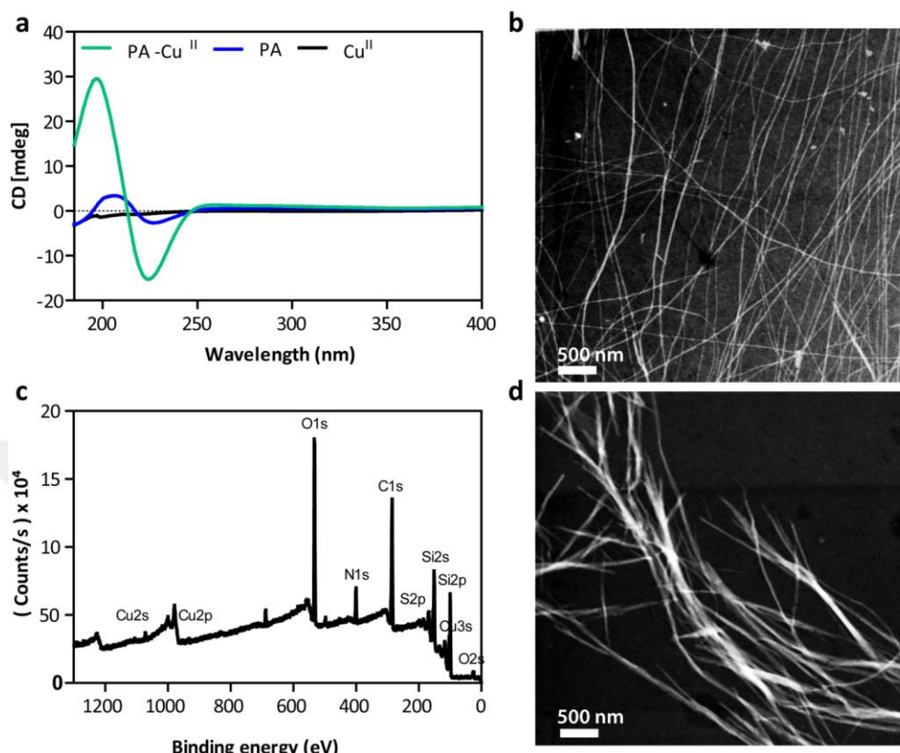
Figure 4.22 (a) CD analysis of PA and PA-Cu II , (b) STEM image of the PA nanofibers, (c) XPS and (d) STEM image of PA-Cu II nanofibers.
