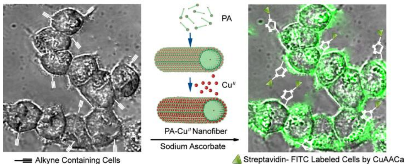
Scheme 3. Schematic representation of labeling live-cells by PA-Cu II nanofibers.
