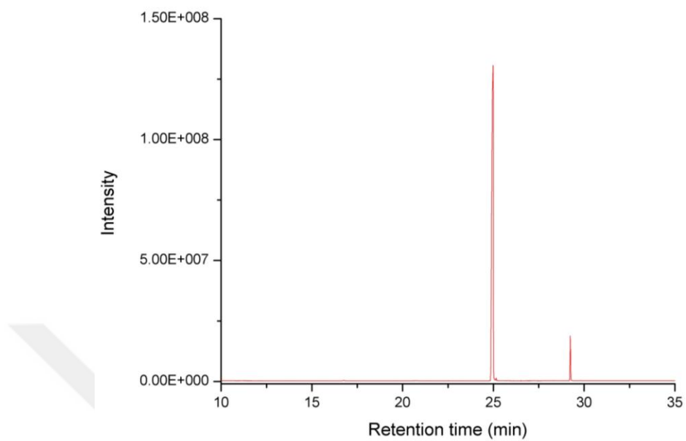
Figure 3.11 Gas Chromatogram of 4-methoxybiphenyl (Fifth run).
