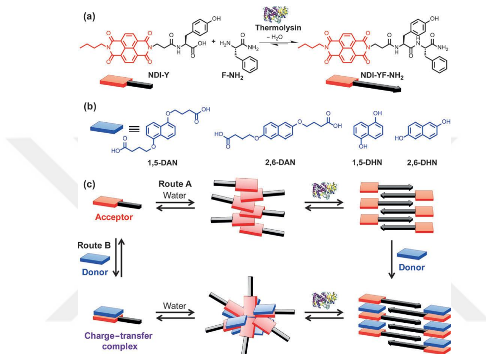
Figure 1.12 Biocatalytic self-assembly of acceptor-appended peptides to form charge-transfer nanostructures.
