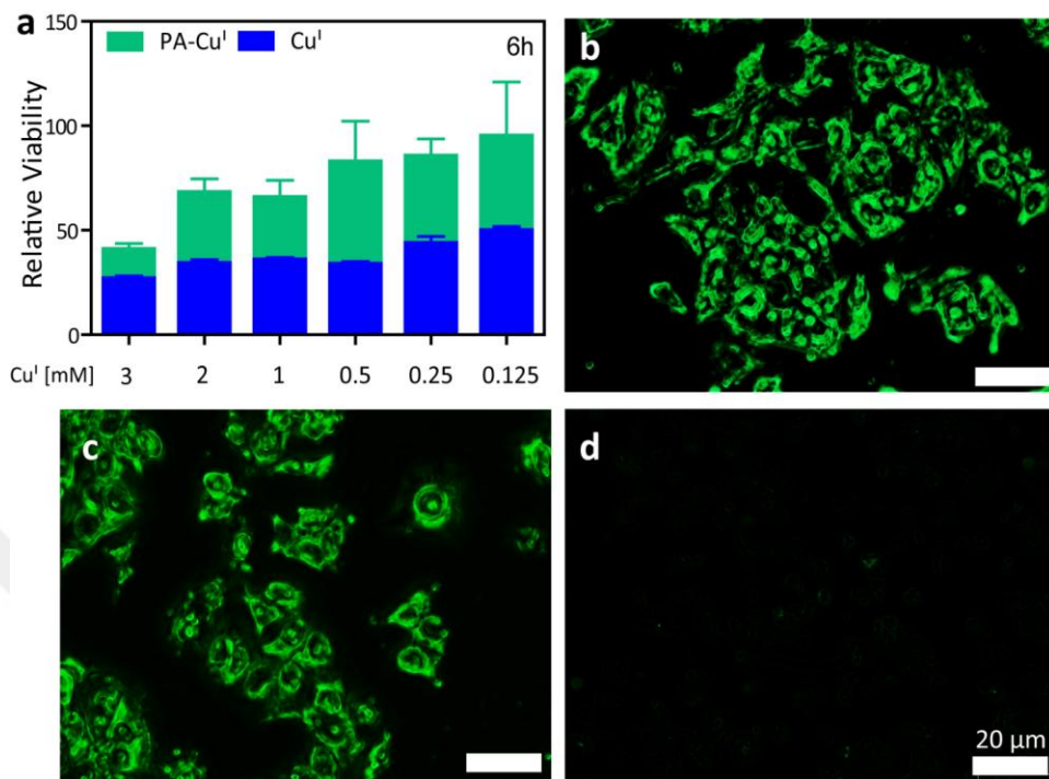
Figure 4.38 Viability of MCF-7 cells in the presence of PA- \text{Cu}^{\text{I}} and \text{Cu}^{\text{I}} (a), microscopic analysis of fixed cells labeled with PA- \text{Cu}^{\text{I}} nanofibers after 6 h (b), and after 24 h reaction (c) and non-treatment group after 24 h reaction (d). (Scale bars = 20 \mu\text{m} )
