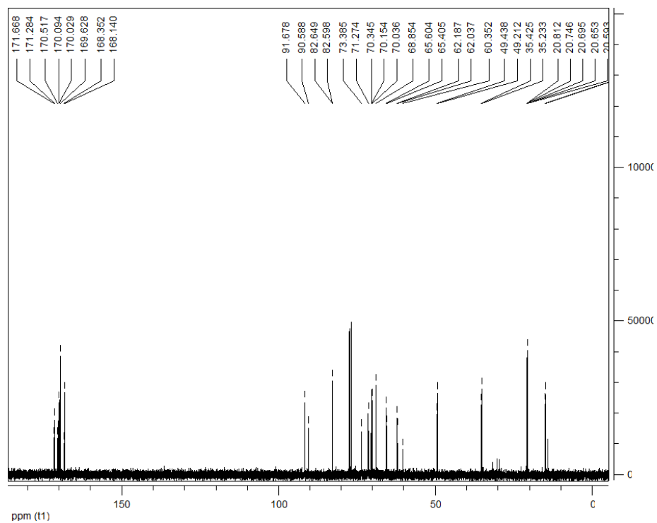
Figure 4.14 13 C spectrum of Ac 4 ManNAI
