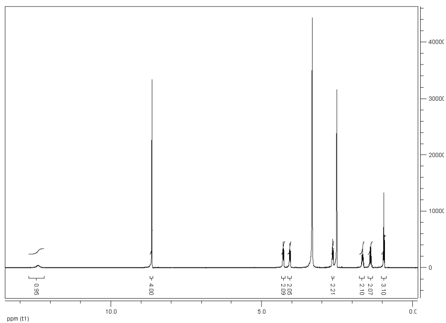
Figure 2.5 1 H NMR of n-Bu-NTA- β alanine
