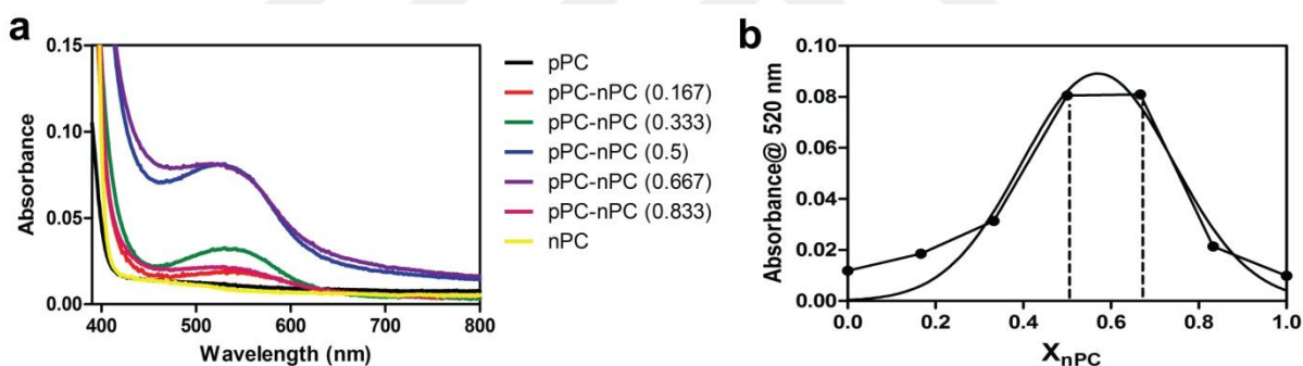
Figure 2.21 (a) UV-vis absorbance spectra of pPC and nPC molecules mixed at different mole ratios. (b) Plot of absorbance at 520 nm (CT band) versus mole ratio of nPC ( X_{nPC} ).
