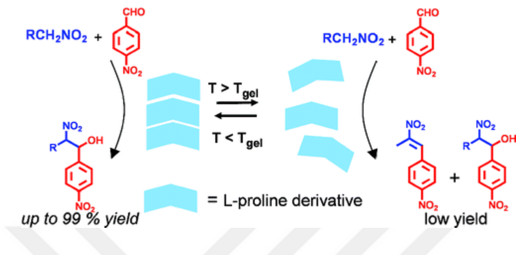
Figure 1.10 Schematic representation of L-proline catalyzed Henry nitroaldol reaction.
