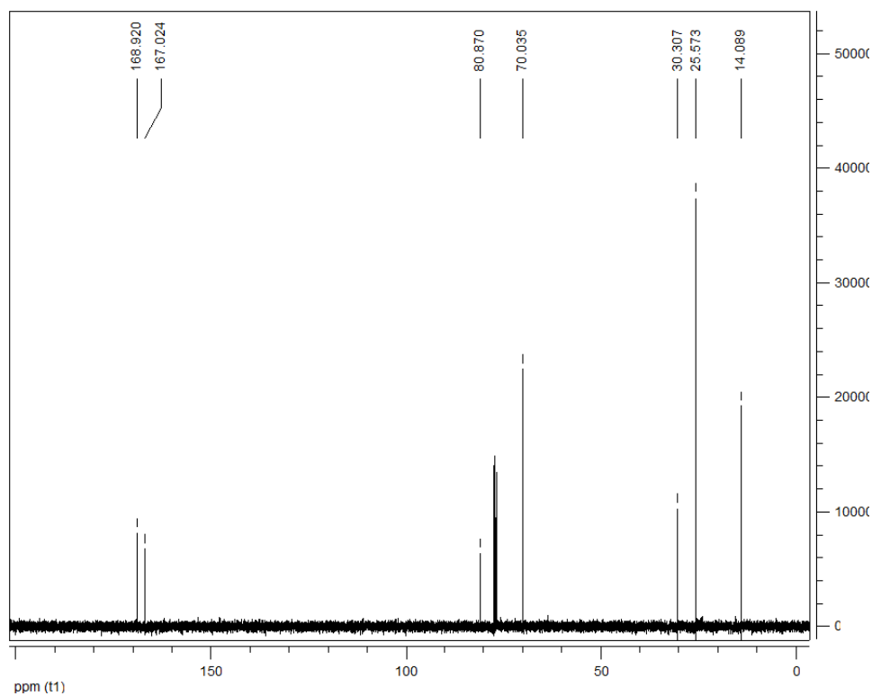
Figure 4.10 13 C NMR of N-succinimidyl-4-pentynoate
