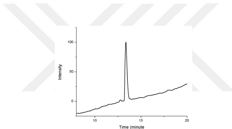
Figure 4.16 Liquid chromatogram of peptide amphiphile.
