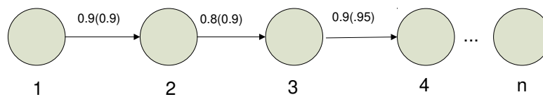
Figure 4.14 Confined serial trust chain for n=4
