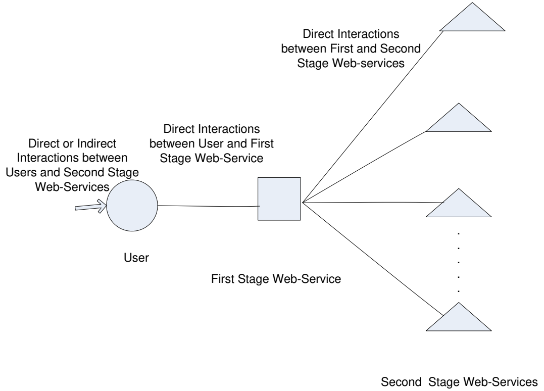
Figure 4.16 User interaction with first and second stage web-services
