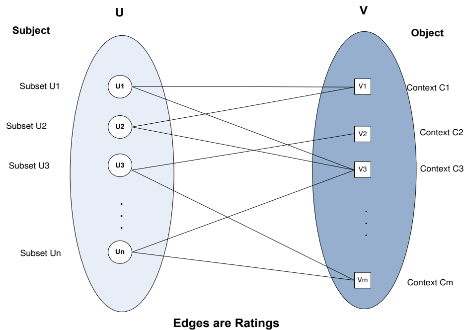
Figure 3.4 Bipartite-graph modeling
