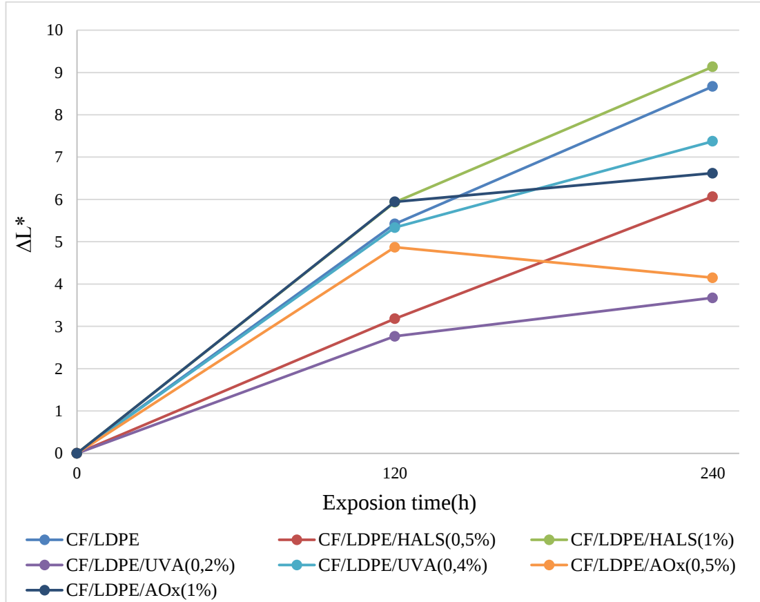
Figure 4.13 : \Delta L^* values of unstabilized and stabilized composites
