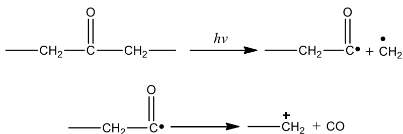
Figure 2.5 : Norrish type I reaction[29]
