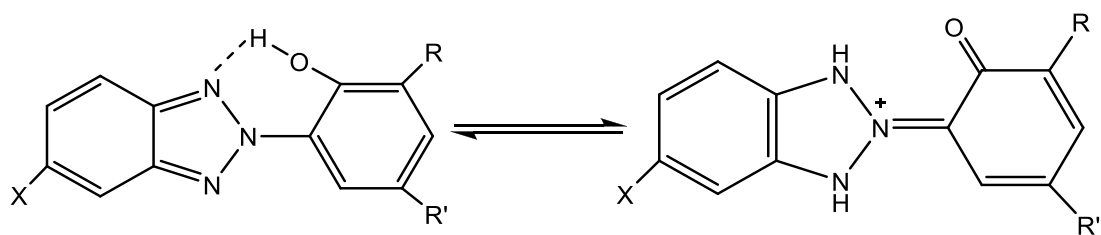
Figure 2.14 : Hydroxybenzotriazole mechanism[44]
