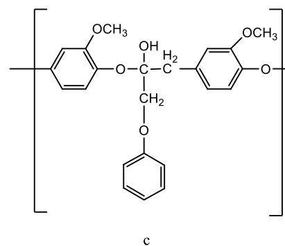
Figure 2.2 : Chemical structure of (a) cellulose (b) hemicellulose and (c) lignin [3]
