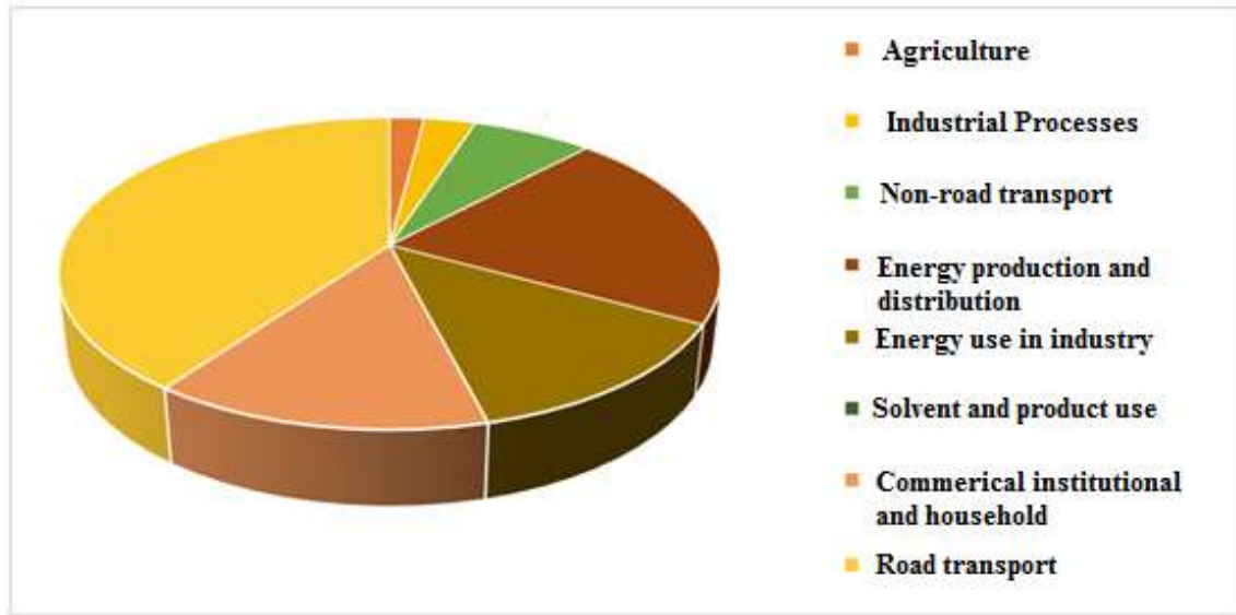
Figure 1.1: Distribution of NO x emissions among different sectors in EU (2011). Adapted from Ref [14].
