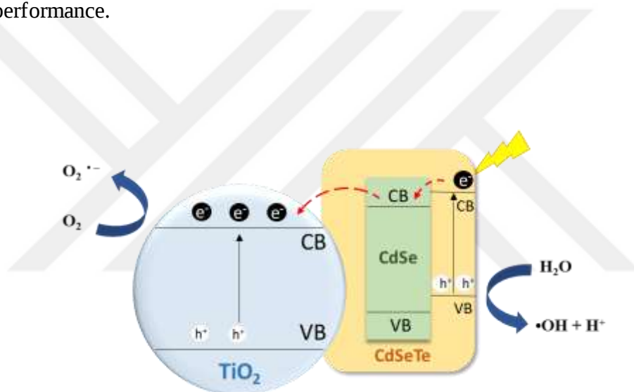
Figure 1.10: A possible illustration of electron-hole transport in CdSe/CdSeTe/P25 catalyst.
