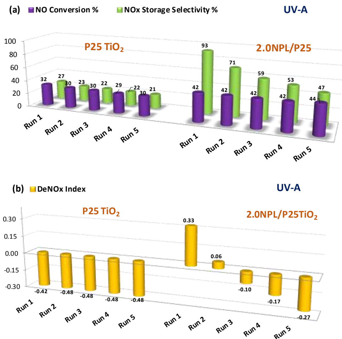
Figure 3.30: Long term %NO conversion, %NO x storage selectivity and DeNO x index results of P25 and 2.0NPL/P25 under UV-A light irradiation.
