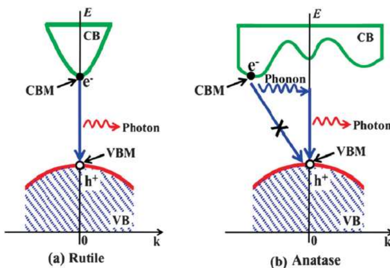
Figure 1.5: Recombination process of photogenerated electron-hole for a) direct bandgap rutile. b) indirect bandgap anatase. Adapted from Ref [41].
