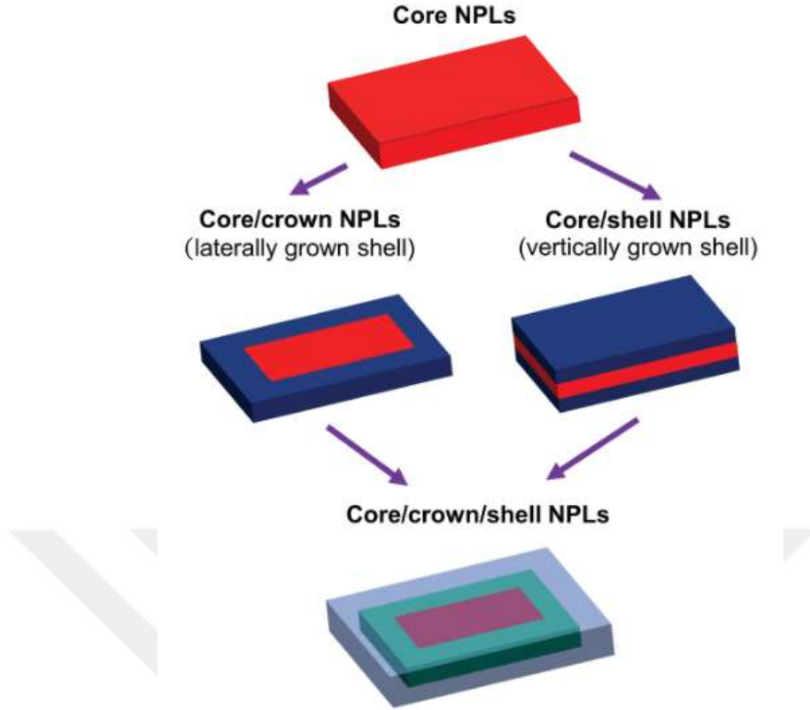
Figure 1.7: Schematic representation of different configurations in NPL. Adapted from Ref [57].
