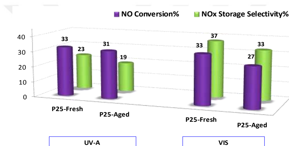
Figure 3.12: NO(g) conversion %, and NO x storage selectivity % for fresh and aged P25 under UV-A & VIS illumination.
