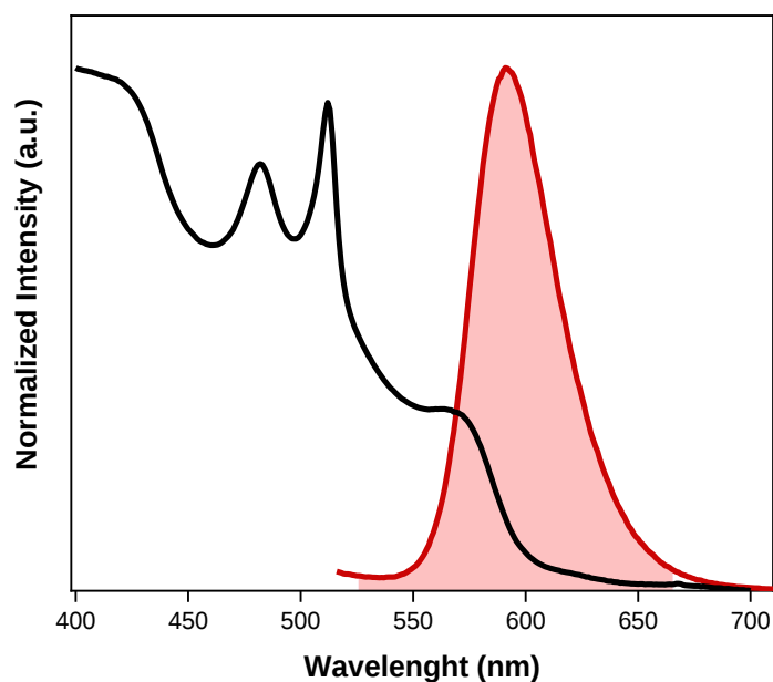
Figure 3.8: PL spectra of core/crown CdSe/CdSeTe quantum well NPL[77].
