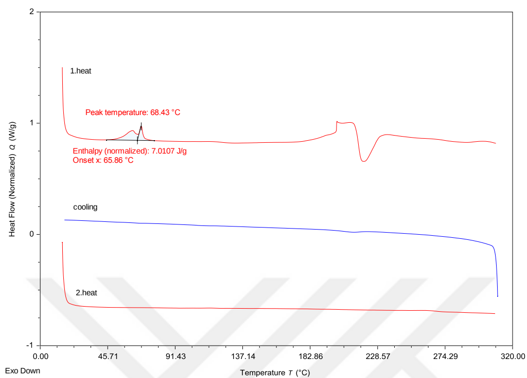
Figure B.7. Thermal analysis result obtained from DSC for RP2
