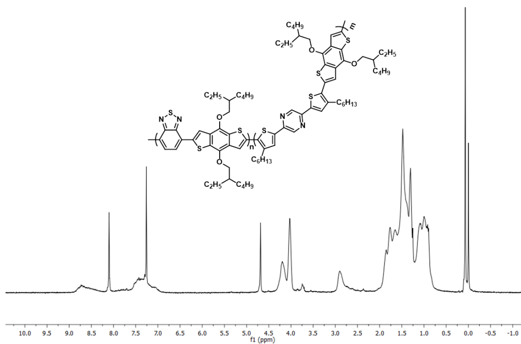
Figure A.12. ^1\text{H} NMR of RP2
