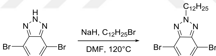
Figure 2.8. Synthesis of 4,7-dibromo-2-dodecyl-2H-benzo[d][1,2,3]triazole
