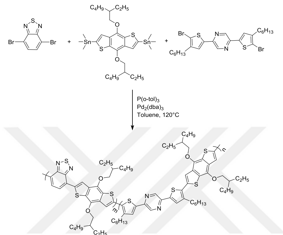
Figure 2.10. Synthesis of RP2
