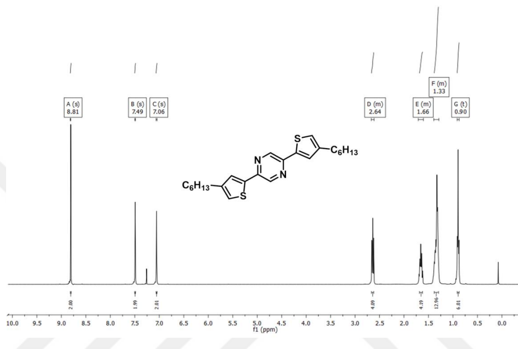
Figure A.1. 1 H NMR of 2,5-di(3-hexylthiophen-2-yl)pyrazine
