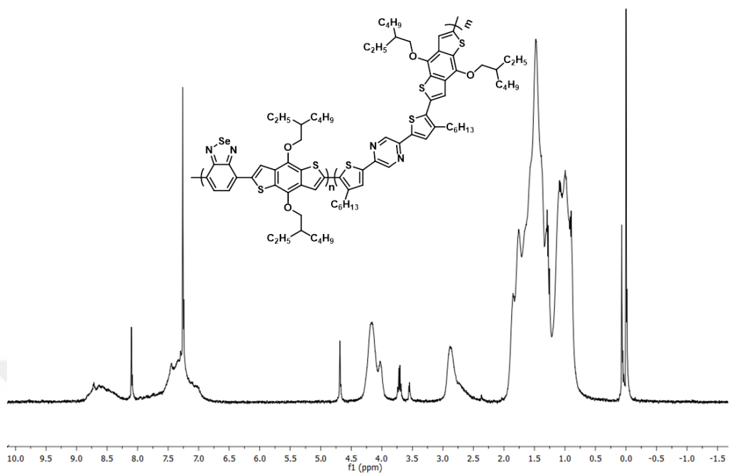
Figure A.13. ^1\text{H} NMR of RP3
