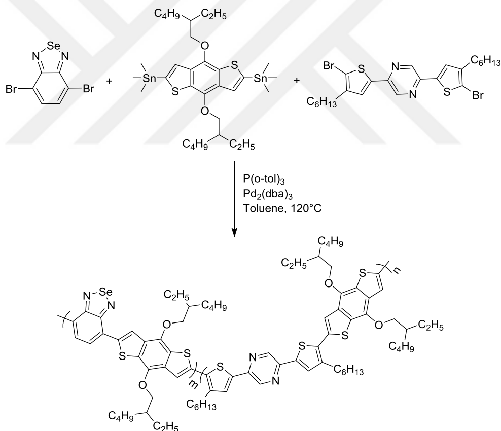
Figure 2.11. Synthesis of RP3
