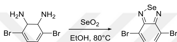
Figure 2.6. Synthesis of 4,7-dibromobenzo[c][1,2,5]selenadiazole
