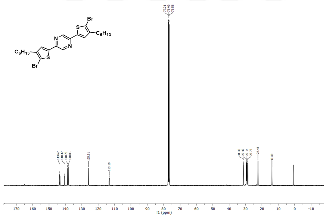
Figure A.4. ^{13}\text{C} NMR of 2,5-bis-(5-bromo-4-hexylthiophen-2-yl)pyrazine
