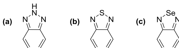
Figure 1.10. Structure of benzazole acceptor units; (a) benzotriazole (BTz), (b) benzothiadiazole (BT), (c) benzoselenadiazole (BSe)
