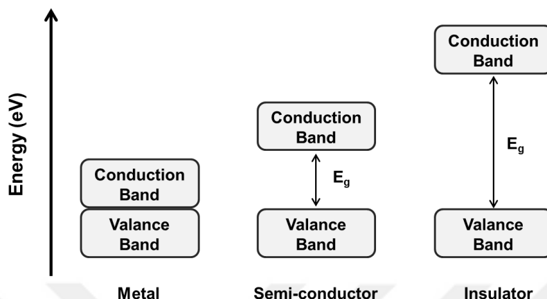
Figure 1.6. Representation of the energy gap ( E_g ) between HOMO and LUMO in a metal, a semi-conductor, and an insulator
