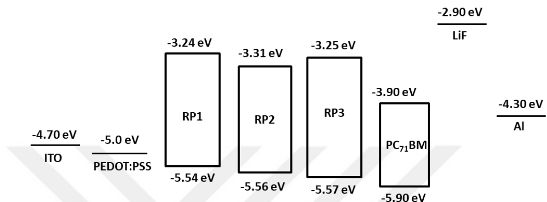
Figure 3.9. Energy level representation of the polymers RP1 , RP2 and RP3 with materials used in fabricating OPVs
