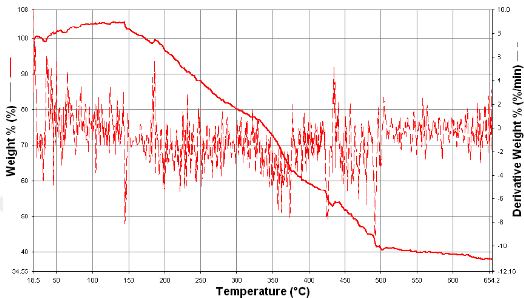
Figure B.1. Thermal analysis result obtained from TGA for RP1
