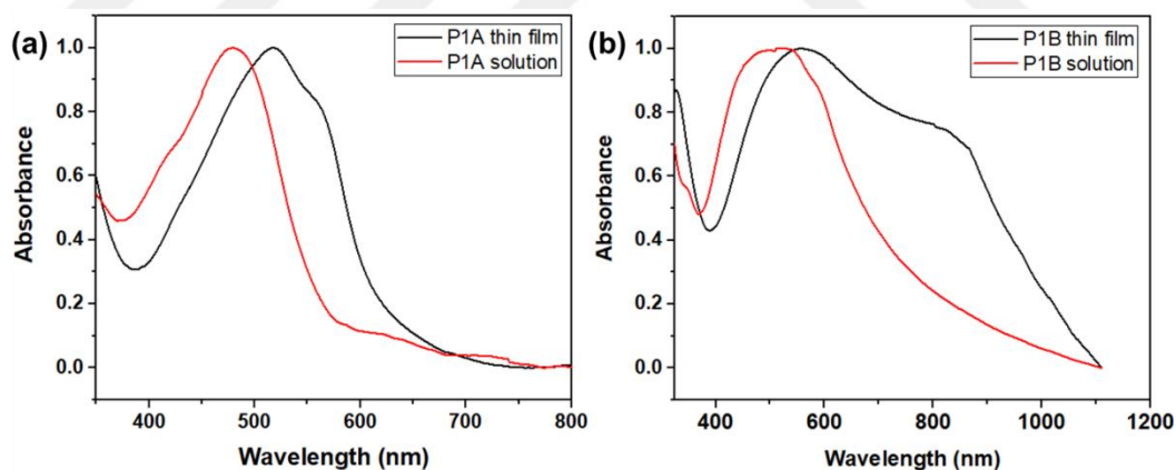
Figure 3.2. UV-Vis absorption spectra of polymers (a) P1A and (b) P1B in dilute \text{CHCl}_3 solution (red) and as thin film (black)
