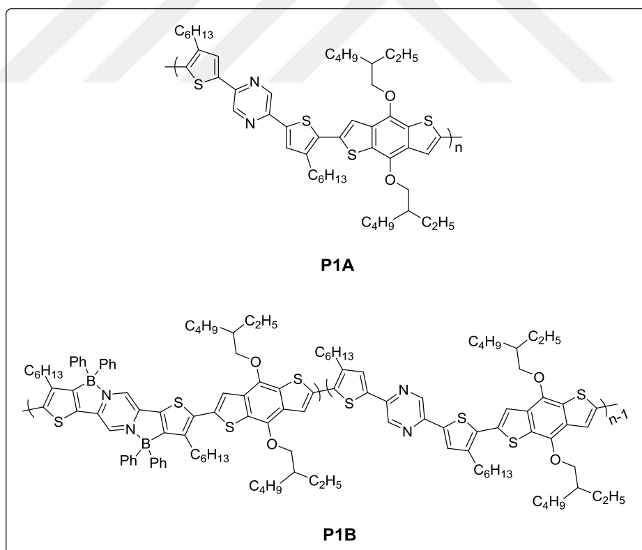
Figure 1.15. Structure of polymers P1A and P1B
