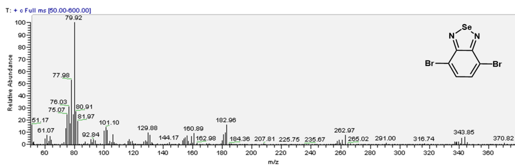
Figure A.8. GC-MS result of 4,7-dibromobenzo[c][1,2,5]selenadiazole
