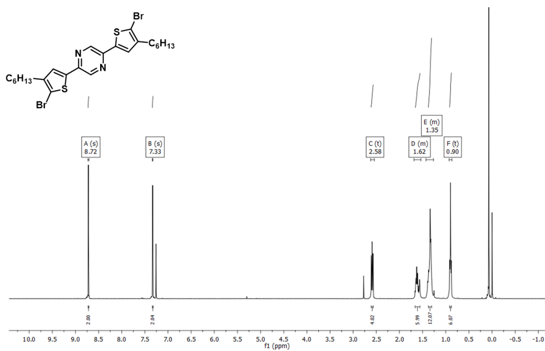
Figure A.3. ^1\text{H} NMR of 2,5-bis-(5-bromo-4-hexylthiophen-2-yl)pyrazine
