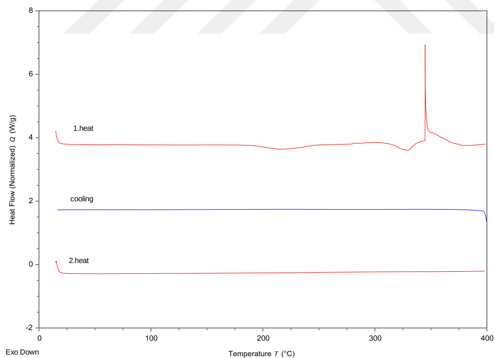
Figure B.8. Thermal analysis result obtained from DSC for RP3
