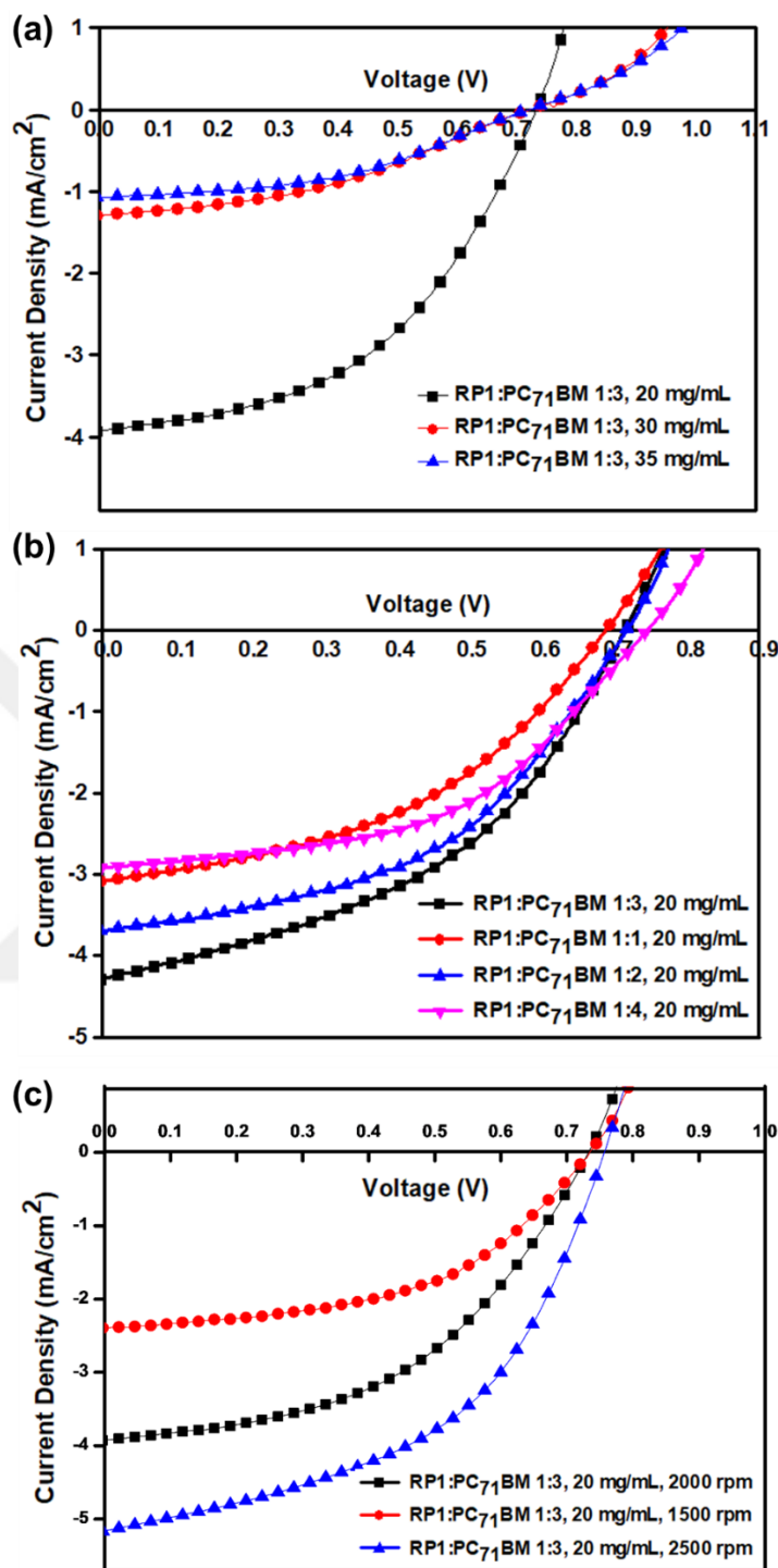
Figure 3.10. J-V curves of the OPV devices based on RP1:PC 71 BM summarizing optimization of (a) blend concentrations, (b) D/A ratios, (c) spin coating rates
