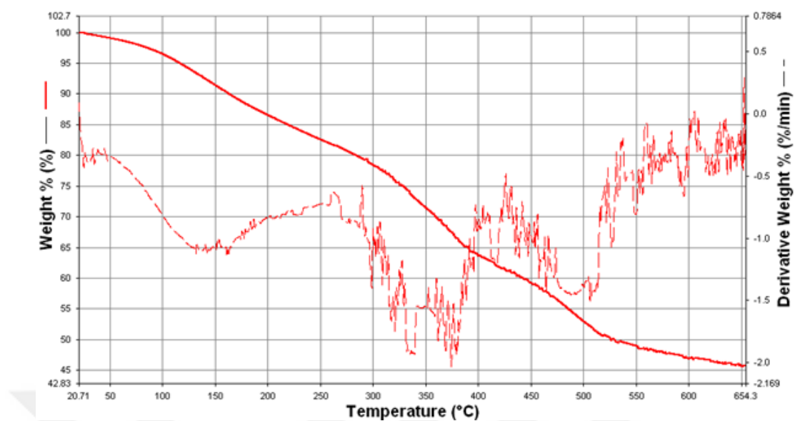
Figure B.5. Thermal analysis result obtained from TGA for P1B
