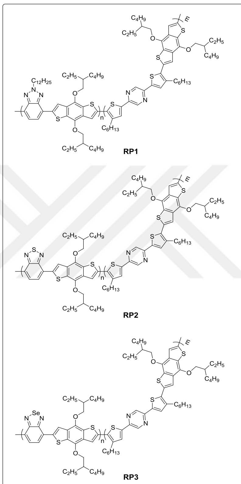
Figure 1.16. Structure of polymers RP1 , RP2 , and RP3
