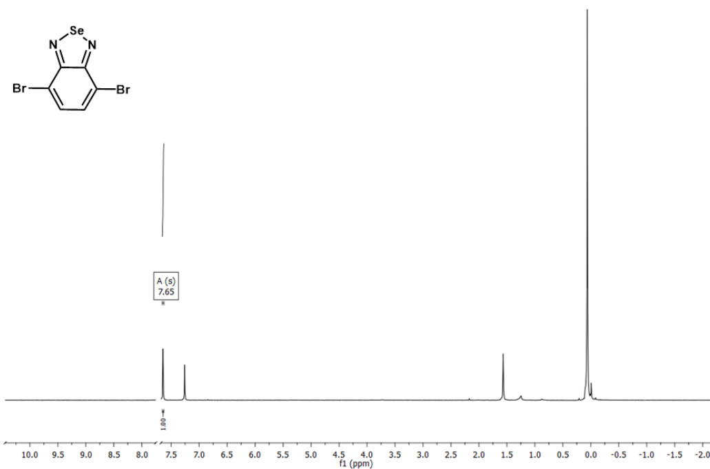
Figure A.7. 1 H NMR of 4,7-dibromobenzo[c][1,2,5]selenadiazole
