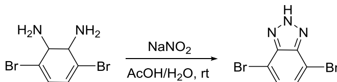
Figure 2.7. Synthesis of 4,7-dibromo-2H-benzo[d][1,2,3]triazole
