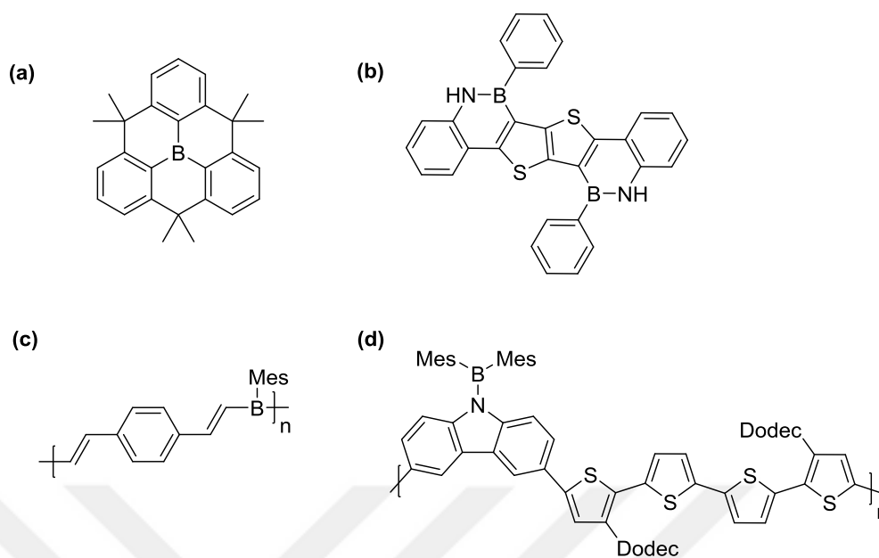
Figure 1.13. Some examples of tricoordinated boron-containing organoboron compounds, (a) and (b), and polymers, (c) and (d)
