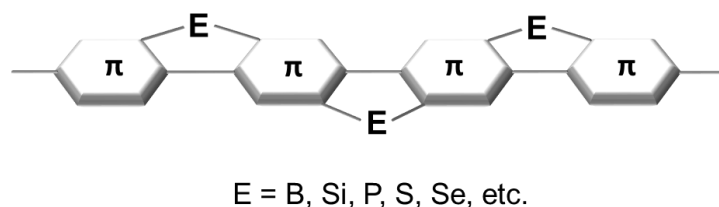
Figure 1.11. Schematic representation of the incorporation of main-group elements into \pi -conjugated framework
