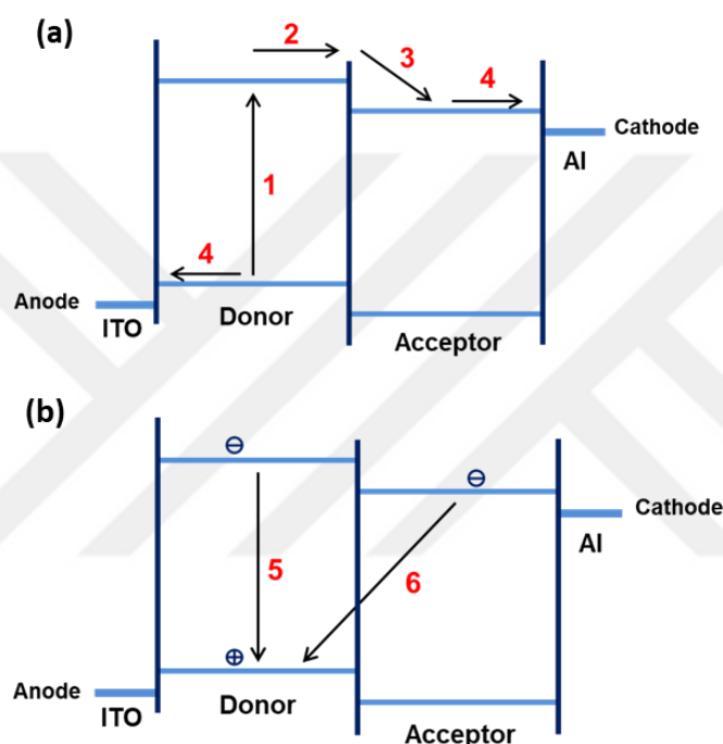
Figure 1.3. Schematic illustration of the working principle of BHJ OPVs on which corresponding numbers indicate (a) four stages of the operation of the cell, and (b) undesired processes in operating BHJ OPVs
