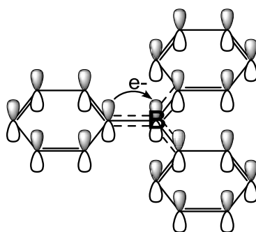
Figure 1.12. \pi -conjugation with boron
