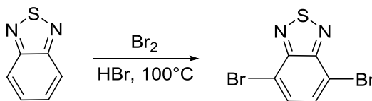
Figure 2.4. Synthesis of 4,7-dibromobenzo[c][1,2,5]thiadiazole
