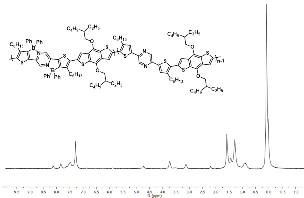
Figure A.15. ^1\text{H} NMR of P1B
