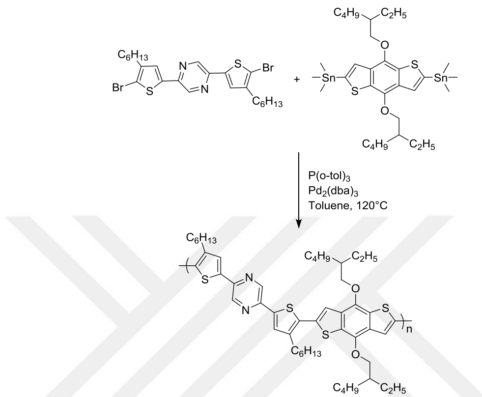
Figure 2.12. Synthesis of P1A
