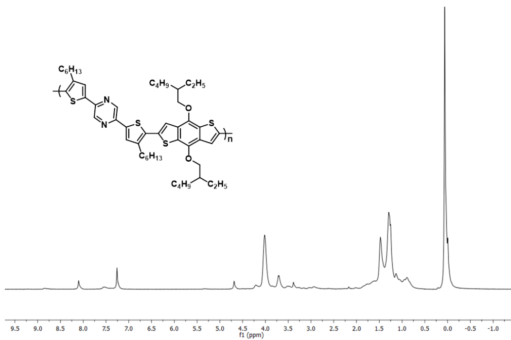
Figure A.14. ^1\text{H} NMR of P1A
