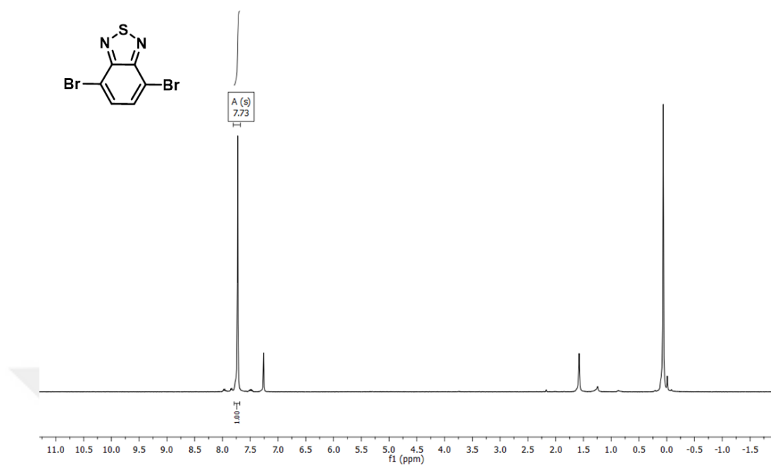
Figure A.5. 1 H NMR of 4,7-dibromobenzo[c][1,2,5]thiadiazole
