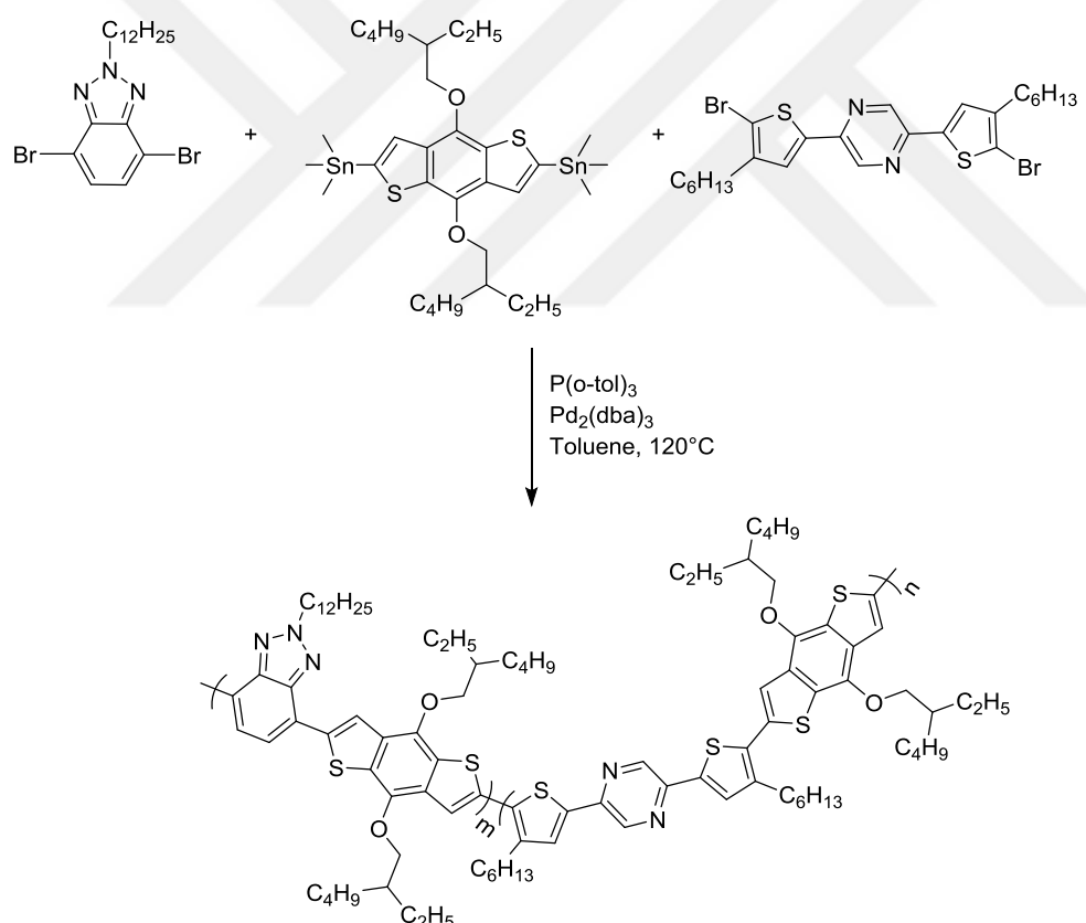
Figure 2.9. Synthesis of RP1
