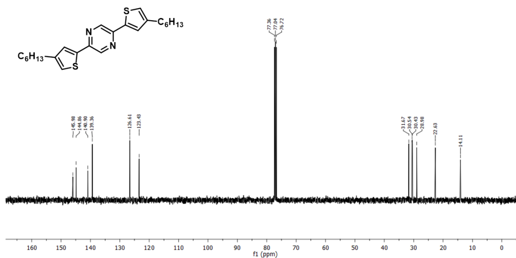
Figure A.2. 13 C NMR of 2,5-di(3-hexylthiophen-2-yl)pyrazine
