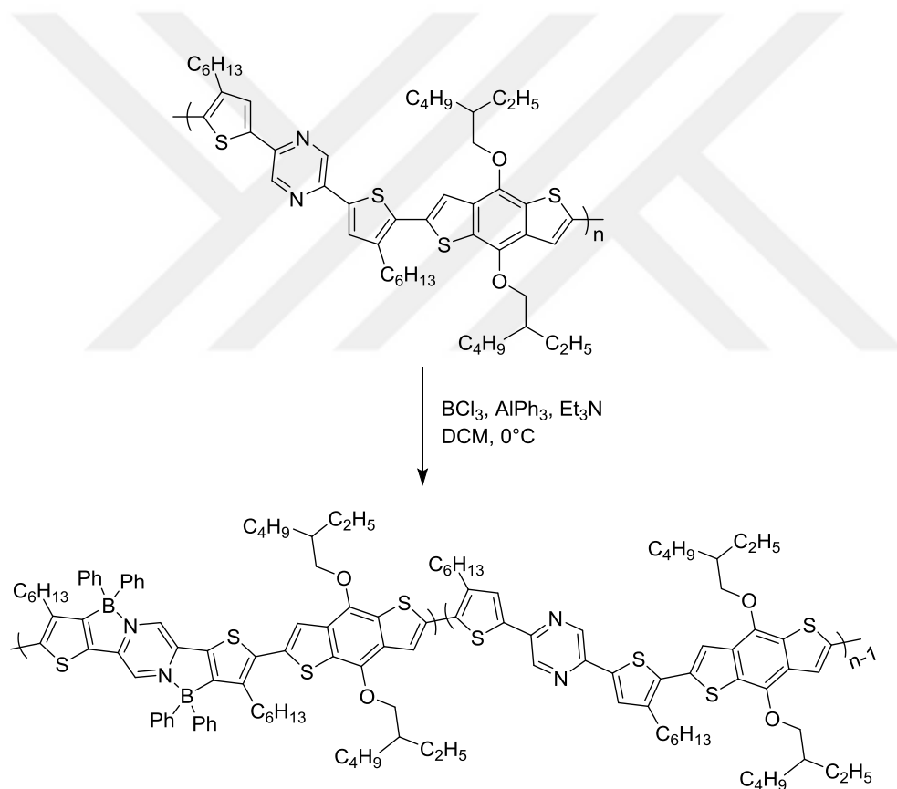
Figure 2.13. Synthesis of P1B
