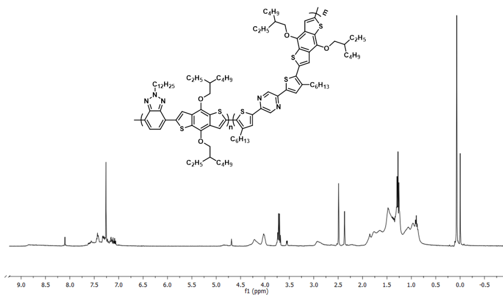
Figure A.11. ^1\text{H} NMR of RP1
