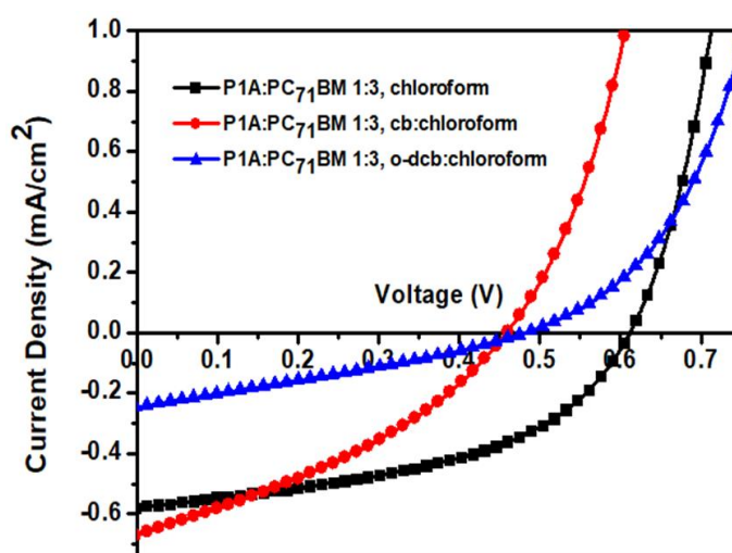
Figure 3.5. J-V curve summarizing the solvent optimization of P1A -based OPVs
