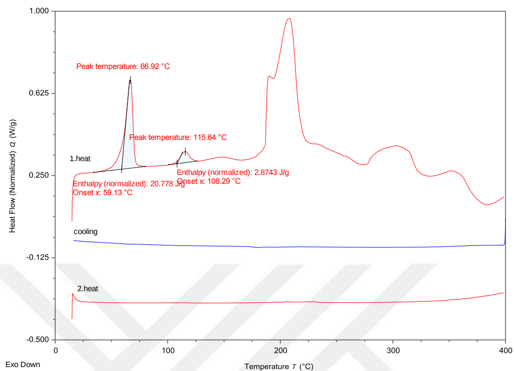
Figure B.9. Thermal analysis result obtained from DSC for P1A
