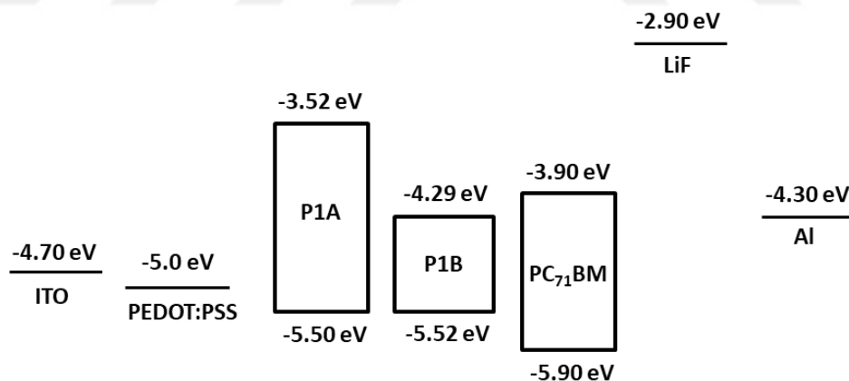
Figure 3.8. Energy level diagrams of P1A and P1B based organic solar cells
