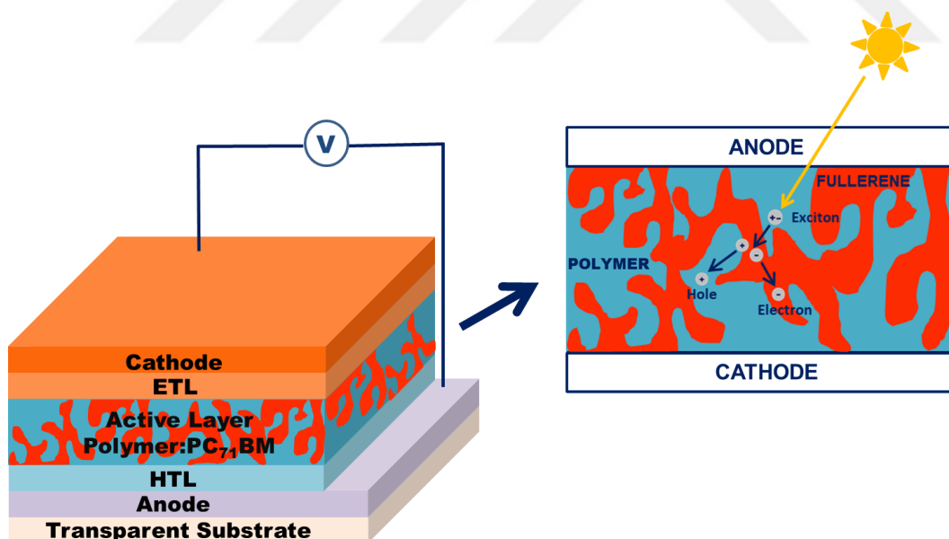
Figure 1.2. Device architecture of a BHJ OPV, containing blend of donor material polymer (blue) and acceptor material fullerene (red)
