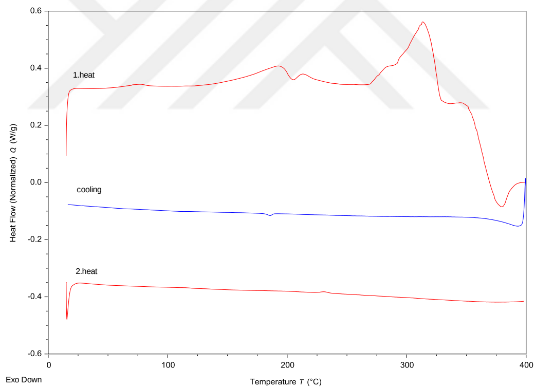
Figure B.6. Thermal analysis result obtained from DSC for RP1
