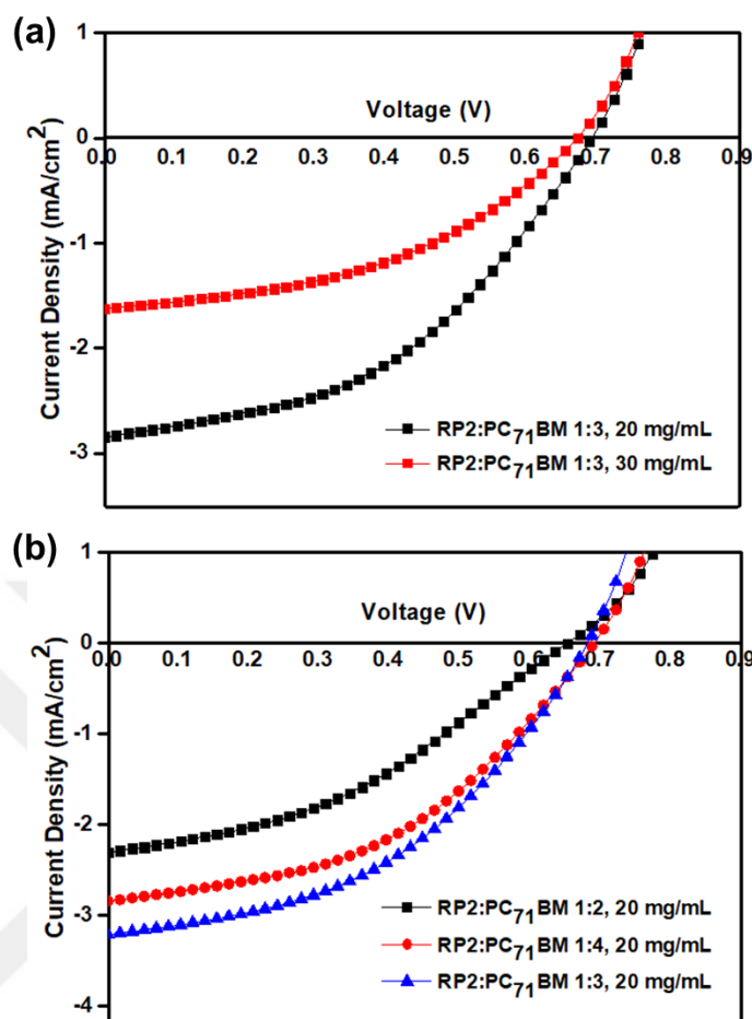
Figure 3.11. J-V curves of the OPV devices based on RP2:PC 71 BM summarizing optimization of (a) blend concentrations and (b) D/A ratios
