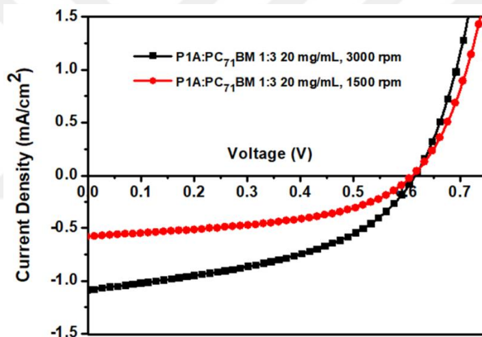
Figure 3.6. J-V curve summarizing the thickness optimization of P1A -based OPVs prepared using chloroform
