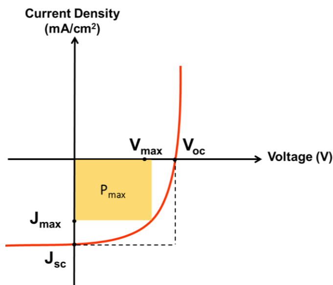
Figure 1.4. Schematic illustration of a J-V curve of a photovoltaic device
