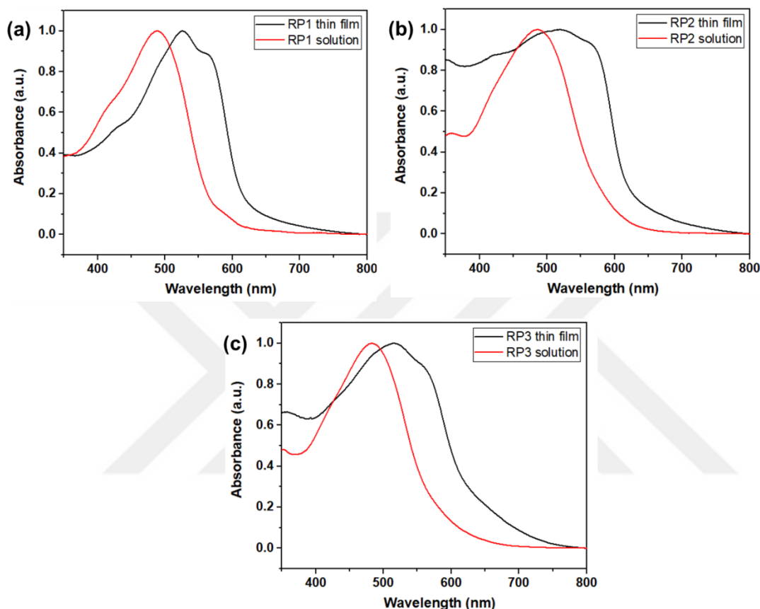
Figure 3.1. UV-Vis absorption spectra of polymers (a) RP1 , (b) RP2 , (c) RP3 in dilute \text{CHCl}_3 solution (red) and as thin film (black)
