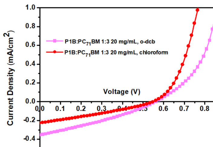
Figure 3.7. J-V curve summarizing the solvent optimization of P1B -based OPVs
