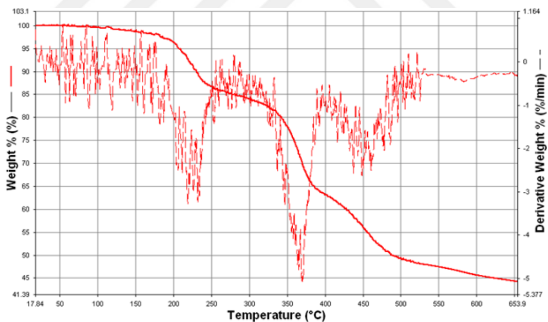
Figure B.2. Thermal analysis result obtained from TGA for RP2
