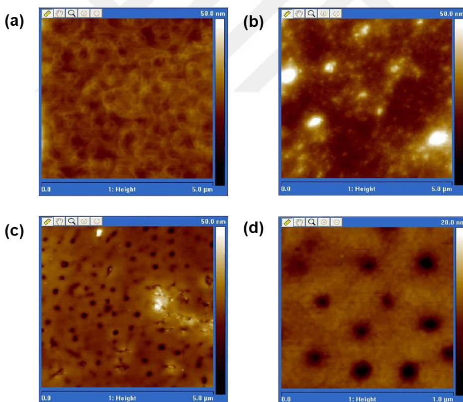
Figure 3.13. AFM images of the best performed devices (a) RP1 :PC 71 BM (1:3, w:w), (b) RP1 : PC 71 BM (1:3, w:w) with the additive DPE, (c) RP2 :PC 71 BM (1:3, w:w) and (d) RP3 :PC 71 BM (1:3, w:w)
