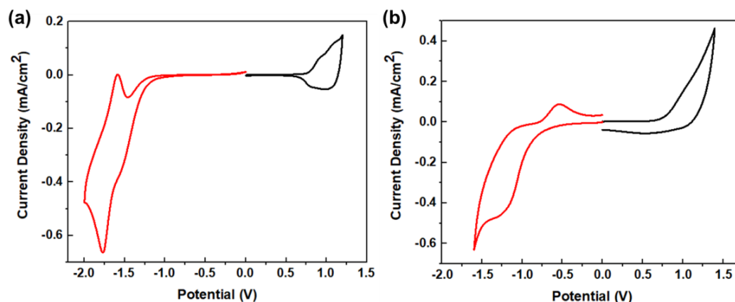
Figure 3.4. Single scan cyclic voltammograms of polymers (a) P1A and (b) P1B in 0.1 M TBAPF 6 /ACN electrolyte solution
