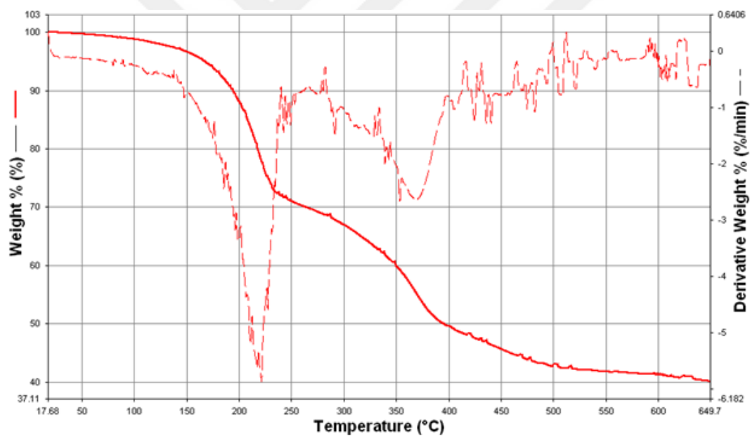
Figure B.4. Thermal analysis result obtained from TGA for P1A
