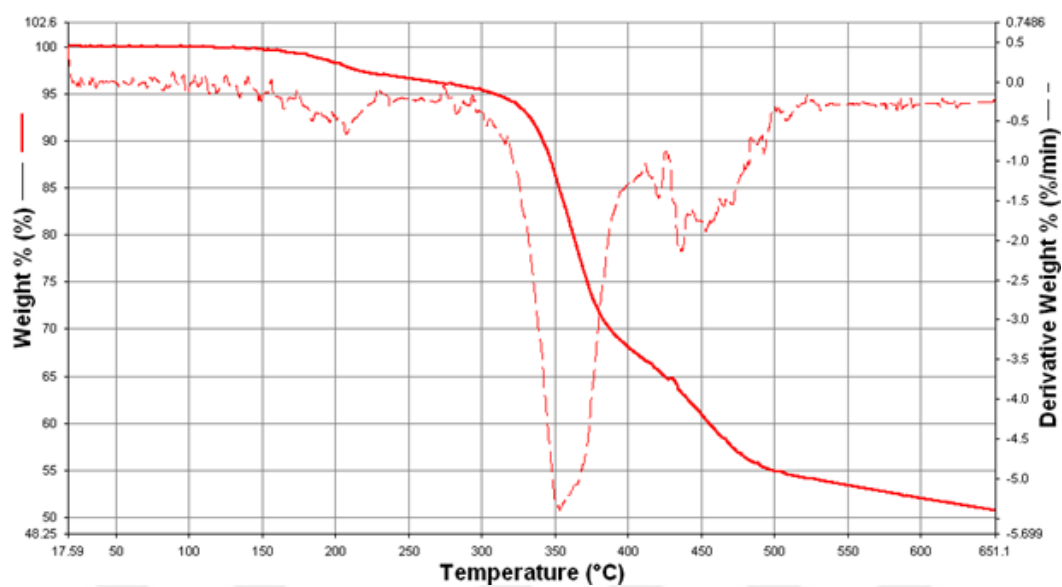
Figure B.3. Thermal analysis result obtained from TGA for RP3
