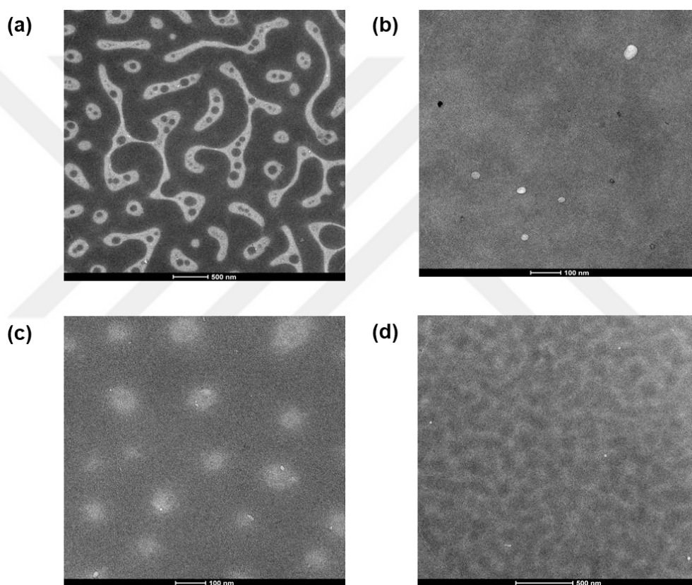
Figure 3.14. TEM images of the best performed devices (a) RP1 :PC 71 BM (1:3, w:w), (b) RP1 : PC 71 BM (1:3, w:w) with the additive DPE, (c) RP2 :PC 71 BM (1:3, w:w) and (d) RP3 :PC 71 BM (1:3, w:w)
