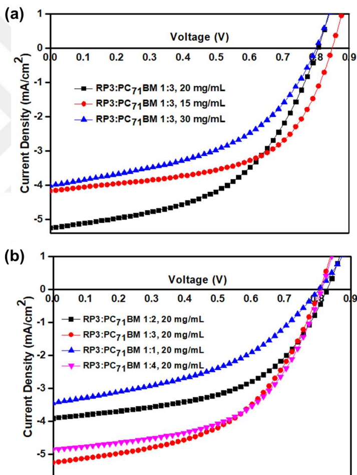
Figure 3.12. J-V curves of the OPV devices based on RP3 :PC 71 BM summarizing optimization of (a) blend concentrations and (b) D/A ratios
