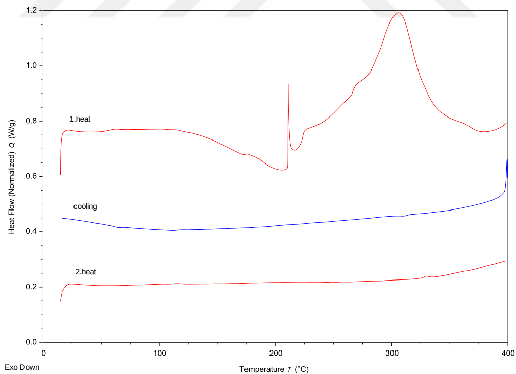
Figure B.10. Thermal analysis result obtained from DSC for P1B
