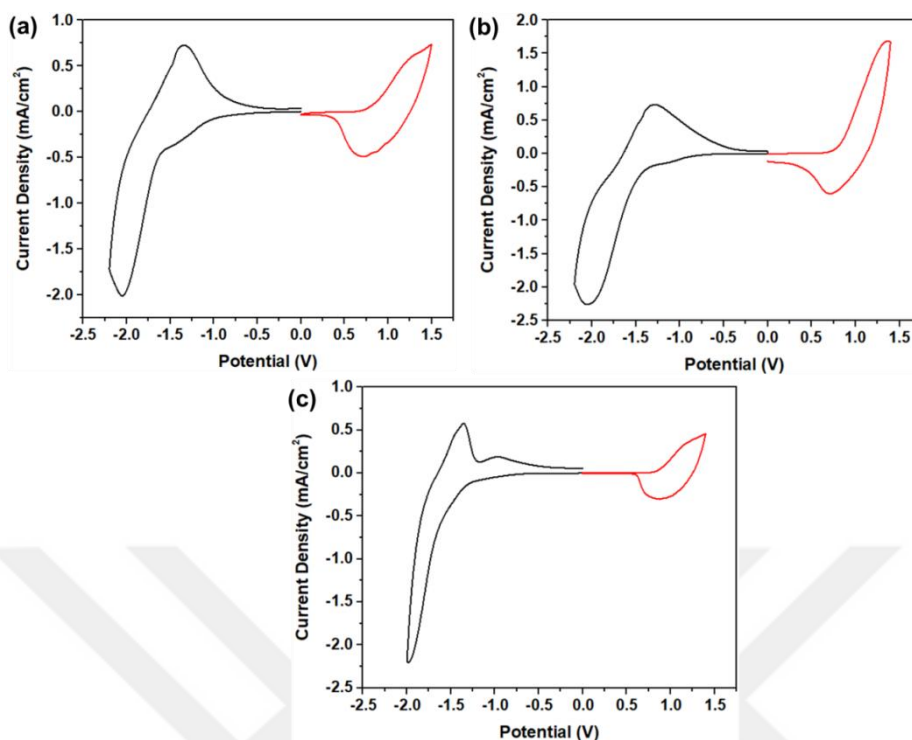
Figure 3.3. Single scan cyclic voltammograms of random polymers (a) RP1 , (b) RP2 and (c) RP3 in 0.1 M TBAPF 6 /ACN electrolyte solution
