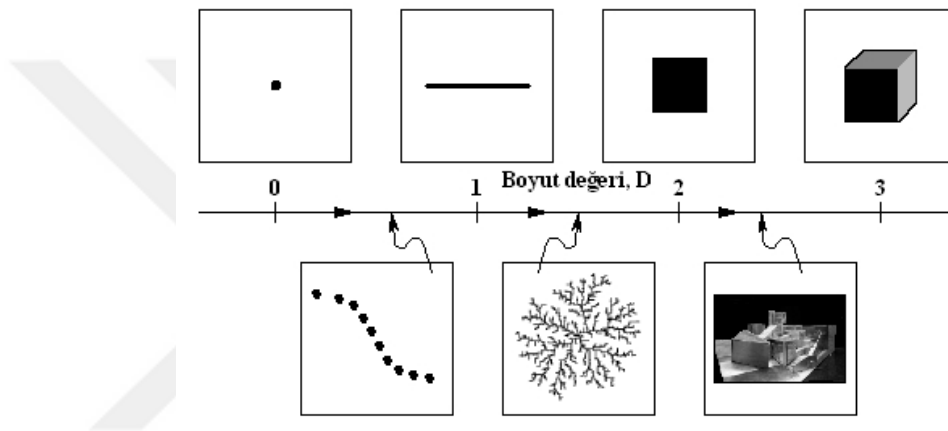
Figure 3-1. Euclidian and fractal dimensions (Kaya, 2003, p. 46)
