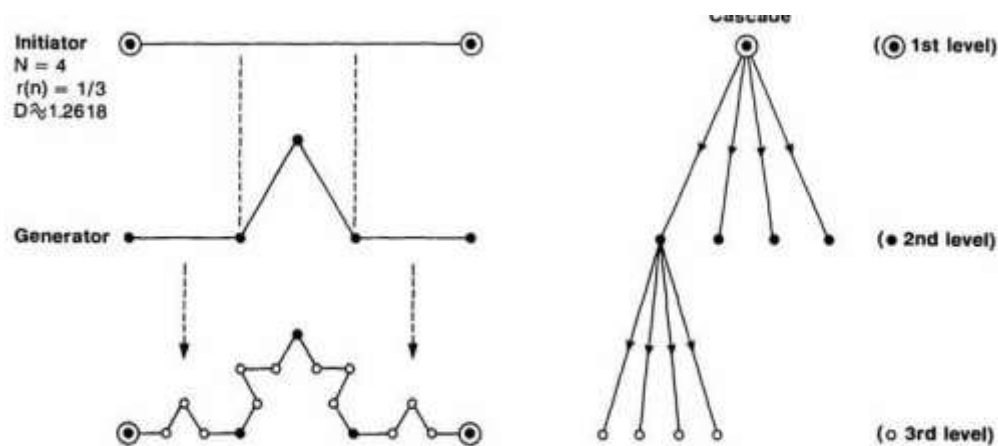
Figure 3-3 The construction of the Koch Curve (Batty & Longley, 1994, p. 62)
