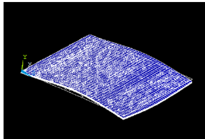
Mode 3 (319.98 Hz)
