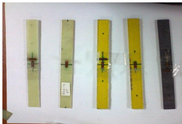
Figure 4.3 Test specimens for strain gauge experiment
