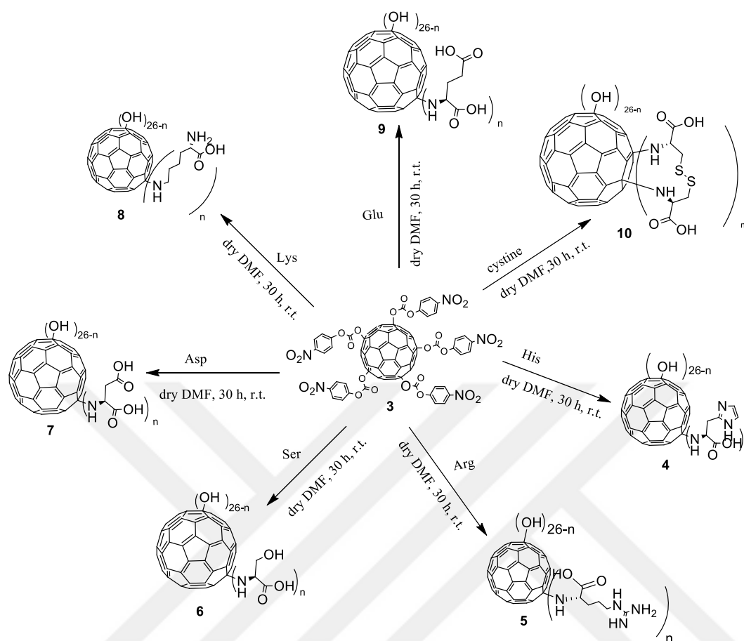
Scheme 1.8 Synthesis of fullerol-amino acid derivatives.
