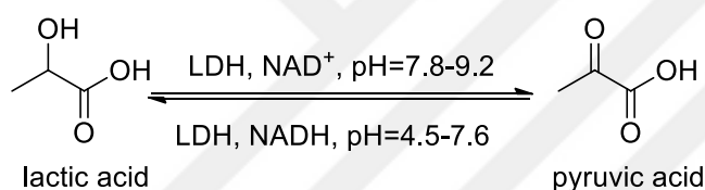
Scheme 1.1 Reaction catalyzed by Lactate dehydrogenase.
