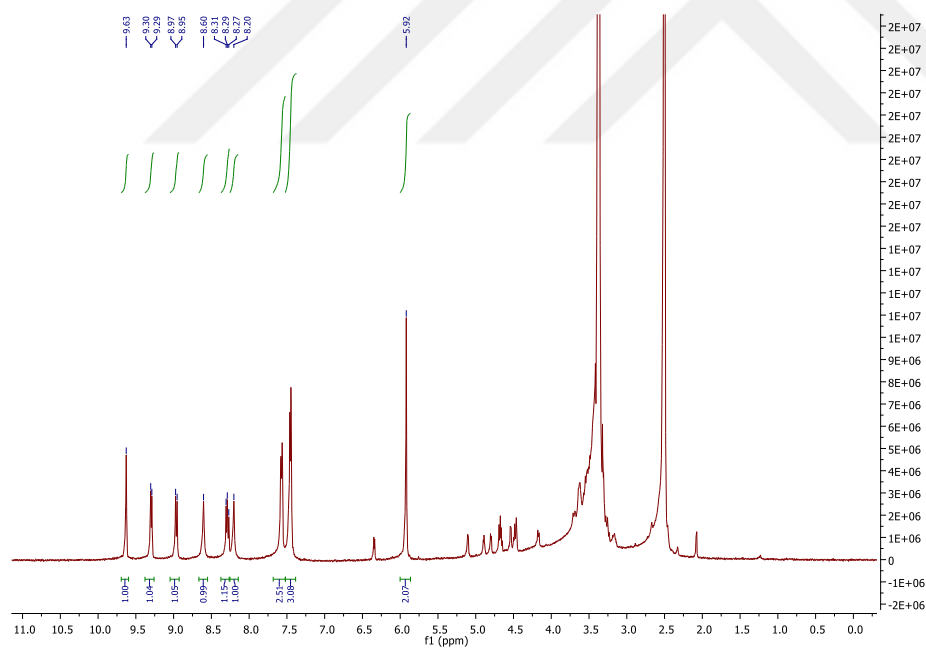
Figure A. 8 ^1\text{H} NMR spectrum of 12.
