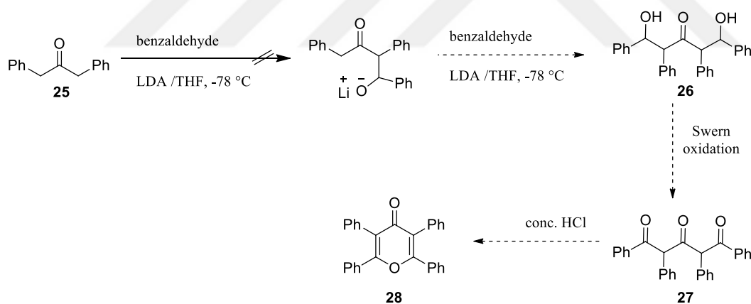
Scheme 2.1 First synthesis attempts for the synthesis of 2,3,4,5-tetraphenyl-4H-pyran-4-one.
