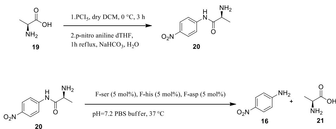
Scheme 1.13 Synthesis of the reactant L-alanine anilide (above), reaction with ser protease mimic (below).
