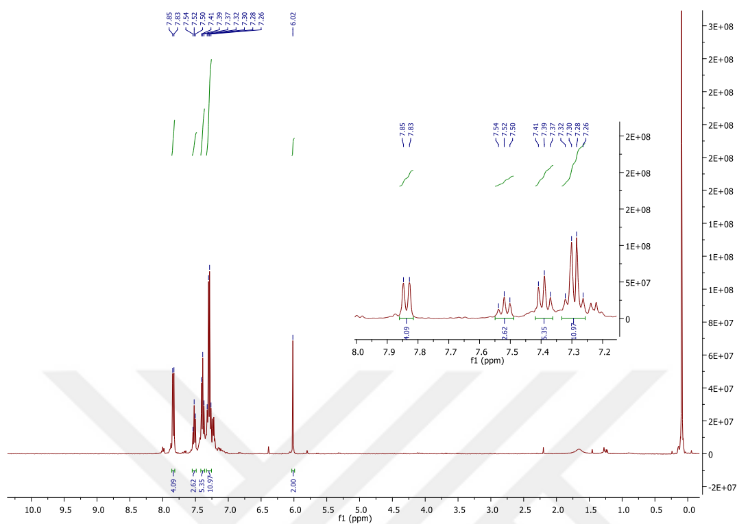
Figure 2.13 ^1\text{H} NMR spectrum of 27 .
