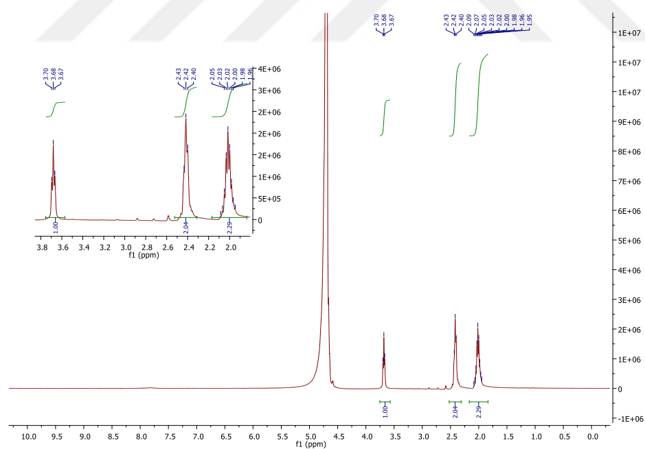
Figure A. 6 ^1\text{H} NMR spectrum of 9.
