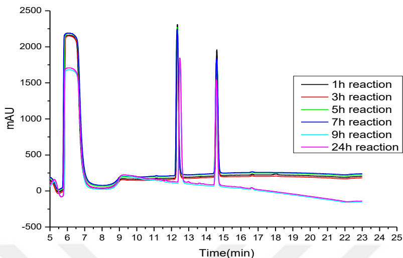
Figure 1.11 HPLC chromatogram of the oxidation reaction with LDH mimics.
