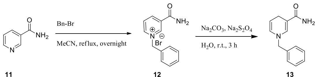
Scheme 1.9 Synthesis scheme of \text{NAD}^+ and NADH coenzyme analogs.
