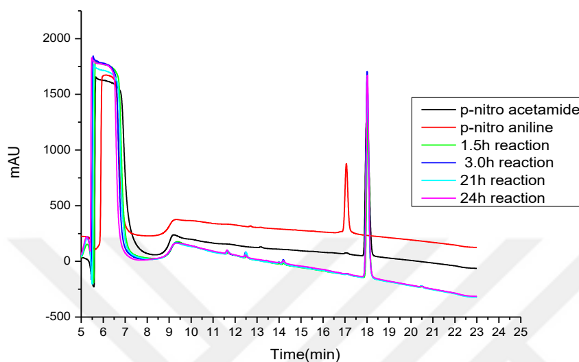
Figure 1.12 HPLC chromatogram of the reaction with ser protease mimic elements.
