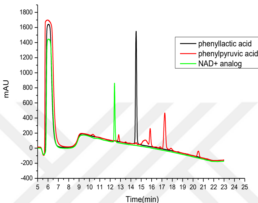
Figure 1.10 HPLC chromatogram of reactant, expected product and NAD + analog.
