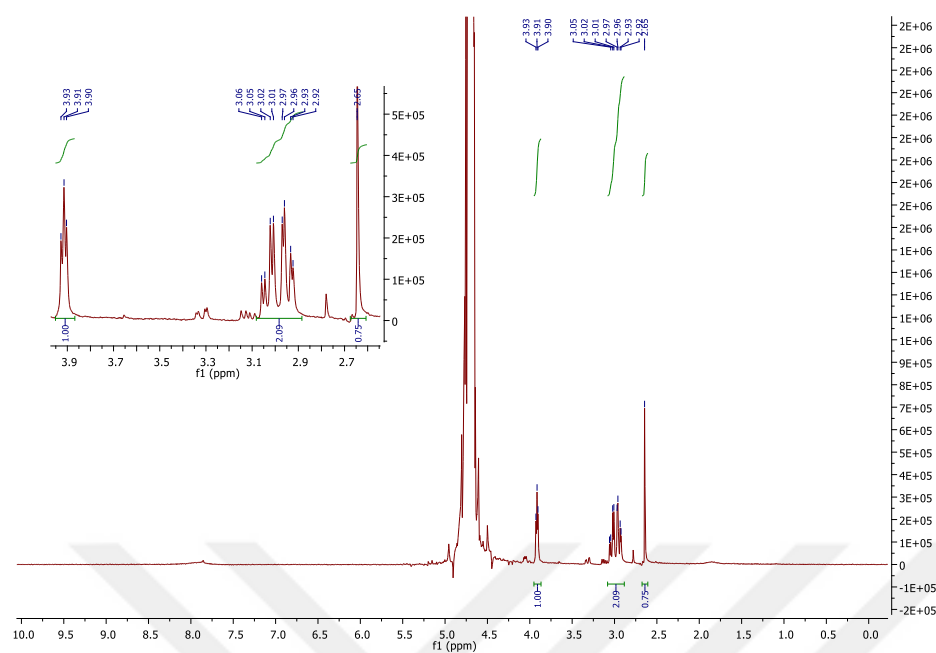
Figure A. 7 ^1\text{H} NMR spectrum of 10.
