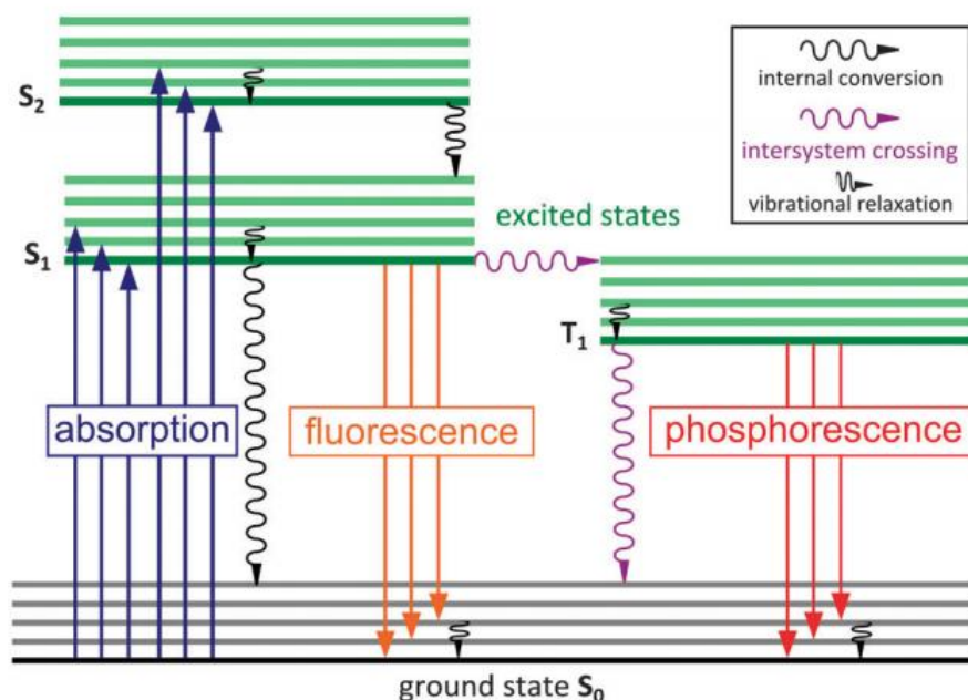
Figure 2.3 Photoluminescence processes in Jablonski diagram. 50
