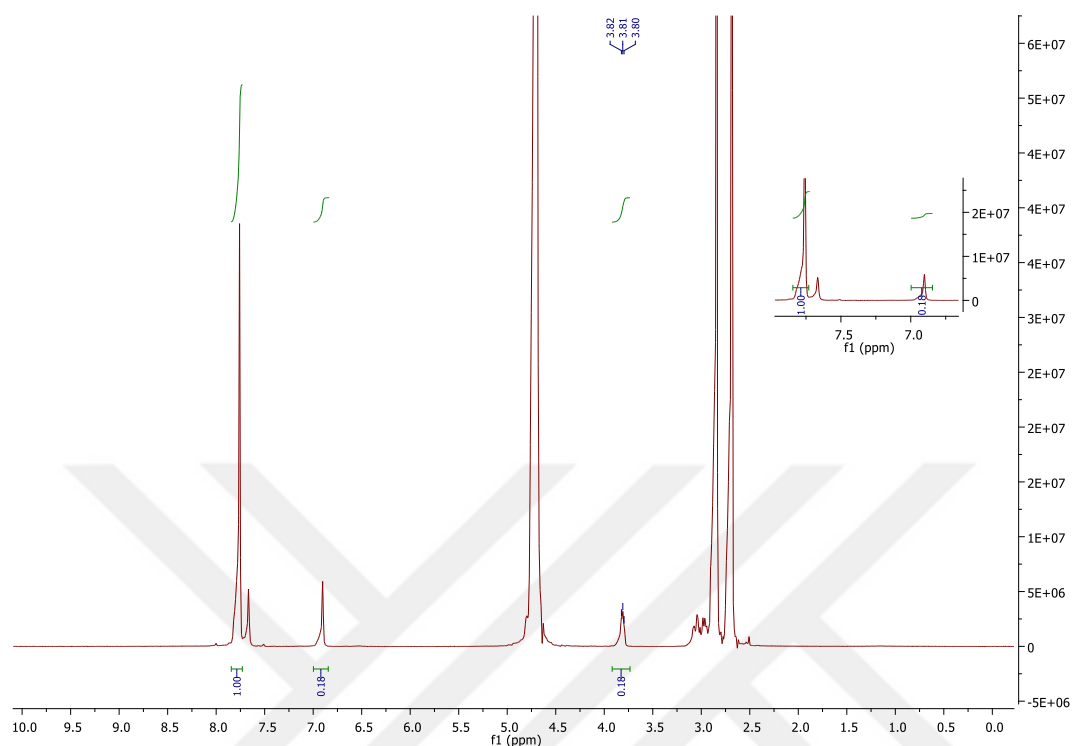
Figure 1.8 ^1\text{H} NMR spectrum of F-His derivative with internal standard DMF.
