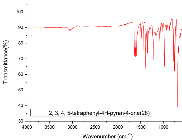
Figure B. 2 IR spectrum of 28.
