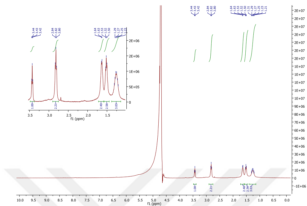
Figure A. 5 ^1\text{H} NMR spectrum of 8.
