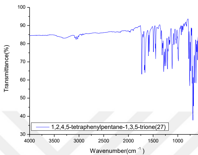
Figure B. 1 IR spectrum of 27.
