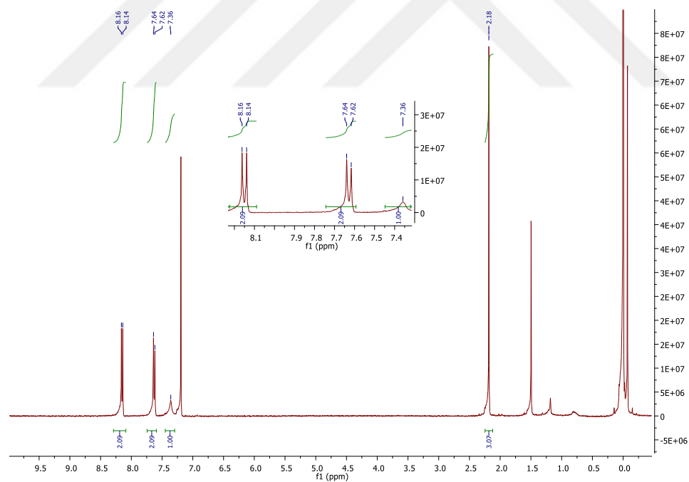
Figure A. 10 ^1\text{H} NMR spectrum of 17.
