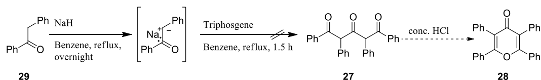
Scheme 2.8 The synthesis of 2,3,4,5-tetraphenyl-4H-pyran-4-one in this study.
