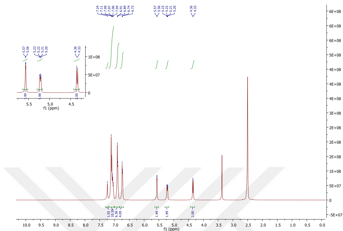
Figure 2.7 ^1\text{H} NMR spectrum of 26.
