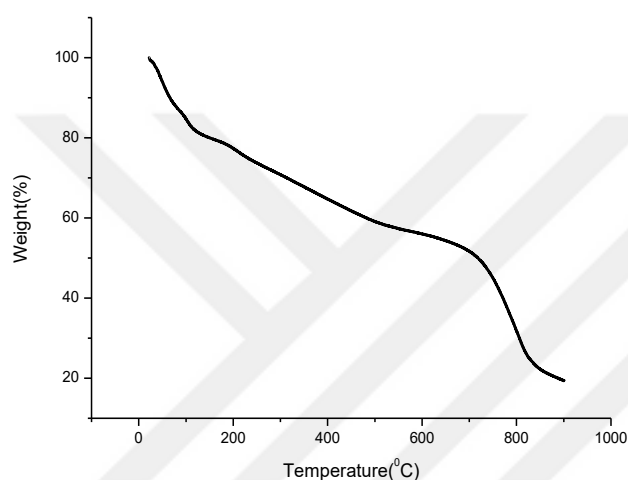
Figure 1.5 TGA thermogram of fullerol.
