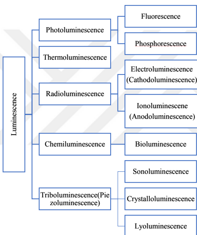
Figure 2.2 Classification of luminescence.
