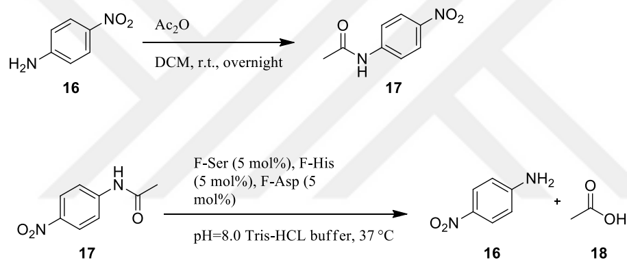
Scheme 1.12 Synthesis of the reactant (above), reaction with ser protease mimic (below).
