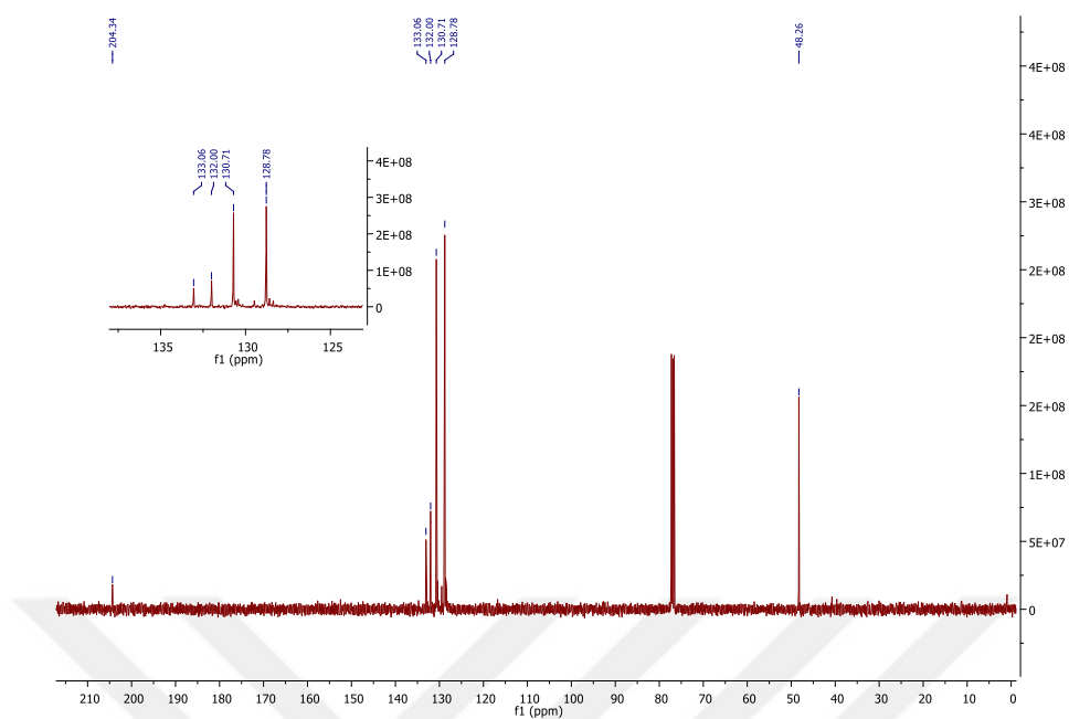
Figure A. ^{13}\text{C} NMR spectrum of 29.
