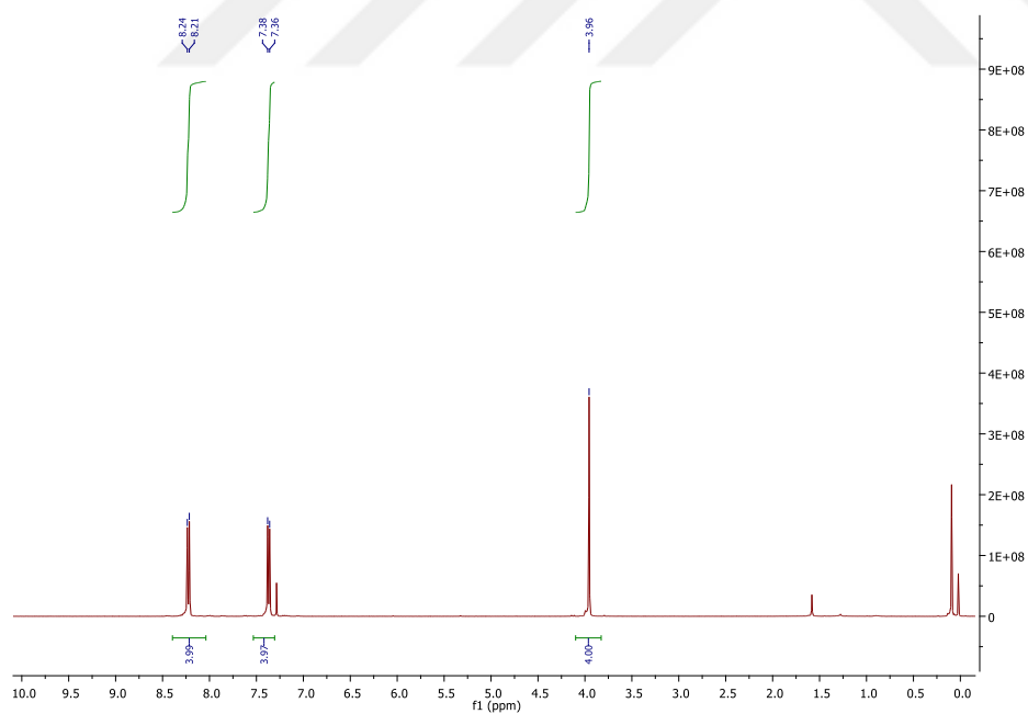
Figure A. 16 ^1\text{H} NMR spectrum of 31.
