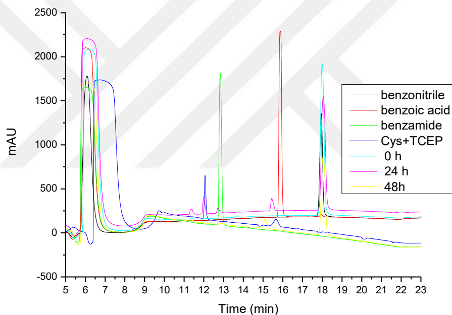
Figure 1.15 HPLC chromatogram of reaction of benzonitrile with active site amino acids.
