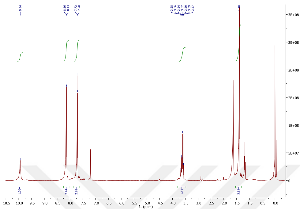
Figure A. 11 ^1\text{H} NMR spectrum of 20.
