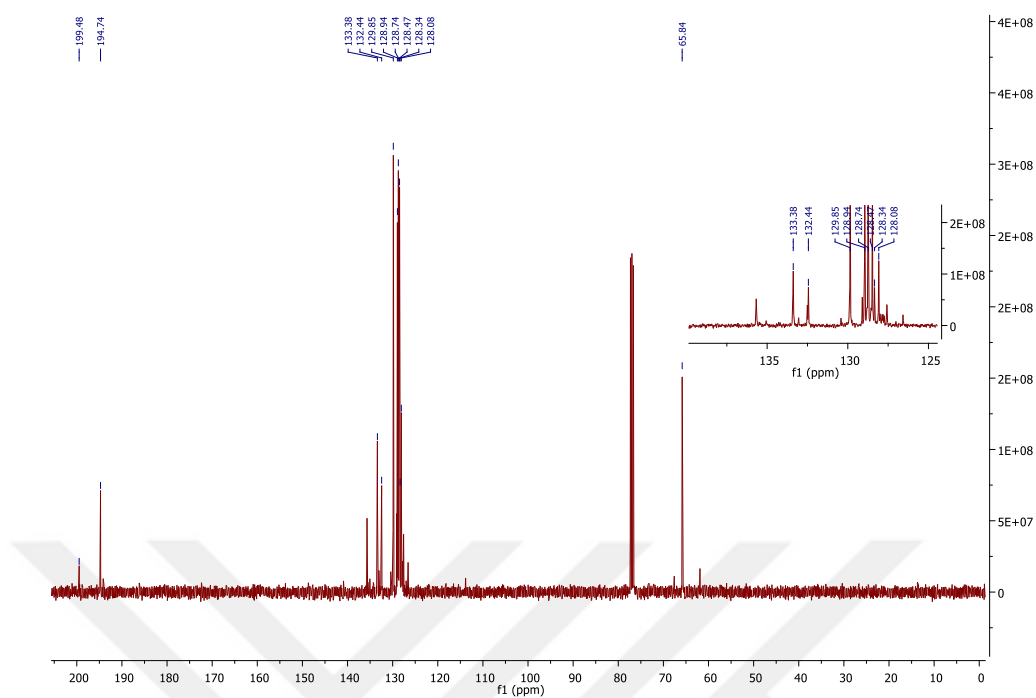
Figure 2.14 ^{13}\text{C} NMR spectrum of 27 .
