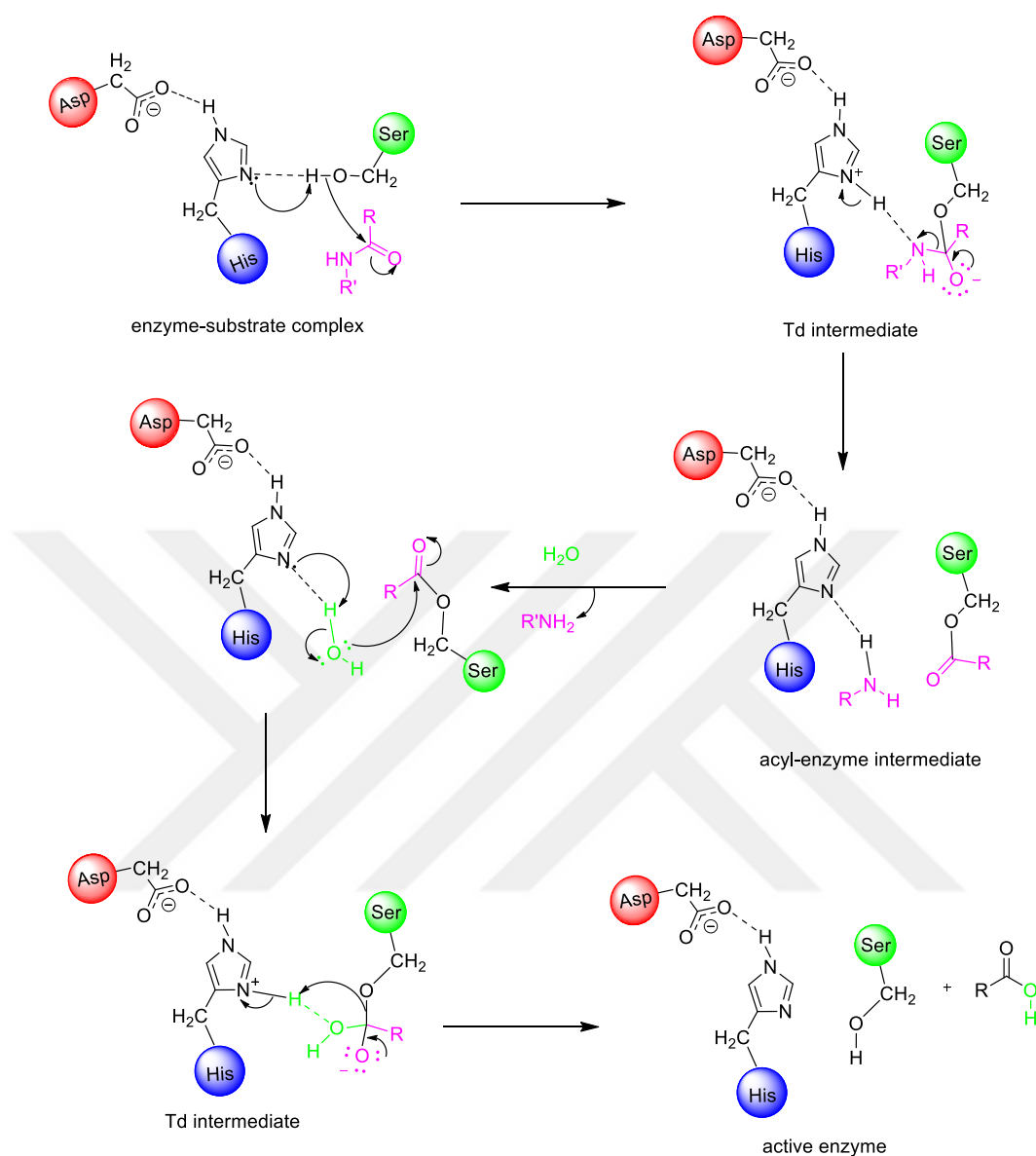
Scheme 1.4 Proposed mechanism of serine protease. 34
