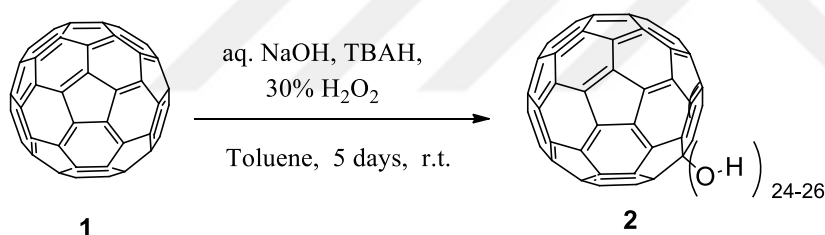
Scheme 1.6 Synthesis of fullerol.
