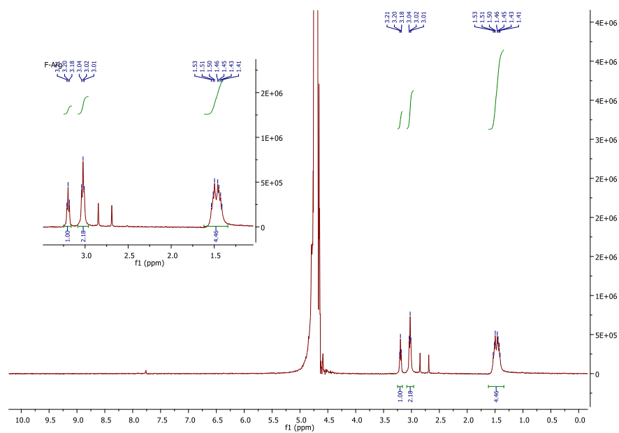
Figure A. 2 ^1\text{H} NMR spectrum of 5.
