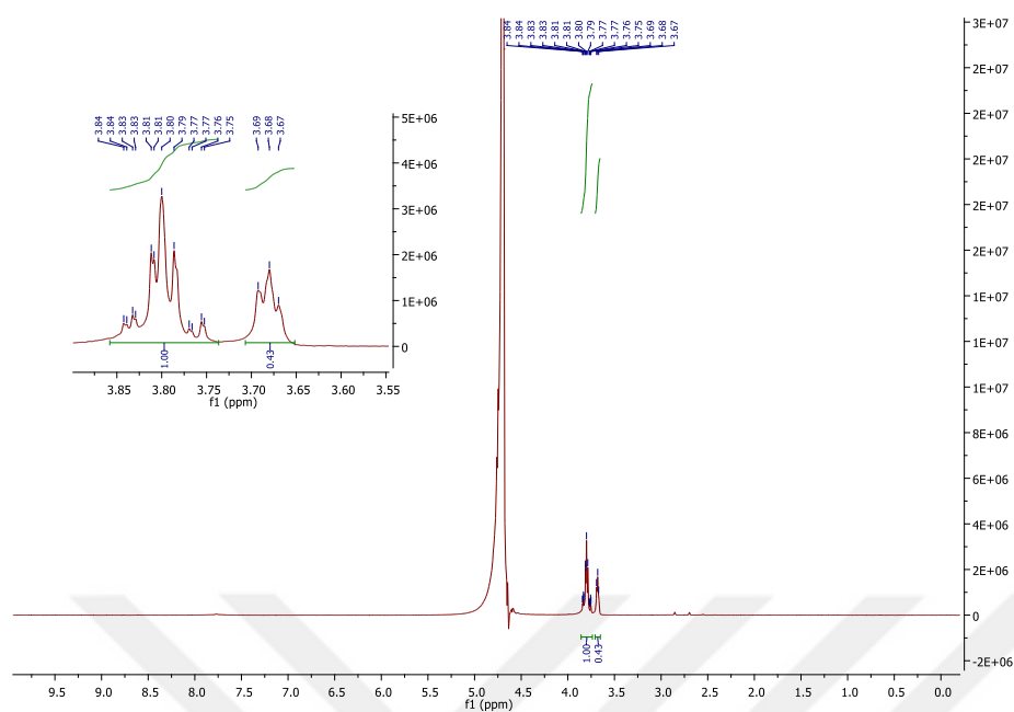
Figure A. 3 ^1\text{H} NMR spectrum of 6.
