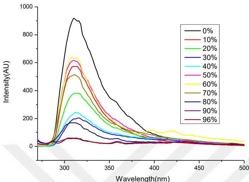
Figure 2.17 Fluorescence spectrum of 28 with varying water %.
