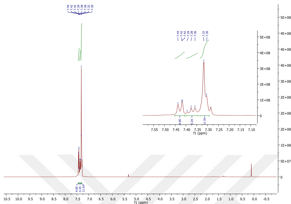
Figure 2.15 ^1\text{H} NMR spectrum of 28 .
