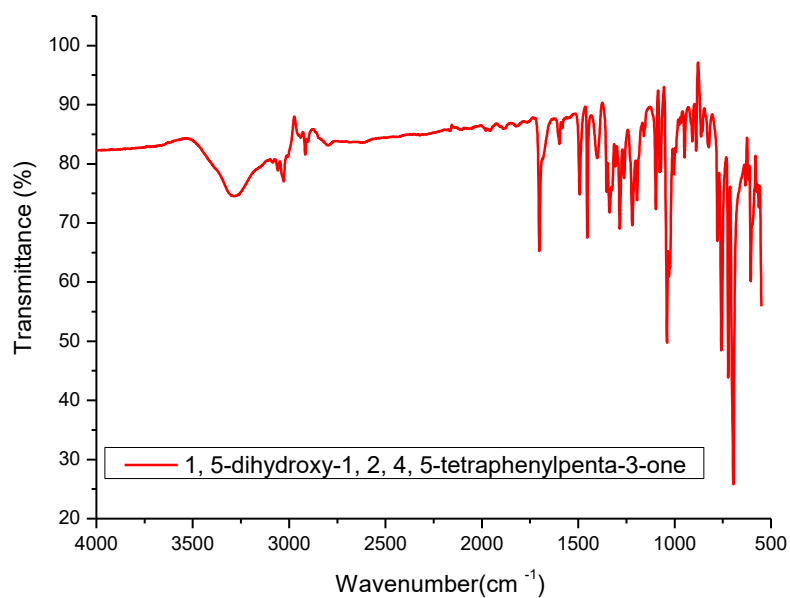
Figure 2.10 IR spectrum of 26.
