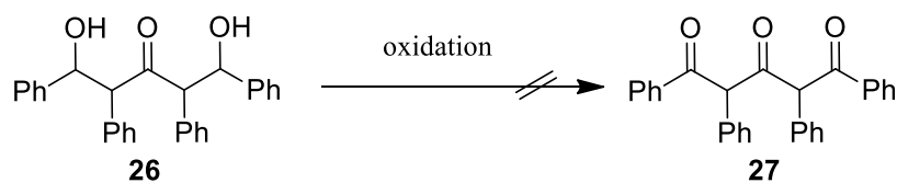
Scheme 2.5 Oxidation of 26 to 27 .
