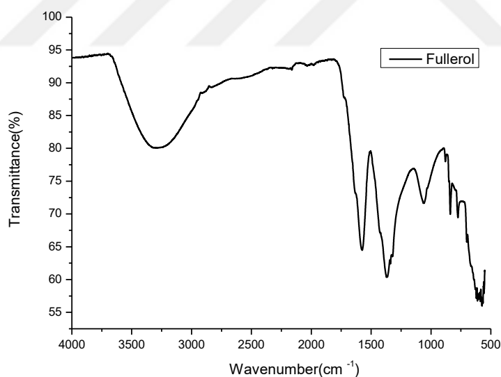
Figure 1.4 IR spectrum of fullerol.
