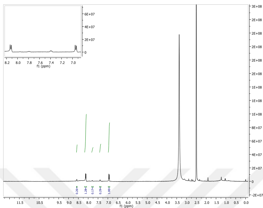
Figure 1.6 ^1\text{H} NMR spectrum of activated fullerol.
