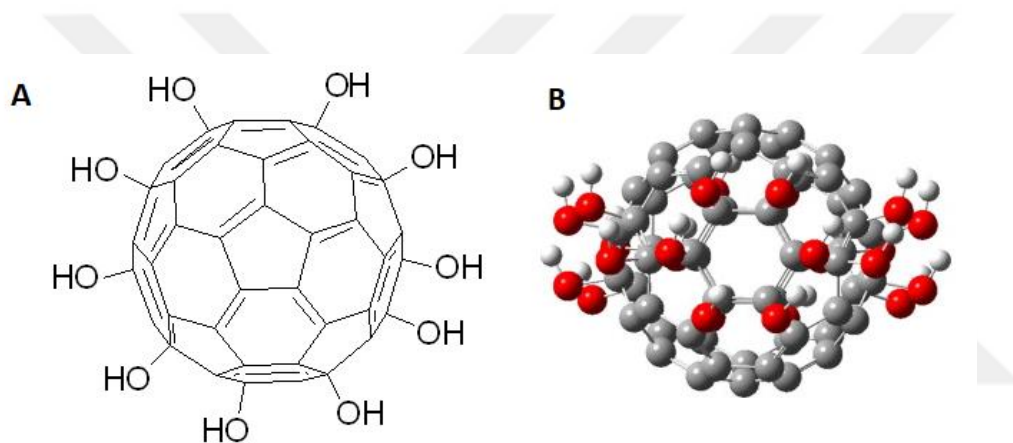
Figure 1.2 Structure of fullerol (A) and hydroxyl groups located on equatorial region (B). Reprinted with permission from (He, H., Zheng, L., Jin, P. & Yang, M. The structural stability of polyhydroxylated C_{60}(OH)_{24} : Density functional theory characterizations. Computational and Theoretical Chemistry 974 , 16–20 (2011).). Copyright © 2011 Elsevier B.V.
