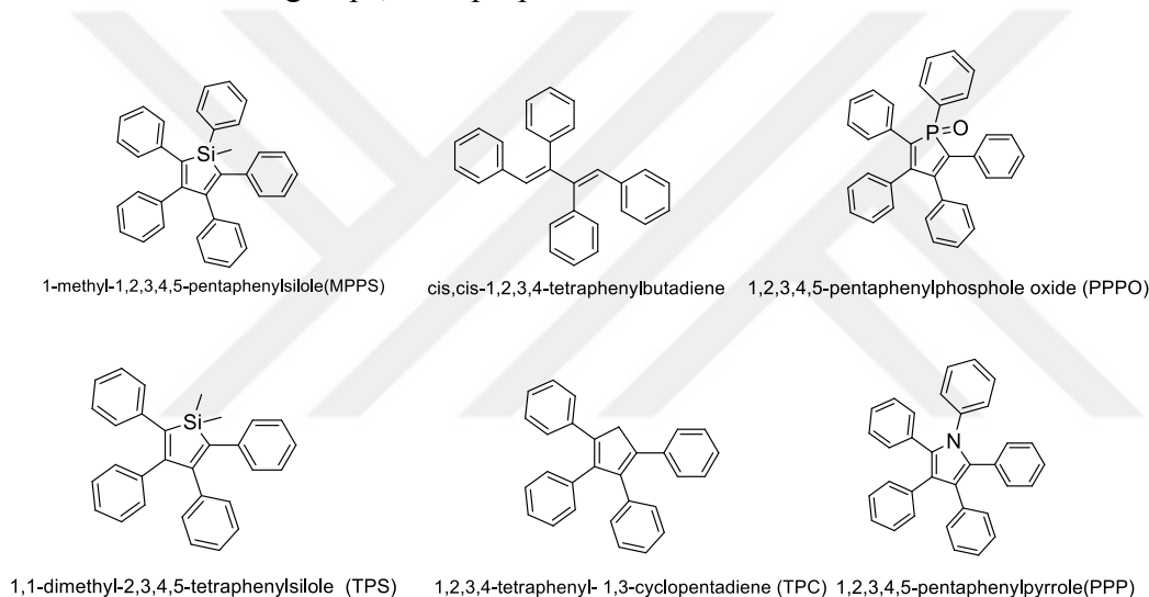
Figure 2.5 Synthesized molecules in the literature with AIE property.
