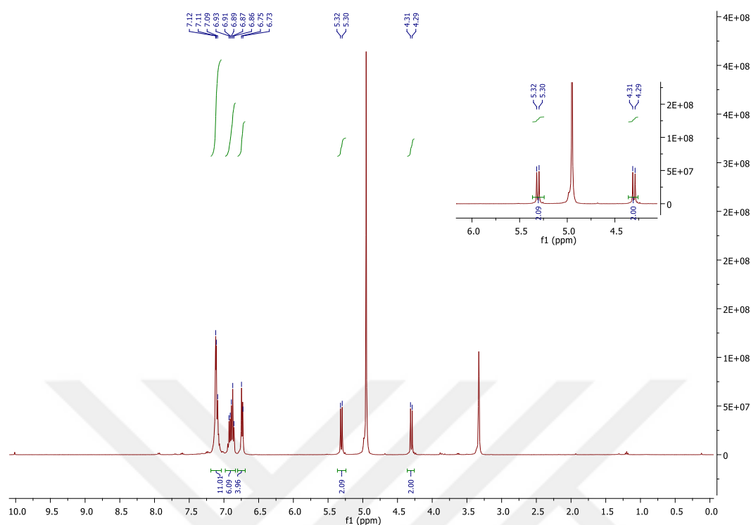
Figure 2.8 ^1\text{H} NMR spectrum of 26 in deuterated methanol.
