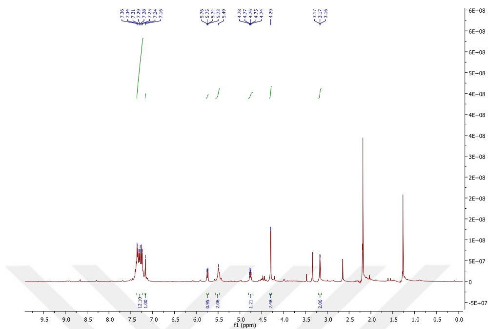
Figure A. 9 ^1\text{H} NMR spectrum of crude 13.
