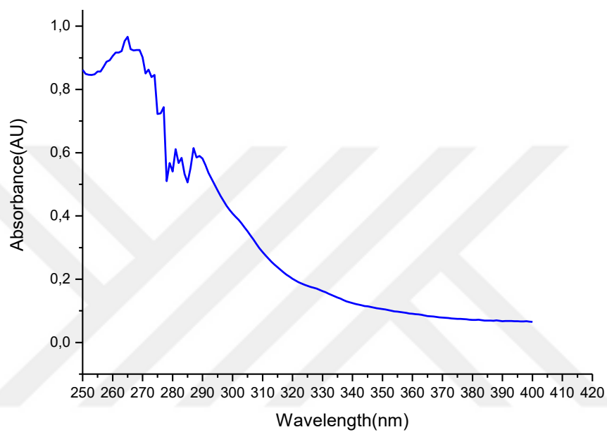
Figure C. 1 UV spectrum of 2,3,5,6-tetraphenyl-4H-pyran-4-one (28) in THF.
