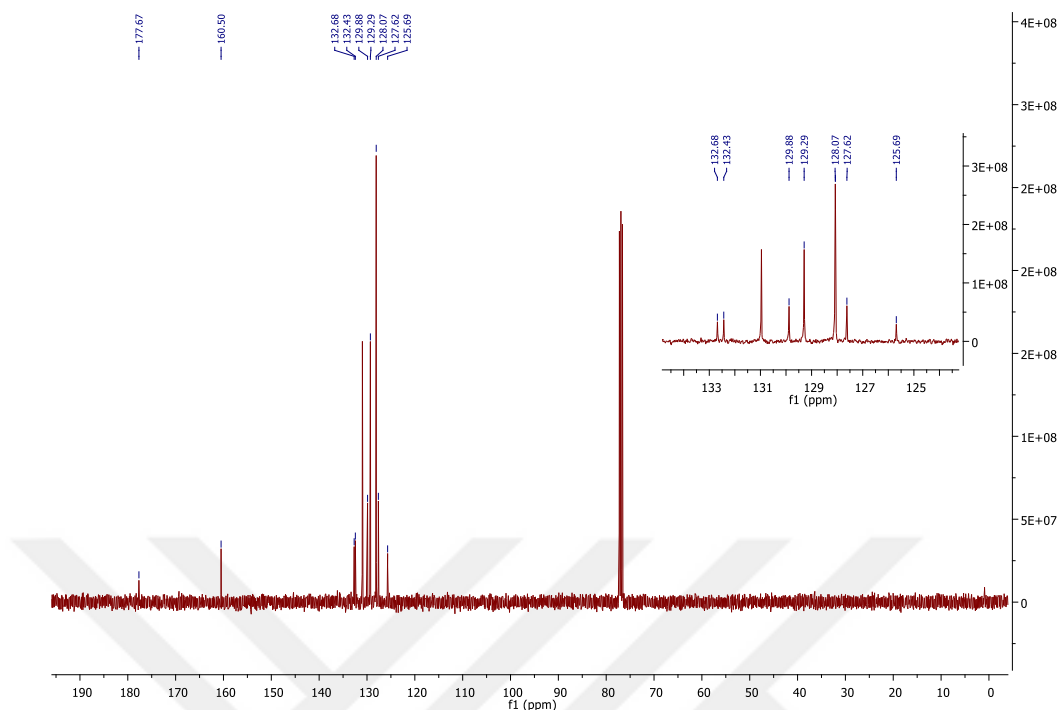
Figure 2.16 ^{13}\text{C} NMR spectrum of 28 .
