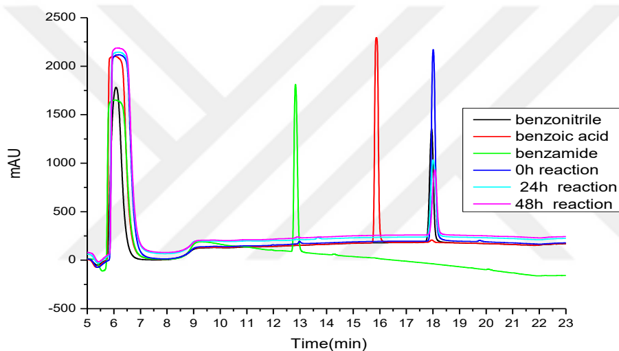
Figure 1.14 HPLC chromatogram of benzonitrile in sodium carbonate-sodium bicarbonate buffer at 50 °C.
