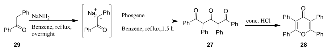
Scheme 2.7 The synthesis of 2, 3, 4, 5-tetraphenyl-4H-pyran-4-one in the literature.
