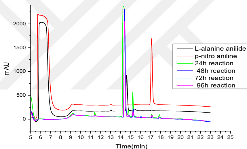
Figure 1.13 HPLC chromatogram of the reaction with ser protease mimic elements.
