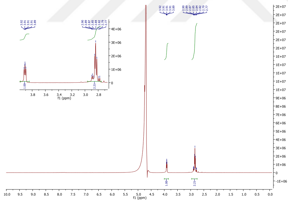
Figure A. 4 ^1\text{H} NMR spectrum of 7.
