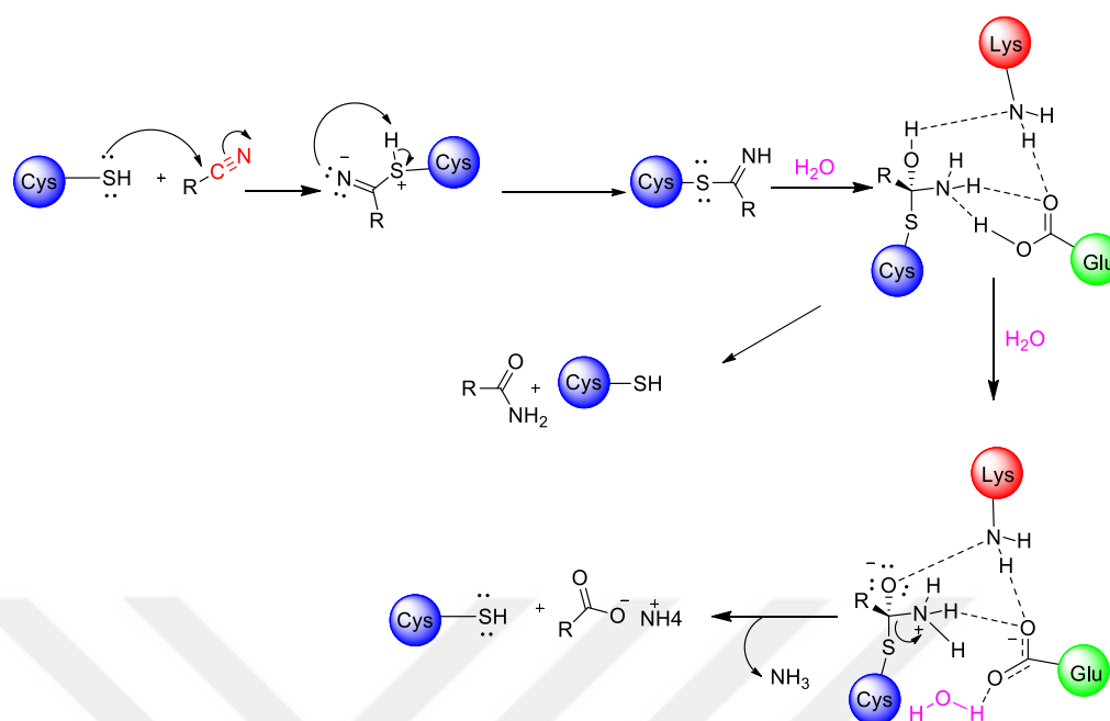
Scheme 1.5 Proposed mechanism for the nitrilase. 38
