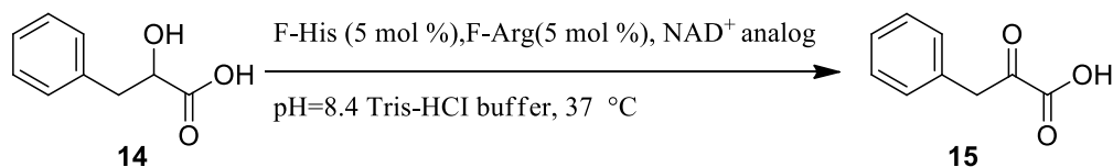
Scheme 1.10 Oxidation reaction with LDH mimics.
