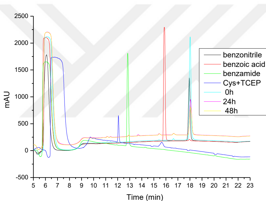
Figure 1.16 HPLC chromatogram of reaction of benzonitrile with Cys, F-Glu and F-Lys.
