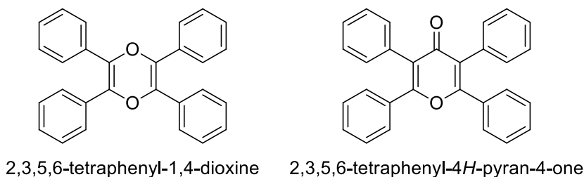
Figure 2.6 Previously synthesized dioxin derivative (left) and the molecule aimed to be synthesized in this study (right).
