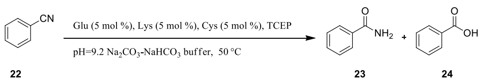
Scheme 1.14 Reaction of benzonitrile with active site amino acids.
