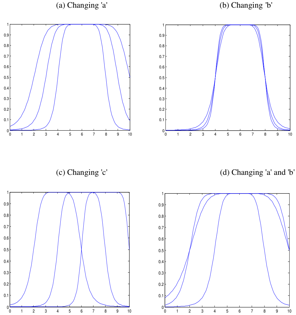
Figure 2.4 The effects of changing parameters in bell MFs: (a) changing parameters a ; (b) changing parameters b ; (c) changing parameters c ; (d) changing a and b simultaneously but keeping their ratio constant.
