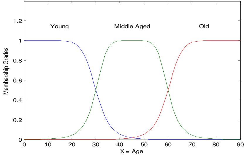
Figure 2.2 Typical MF's of linguistic values "young" "middle aged" and "old."
