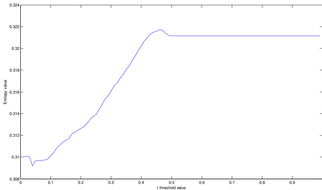
Figure 5.8 The chart of entropy depending on t value
