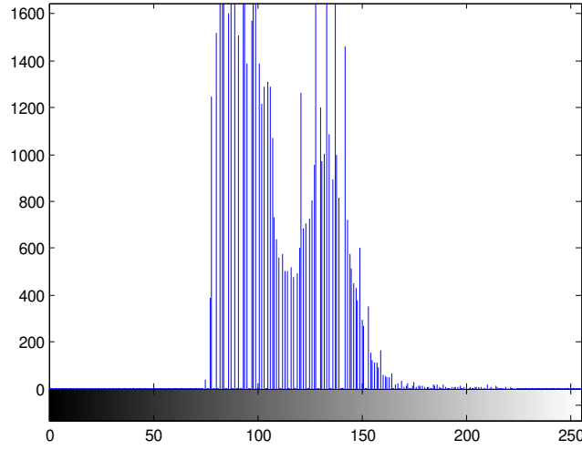
Figure 5.1 An example of set Q histogram
