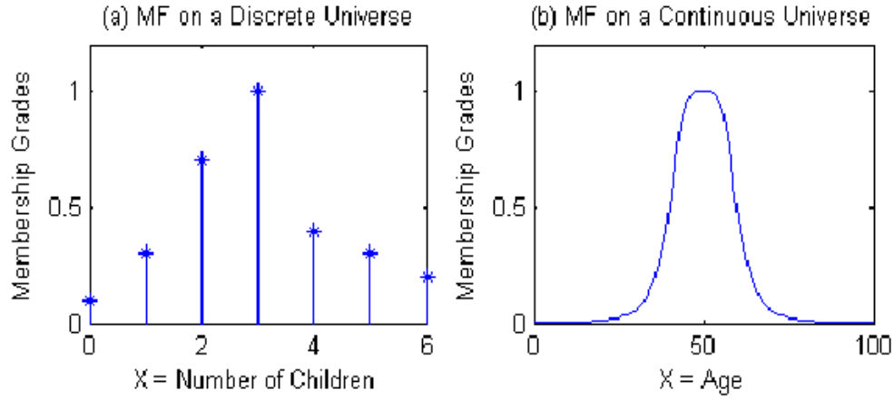
Figure 2.1 (a) A = “sensible number of children in a family”; (b) B = “about 50 years old.”
