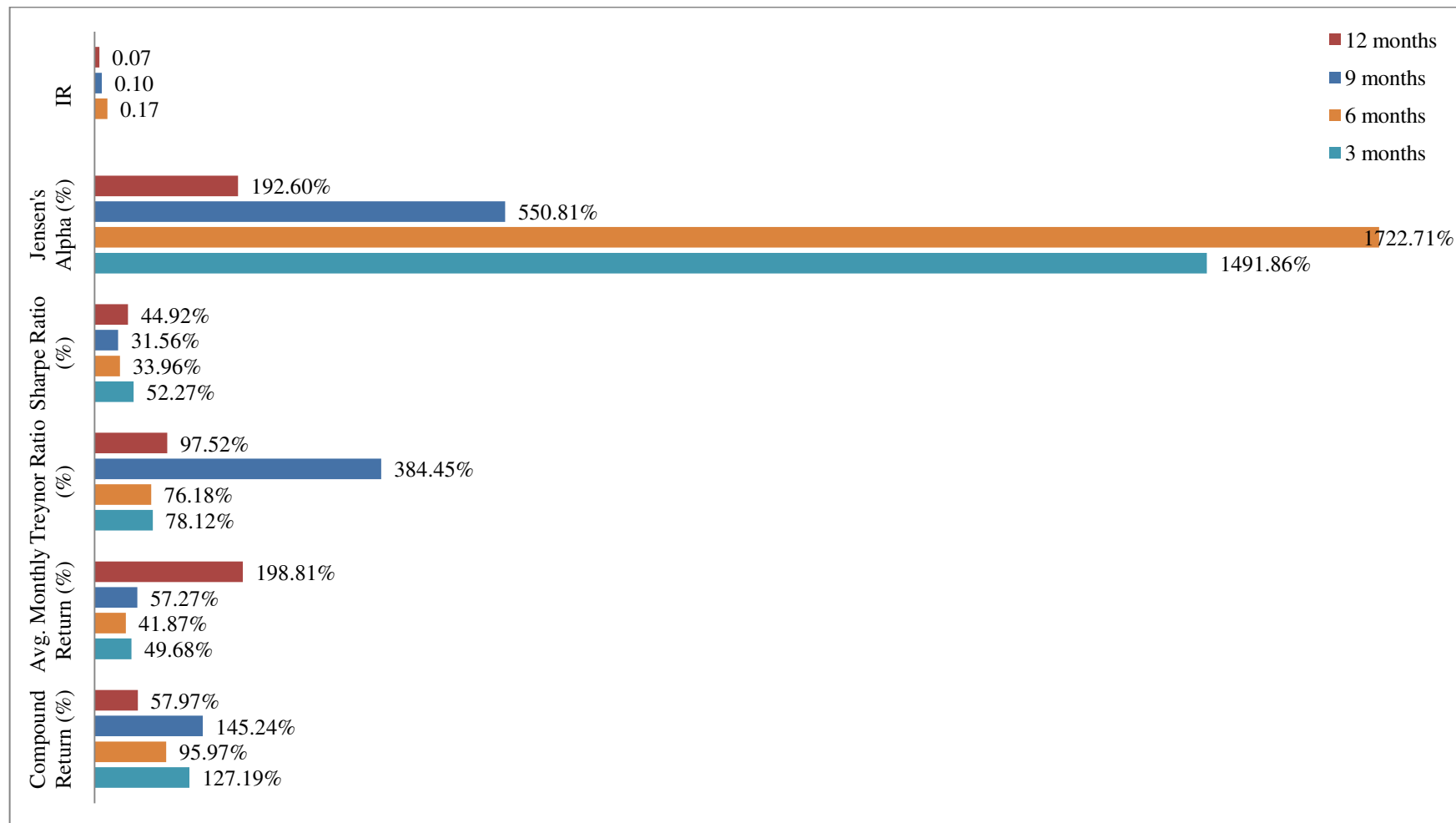
Figure 6.6 Average performance levels relative to benchmark index for different investment period lengths.
