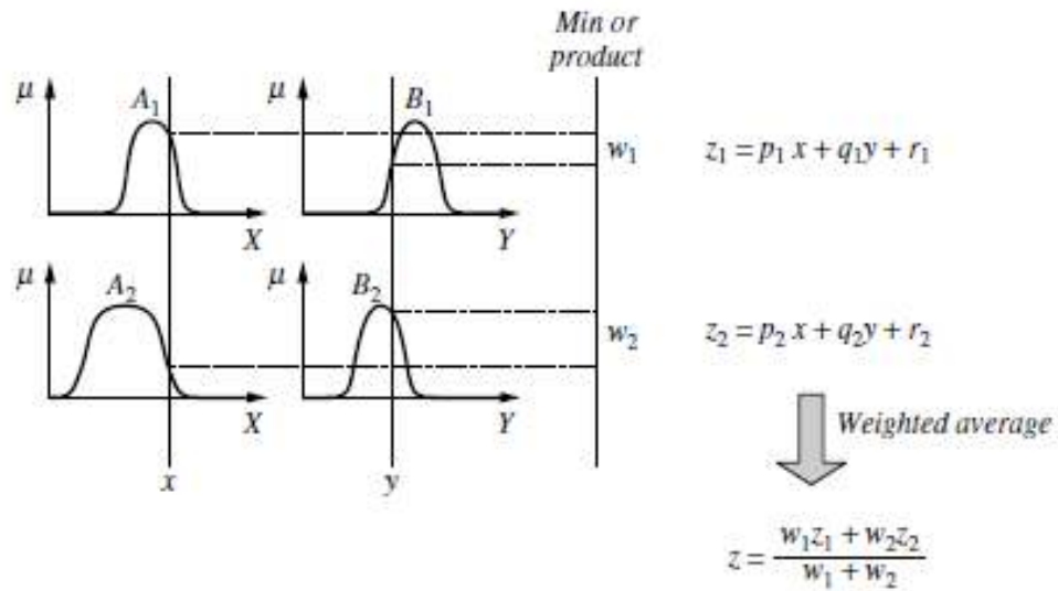
Figure 4.11 TSK fuzzy model (Jang, et. al., 1997).
