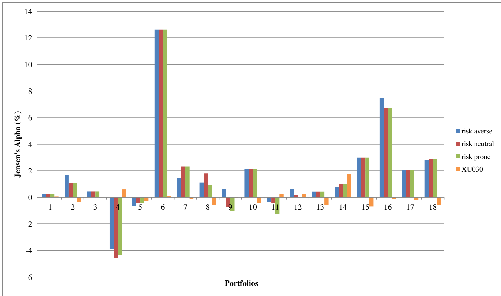
Figure 6.5 Performance evaluation results of the proposed ES in terms of Jensen's alpha for different risk profiles.
