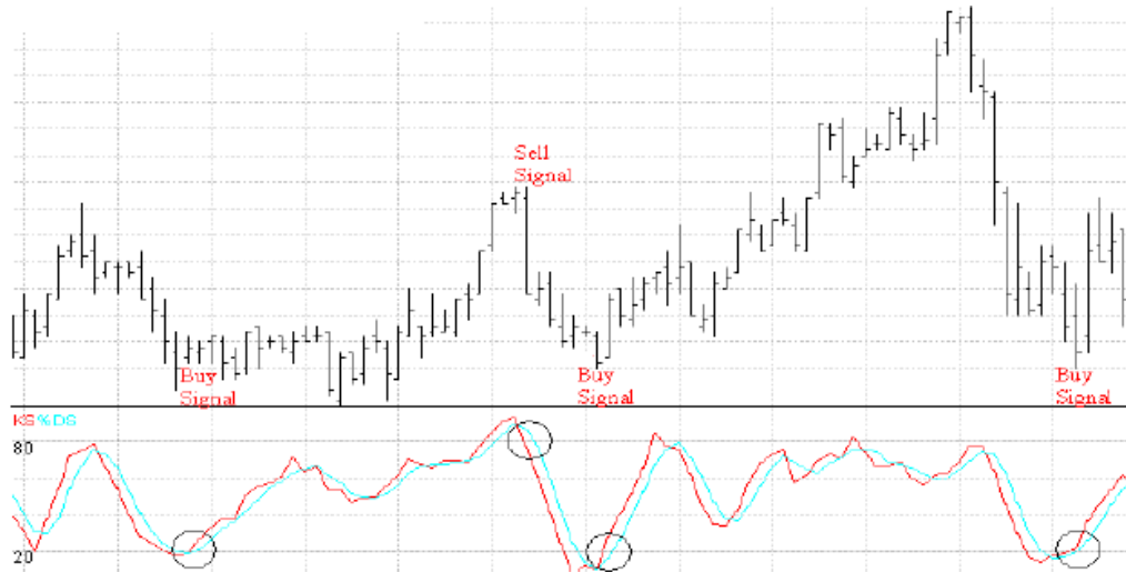
Figure 3.10 Buy and sell signals generated by stochastic oscillator (realtimeforex, n.d.).
