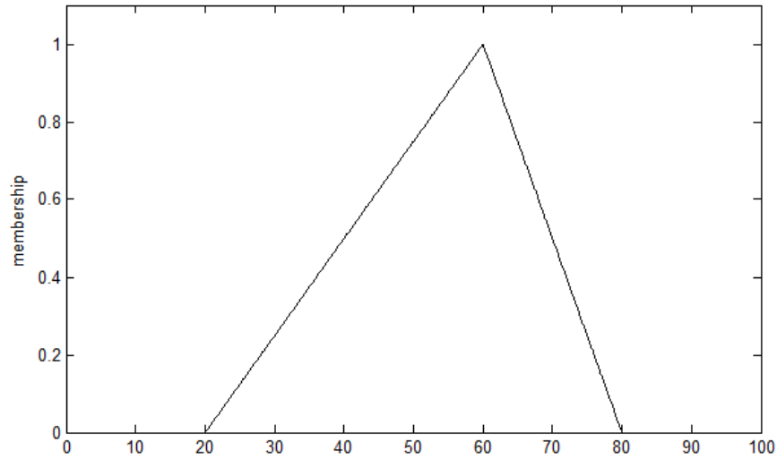
Figure 4.4 Triangular MF.
