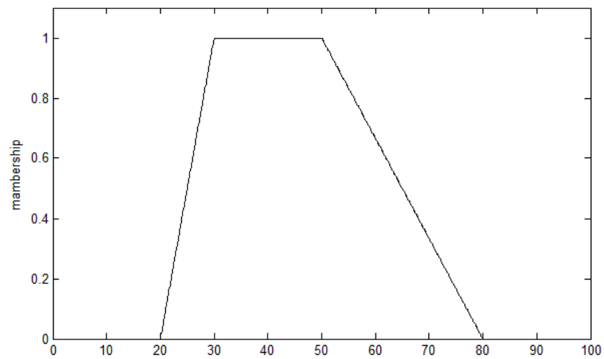
Figure 4.5 Trapezoidal MF.
