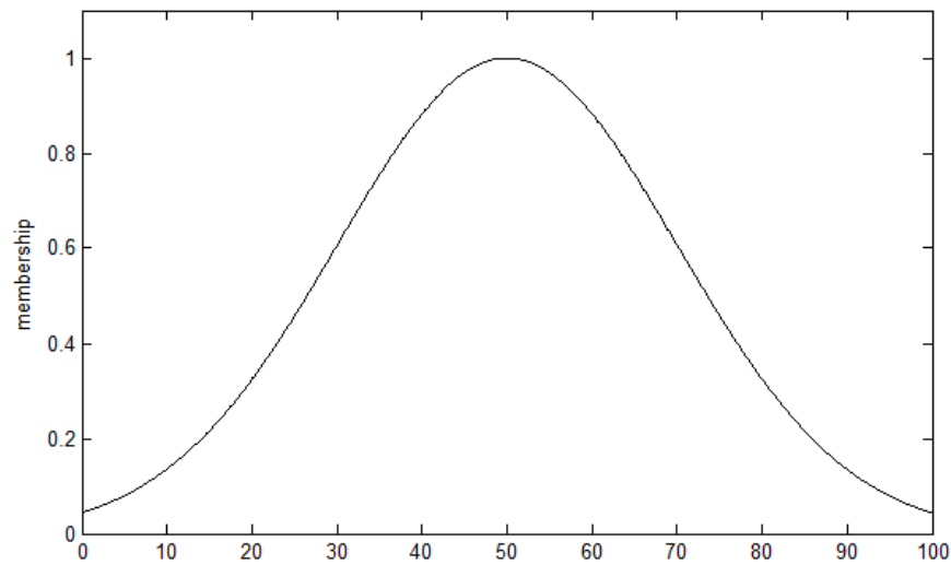
Figure 4.6 Gaussian MF.
