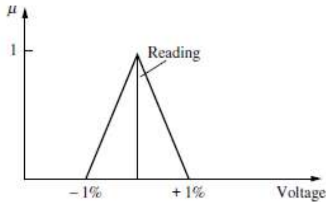
Figure 4.8 MF representing imprecision in “crisp voltage reading” (Ross, 2004).
