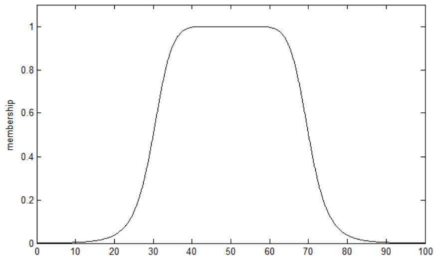
Figure 4.7 Bell MF.
