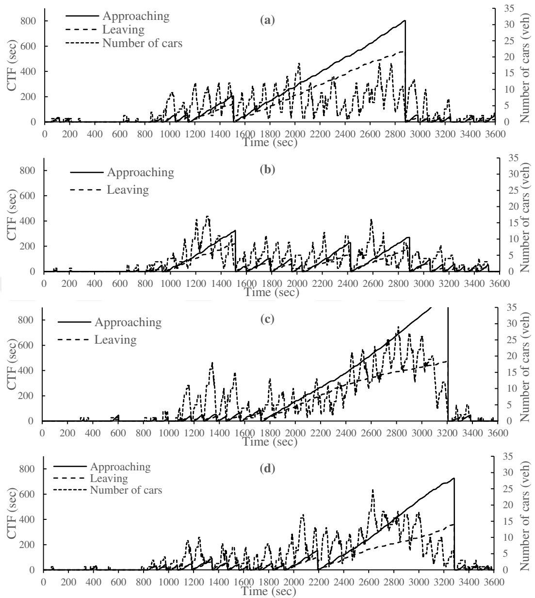
Figure 4.3 Estimated patterns versus real data for incoming edges with (a) 180^\circ (b) 0^\circ (c) 90^\circ and (d) -90^\circ direct.
