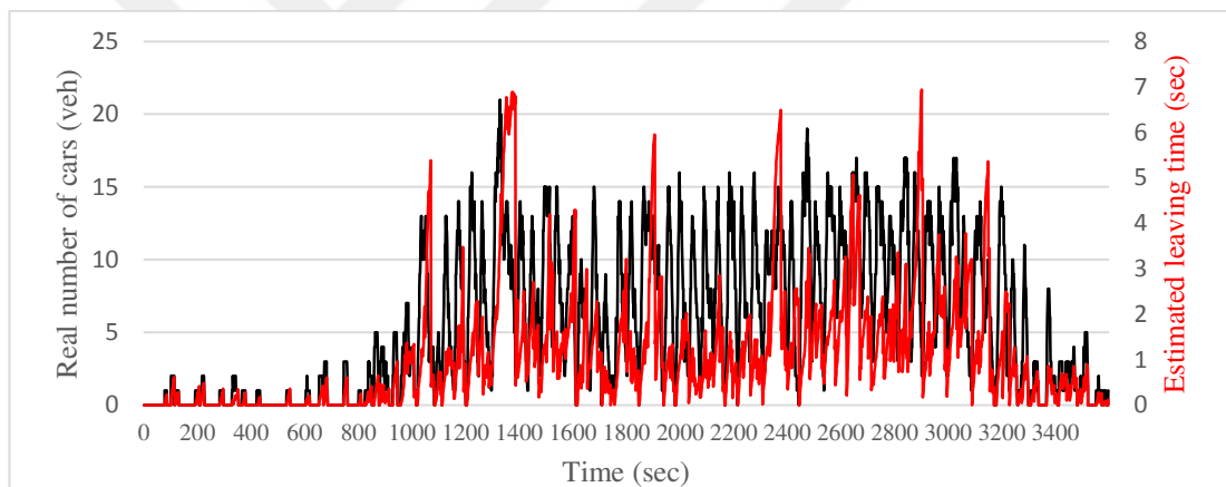
Figure 3.5 Leaving time estimated with real number of cars.
