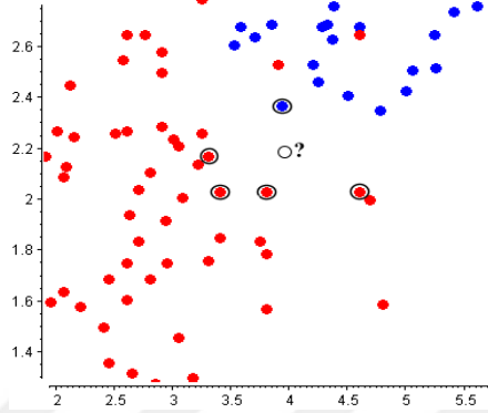
Figure 3.12 k-NN sample
