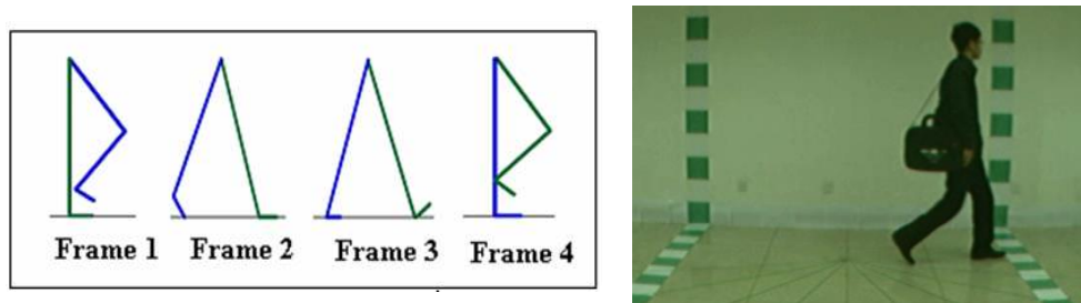
Figure 3.8 Bezier Curves [33].
