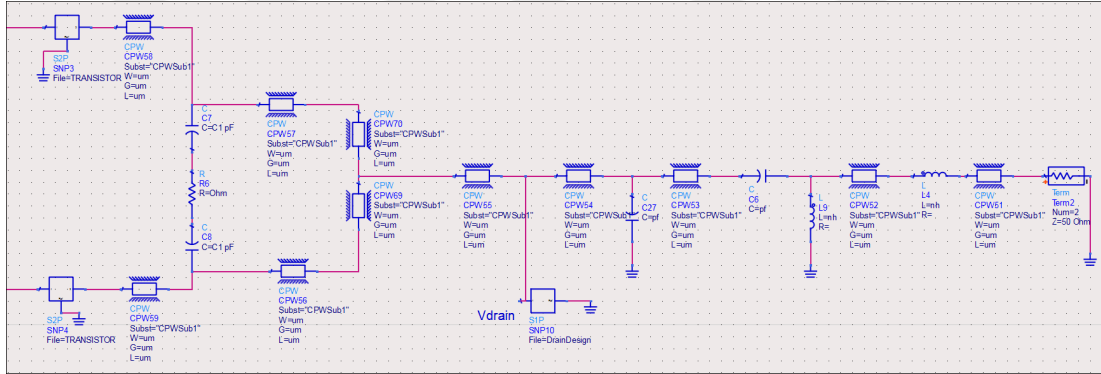
Figure 3.25: Output matching circuit with CPW structures
