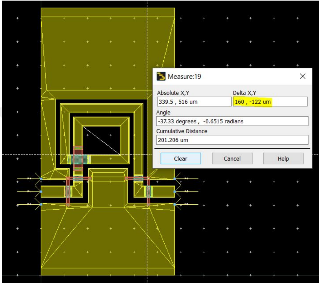
Figure 3.57: Designed inductor layout
