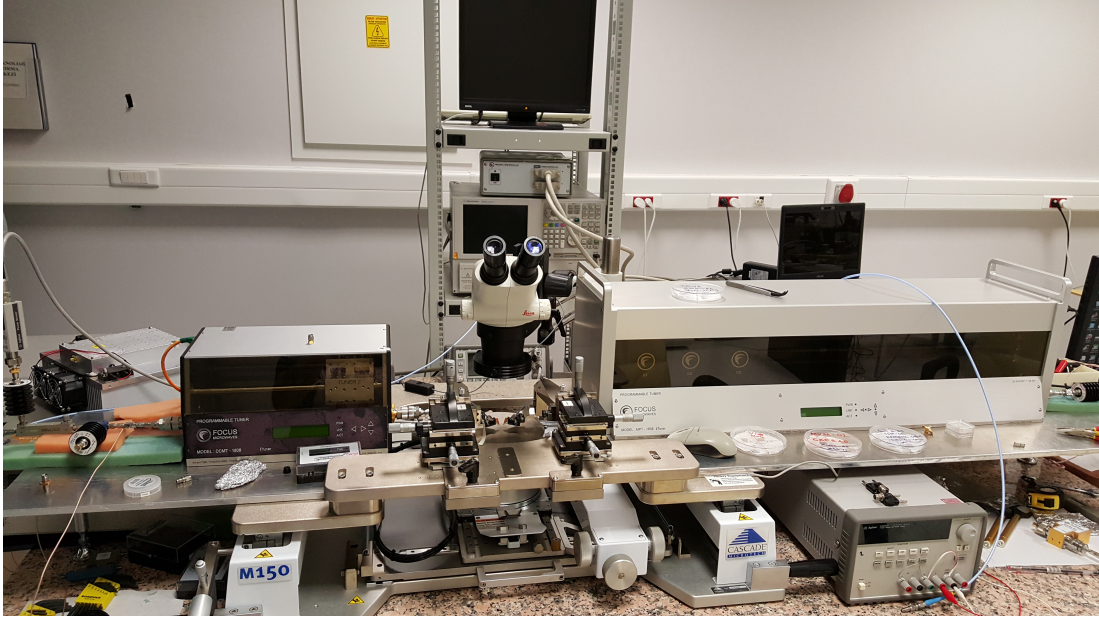
Figure 3.7: Load-Pull measurement setup
