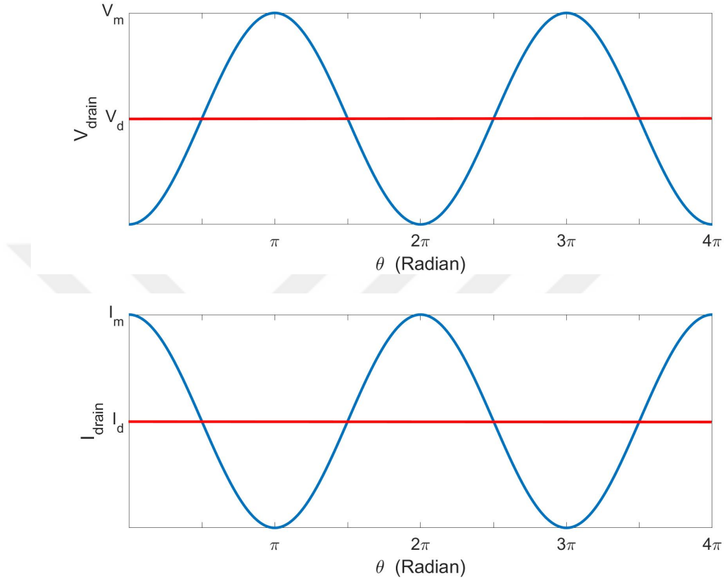
Figure 2.2: Class A Amplifier Waveforms
