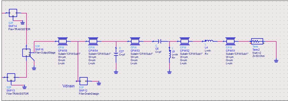
Figure 3.35: Output matching circuit
