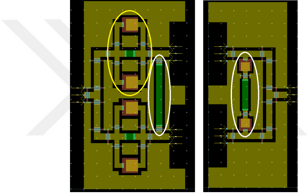
Figure 3.33: Initial input (left) and output (right) stages of the PA layout
