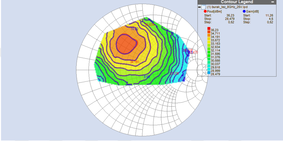
Figure 3.8: Transistor output power contour
