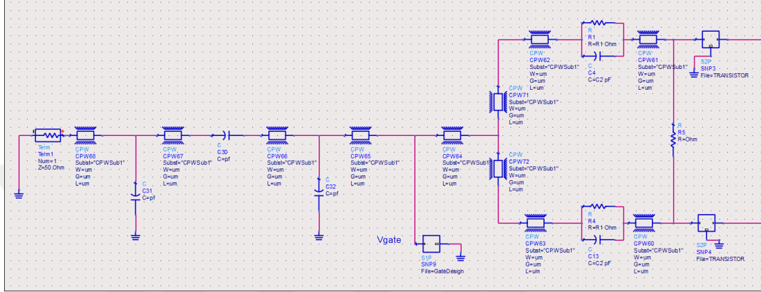
Figure 3.24: Input matching circuit with CPW structures
