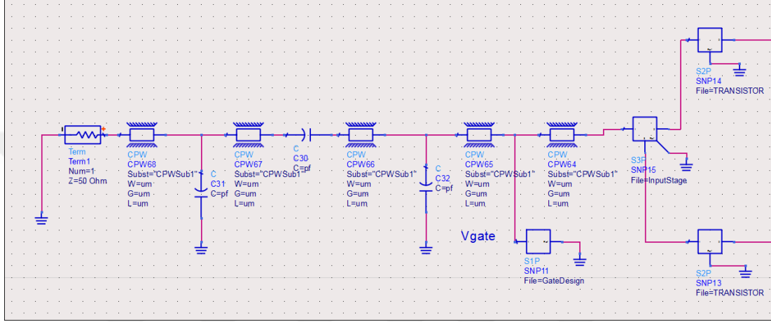
Figure 3.34: Input matching circuit
