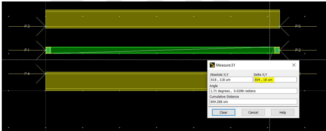
Figure 3.55: Designed resistor layout
