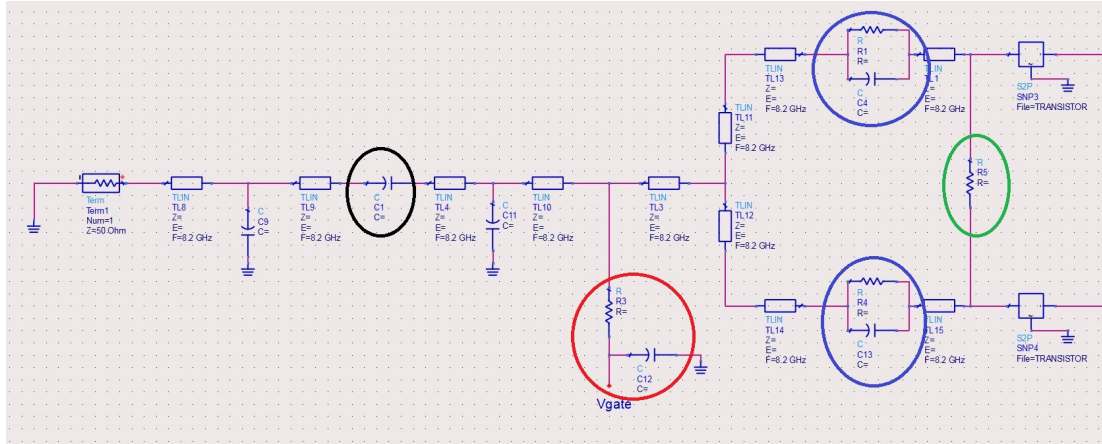
Figure 3.15: Input matching circuit with ideal elements
