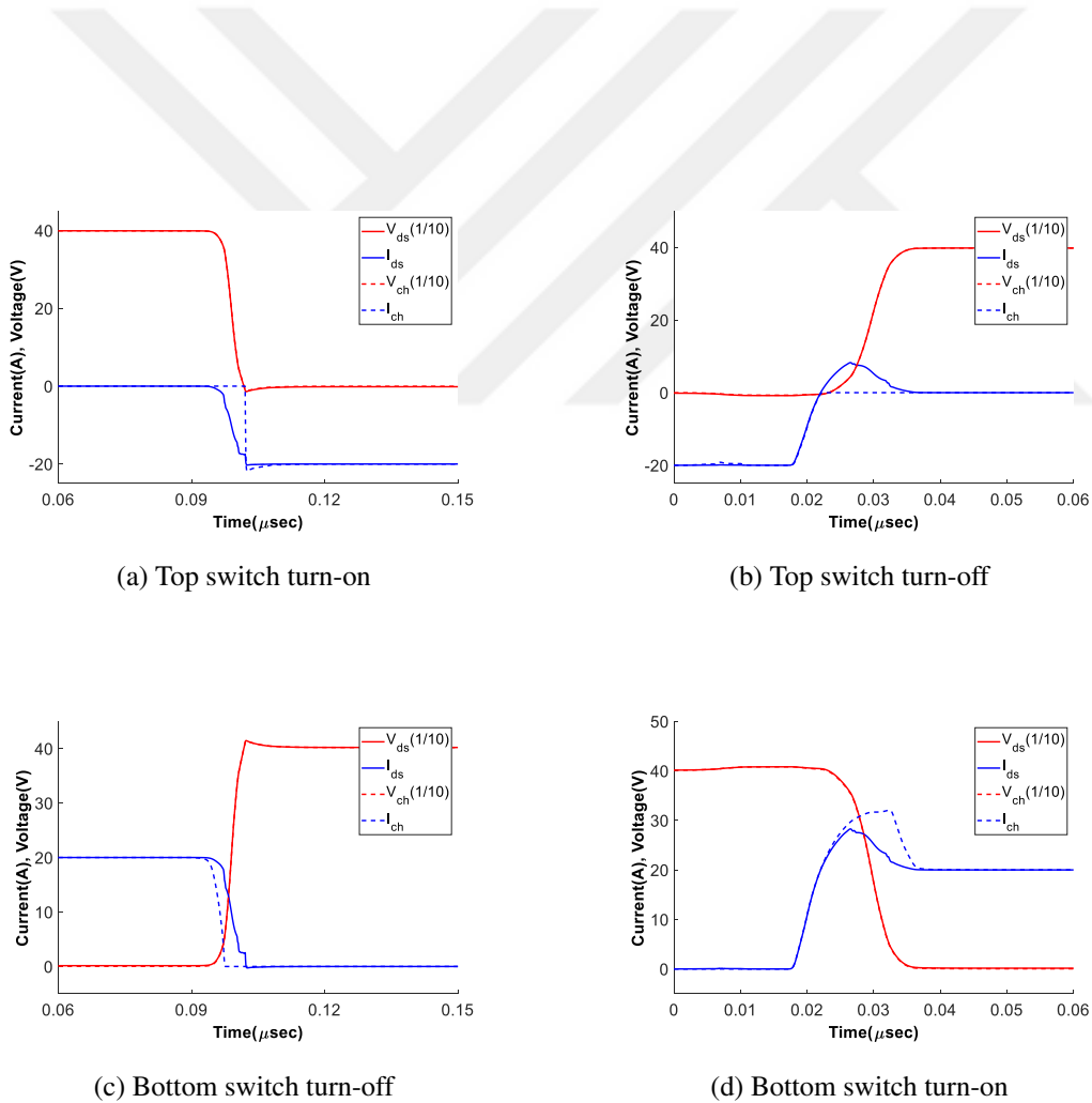
Figure 3.9: Switching transients obtained using Model 2 [8]
