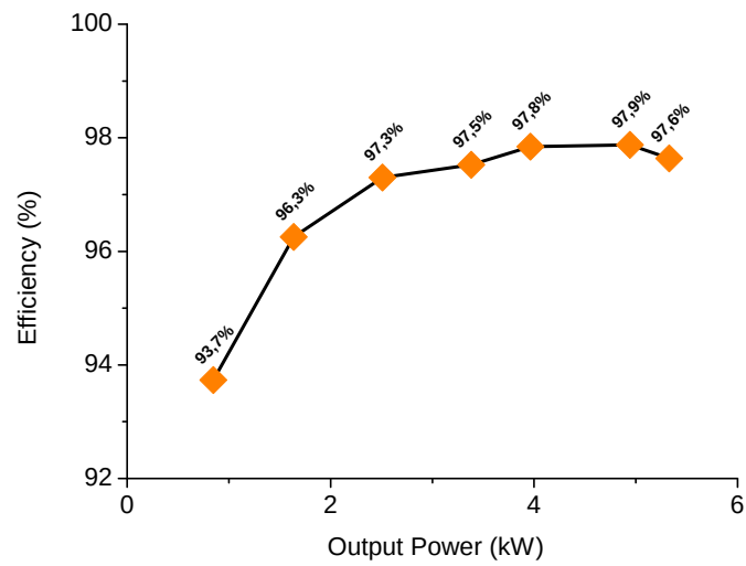
Figure 5.25: Efficiency curve of buck mode operation based on electrical measurements
