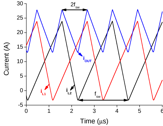
Figure 5.11: Interleaved inductor currents and output current
