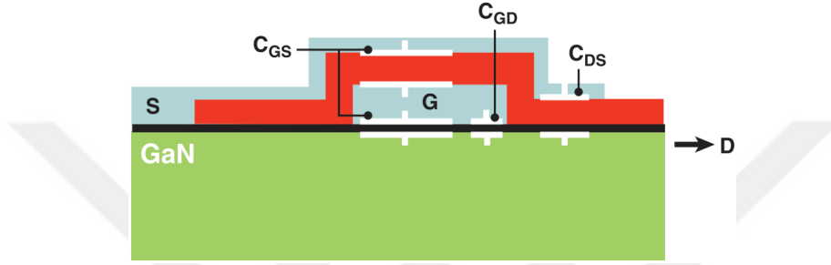
Figure 1.7: Source of the parasitic capacitances [2]
