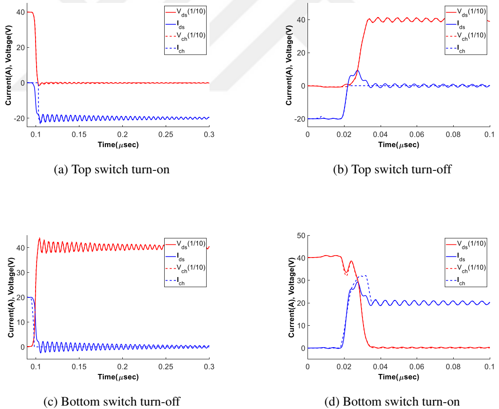
Figure 3.10: Switching transients obtained using Model 3 [8]
