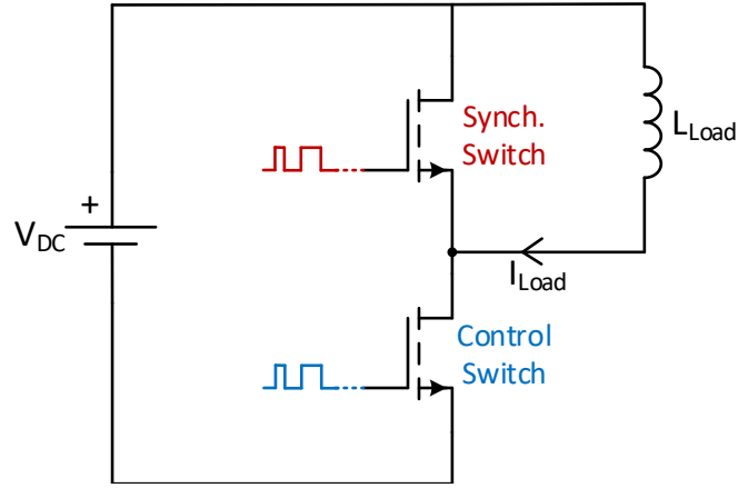
Figure 3.7: Double Pulse Test (DPT) circuit [8]
