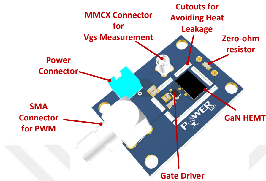
Figure 2.3: Gate loss characterization PCB
