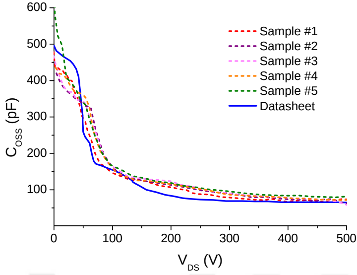
Figure 2.12: Output capacitances
