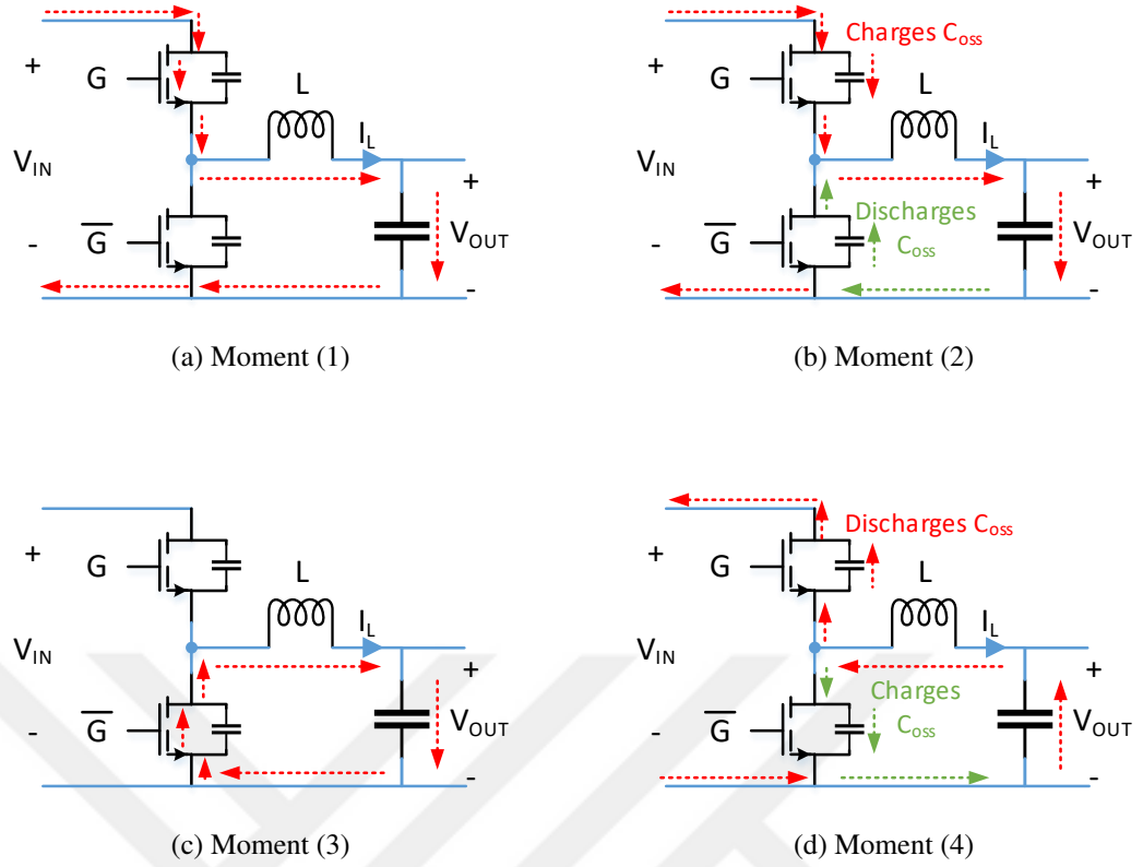
Figure 5.4: Steps of quasi-square wave zero voltage switching defined in Fig. 5.3 for buck mode operation
