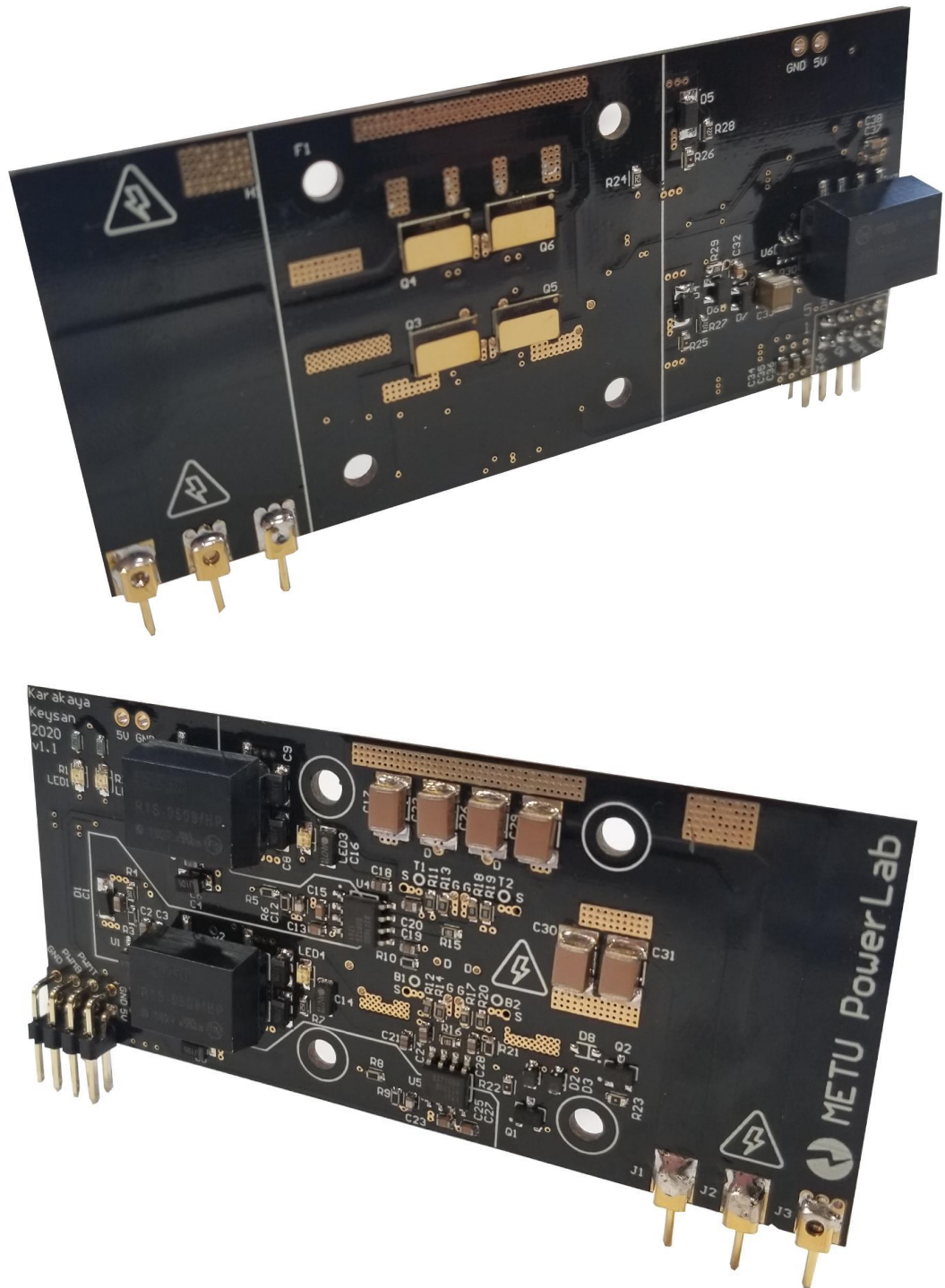
Figure 4.2: Three dimensional view of the half-bridge board
