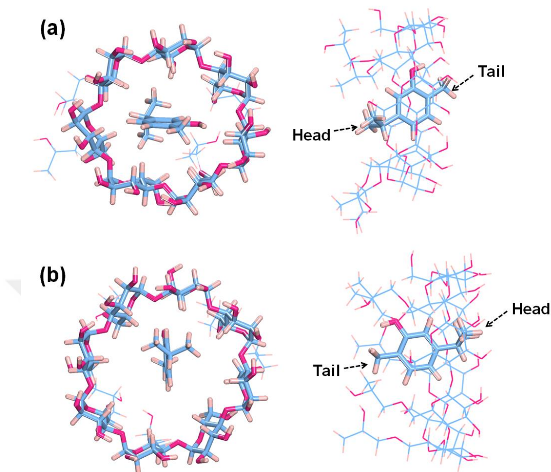
Figure 17. Top and side view of inclusion complexes of (a) HPβCD and (b) HPγCD with carvacrol. The tail and head vertical orientation of carvacrol is shown by arrows. (Blue, pink and light brown balls represent carbon, oxygen, and hydrogen atoms, respectively).
