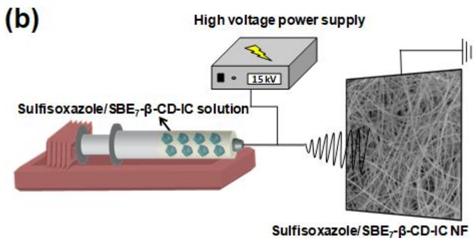
Figure 45. (a) The chemical structure of sulfisoxazole and SBE 7 -β-CD with a schematic representation of sulfisoxazole, SBE 7 -β-CD and their IC, (b) Schematic representation of the electrospinning of sulfisoxazole/SBE 7 -β-CD-IC nanofibers (NF).
