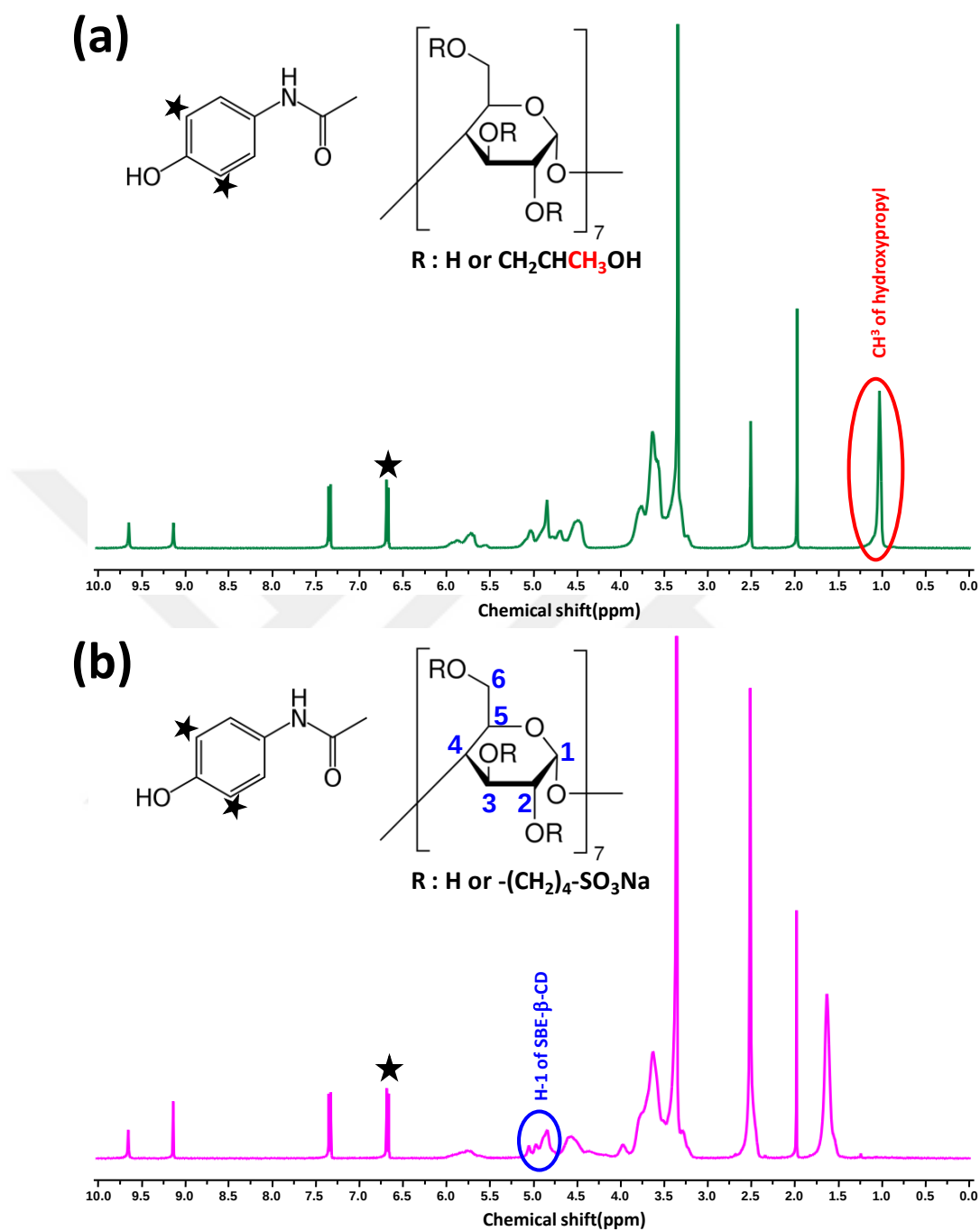
Figure 57. The ^1H -NMR spectra of (a) paracetamol/HPβCD-IC NFs and (b) paracetamol/SBE-β-CD-IC NFs which was dissolved in d_6 -DMSO.
