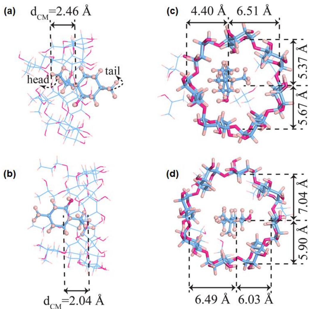
Figure 7. The optimized, lowest energy configurations of side views of ICs of (a) HPβCD and (b) HPγCD; and top view of ICs of (c) HPβCD and (d) HPγCD with menthol. The tail and head vertical orientation of menthol is shown by arrows. (Blue, pink, and light brown balls represent carbon, oxygen, and hydrogen atoms, respectively).
