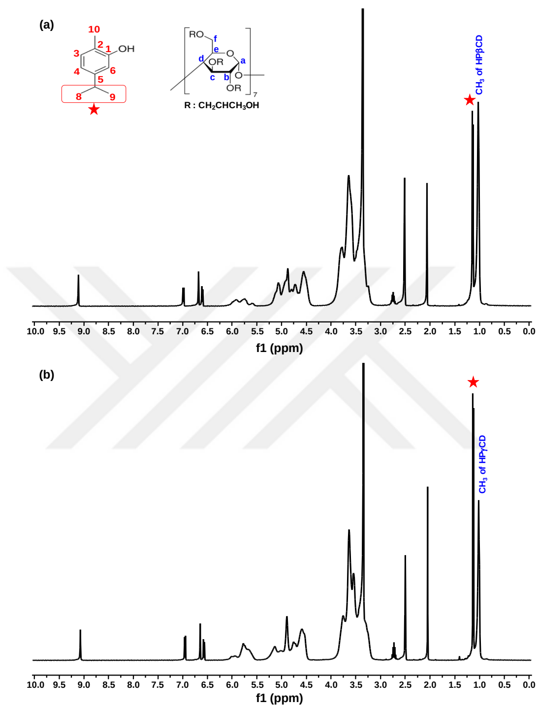
Figure 21. ^1\text{H} -NMR spectra of (a) carvacrol/HP \beta CD-IC and (b) carvacrol/HP \gamma CD-IC fibrous web (dissolved in \text{d}_6 -DMSO) which were produced 3 years ago.
