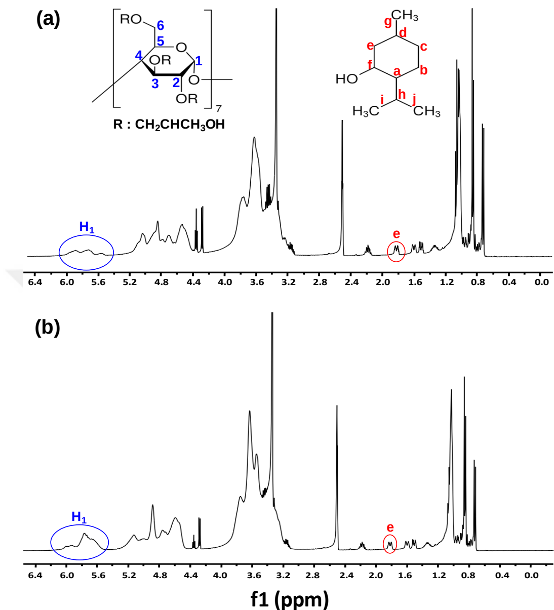
Figure 11. ^1\text{H} NMR spectra of (a) menthol/HP \beta CD-IC NFs and (b) menthol/HP \gamma CD-IC NFs dissolved in d_6 -DMSO.
