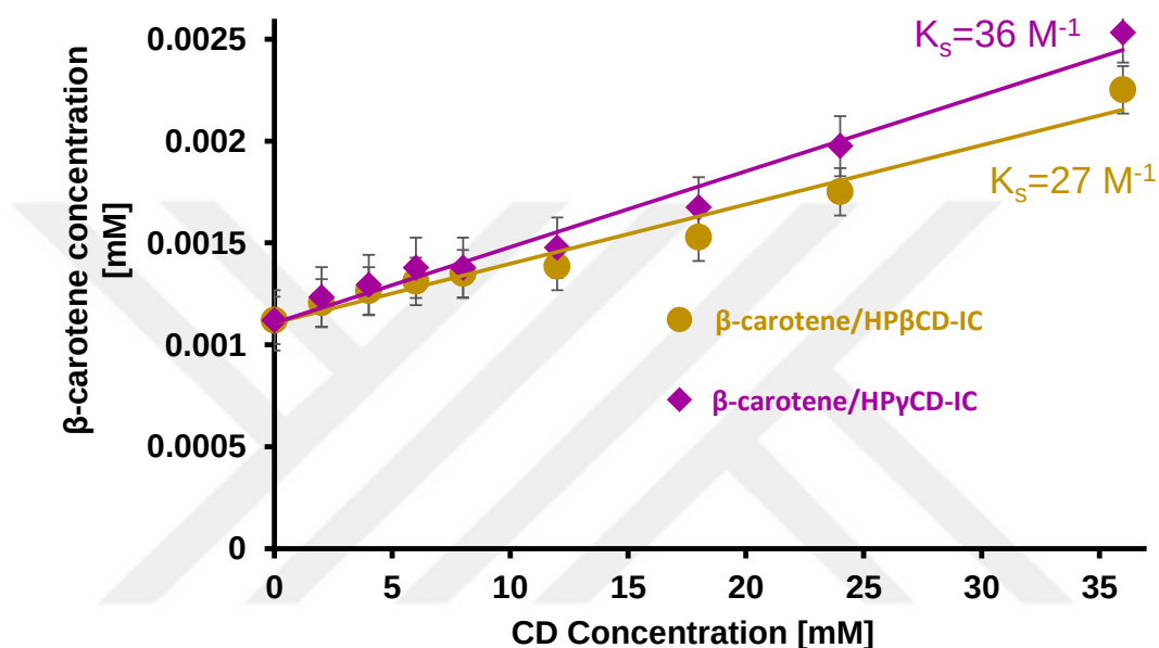
Figure 38. Phase solubility diagrams of \beta -carotene/HP \beta CD-IC and \beta -carotene/HP \gamma CD-IC, ( n = 3 ).
