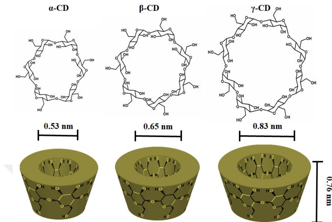
Figure 2. Chemical structure and schematic view of \alpha -CD, \beta -CD and \gamma -CD.
