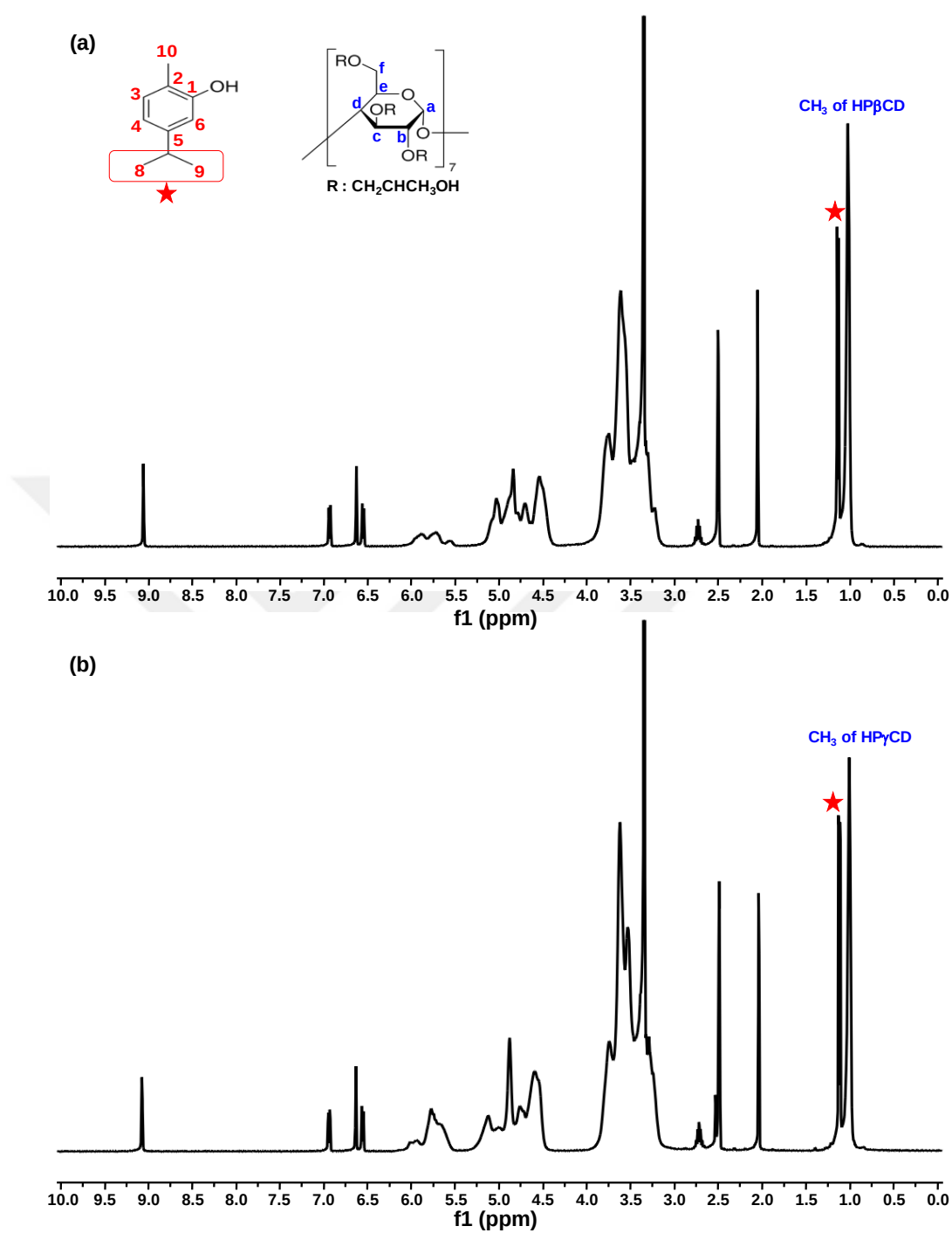
Figure 20. ^1\text{H} -NMR spectra of (a) carvacrol/HP \beta CD-IC and (b) carvacrol/HP \gamma CD-IC fibrous web dissolved in \text{d}_6 -DMSO.
