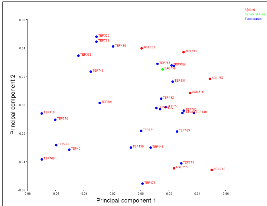
Figure 16: Principal Component Scores plotted for Ovis aries metacarpal from all sites.
