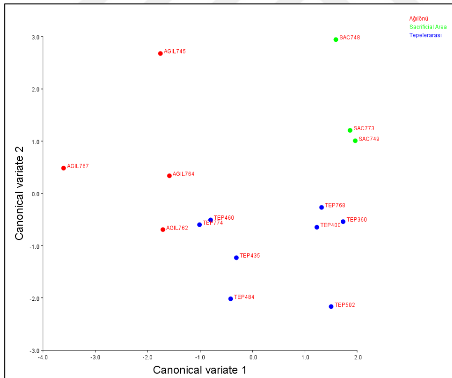
Figure 19: Canonical Variate Scores plotted for Capra hircus metacarpal from all areas.
