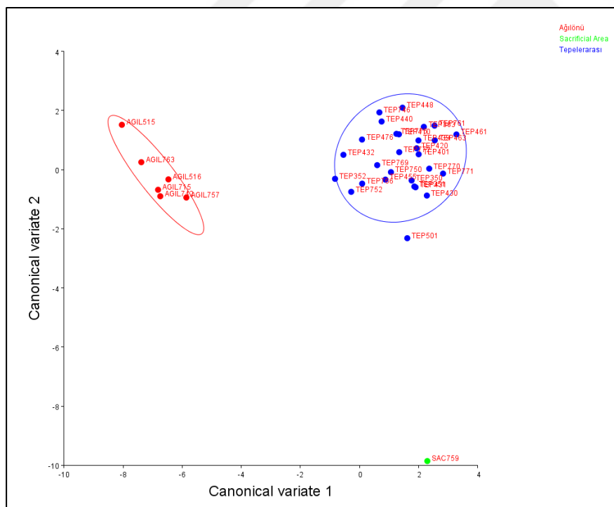
Figure 17: Canonical Variate Scores plotted for Ovis aries metacarpal from all areas.
