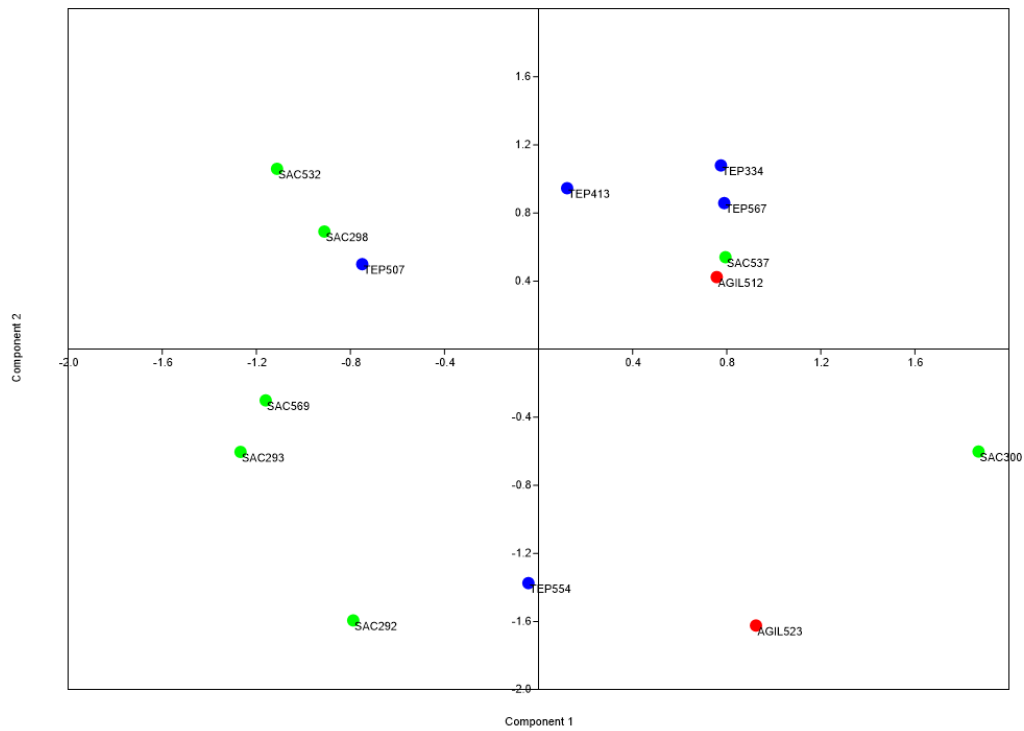
Figure 26: Princpal Component Scores plotted for Capra hircus astragalus from all areas.
