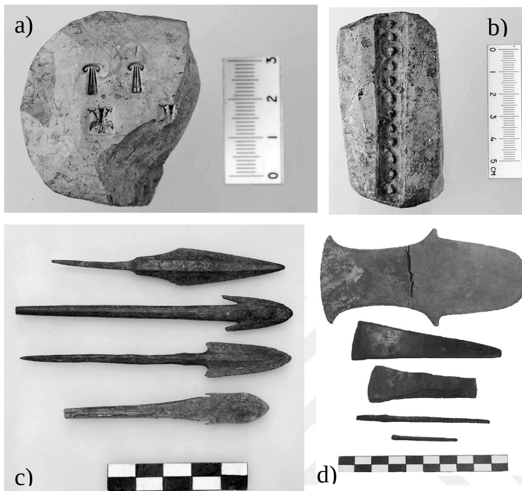
Figure 9: Clay moulds (a and b), bronze arrows (c), and metal materials (d) obtained from Workshops, Tepelerarası (images adapted from Süel 2017,70-73 , Fig. 8, 9, 18, 22.
