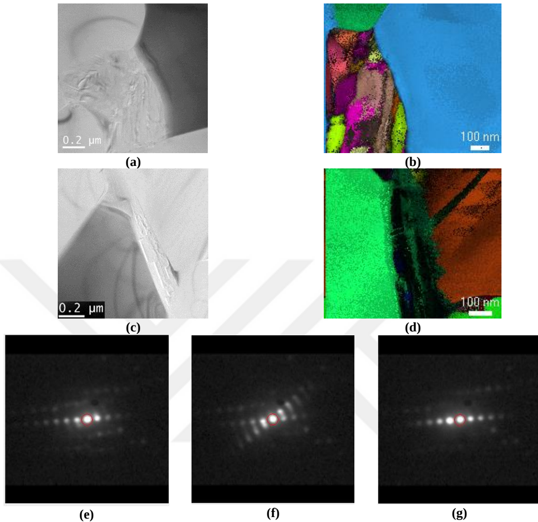
Figure 5.15. (a) TEM-BF image of \text{TiB}_2 and graphite neighbors and (b) respective orientation map showing local orientation change within graphite, (c) TEM-BF image of another neighbors and (d) respective orientation map showing low reliability due to overlapped diffraction patterns from different strands as shown in (e-f)
