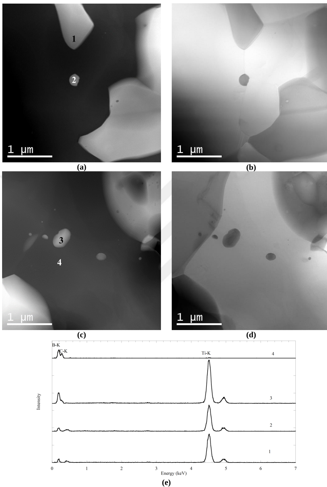
Figure 5.29. (a, c) STEM-HAADF, (b, d) STEM-BF images showing intergranular and intragranular \text{TiB}_2 particles within 50/50-BM sample and (e) STEM-EDX spectra obtained from points labelled in (a) and (c)
