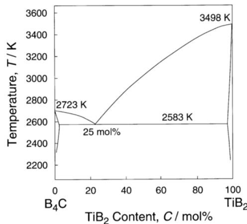
Figure 5.1. Binary phase diagram of TiB 2 -B 4 C [73]
