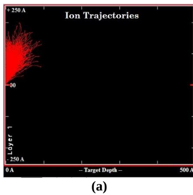
Figure 8.11. Ion implantation simulation results for (a) 6 keV ions at 8°, and 3 keV ions at 4° of incidence angle obtained with SRIM.
