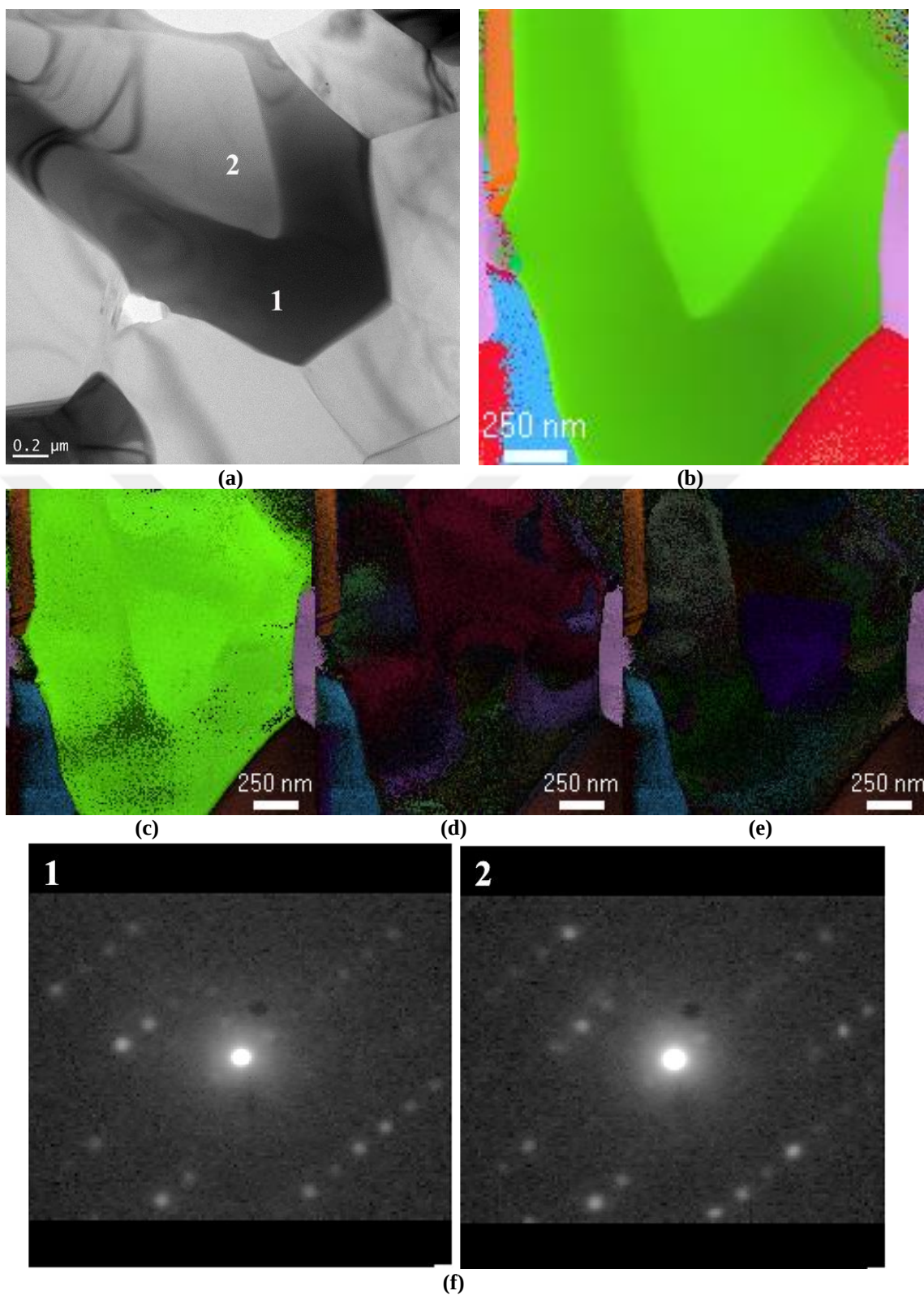
Figure 5.35. (a) TEM-BF image of core/rim structure found in 50/45/5-BM sample, (b) orientation map combined with VBF, orientation maps combined with reliability obtained by using (c) (\text{Ti}_{0.9}\text{W}_{0.1})\text{B}_2 (d) (\text{Ti}_{1.6}\text{W}_{2.4})\text{B}_4 (e) (\text{Ti}_{0.7}\text{W}_{0.3})\text{B}_1 and (f) diffraction spots obtained from points labelled in (a)
