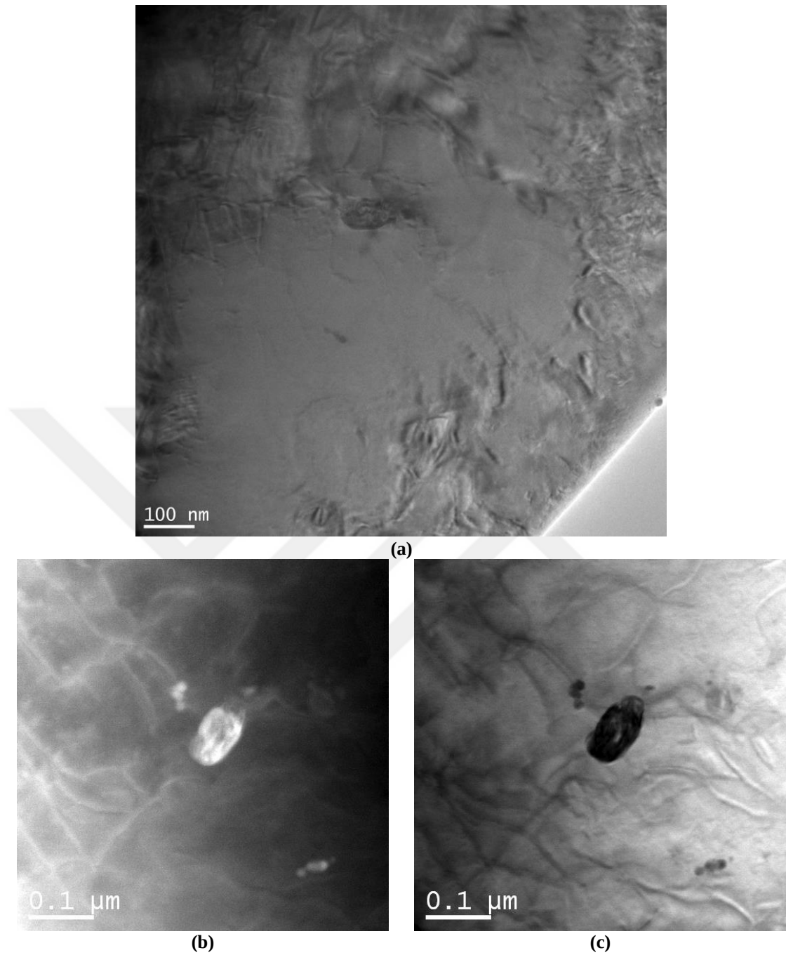
Figure 7.1. (a) TEM-BF image of a region with a precipitate, (b) STEM-HAADF and (c) STEM-BF image of the same region
