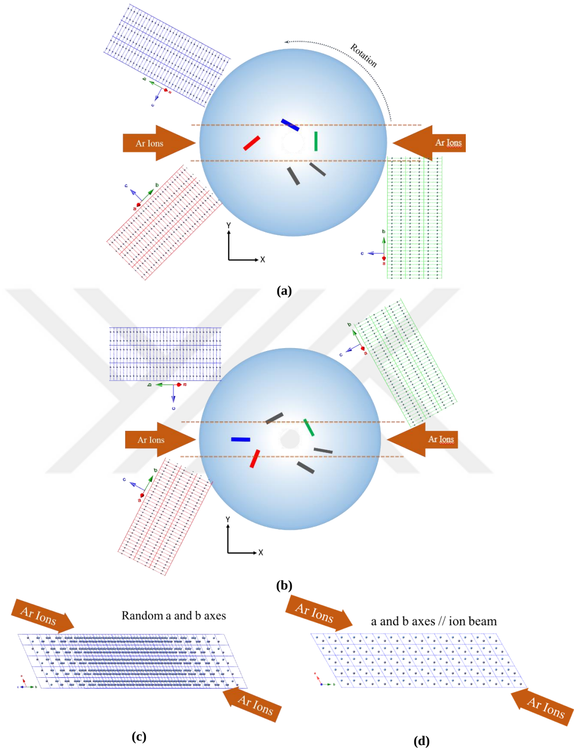
Figure 8.12. Proposed ion implantation scheme for hBN particles that do not fulfill channeling conditions during ion beam milling (a) before rotation of the sample, none of the particles fulfill the requirements, (b) sample rotated and blue particle come into position that fulfill the requirements but others not. (c) ion beam position for blue particle in (a) condition (random a and b axes) and (d) ion beam position for blue particle in (b) condition (a and b axes are parallel to ion beam)
