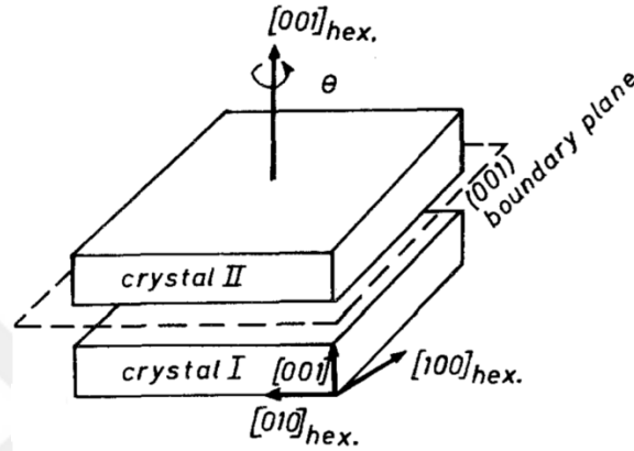
Figure 4.11. Schematic explanation of [0001] twist boundary in hexagonal bicrystal [63]
