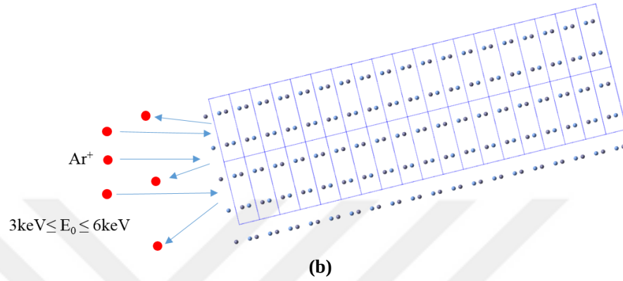
Figure 8.10. Proposed ion channeling mechanism when c -axis perpendicular to the ion source and (b) backscattering of ions when crystal orientation is changed and c -axis is no more perpendicular to the Ar source
