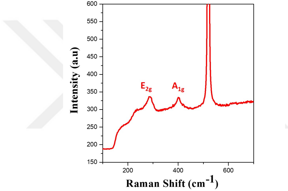
Figure 5.18: Raman spectrum of 2H-TaS 2 mechanical exfoliated crystal. Two characteristic peak a labeled E_{2g} and A_{1g} which correspond to inplane and out of plane vibration modes of phonons respectively.
