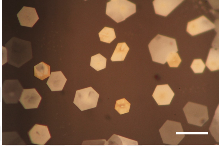
Figure 5.13: Optical microscope images of \text{V}_2\text{O}_3 crystals with different morphologies, shapes and thickness grown by salt-assisted chemical vapor deposition. Scale bar is 20\mu\text{m} . Reproduced from ref. [119]. Copyright American Physical Society 2019.
