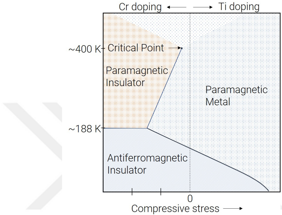
Figure 5.11: The phase diagram of V_2O_3 based on reference. The paramagnetic metal (PM) and insulator (PI) phases have corundum structure, while the antiferromagnetic insulator phase (AFI) has a monoclinic structure. Reproduced from ref. [119]. Copyright American Physical Society 2019.
