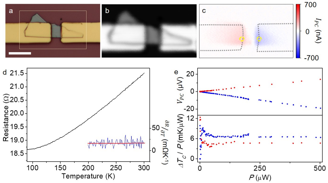
Figure 3.12: (a) Optical micrograph of the TC1 is shown with marked square region in which SPCM is performed. Scale bar is 10μm (b) Reflection map obtained by scanning the laser on top of the device and (c) corresponding photocurrent map under zero applied bias. The photocurrent is confined around the edges which are marked by the dashed black lines. (d) Resistance vs temperature plot of the same device showing characteristic metallic behavior. The inset shows \partial R / \partial T as a reference. (e) Upper panel shows V_{PC} plotted as a function of laser power. The measurement is taken from NbS 2 metal junction marked by yellow dashed circle on the photocurrent map. Red and blue points from left and right electrodes respectively. By using V_T vs P data, calculated \Delta T_C / P is plotted in the lower panel. Reproduced from ref. [91]. Copyright American Physical Society 2018
