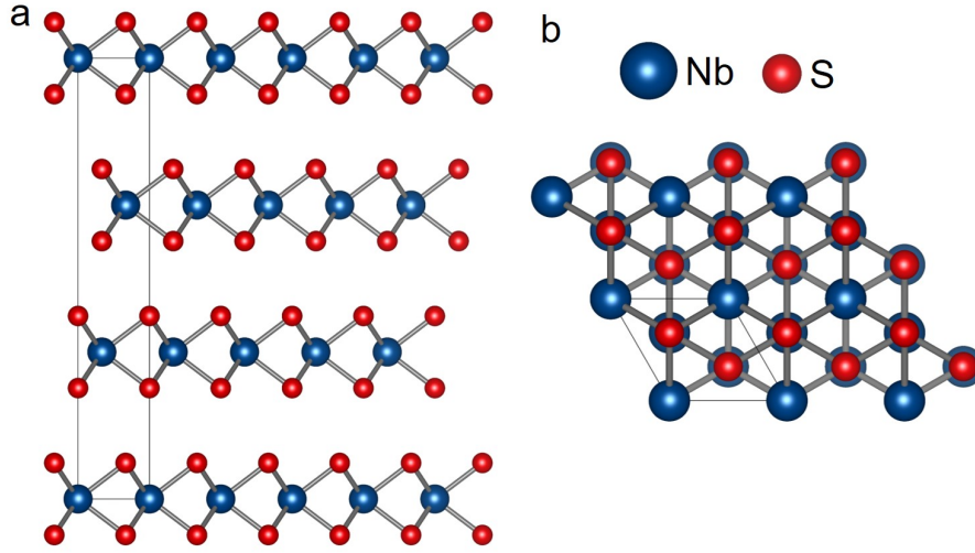
Figure 3.7: Schematic of the side view (a) and top view (b) of the crystal structure of 3R-NbS 2 . Reproduced from ref. [91]. Copyright American Physical Society 2018
