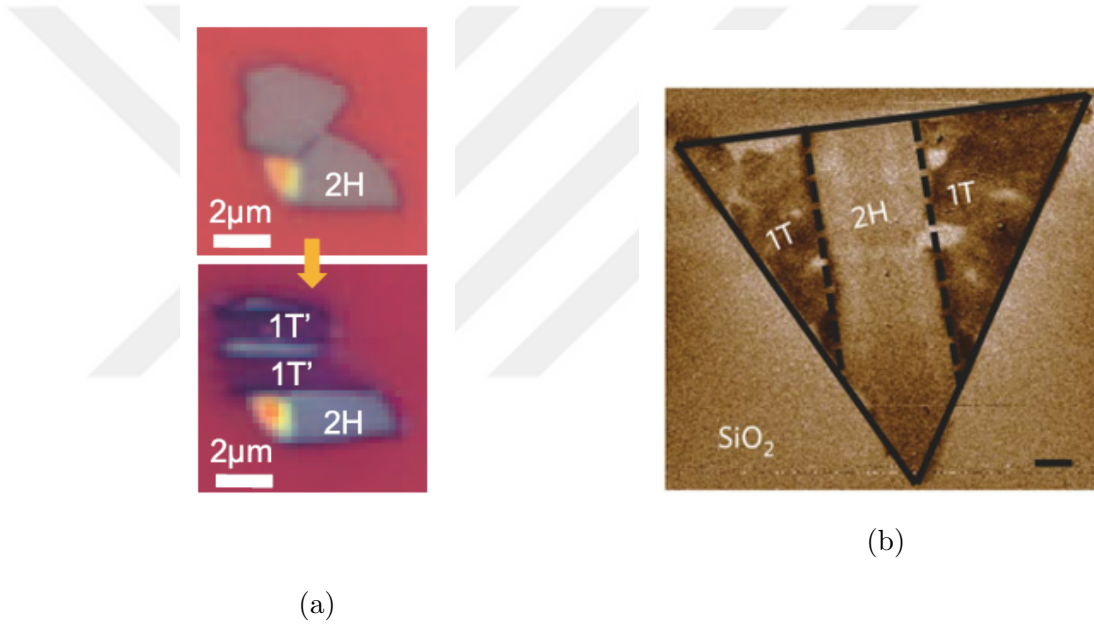
Figure 1.4: (a) Laser induced phase transformation of \text{MoTe}_2 from 2H phase to 1T'. Copyright American Association for the Advancement of Science 2015(b) CVD grown 2H- \text{MoS}_2 crystal selectively converted to 1T phase upon treatment with n-butyl lithium. Copyright Springer Nature 2014
