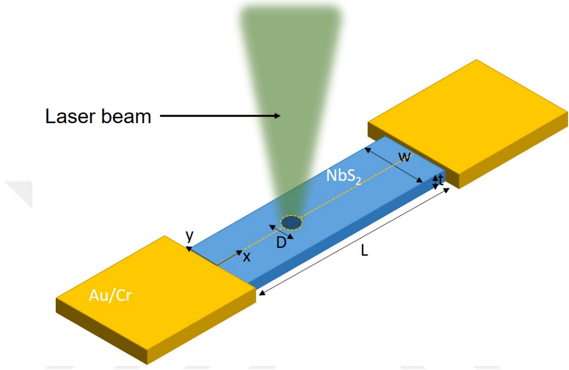
Figure 3.15: Schematic model showing different parameters used to calculate \partial T_l using a python code. Reproduced from ref. [91]. Copyright American Physical Society 2018
