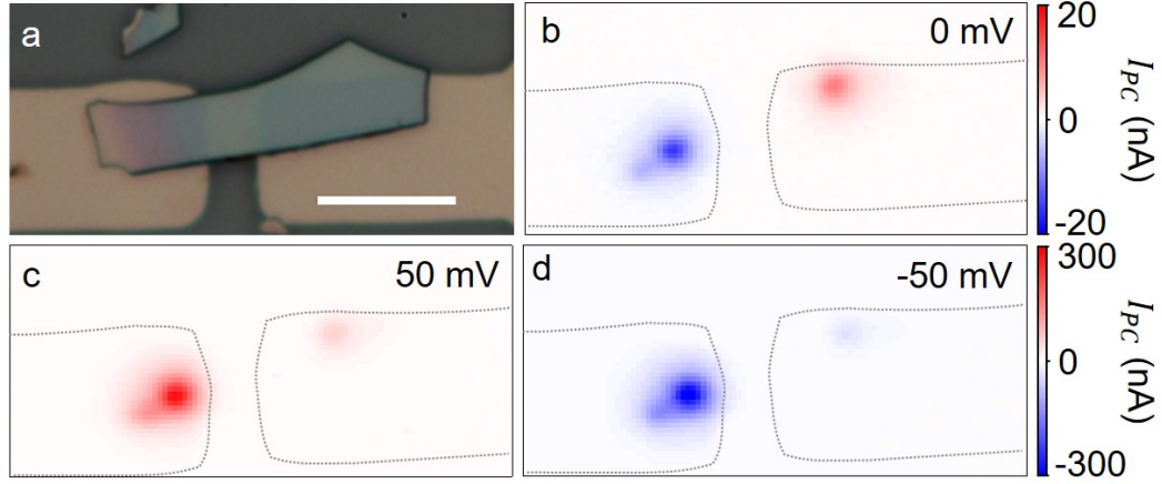
Figure 3.17: (a) Optical micrograph of a bottom contact device. scale bar is 10\mu\text{m} . (b) Photocurrent map under zero applied bias. The photoresponse is localized to a small region and is a magnitude smaller than TC device. (c) and (d) photocurrent maps at 50mV and -50mV applied biases respectively. Photoresponse changed only at the \text{NbS}_2 /metal junction and no response is observed through middle of the crystal. Reproduced from ref. [91]. Copyright American Physical Society 2018
