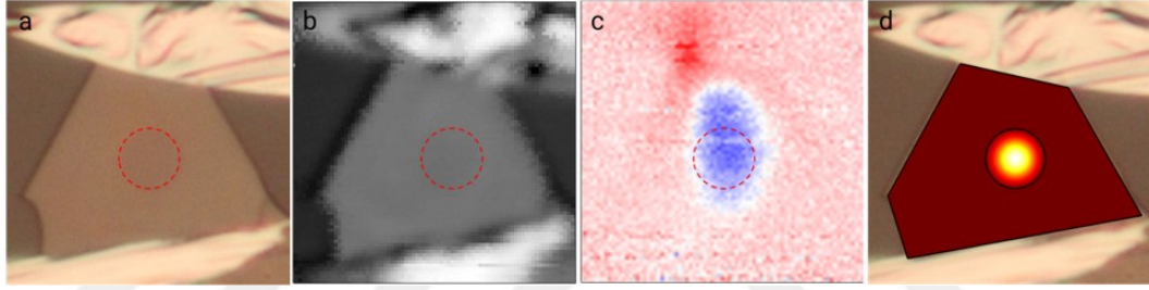
Figure 5.16: (a) Optical microscope image of \text{V}_2\text{O}_3 device prepared for thermal conductivity measurements. The red dashed line represents the location of hole under the crystal. (b) Reflection map collected during SPCM of the same device. (c) Photocurrent map of the device under applied bias. (d) FEM simulation of thermal profile of the devices mapped onto optical microscope image. Under 9.5 \mu\text{W} laser power, the maximum temperature rise at the center of the hole is 2.5K above room temperature. Reproduced from ref. [115]. Copyright IOP Publishing Ltd. 2020.
