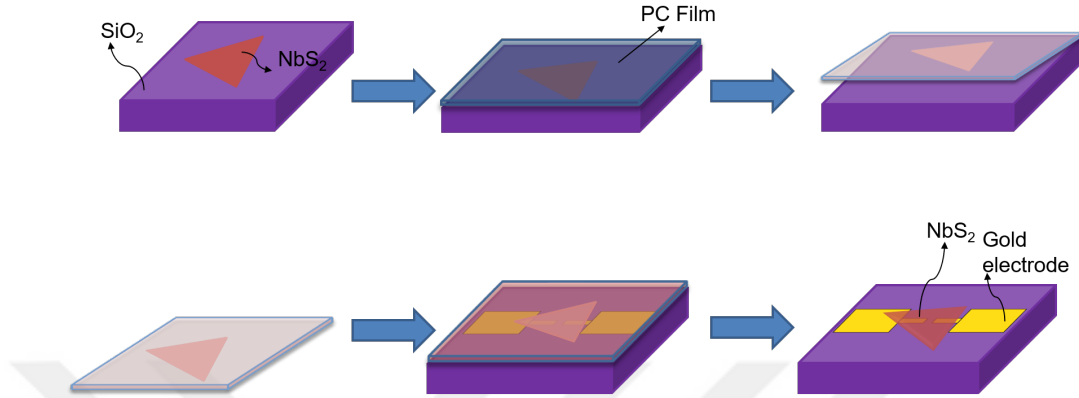
Figure 3.2: Schematic of the deterministic crystal transfer starting from mechanical exfoliation of the NbS 2 till the selected flake aligned and transferred on top of metal electrode.
