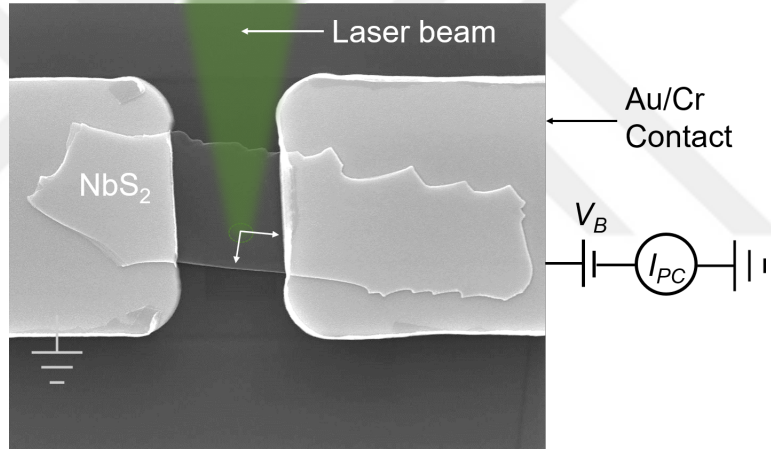
Figure 3.11: SEM micrograph of two terminal device with measurement configuration depicted on it. A diffraction limited laser spot raster scans the samples in x-y direction. In all our experiments, left electrode is grounded and the bias is applied from the right electrode. Reproduced from ref. [91]. Copyright American Physical Society 2018
