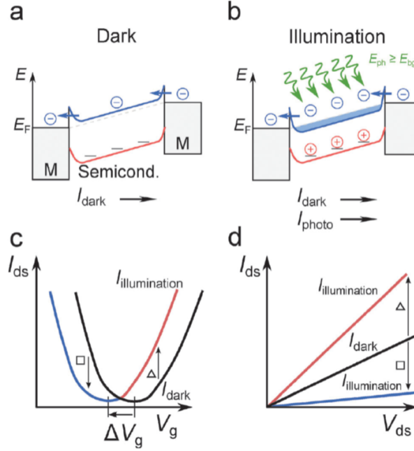
Figure 2.2: (a) Schematic of band alignment when two metal contacts are made to semiconducting material under some applied bias without illumination. (b) Band alignment under applied bias when a device is illuminated with photons of energy E_{ph} greater than band gap E_{bg} . Holes are shown to be trapped at the band edge. Upon illumination and under applied bias, field effect produces electrons in the channel which contribute towards photocurrent generation. (c) Current plotted against applied gate voltage with and without illumination. (d) IV plots in dark (black line) and under illumination (red and blue solid lines). Reproduced from Ref. [62] with permission from The Royal Society of Chemistry.
