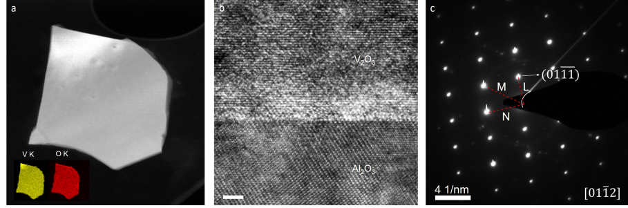
Figure 5.14: (a) Low resolution TEM image of V_2O_3 crystal transferred over holey carbon TEM grid. The inset shows EDS maps of vanadium (yellow) and oxygen (red) elements. (b) High resolution Cross-sectional TEM image of V_2O_3 crystal stacked on top of sapphire substrate. Scale bar is 2nm. (c) Selected area diffraction pattern obtained from cross-sectional TEM sample. This pattern matched uniquely with HCP [01\bar{1}2] diffraction pattern. Reproduced from ref. [119]. Copyright American Physical Society 2019.
