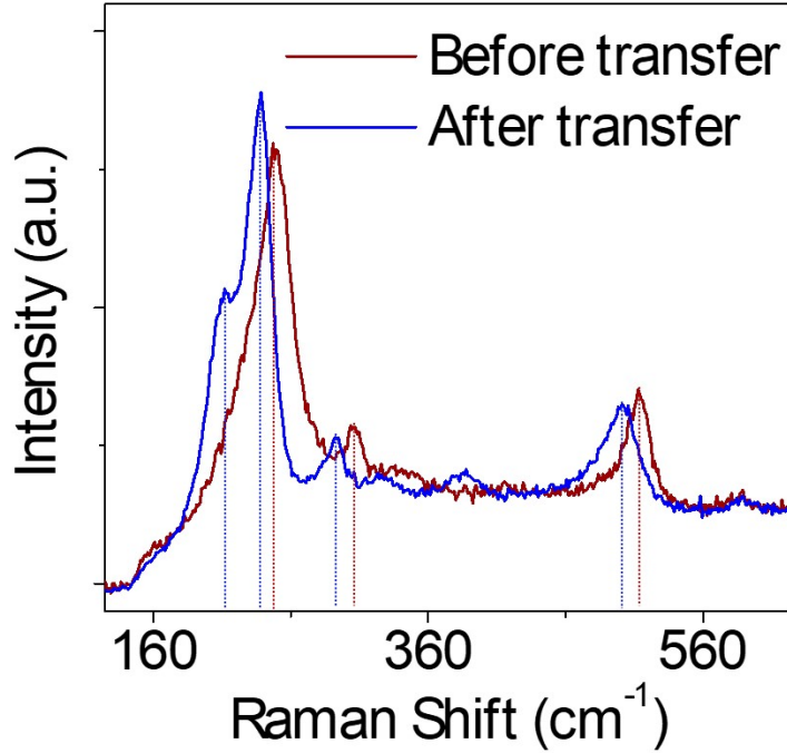
Figure 5.15: Raman spectrum of as-grown (red) and transferred \text{V}_2\text{O}_3 crystals from sapphire substrate. The shift in the peak positions can be seen along with appearance of a shoulder to the 248\text{cm}^{-1} peak. Reproduced from ref. [119]. Copyright American Physical Society 2019.
