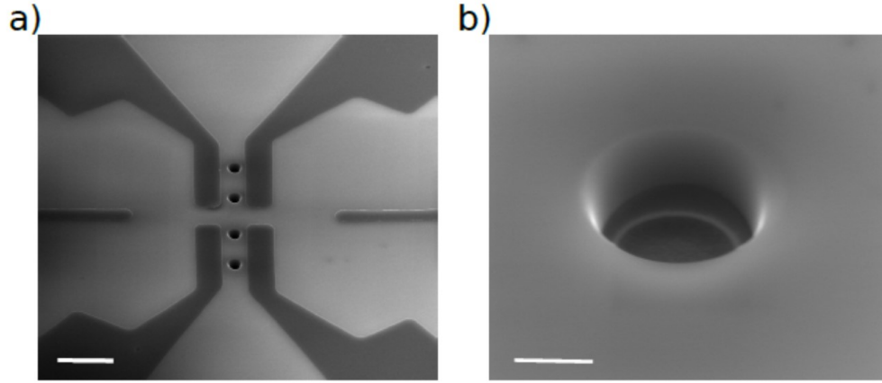
Figure 5.5: (a) SEM image of the drilled hole between the electrodes. Scale bar 10 \mu\text{m} (b) Tilted angle close up of the drilled hole with high aspect ratio and desired shape and size. Scale bar 1 \mu\text{m} . Reproduced from ref. [117]. Copyright Springer Nature 2020.
