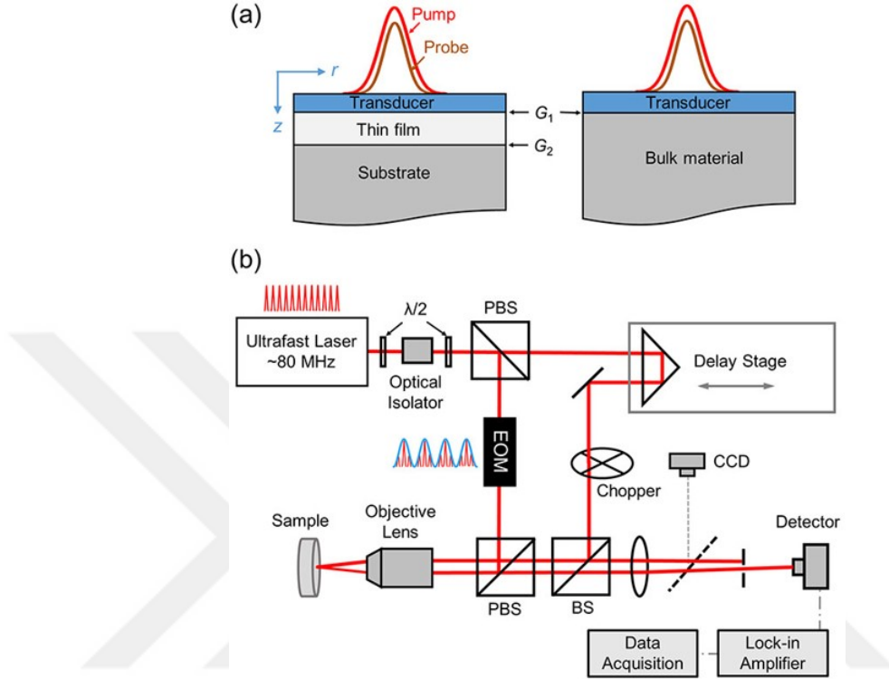
Figure 4.2: (a) Schematic of typical samples used for TDTR technique. Both thin film and bulk sample configuration is shown. (b) Drawing of typical setup used for TDTR setup. Used abbreviation are PBS(Polarizing beam splitter), BS(Beam splitter), EOM(Electro-optic modulator), \lambda/2 (Half wave plate). Reproduced from ref. [110]. Copyright AIP Publishing 2018.
