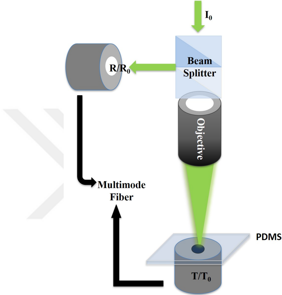
Figure 5.9: Absorbance measurement schematic is shown in the figure. Spectrometer is used to measure the intensities of both reflected and transmitted light.
