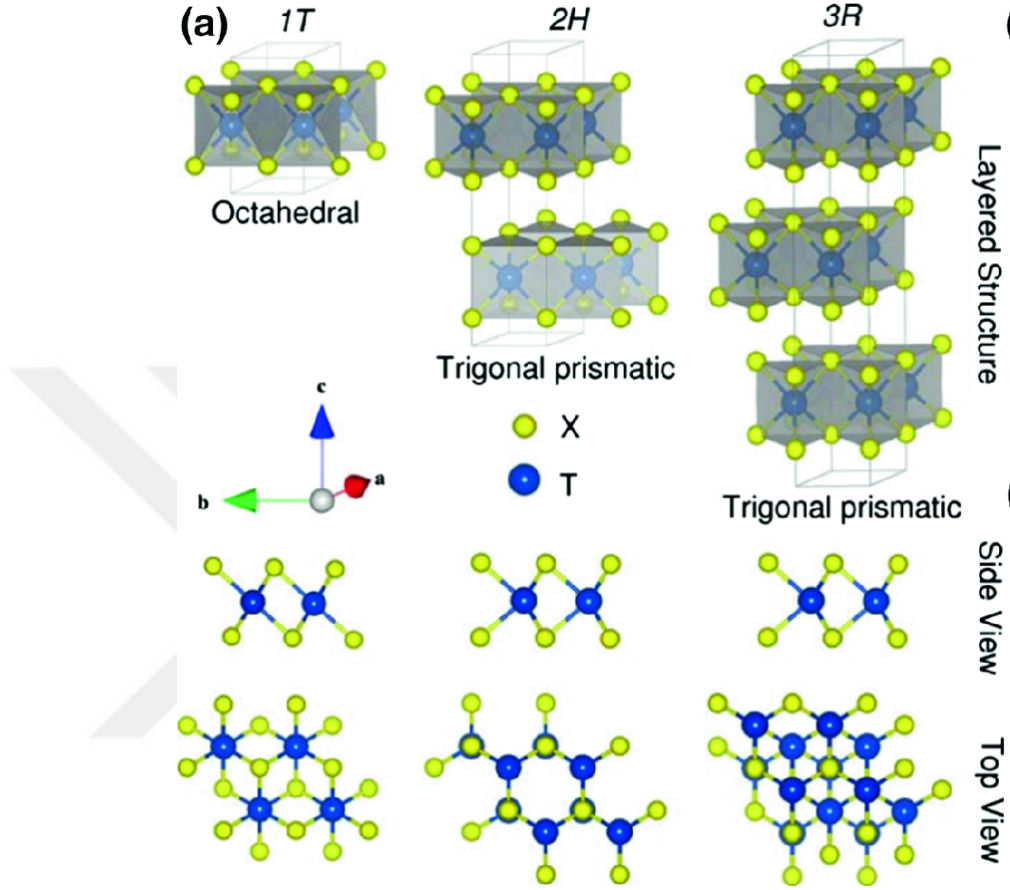
Figure 1.2: Atomic structure schematics of TMDCs showing tetragonal octahedral(1T), hexagonal trigonalprismatic(2H), and rhombohedral trigonal prismatic(3R) crystal phases in monolayer form[25]. Copyright Springer Nature 2019.
