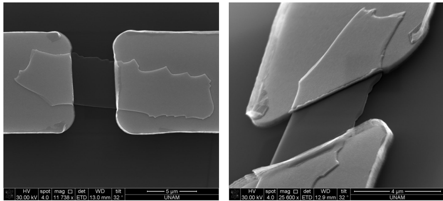
Figure 3.6: Electron microscope images of top contact devices showing top view and side view of the selected device.
