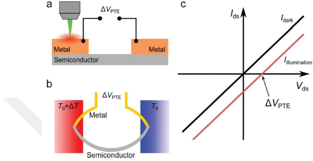
Figure 2.4: (a) Schematic of a FET which is being illuminated locally using a focused laser spot at one of the metal-semiconducting junction. The configuration represent the open circuit case where the thermoelectric potential is generated between the two junctions. (b) represents the circuit diagram of the same device depicted in (a). (c) IV characteristic curve in both dark (black) and under illumination (red) are plotted. Under zero bias, a current is generated in the system driven by the thermoelectric potential difference ( V_{PTE} ). Reproduced from Ref. [62] with permission from The Royal Society of Chemistry.
