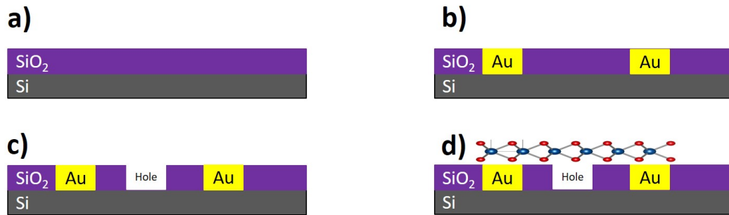
Figure 5.6: (a) 280nm thick SiO 2 wafer is chosen for fabrication (b) Gold metal evaporated into pits prepared after optical lithography and ICP etching. (c) Hole drilled using focused ion beam milling between electrodes. (d) 2D material transferred using all dry visco-elastic stamping method.
