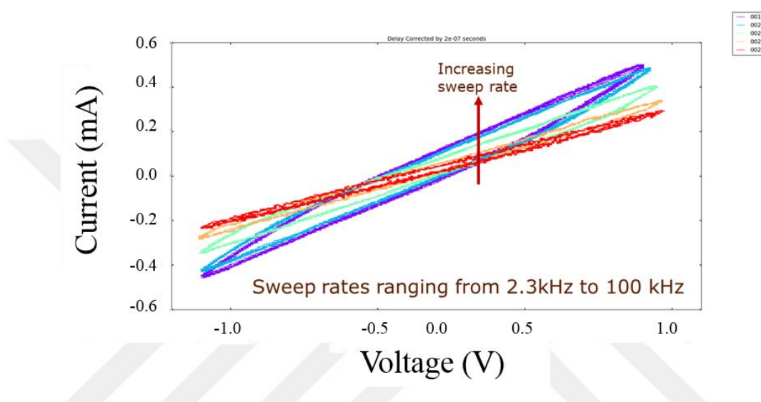
Figure 5. 15 Cyclic voltammograms of a drop cast PEDOT: PSS film onto Pt mesh electrode.
