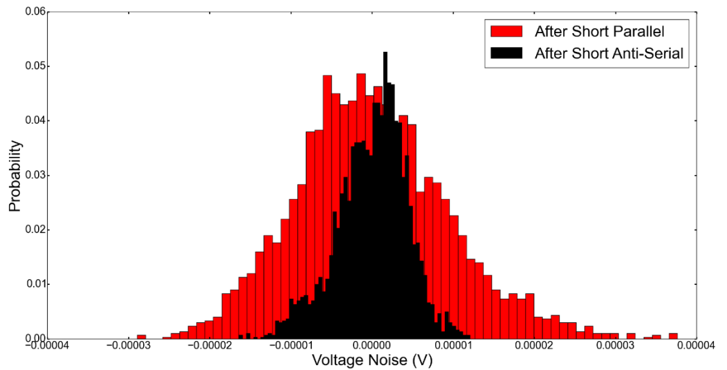
Figure 2. 9 Noise of the same two CR2032 batteries compared in anti-serial and parallel connections after short circuiting the batteries.
