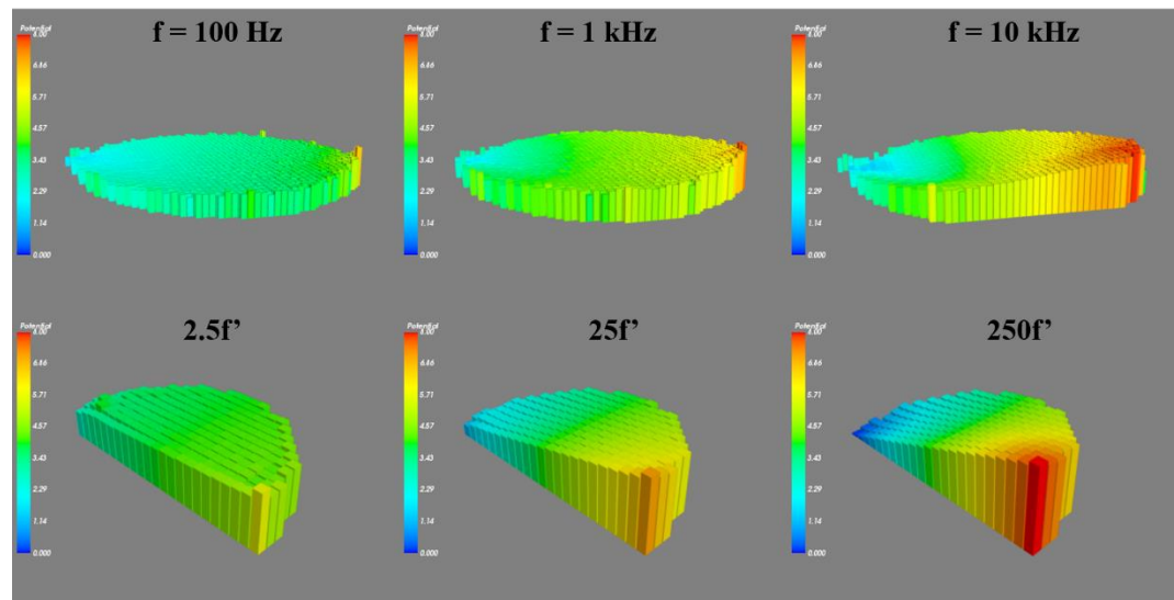
Figure 6. 7 The response of the ionic liquid to an 8 V p-p square wave at varying frequencies a) measured by XPS for a device with two Pt point contacts, b) simulated by the coarse grained electrostatic model
