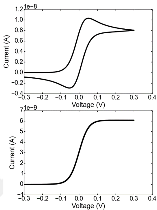
Figure 1. 8 Transient(top) and steady state voltammograms(bottom) of a fast redox couple simulated assuming equal diffusion coefficients of the oxidized and the reduced species ( 10^{-5} ) at a hemispherical UME of radius 10 \mu\text{m} at 1 \text{ V/s} and 0.001 \text{ V/s} sweep rates.
