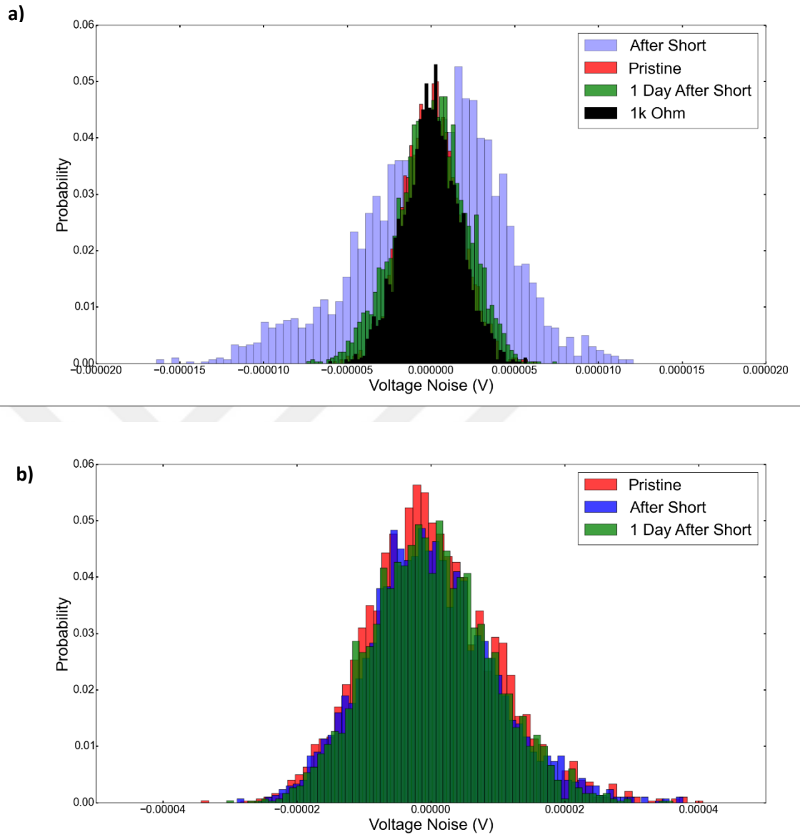
Figure 2.10 a) Noise of two CR2032 coin-cells attached in anti-serial connection. b) Noise of the same two CR2032 coin-cells attached in parallel connection. (Figure 2.5 serves as a scale for these two graphs for ease of view.)
