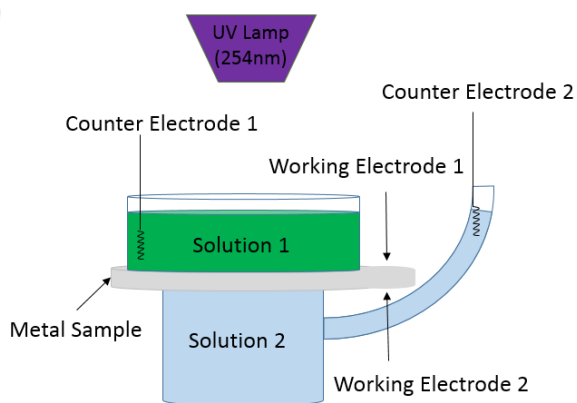
Figure 3. 1 Schematic representation of the setup (left). The actual setup (right).
