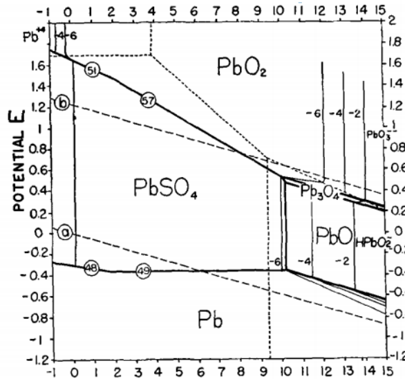
Figure 4. 1. The well-known Pourbaix Diagram for Pb species in sulfuric acid solution. Reprinted by permission from[90].
