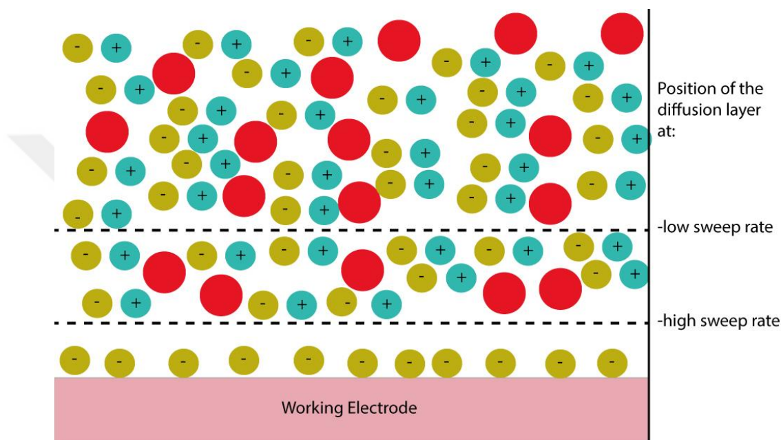
Figure 5. 1 The depiction of the position of diffusion layer with respect to sweep rate. Red circles denote electroactive species while the rest are electrolyte ions
