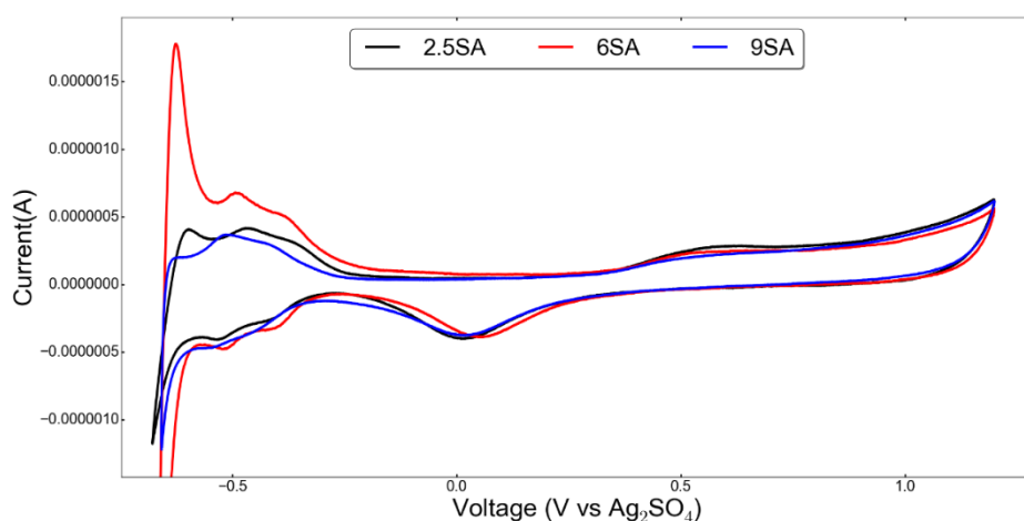
Figure 4. 10 Pt in acid cyclic voltammograms of Liquid crystals containing different sulfuric acid ratios (9,6 and 2.5). CV was taken at 10 V/s, with Pt working electrode.
