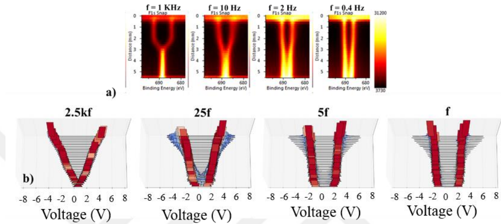
Figure 6. 6 The response of the ionic liquid to an 8 V p-p square wave at varying frequencies a) measured by XPS for a device with two planar Au contacts, b) simulated by the coarse grained electrostatic model.
