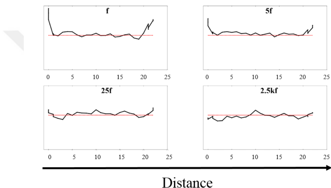
Figure 6. 8 Number of particles at various positions at the ionic liquid surface across different timescales (red line is the initial number of particles).
