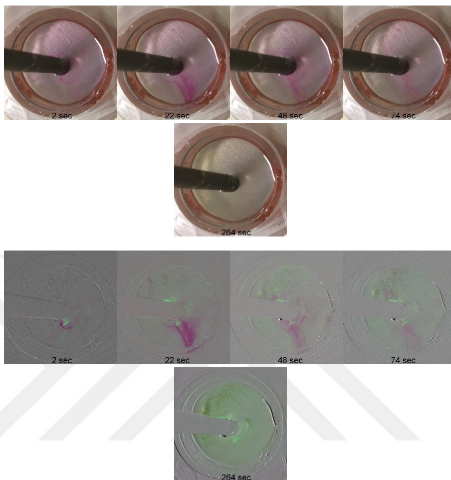
Figure 3. 4 Background subtracted images (bottom), unsubtracted images (top). Green color indicates regions of low pH while red indicates an increase in pH.
