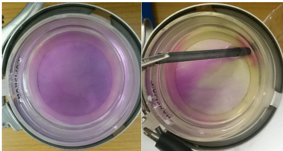
Figure 3. 2 The initial experiments with phenolphthalein indicator. Loss of bulk color can be seen on the right.
