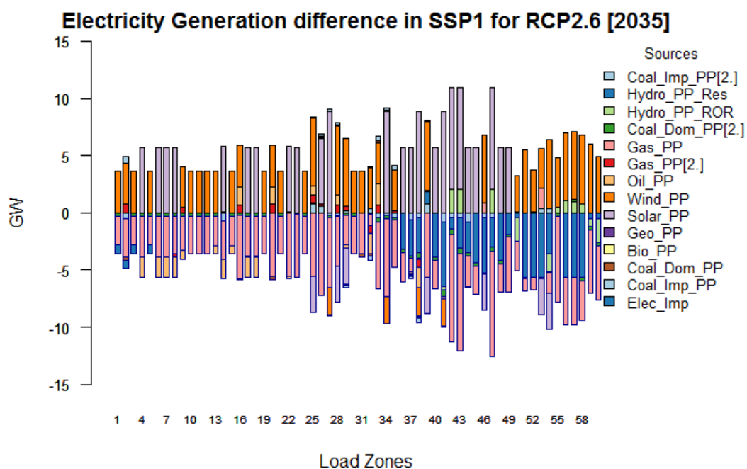
Figure 3.23: Electricity supply difference in SSP1 for RCP3.4 [2035]
