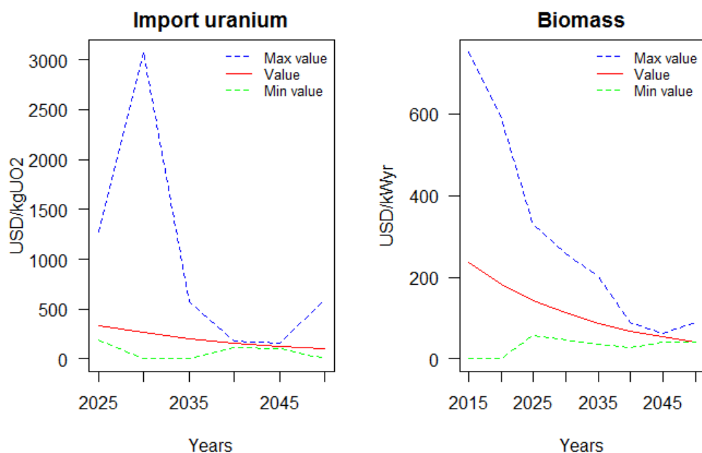
Figure 3.114: Primary fossil fuel costs for Baseline in SSP2
