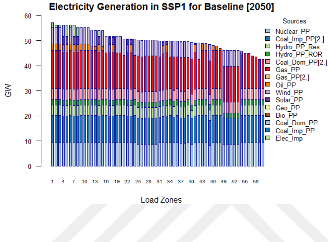
Figure 3.25: Electricity supply in SSP1 for Baseline [2050]
