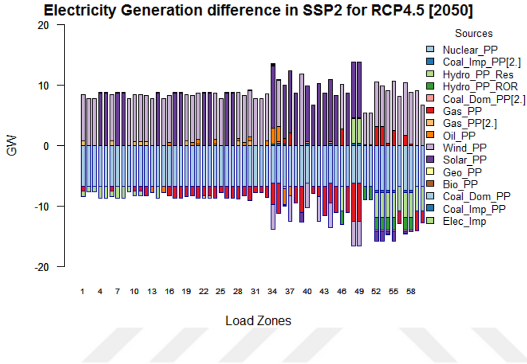
Figure 3.37: Electricity supply difference in SSP2 for RCP4.5 [2050]
