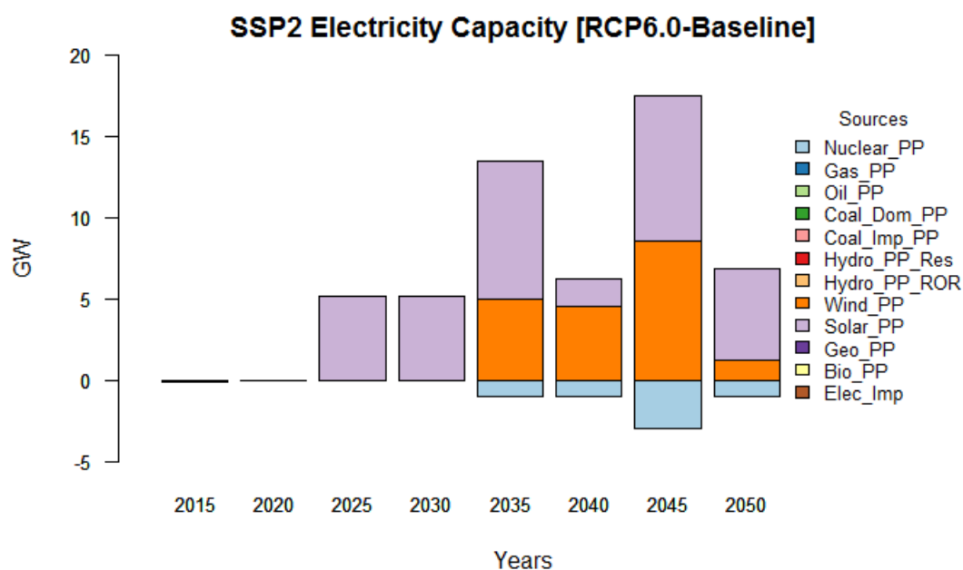
Figure 3.11: Electricity capacity expansion in SSP2 for Baseline
