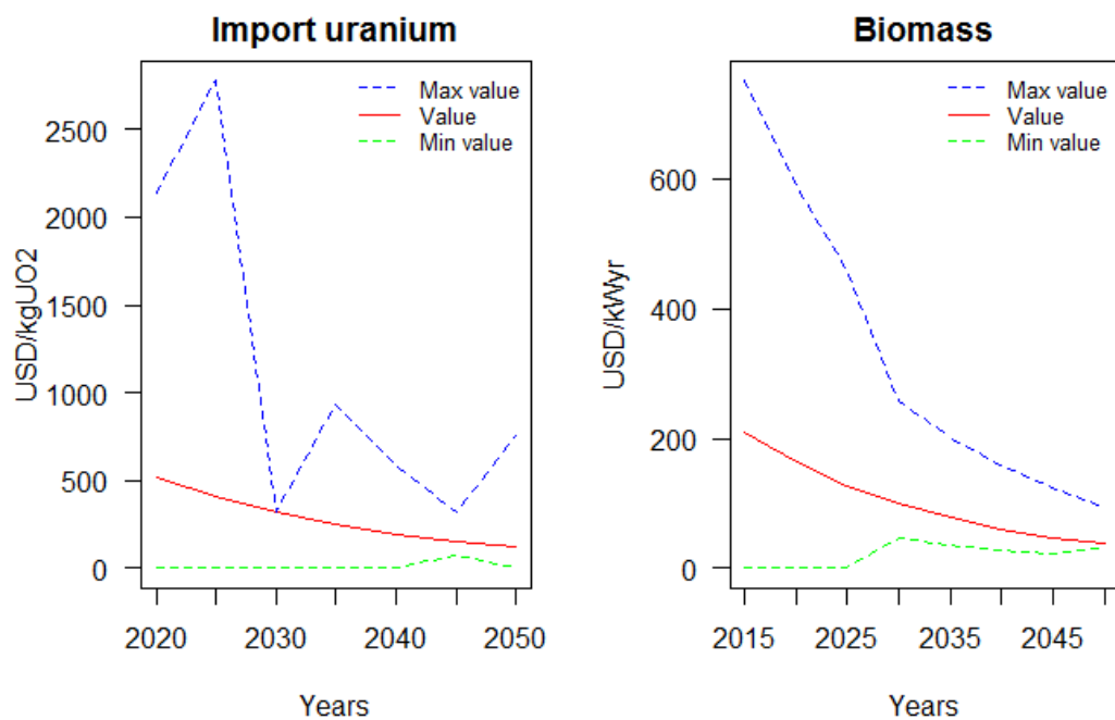
Figure 3.118: Primary fossil fuel costs for Baseline in SSP3
