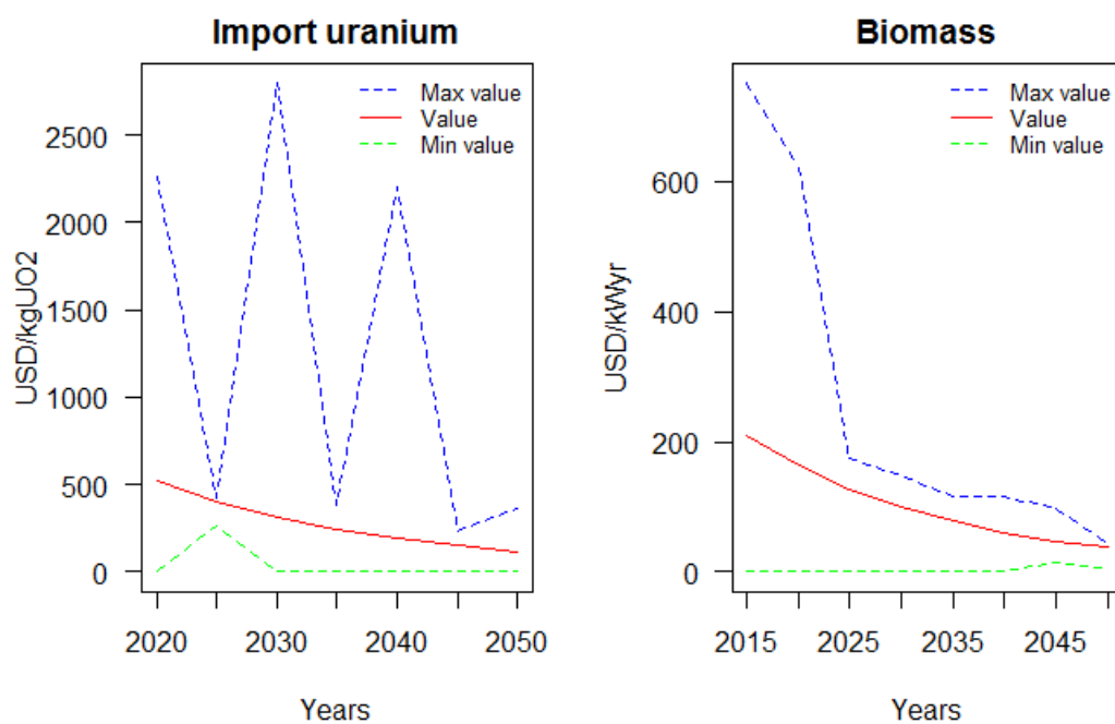
Figure 3.120: Primary fossil fuel costs for RCP3.4 in SSP3
