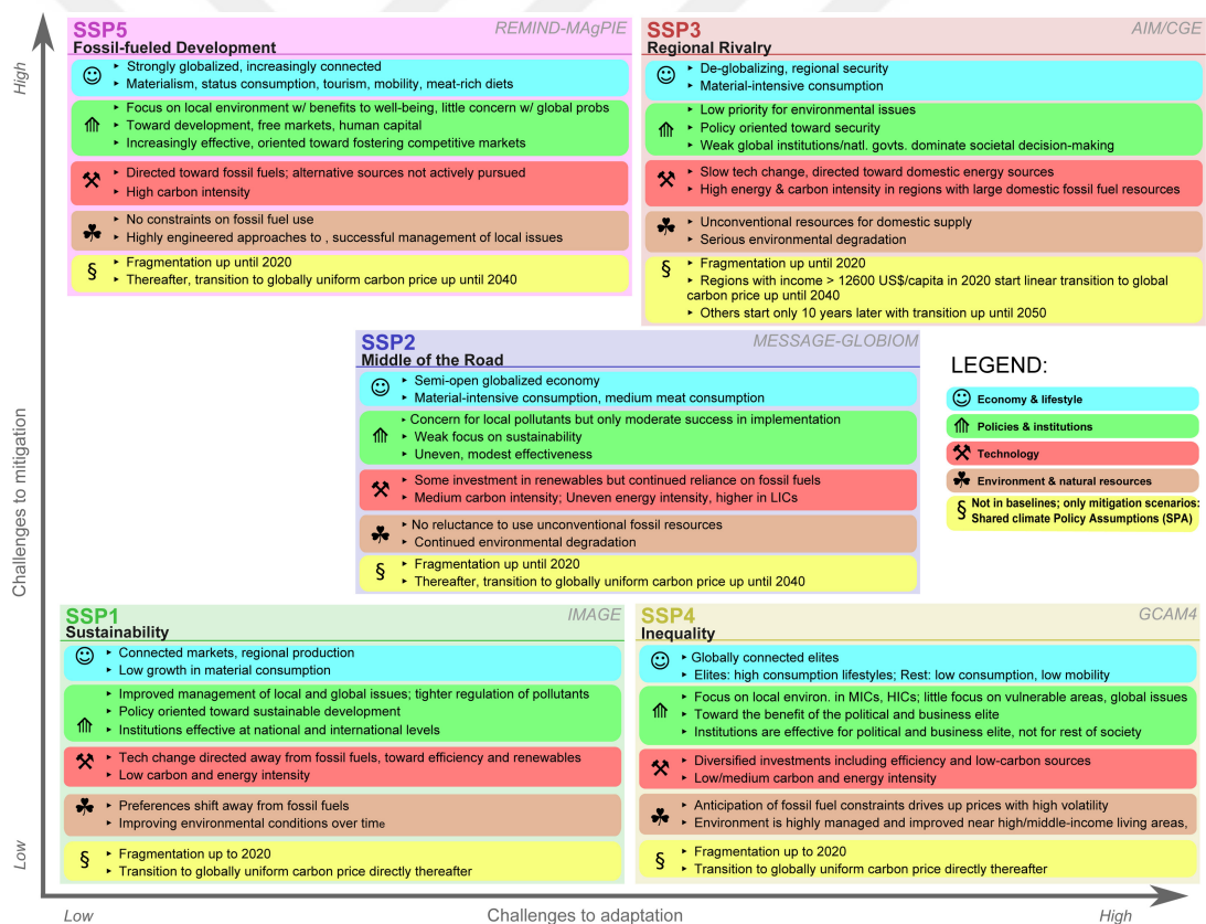
Figure 1.2: Classification of SSPs
