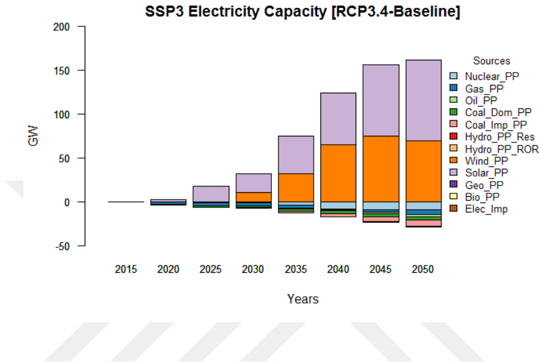
Figure 3.19: Electricity capacity difference in SSP3 for RCP3.4
