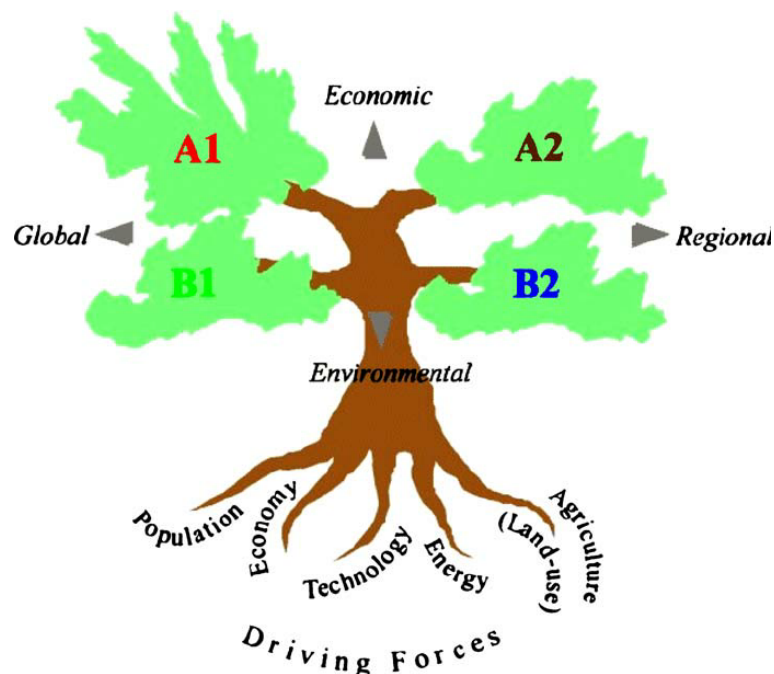
Figure 1.1: Classification of SRES scenarios
