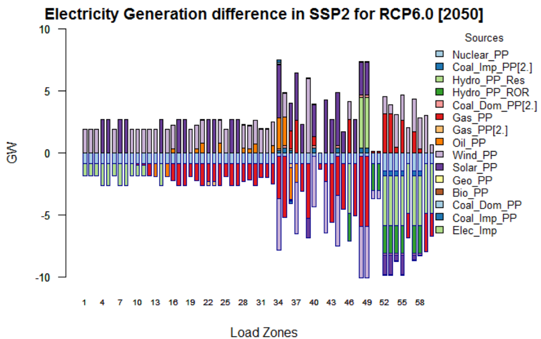
Figure 3.35: Electricity supply in SSP2 for Baseline [2050]
