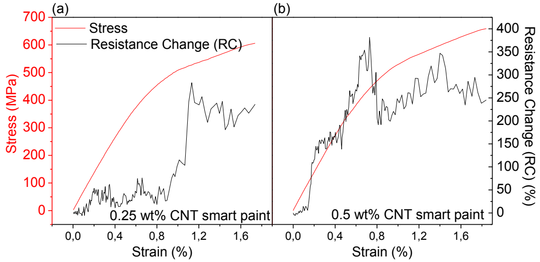
Figure 4.14 : Stress / Resistance Change vs. Strain results for plastic deformation (a) 0.25 wt% CNT specimen, (b) 0.5 wt% CNT specimen.
