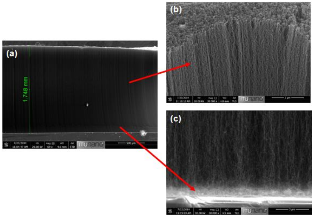
Figure 3.3 : SEM images of A-CNTs synthesized by CVD method showing the top and bottom sections of aligned arrays.
