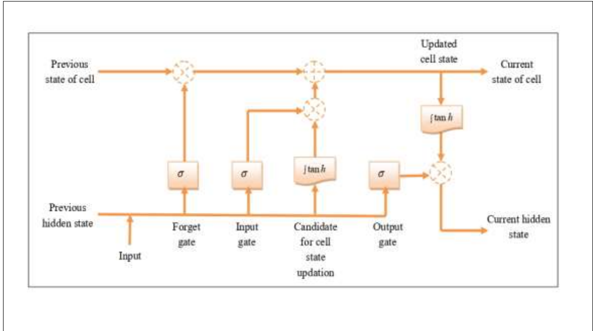
Figure 3.7: Diagrammatic Representation of the Conventional LSTM Model.
