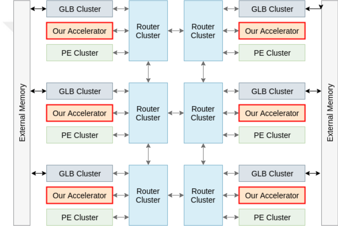
Figure 5.10: Top level architecture for the integration of the reuse-centric accelerator into Eyeriss [2].
