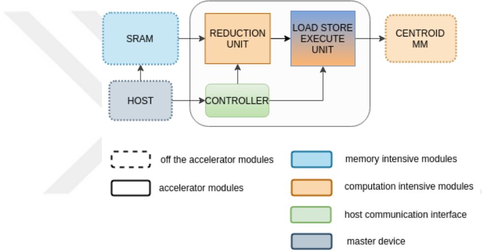
Figure 4.2: Base reuse-centric accelerator architecture.
