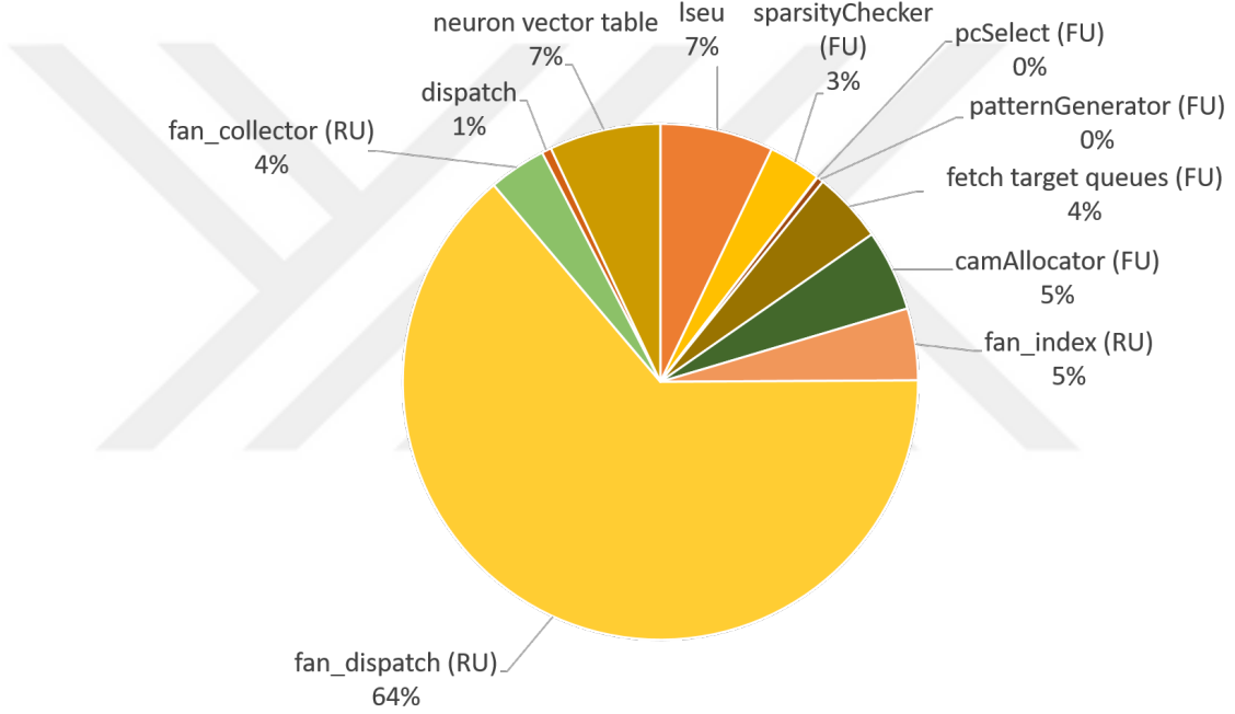
Figure 6.5: Area breakdown of the modules in the advanced architecture based on the lookup tables (LUTs) and registers.
