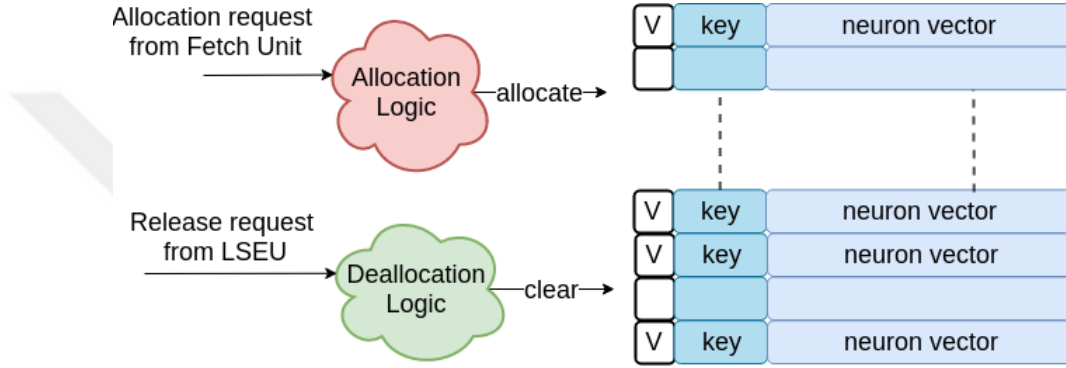
Figure 5.3: Banked content addressable memory and neuron vector allocation.
