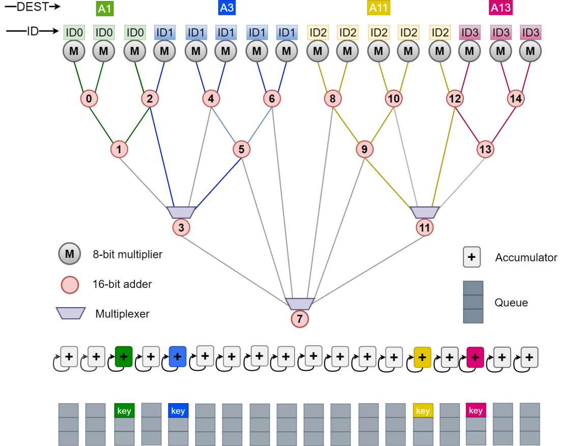
Figure 5.5: Forwarding adder network topology with collector and index modules.
