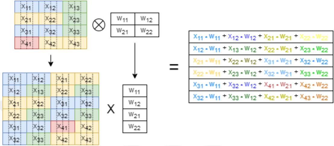
Figure 2.1: An example matrix multiplication based convolution operation leveraging general reuse. Color coding shows the available reuse.
