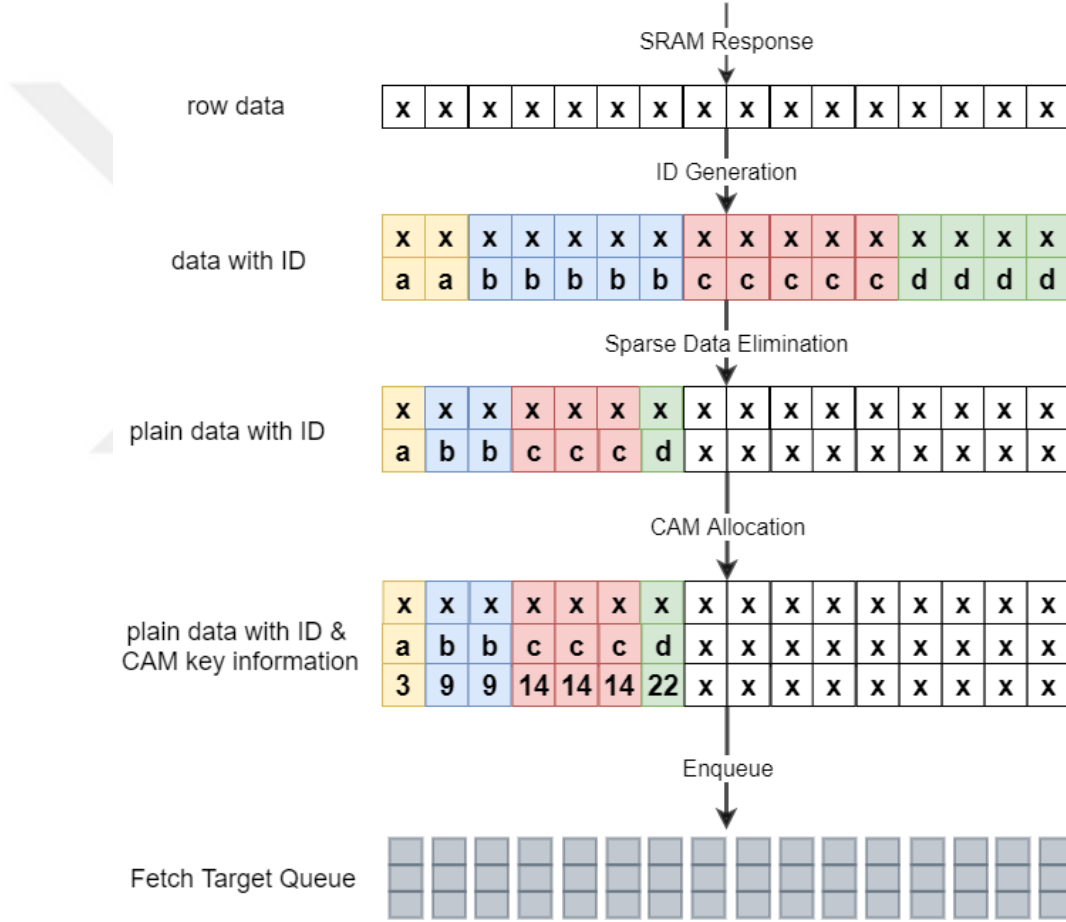
Figure 5.2: An example fetch unit execution.
