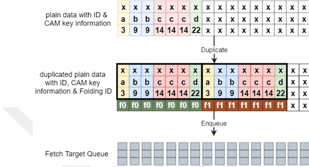
Figure 5.8: Fetch unit supporting fold operation.
