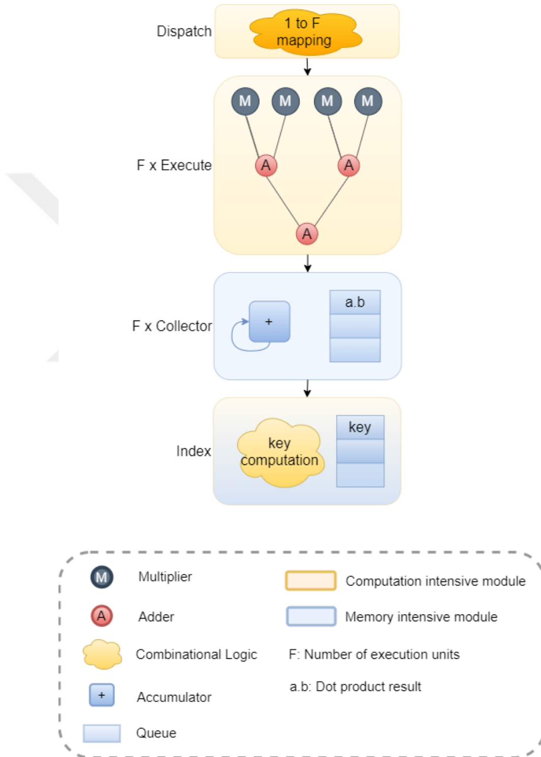
Figure 5.4: Details of the reduction unit with four modules, namely dispatch, execute, collector, and index.
