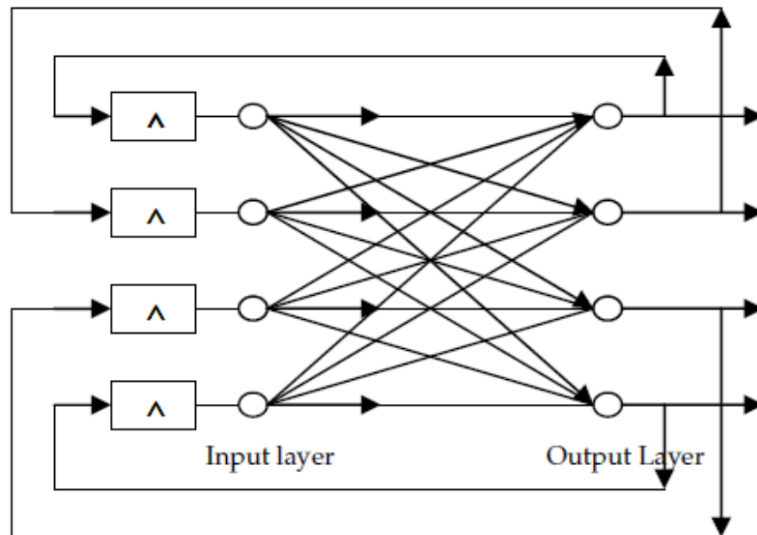
Figure 3.4: Recurrent Network
