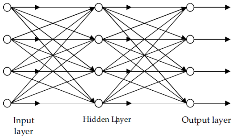
Figure 3.3: Multilayer Feed Forward Network
