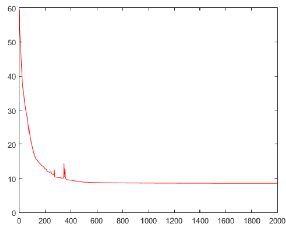
Figure 4.1: Error graph performance using ANN-GA for Breast Cancer Dataset
