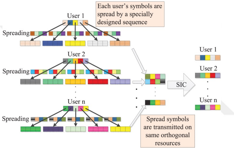
Figure 1.12: MUSA code generation and receiver structure [4]
