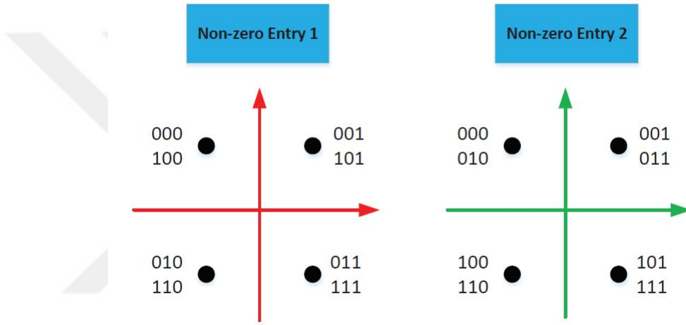
Figure 1.11: Example of SCMA 8-point codebook [5]
