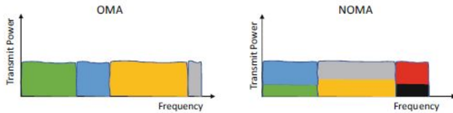
Figure 1.9: OMA and NOMA power and spectral allocations [3]
