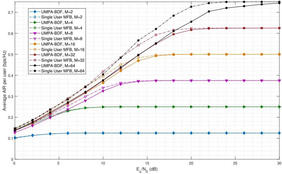
Figure 4.18: AIR vs E_s/N_0 dB for MUSA N_c = 8 , M = 2, 4, 8, 16, 32, 64 , L_c = 8 N = 12 , 200% Loading;; Gaussian distributed tabs for MAC
