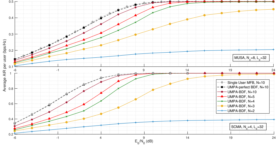
Figure 4.7: AIR vs E_b/N_0 for MUSA ( N_c = 8, K = 12 ) and SCMA ( N_c = 4, K = 6 ) under 150% loading, M = 16, L_c = 32 N = 1, 2, 3, 4, 5, 10 ; Gaussian distributed tabs for MAC
