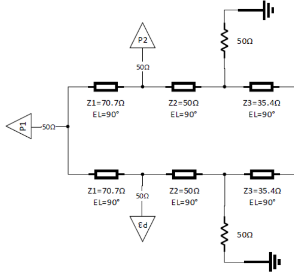
Figure 1.1: Circuit Model of Conventional Gysel Power Divider
