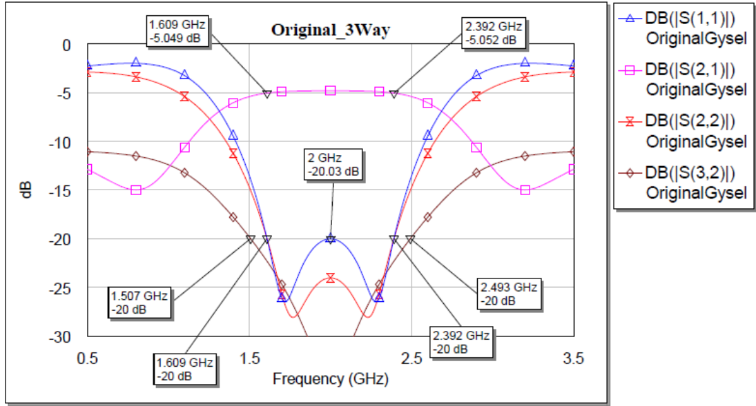
Figure 5.2: Traditional Gysel Power Divider Scattering Parameters, 3 Way
