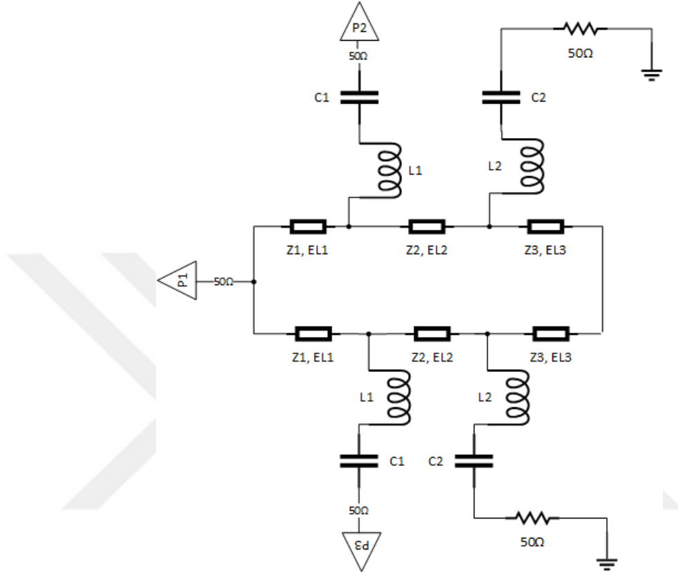
Figure 3.1: Proposed Modified Gysel Power Divider Topology
