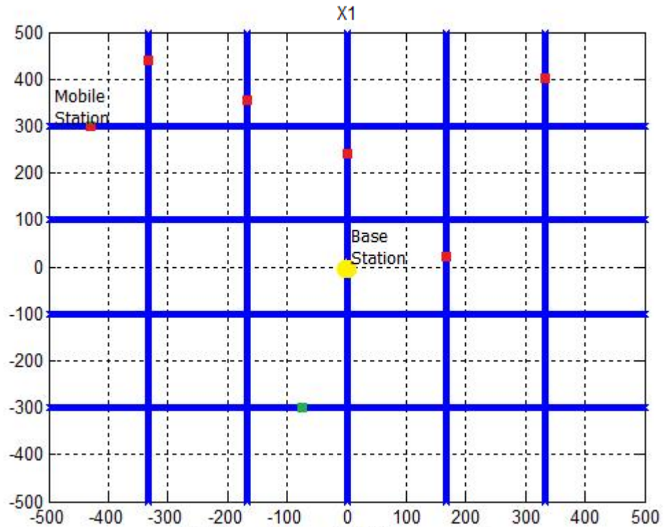
Figure 4.2: Simulation Environment
