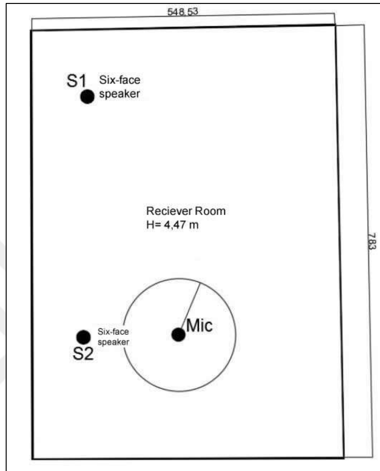
Figure 21. Top view of the speaker and microphone location in the receiver room (Figure from TSE Tuzla Acoustic Laboratory Test Report for Eray Erdemli)
