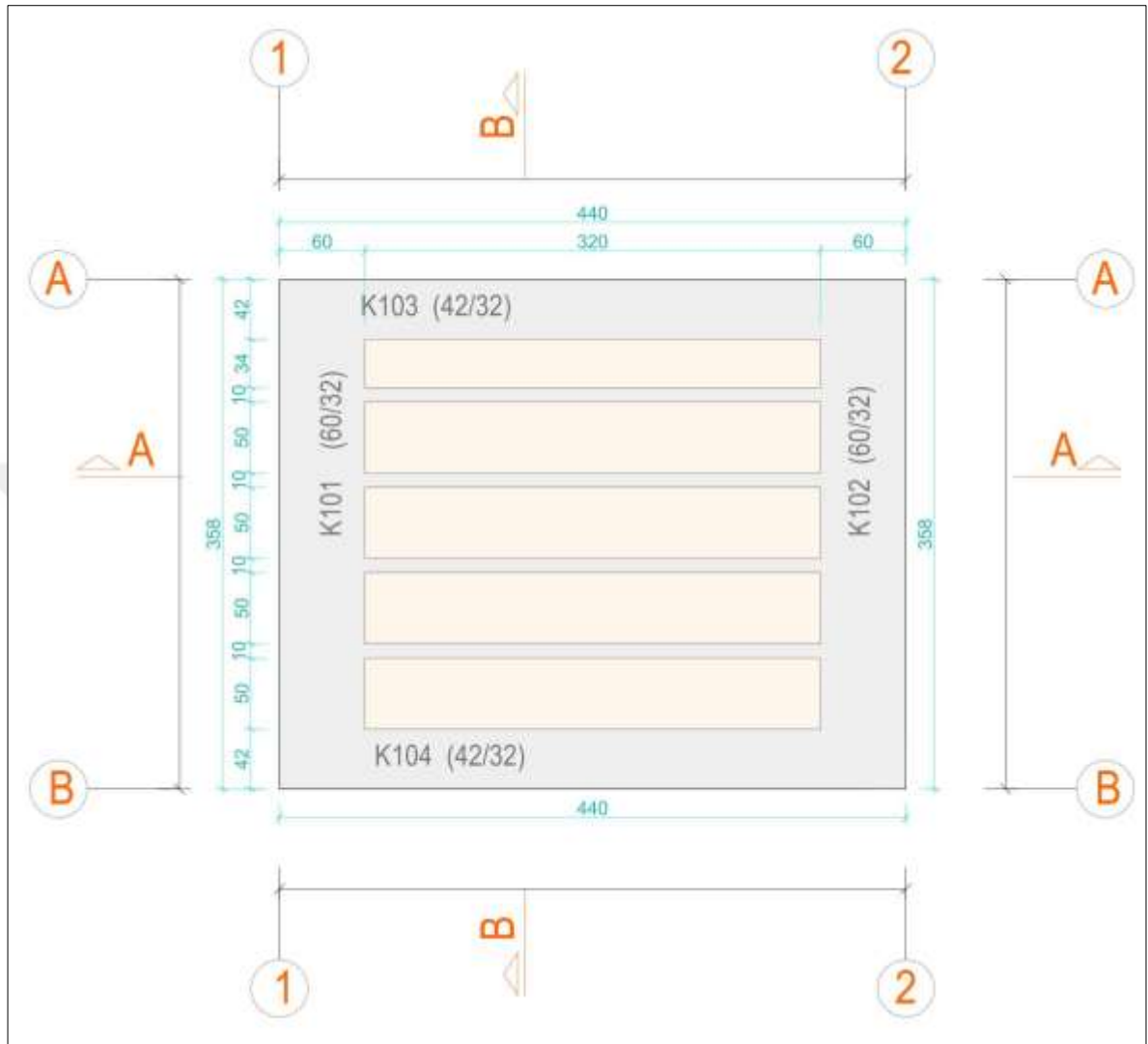
Figure 4. Top view of the sample one way hollow core slab system, not in scale
