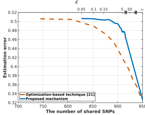
(a) Error vs. utility for the proposed SNP sharing mechanism and the optimization-based technique.
