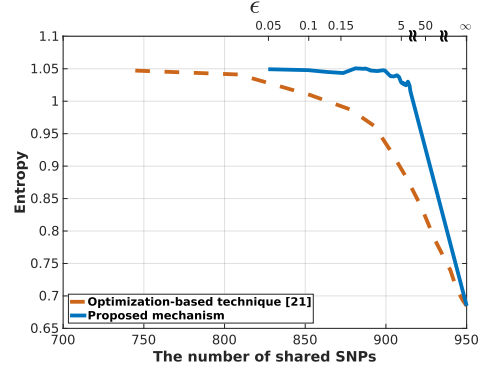
(b) Entropy vs. utility for the proposed SNP sharing mechanism and the optimization-based technique.
