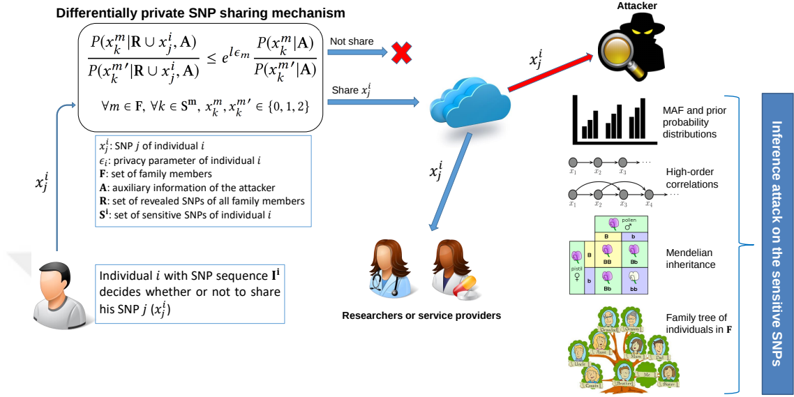
Figure 4.1: The donor (individual i ) wants to share his SNP sequence with a service provider. We illustrate one instance of this sharing for SNP x_j^i .
