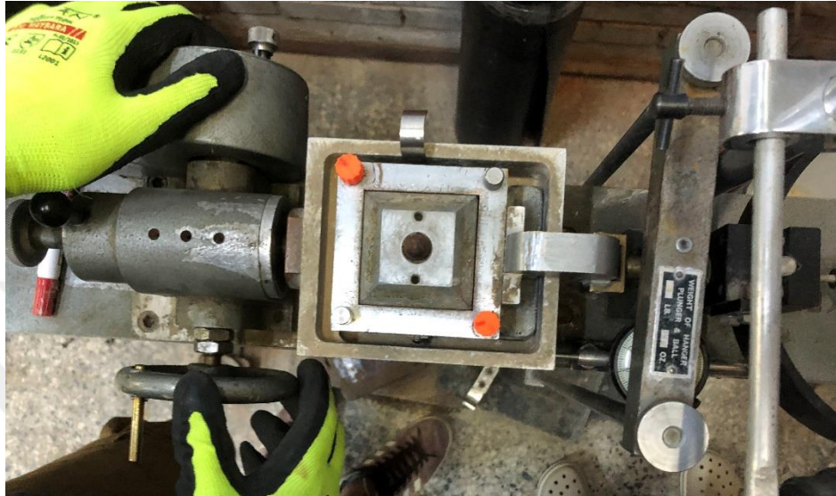
Figure 3.24 - Assembled and placed shear box assembly to the shearing device.
