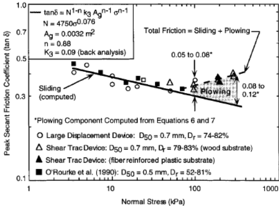
Figure 2.4 - Interfacing mechanism between smooth HDPE geomembrane - dense Ottawa 20/30 sand interface (Dove & Frost, 1999)
