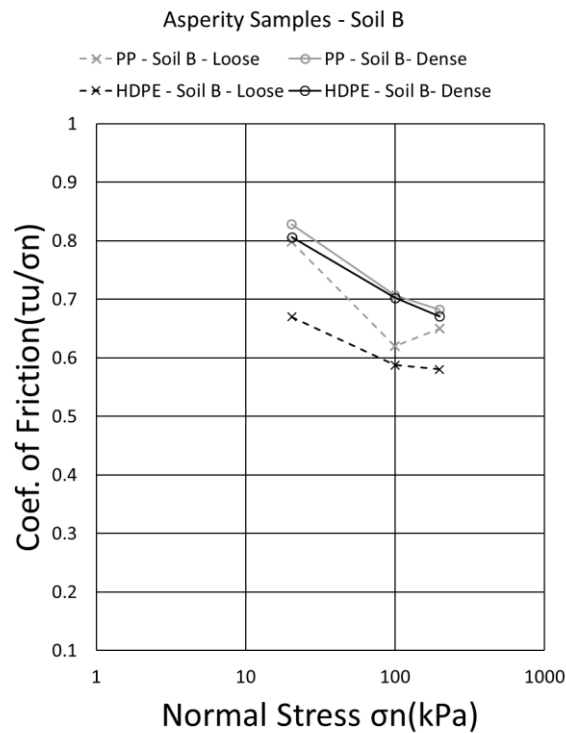
Figure 4.21 - Coefficient of friction vs. Normal Stress curves plotted using peak shear strength parameters of direct shear test for asperity HDPE and PP geomembranes interfaced with soil B.
