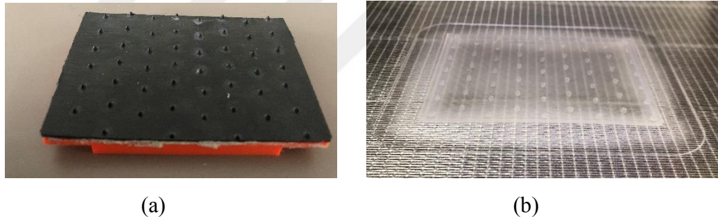
Figure 3.18 - Side by side comparison of: (a) Reference asperity HDPE geomembrane; (b) PP asperity geomembrane
