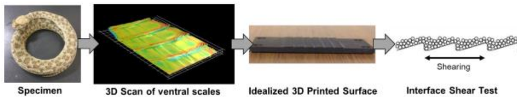
Figure 2.20 - Development workflow of snake-inspired surfaces (Martinez & Palumbo, 2018)
