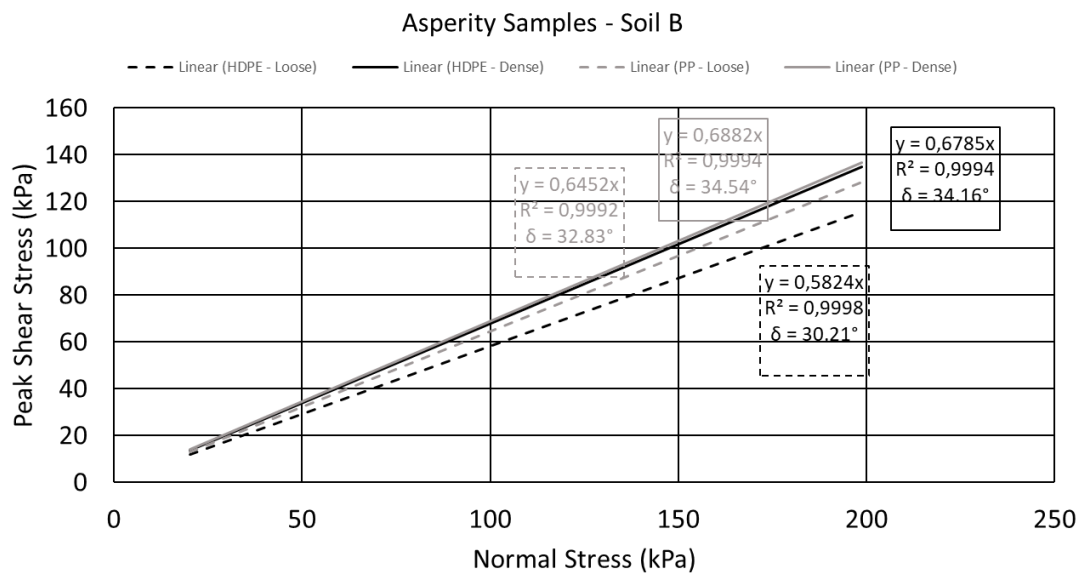
Figure 4.22 - Mohr – Coulomb failure envelopes of the direct shear tests performed on asperity HDPE and PP geomembranes interfaced with soil B.
