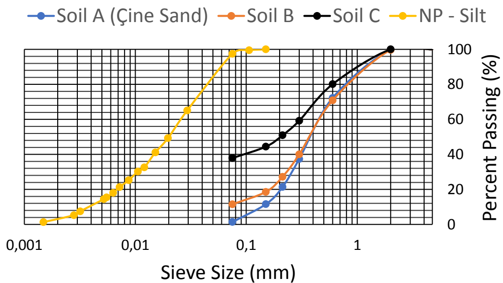
Figure 3.5 - Particle size distributions of soil mixtures A, B, and C
