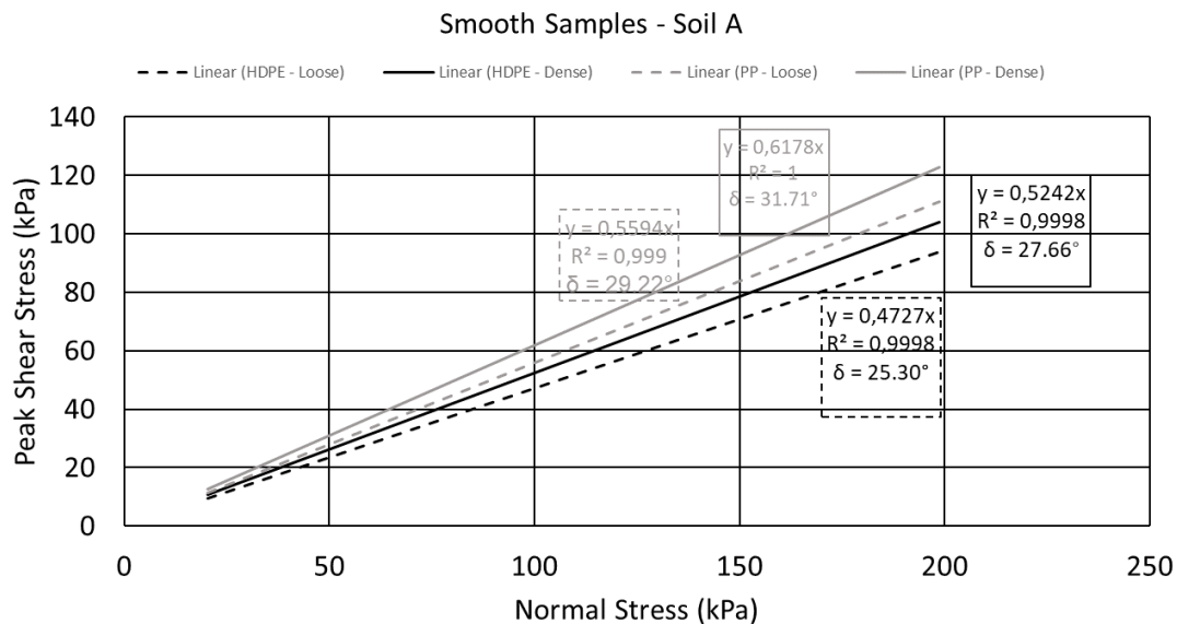
Figure 4.10 – Mohr – Coulomb failure envelopes of the direct shear tests performed on smooth HDPE and PP geomembranes interfaced with soil A.
