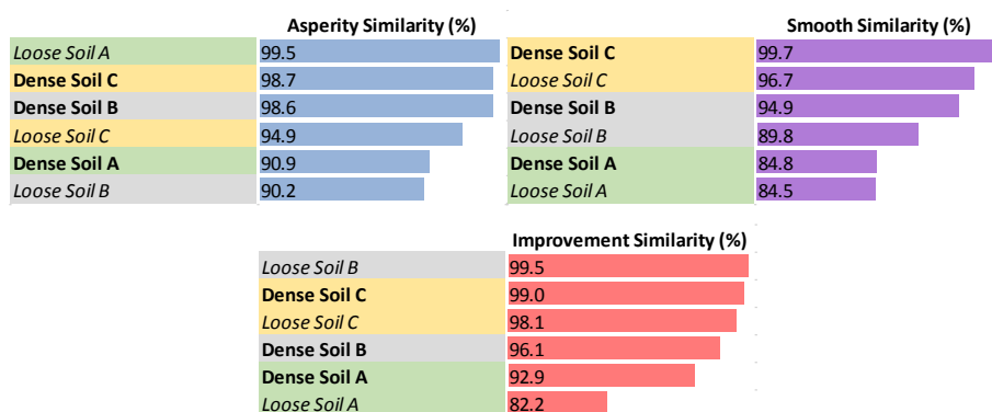
Figure 4.26 – Similarity index values for all soil types.
