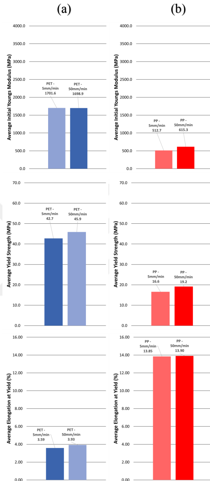
Figure 4.6 - Comparison of (a) re-PETG, (b) PP specimens regarding average initial Young's modulus, average yield strength, and average elongation at yield
