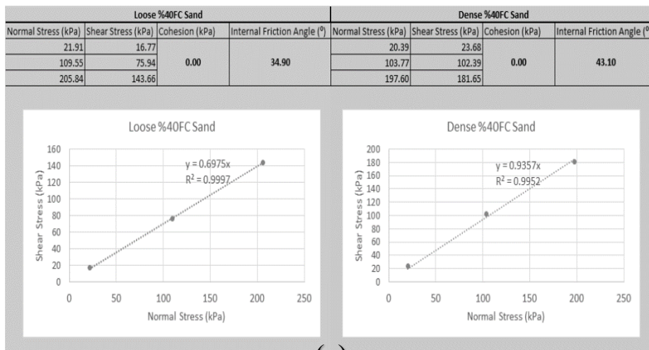
Figure 3.6 - Internal shear behavior Mohr-Coulomb failure envelopes for loose and dense conditions of (a) Soil A; (b) Soil B; (c) Soil C
