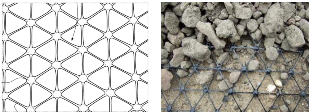
Figure 2.1 - Triaxial HDPE geogrid developed by TENSAR Co.
