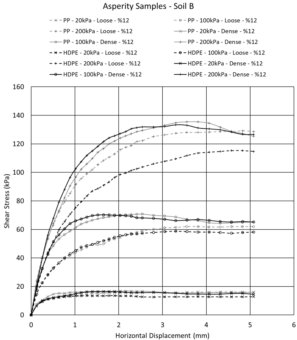
Figure 4.20 - Shear Stress vs. Horizontal Displacement curves of direct shear tests performed on asperity HDPE and PP geomembranes interfaced with soil B
