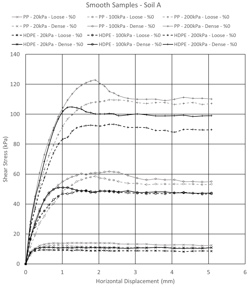
Figure 4.8 – Shear Stress vs. Horizontal Displacement curves of direct shear tests performed on smooth HDPE and PP geomembranes interfaced with soil A.
