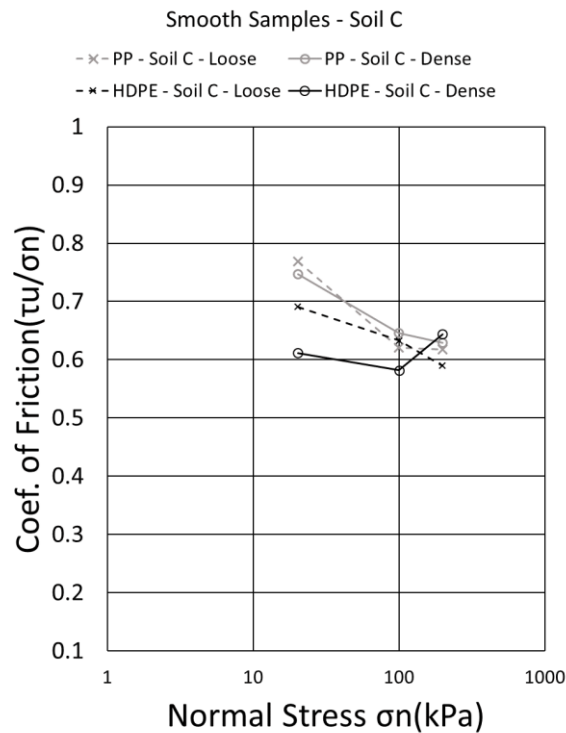
Figure 4.15 - Coefficient of friction vs. Normal Stress curves plotted using peak shear strength parameters of direct shear test for smooth HDPE and PP geomembranes interfaced with soil C.
