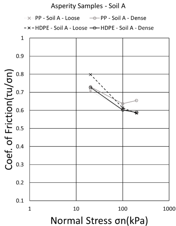
Figure 4.18 - Coefficient of friction vs. Normal Stress curves plotted using peak shear strength parameters of direct shear test for asperity HDPE and PP geomembranes interfaced with soil A.
