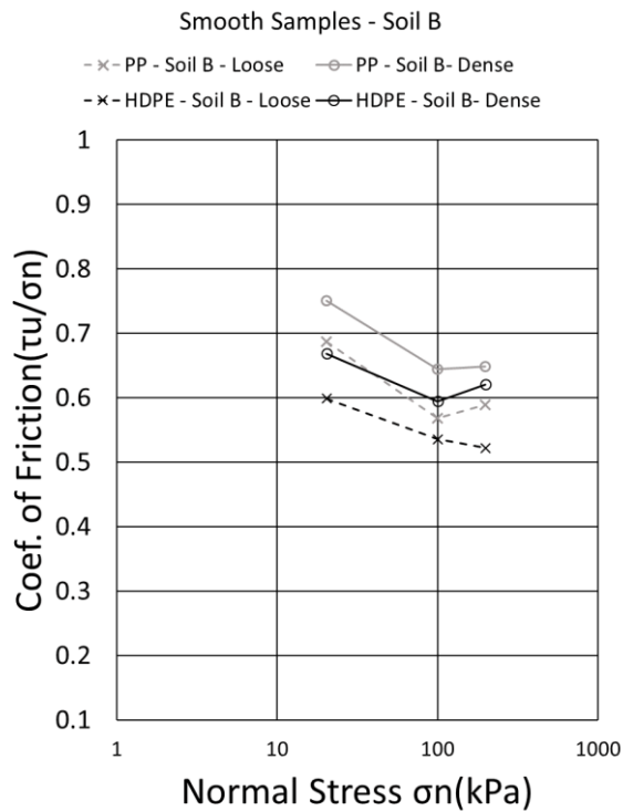
Figure 4.12 - Coefficient of friction vs. Normal Stress curves plotted using peak shear strength parameters of direct shear test for smooth HDPE and PP geomembranes interfaced with soil B.
