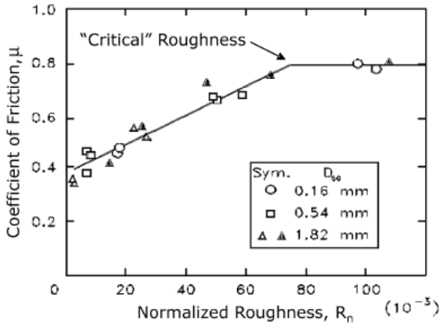
Figure 2.8 - Normalized interface roughness versus coefficient of friction relationship (Uesugi & Kishida, 1986).
