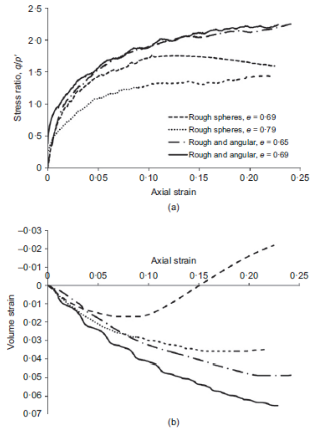
Figure 2.15 - Triaxial shear behavior of pseudo-sand particles: (a) stress ratio; (b) volumetric strain vs. axial strain (Hanaor et al., 2016).
