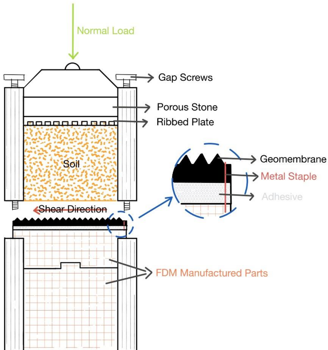
Figure 3.14 - Schematic drawing of the direct shear test setup (not to scale).
