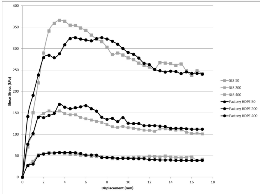
Figure 2.19 - Comparison of reference HDPE and SLS manufactured geomembranes interfaced with sand(Gary John Fowmes et al., 2017).
