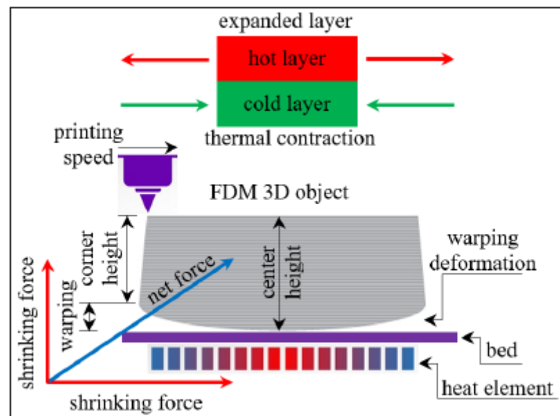
Figure 2.12 - Schematic drawing of the warping phenomenon (Alsoufi & El-Sayed, 2017).
