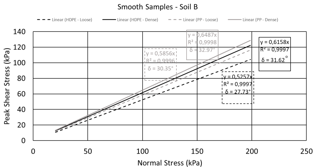
Figure 4.13 - Mohr – Coulomb failure envelopes of the direct shear tests performed on smooth HDPE and PP geomembranes interfaced with soil B.
