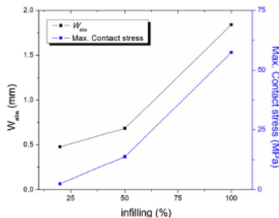
Figure 2.13 - Warpage and maximum contact stress values with increasing infill ratios for an FDM manufactured PP part (Bachhar et al., 2020).
