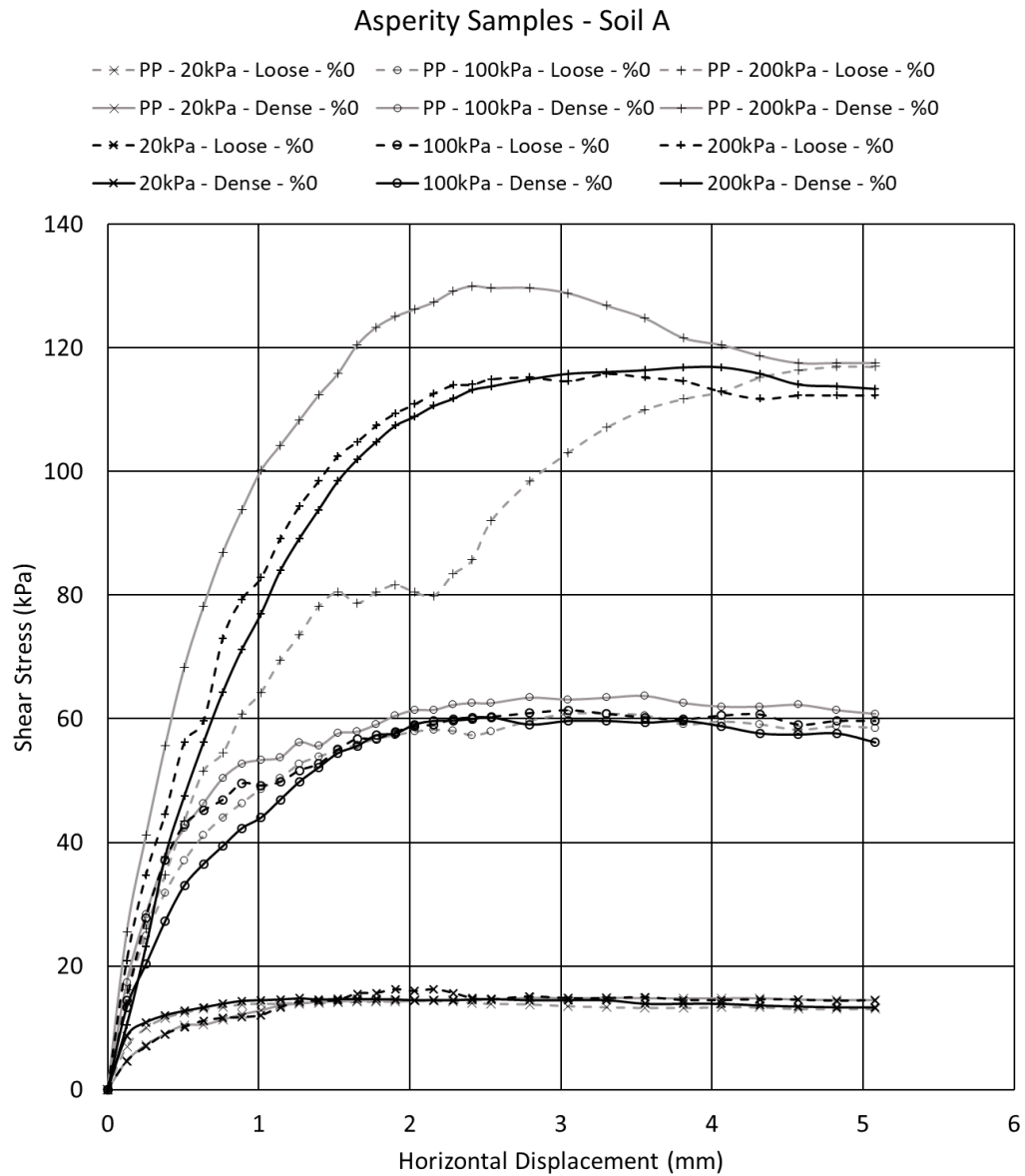
Figure 4.17 - Shear Stress vs. Horizontal Displacement curves of direct shear tests performed on asperity HDPE and PP geomembranes interfaced with soil A.
