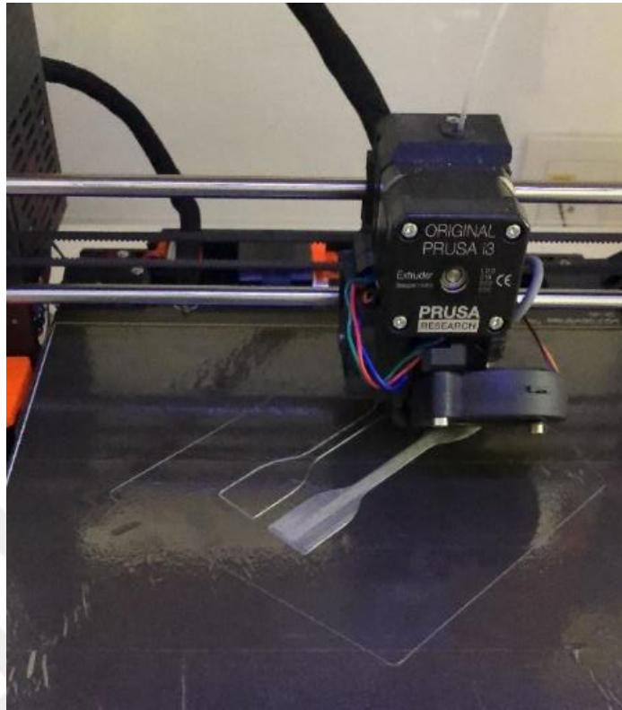
Figure 3.9 - 3D Printing of PP Tensile Strength Specimens
