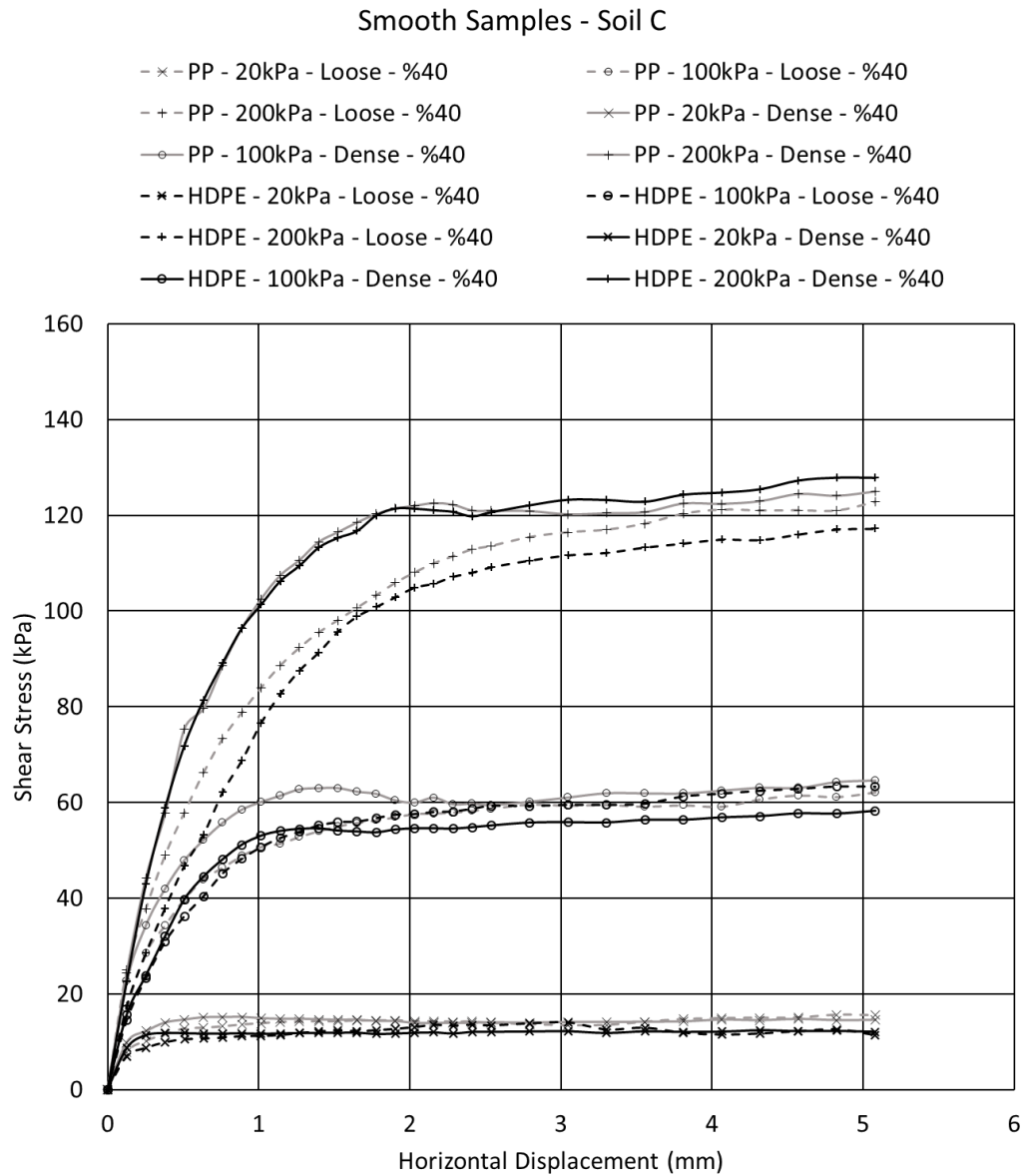
Figure 4.14 - Shear Stress vs. Horizontal Displacement curves of direct shear tests performed on smooth HDPE and PP geomembranes interfaced with soil C.
