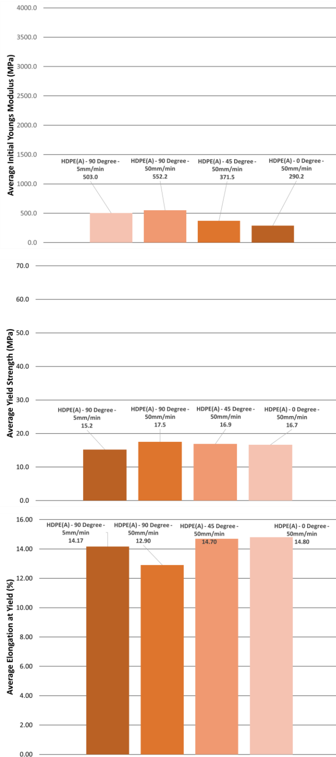
Figure 4.4 - Comparison of asperity HDPE specimens regarding average initial Youngs modulus, average yield strength, and average elongation at yield
