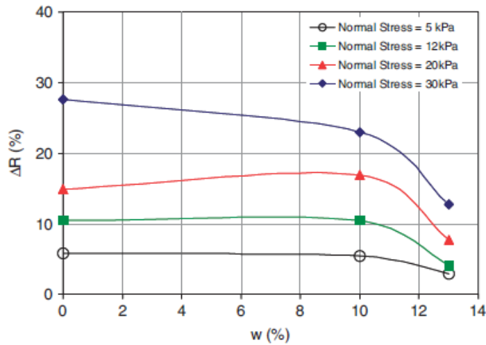
Figure 2.10 - Water content effect on the post-shear surface roughness silty sand - smooth HDPE geomembrane interfaces obtained by surface profilometry (Fleming et al., 2006).
