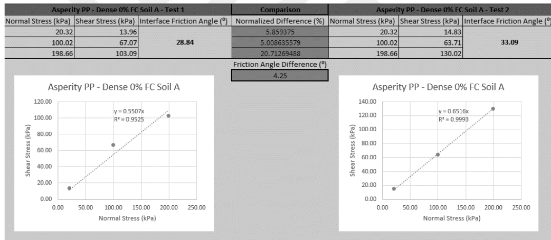
Figure 3.13 – Repeatability comparison between repeated tests involving asperity PP – dense soil A interface type.
