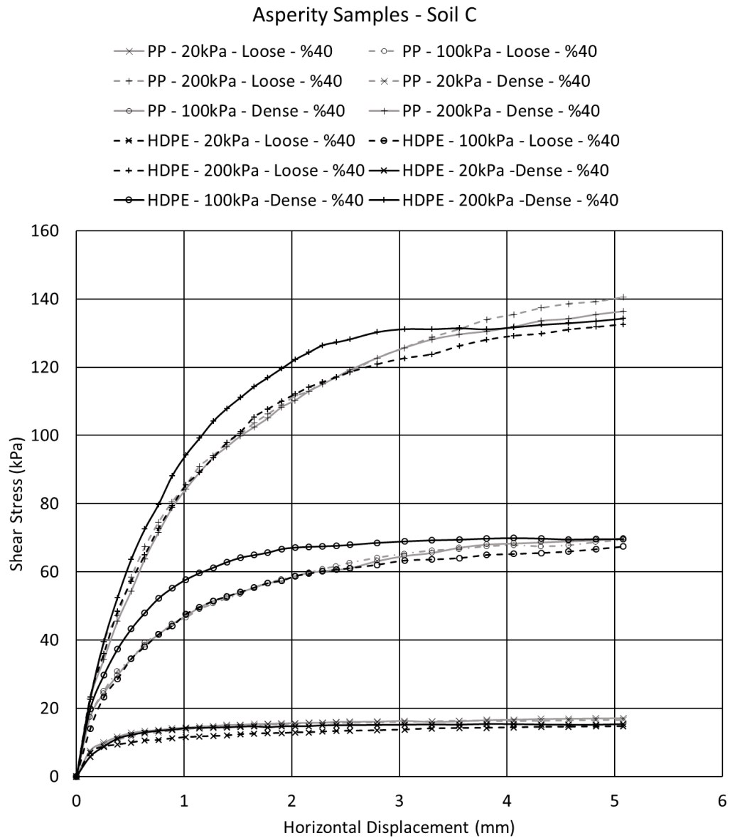
Figure 4.23 - Shear Stress vs. Horizontal Displacement curves of direct shear tests performed on asperity HDPE and PP geomembranes interfaced with soil C
