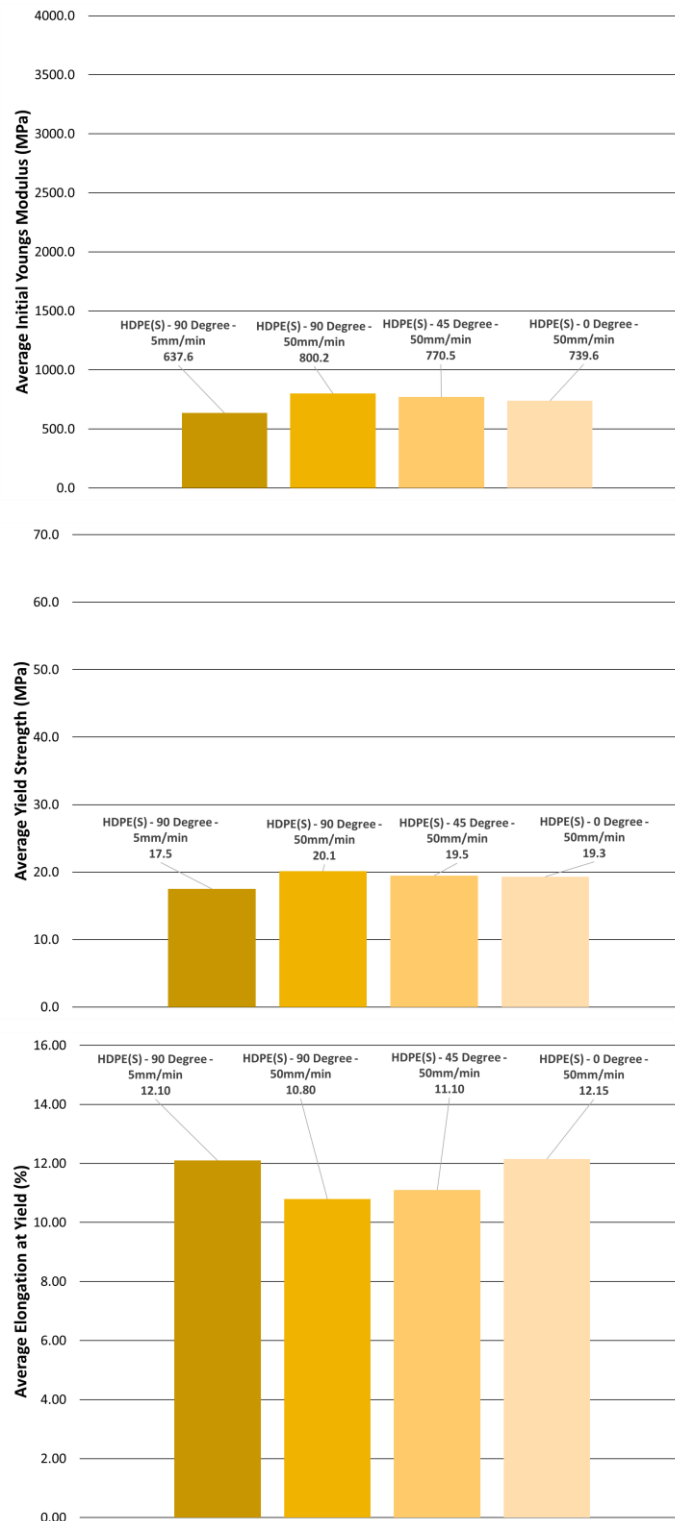
Figure 4.3 – Comparison of smooth HDPE specimens regarding average initial Young's modulus, average yield strength, and average elongation at yield.
