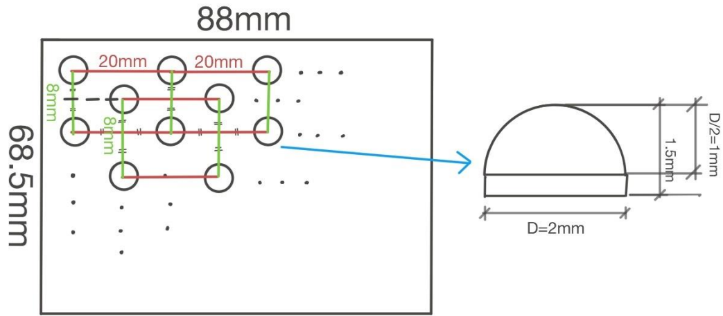
Figure 3.17 - Schematic drawing of the asperity geomembrane model derived from HDPE geomembrane.
