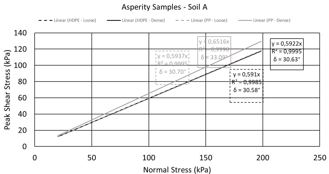
Figure 4.19 - Mohr – Coulomb failure envelopes of the direct shear tests performed on asperity HDPE and PP geomembranes interfaced with soil A.
