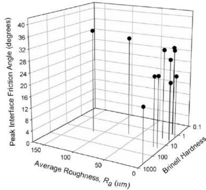
Figure 2.9 - Coupled effect of counterface roughness and hardness using Ottawa 20/30 sand
