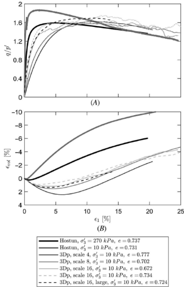
Figure 2.16 - Comparison between additively manufactured particles and benchmark sand using drained triaxial test results: (a) stress ratio; (b) volumetric strain vs. axial strain (Adamidis et al., 2020).
