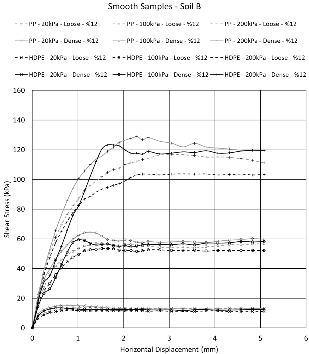
Figure 4.11 - Shear Stress vs. Horizontal Displacement curves of direct shear tests performed on smooth HDPE and PP geomembranes interfaced with soil B
