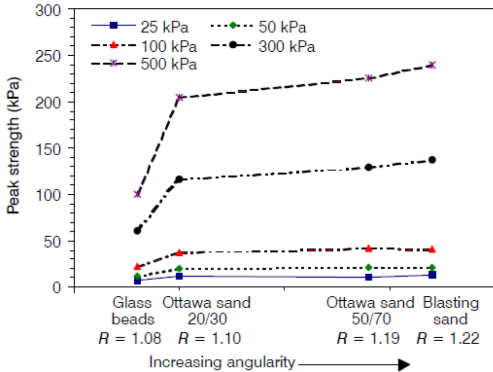
Figure 2.7 - Effect of particle angularity on peak interface shear strength in HDPE geomembrane - particle interfaces under different normal loads. (Zettler et al., 2000)
