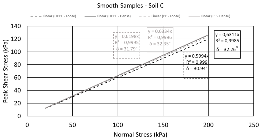
Figure 4.16 - Mohr – Coulomb failure envelopes of the direct shear tests performed on smooth HDPE and PP geomembranes interfaced with soil C.
