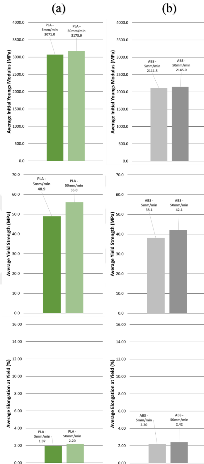
Figure 4.5 - Comparison of (a) PLA, (b) ABS specimens regarding average initial Young's modulus, average yield strength, and average elongation at yield
