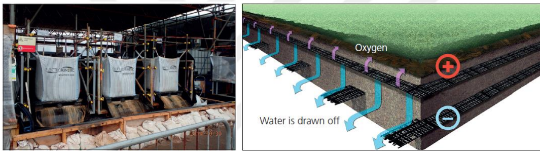
Figure 2.2 - Example pictures utilizing electrokinetic geosynthetics : (a) A dewatering bag ; (b) Drainage control on a sports turf (C. Jones et al., 2017)
