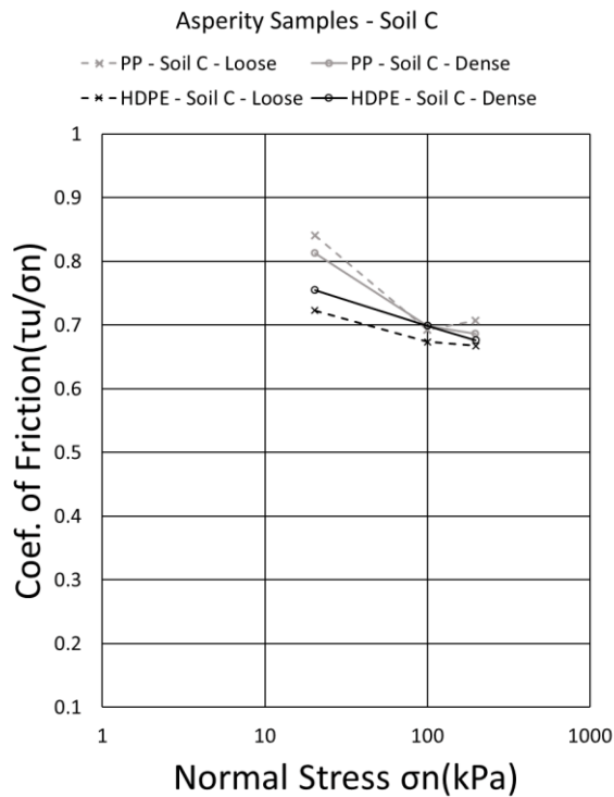
Figure 4.24 - Coefficient of friction vs. Normal Stress curves plotted using peak shear strength parameters of direct shear test for asperity HDPE and PP geomembranes interfaced with soil C.
