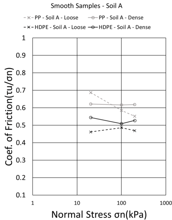
Figure 4.9 – Coefficient of friction vs. Normal Stress curves plotted using peak shear strength parameters of direct shear test for smooth HDPE and PP geomembranes interfaced with soil A.
