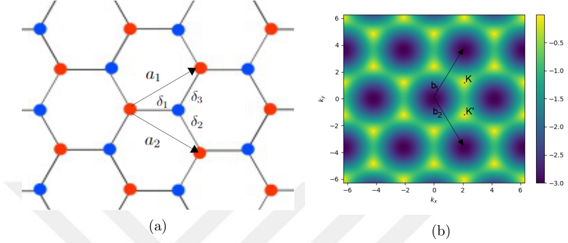
Figure 3.3: (a) Hexagonal lattice representation with nearest neighbour hopping. Sub-lattice A and sub-lattice B are shown with different colours. (b) Brillouin Zone of hexagonal lattice.
