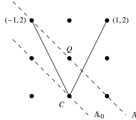
Figure 5.6 The cone C and the polyhedron Q with \bar{r} = [1, 1]
