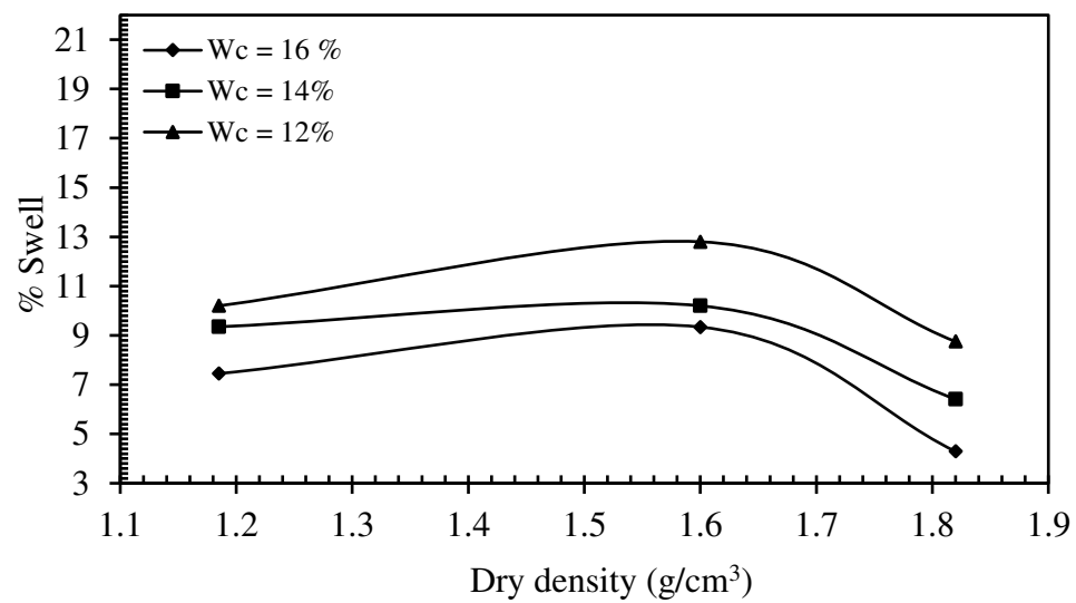
Figure 4.14: Total percent swelling versus dry density using different initial moisture contents under applied vertical stress of 15 kPa.
