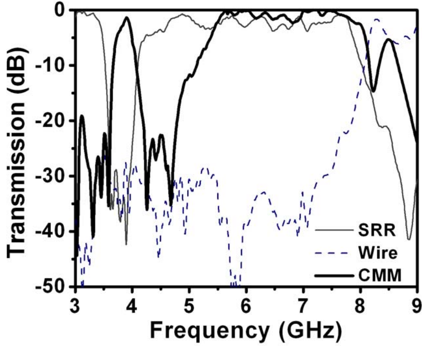
Fig 4.8: Measured transmission spectra of SRRs (solid line), wires (dashed line) and composite metamaterial (bold solid line).
