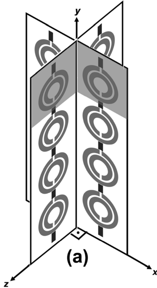
Fig. 5.1: Schematic drawing of 2D CMM structure. Shaded area shows the unit cell of the structure.
