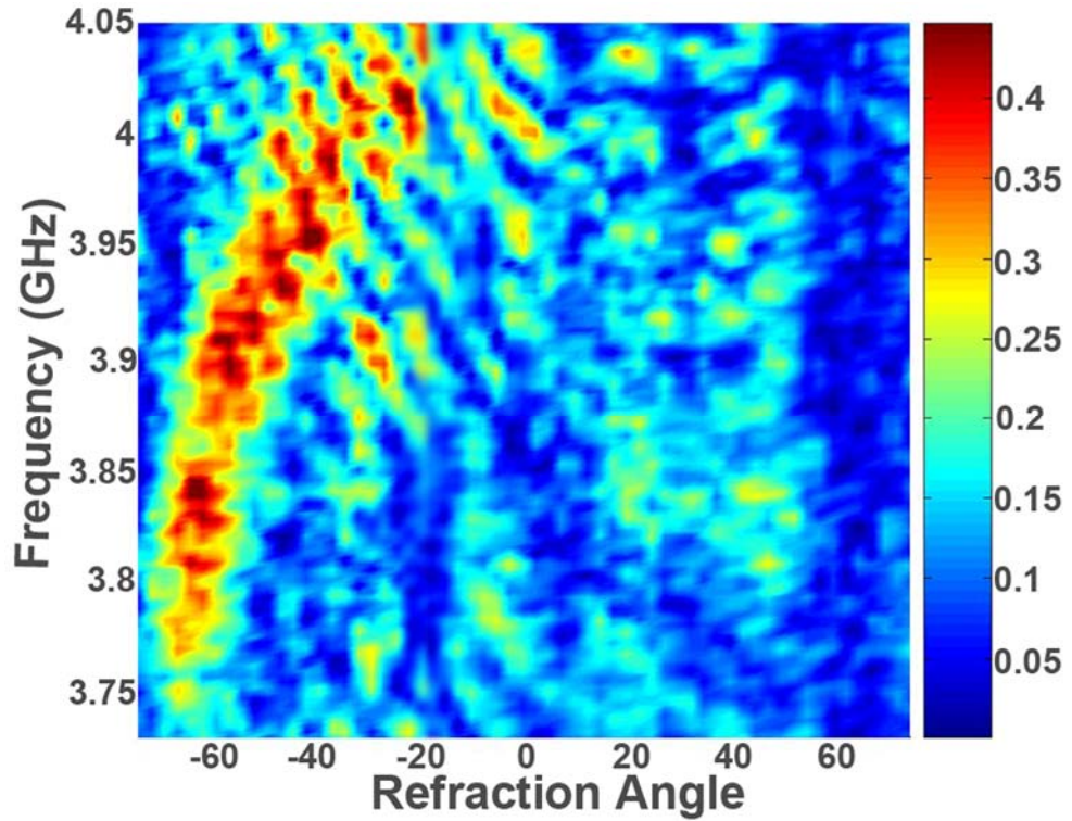
Fig. 5.6: Measured intensity spectrum of wedge shaped LHM sample as a function of frequency and refraction angle
