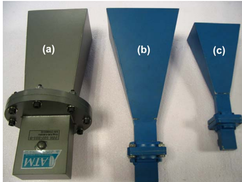
Fig 3.2: Horn antennas used to scan frequency regions (a) 3-7 GHz, (b) 7-14 GHz, (c) 10-22 GHz.
