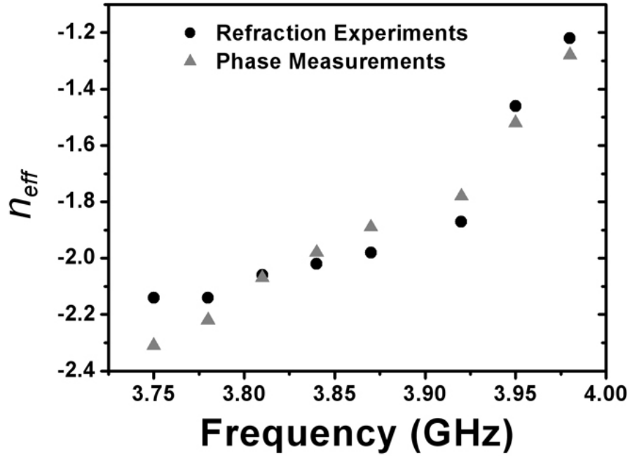
Fig. 5.10: The values of negative refractive indices obtained by using two experimental methods; the refraction experiments and the phase shift measurements. There is a quite good agreement for the values of negative refractive indices for these two experimental methods.
