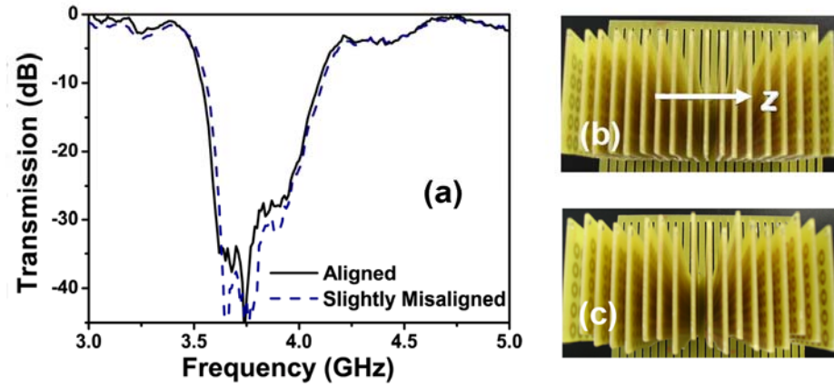
Fig. 4.3: (a) Measured transmission spectra of aligned (solid line) and slightly misaligned (dashed line) SRR structures. (b) Top view of aligned SRRs. (c) Top view of slightly misaligned SRRs.
