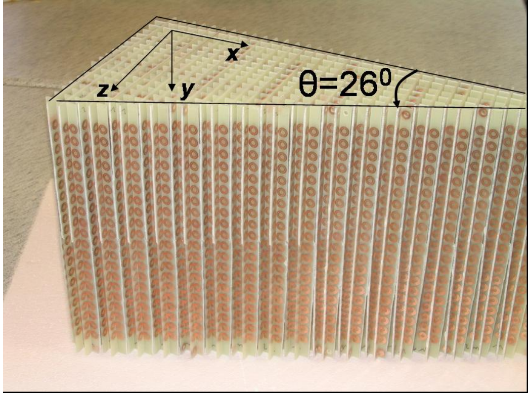
Fig. 5.5: 2D wedge structure.
