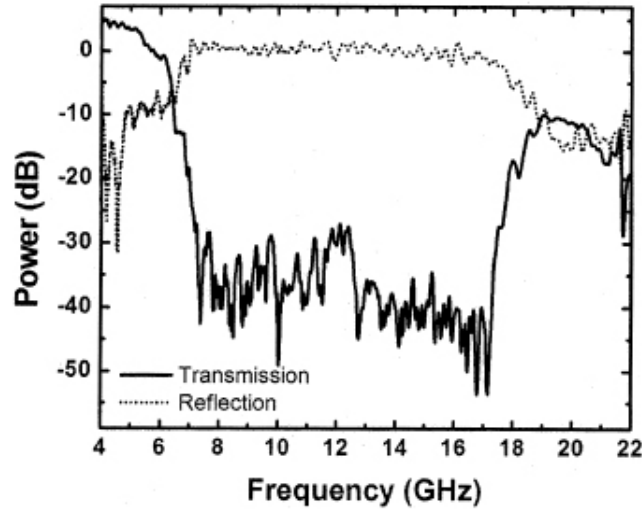
Fig. 3.6: Measured transmission and reflection spectra of the discontinuous thin wire medium.
