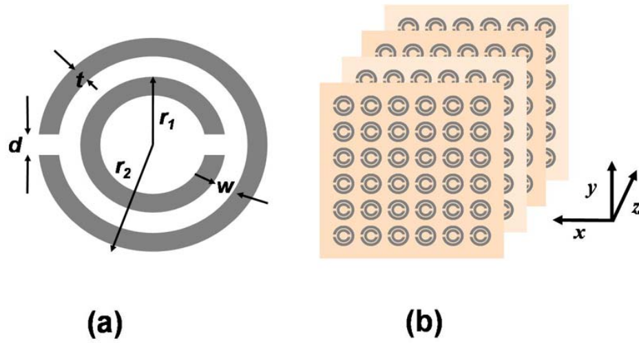
Fig. 3.7: Schematics of (a) single SRR unit, (b) periodical arrangement of SRRs
