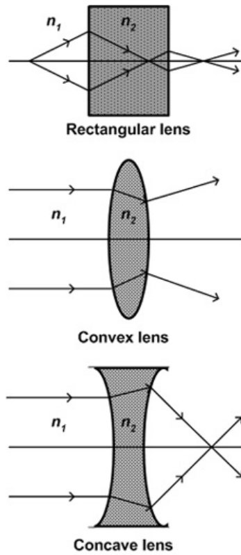
Fig 2.7: Beam path in (a) rectangular, (b) convex, (c) concave lenses made of left-handed materials.
