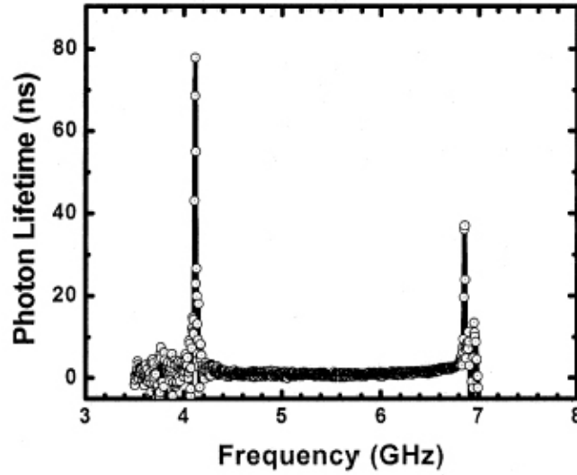
Fig. 3.9: Measured delay time, photon lifetime, as a function of frequency. The delay time increases rapidly as we approach the band edges.
