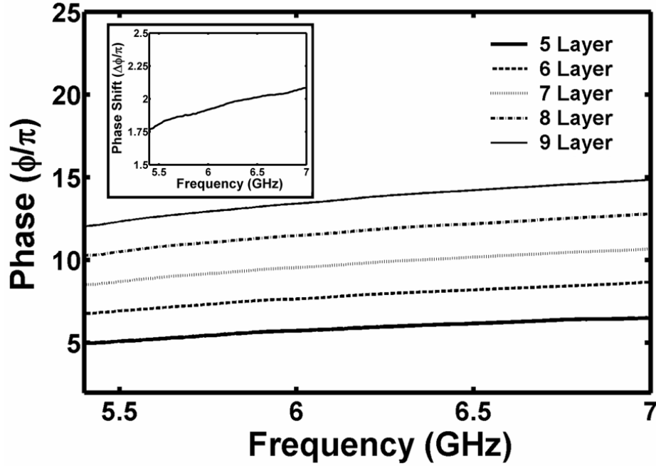
Fig. 5.8: Unwrapped transmission phase data obtained from different lengths of CMM between 5.4 - 7.0 GHz, where right-handed transmission peak takes place. Inset: Average phase difference between consecutive numbers of layers of CMM. Phase shift is positive between 5.4 - 7.0 GHz.
