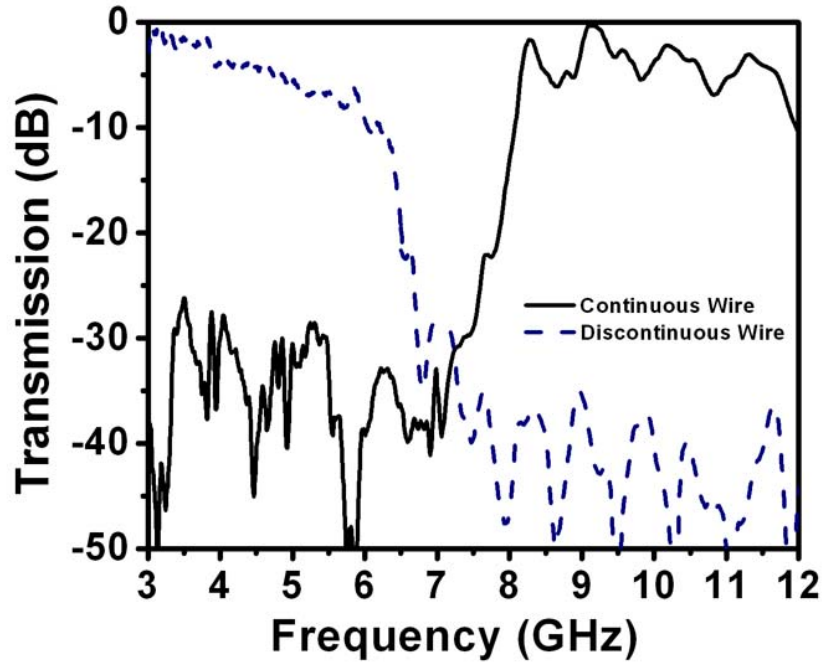
Fig. 4.6: Measured transmission spectra of continuous (solid line) and discontinuous wires (dashed line).
