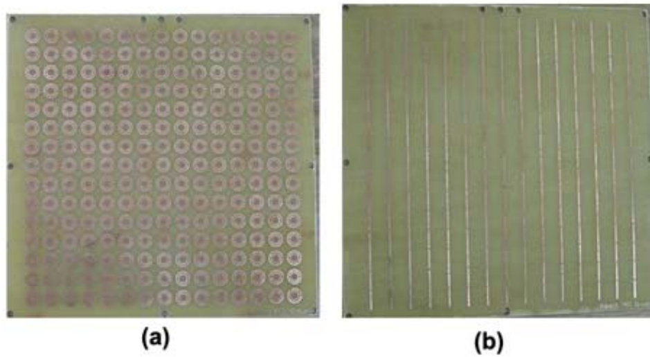
Fig. 3.4: Pictures of PCB boards consisting of (a) 15x15 SRR array, (b) 15x15 discontinuous wire array.
