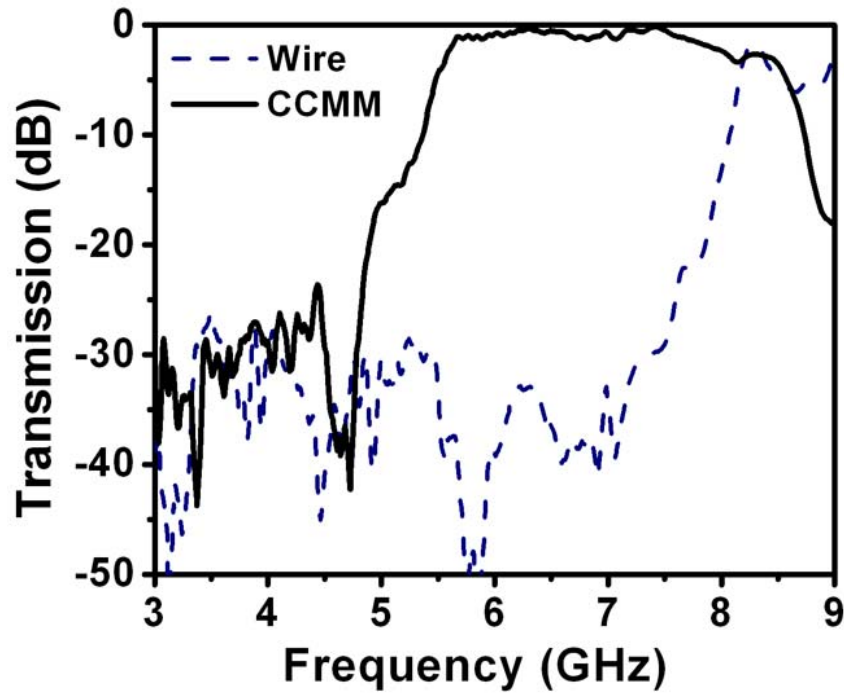
Fig. 4.7: Measured transmission spectra of wires (dashed line) and closed CMM (solid line) composed by arranging closed SRRs and wires periodically.
