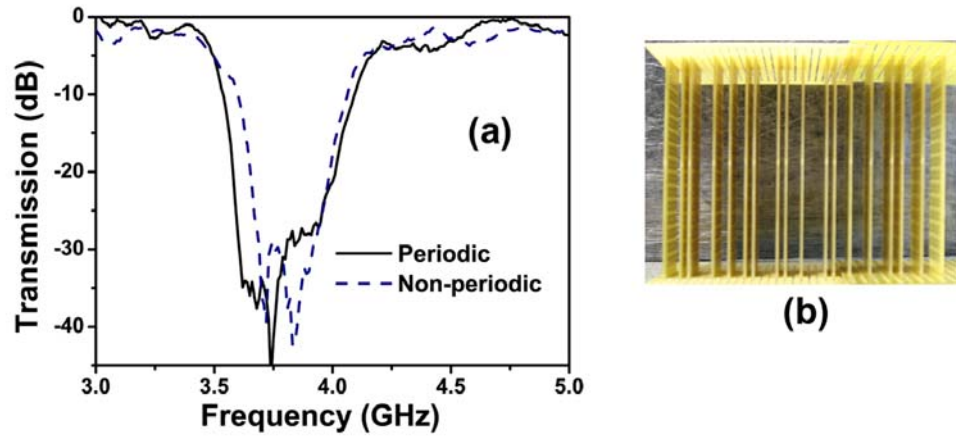
Fig. 4.5: (a) Measured transmission spectra of periodic (solid line) and non-periodic (dashed line) SRR structures. (b) Front view of non-periodic SRRs.
