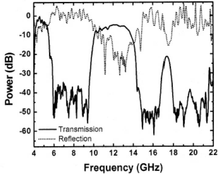
Fig 3.11: Measured transmission and reflection spectra of the composite metamaterial.
