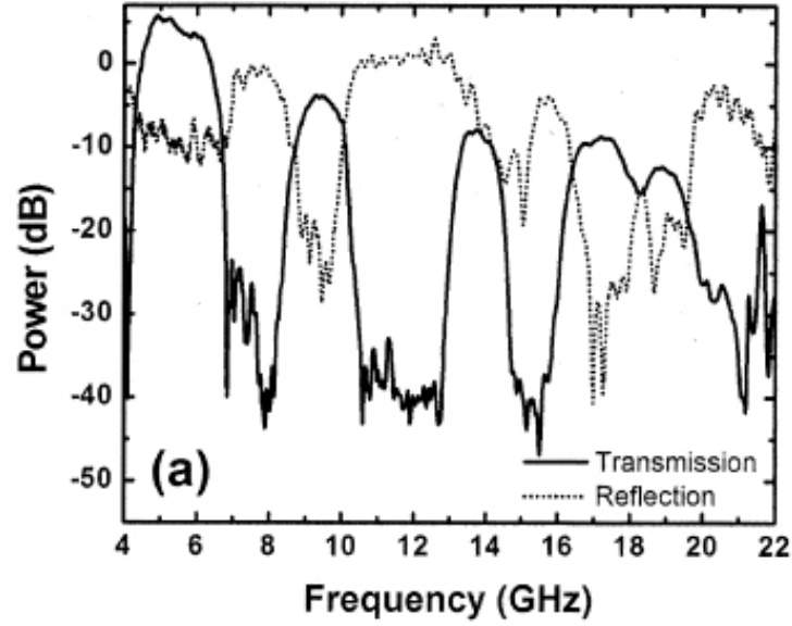
Fig. 3.8: Measured transmission and reflection spectra of the periodic split ring resonator medium.
