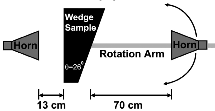
Fig. 5.4: Schematic drawing of experimental setup used for negative refraction experiment.
