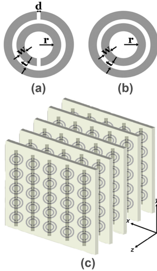
Fig. 4.1: Schematics of (a) a single split ring resonator (SRR) (b) a ring resonator with splits closed (CSRR) (c) Periodic CMM composed of SRRs on one side, wires on the other side of dielectric board.
