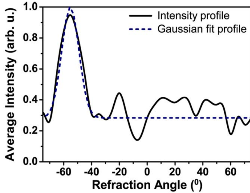
Fig. 5.7: The angular cross section of transmitted beam at 3.92 GHz.
