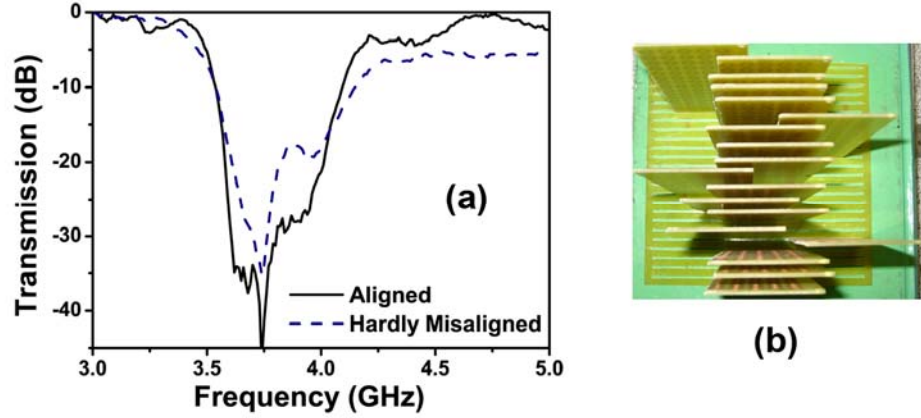
Fig. 4.4: (a) Measured transmission spectra of aligned and hardly misaligned SRR structures. (b) Top view of hardly misaligned SRRs.
