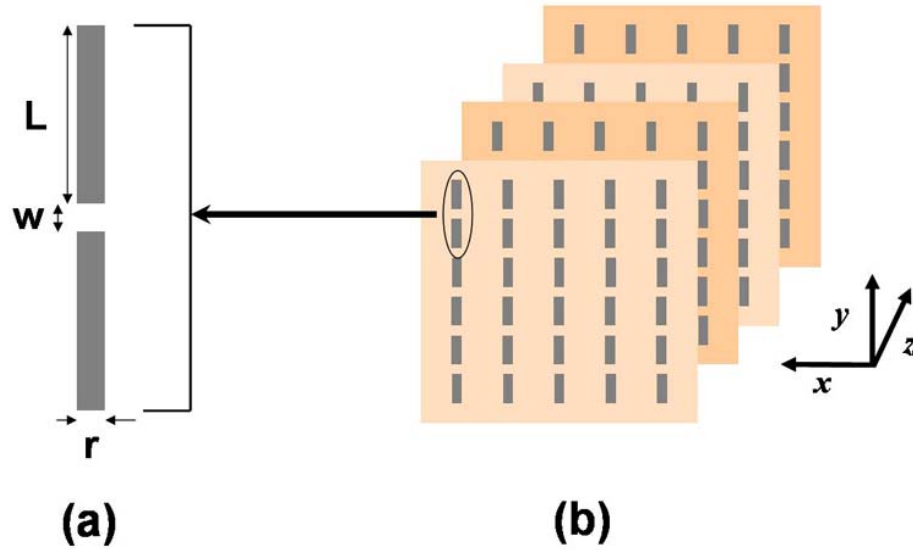
Fig. 3.5: Schematic drawings of (a) two wire strips separated by a gap, (b) periodical arrangement of discontinuous wire strips.
