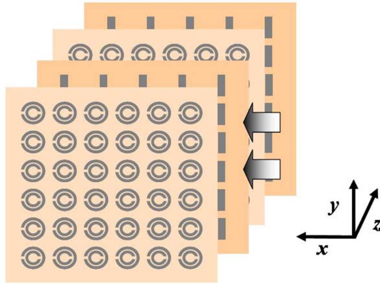
Fig 3.10: Schematic drawing of periodically arranged composite metamaterial composed of alternating layers of SRRs and wires.
