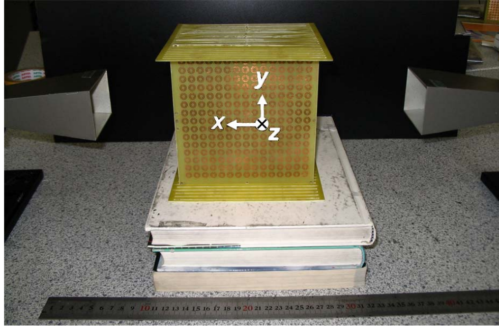
Fig 3.1: Experimental setup for transmission measurements.
