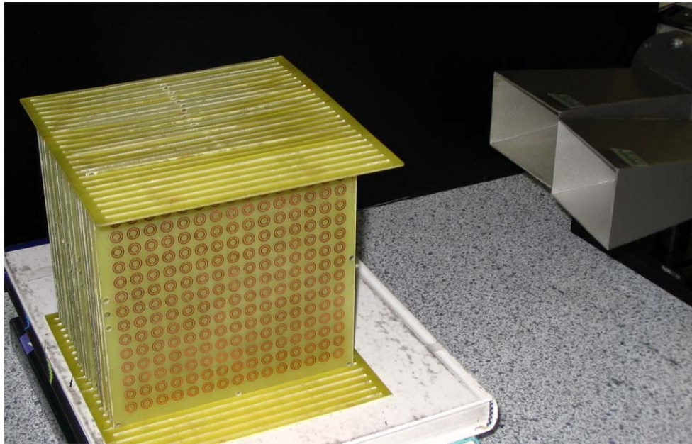
Fig 3.3: Experimental setup for reflection measurements
