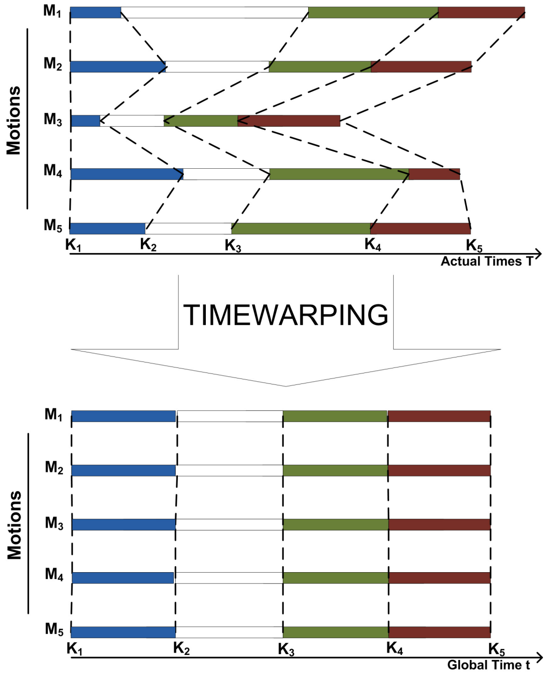
Figure 4.5: The effect of timewarping on motions.
