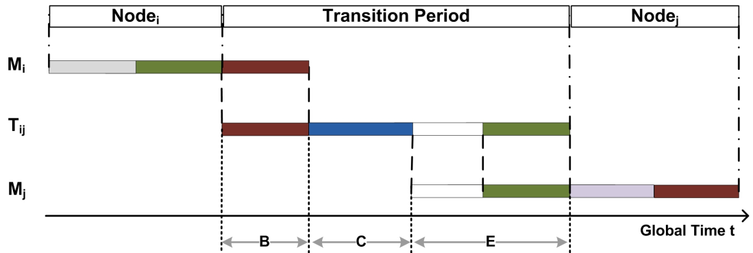
Figure 4.10: A transition period on the edge that connects N_i and N_j .
