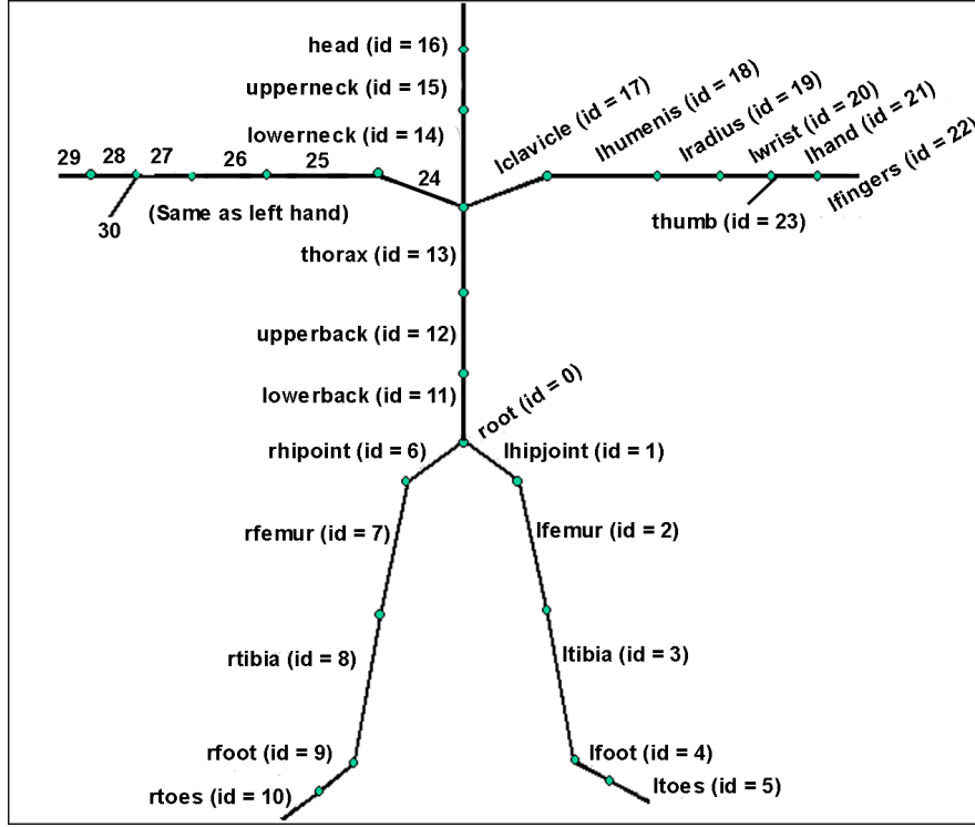
Figure 4.8: Our skeletal model.
