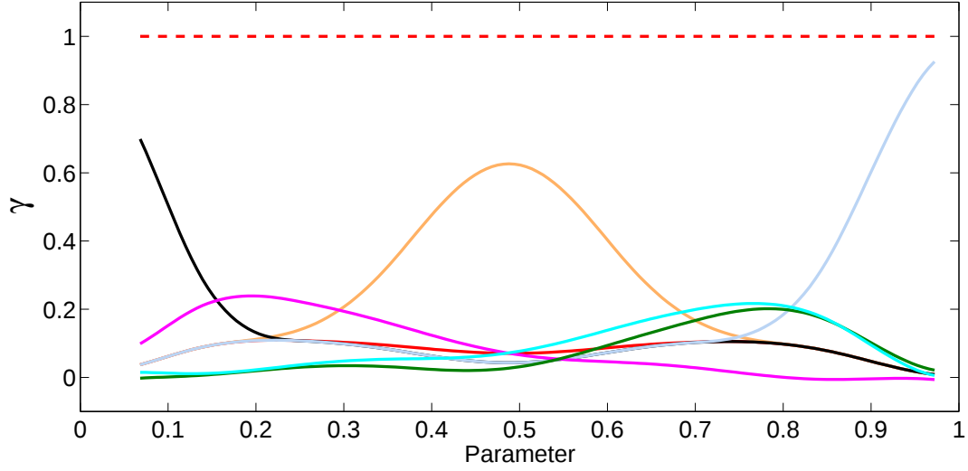
Figure 5.5: The weight values for incremental time update ( \gamma ) vs. normalized angular velocities. The solid lines represent the weights for example motions and the dotted line shows the overall sum.
