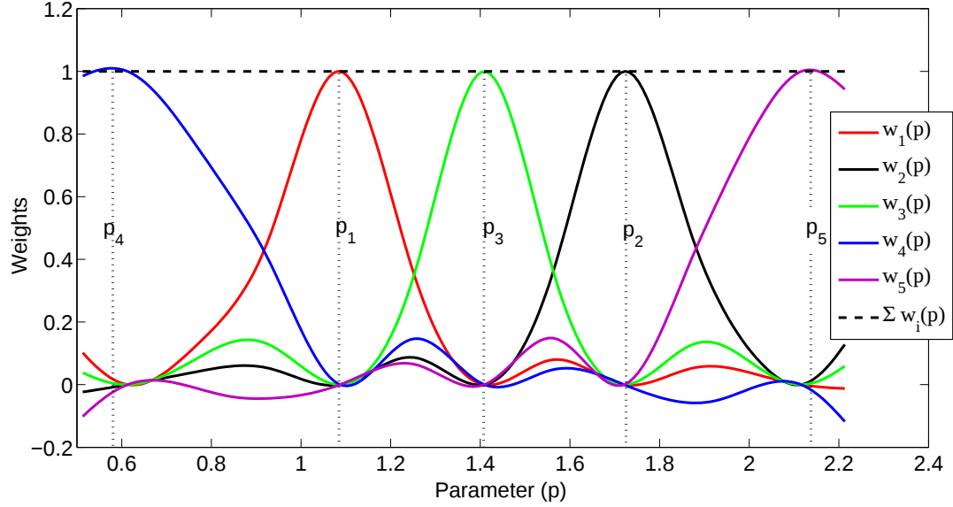
Figure 4.3: The weight values according to the user-specified parameters.
