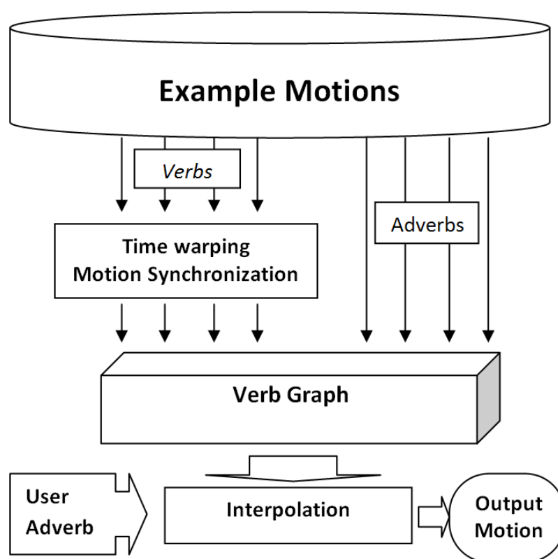
Figure 3.1: The overview of the system described in [27].
