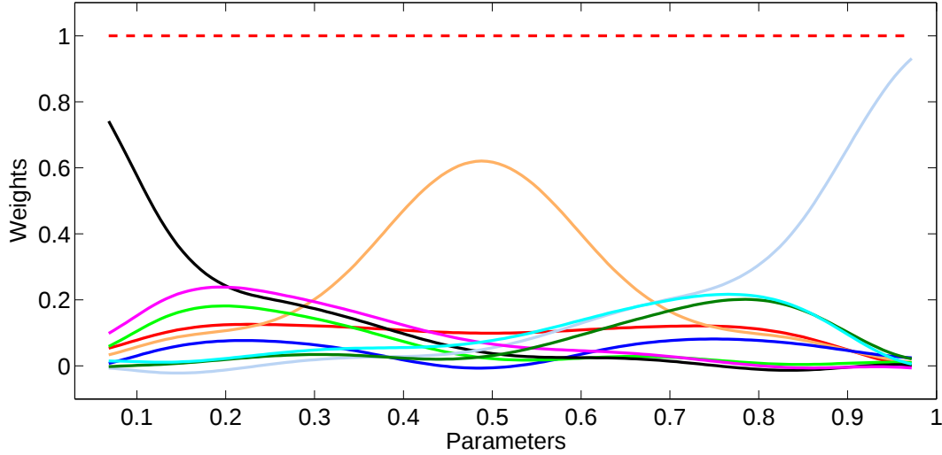
Figure 5.4: The weight values ( w ) vs. the normalized angular velocities. The solid lines represent the weights for example motions and the dotted line shows the overall sum.
