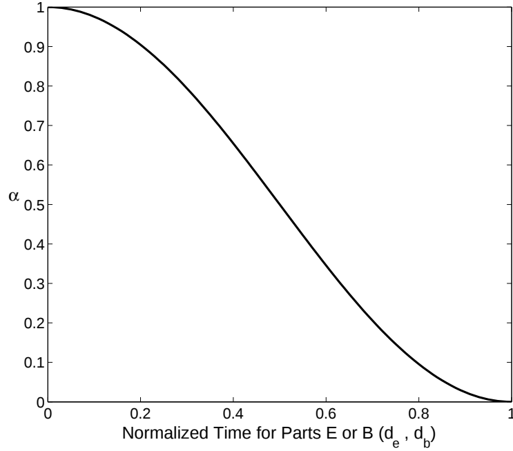
Figure 4.11: The \alpha values for normalized time values of part B and part E : d_b and d_e , respectively, where d_b = \frac{t-b_{start}}{b_{end}-b_{start}} or d_e = \frac{t-e_{end}}{e_{end}-e_{start}} .
