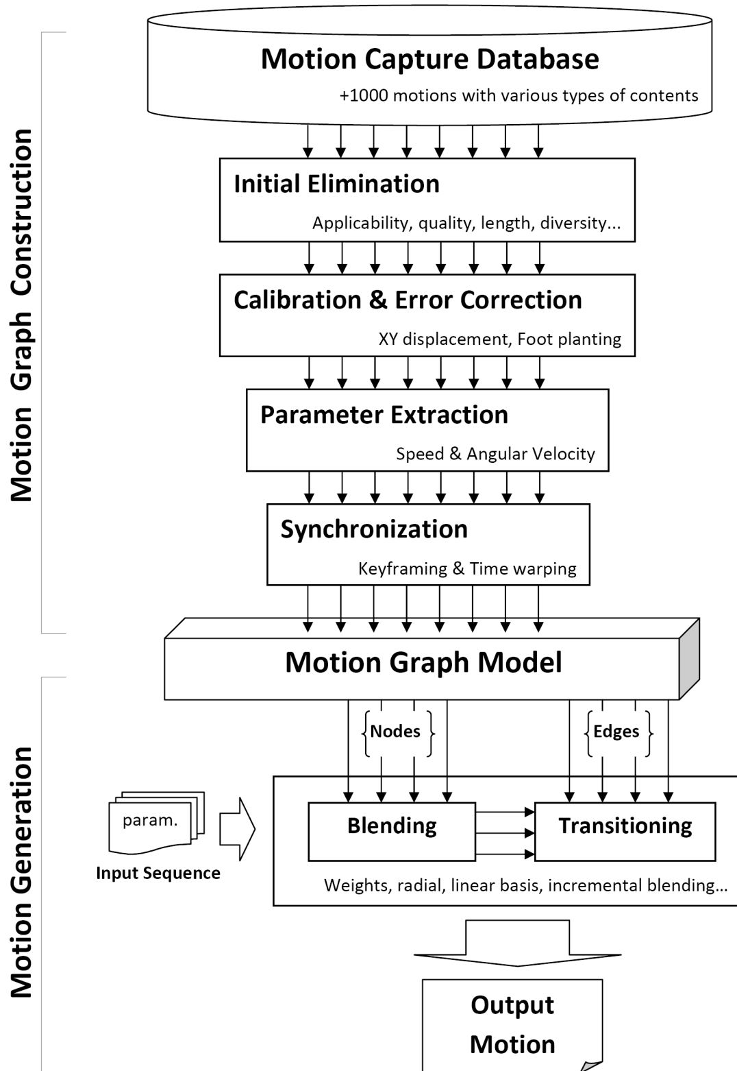
Figure 4.1: The overview of the real-time locomotion generating system.
