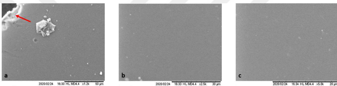
Figure 5.11. SEM images of C2 film at different magnifications a: 1.2 K X (The red arrow shows the edge of the film), b: 2.5 K X, c: 5.0 K X
