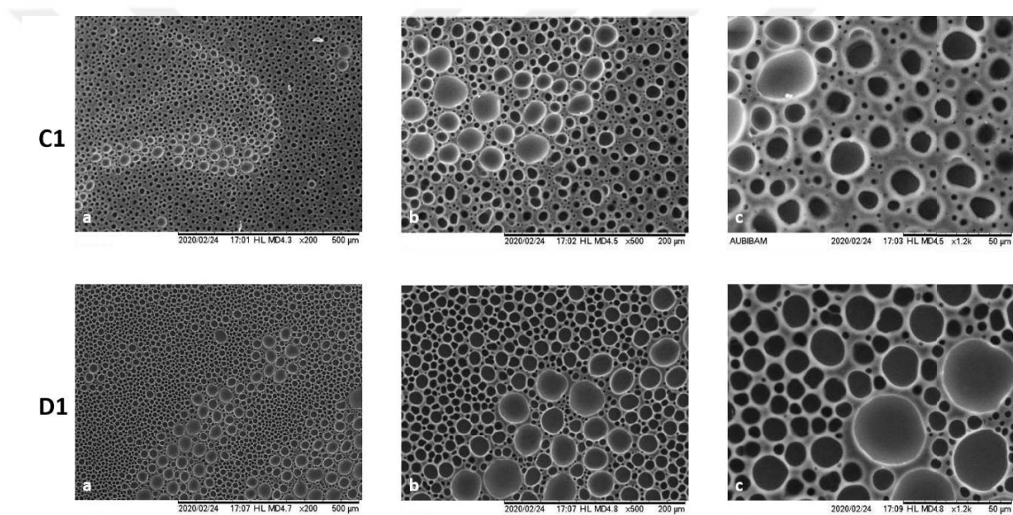
Figure 5.9. SEM images of excluded C1 and D1 films at different magnifications as an indicator of film roughness/smoothness, a: 200 X, b: 500 X, c: 1.2 K X
