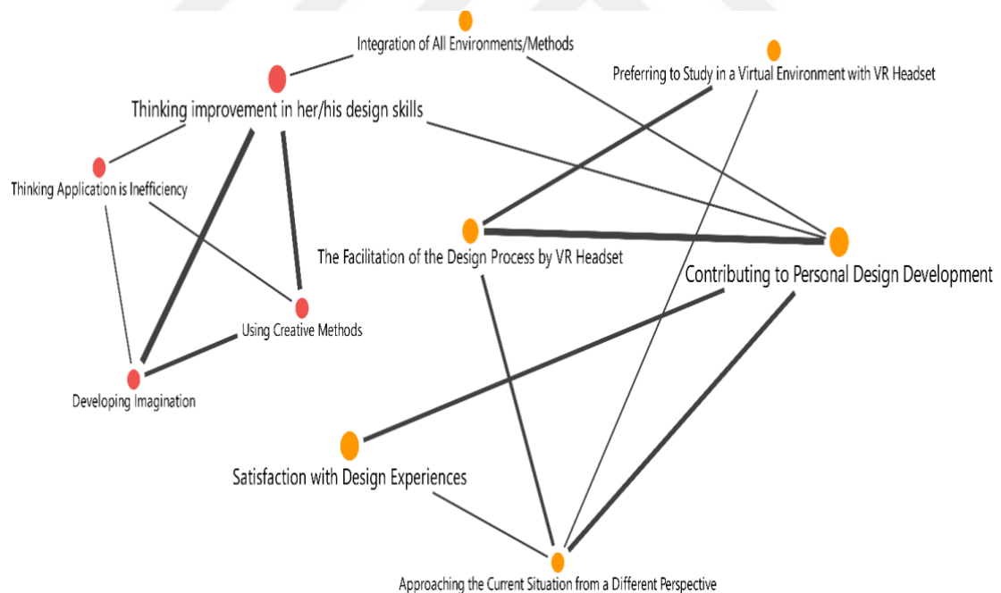
Figure 4.29 Code Map.
