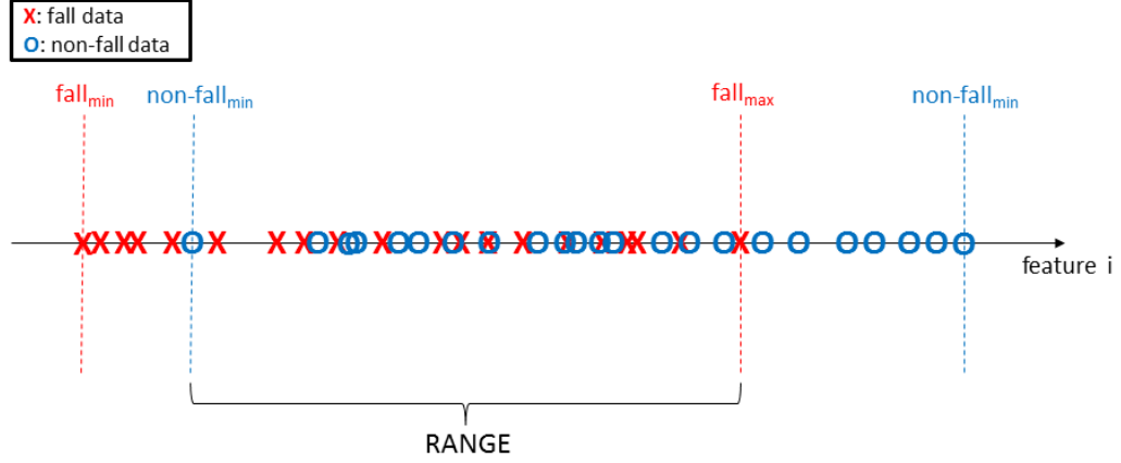
Figure 3.1: A Typical Distribution of a Feature of Non-fall and Fall Data.
