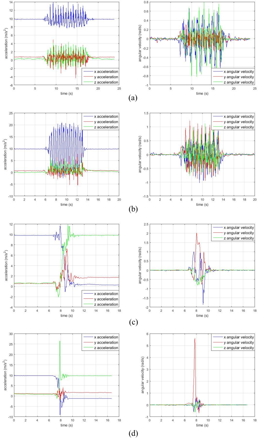
Figure 2.1: Acceleration and angular velocity signals of a) walking (non-fall), b) running (non-fall), c) standing to lying on bed (non-fall), and d) forward fall.
