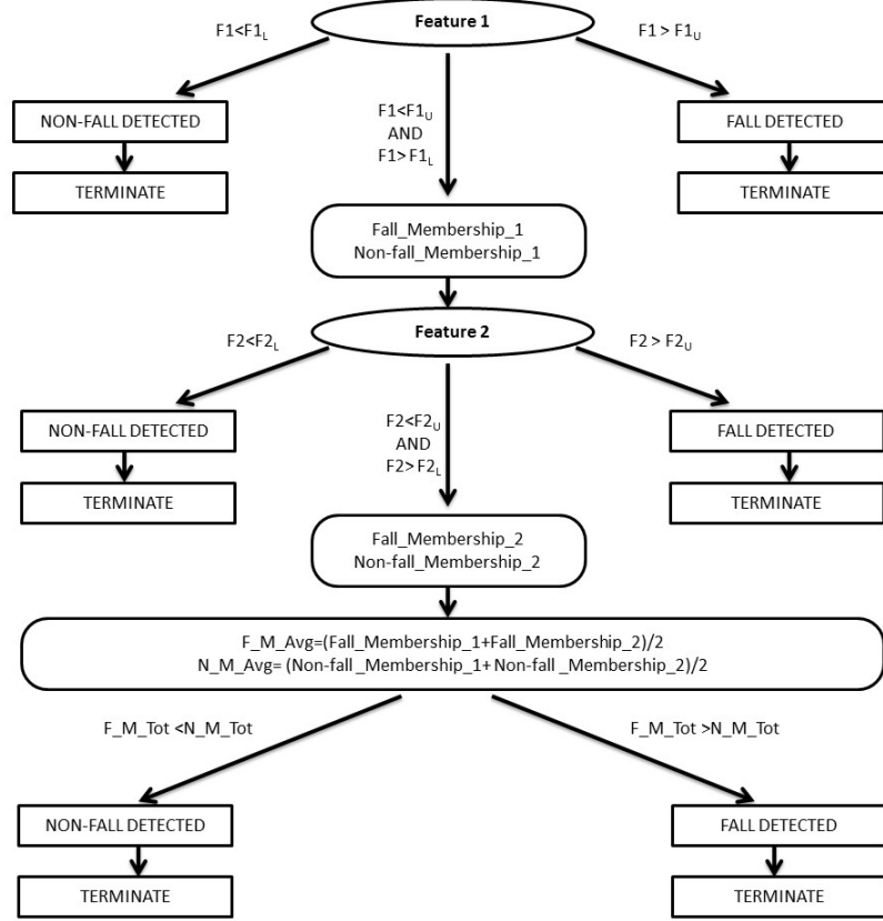
Figure 2.3: Heuristic Fall-Detection Algorithm.
