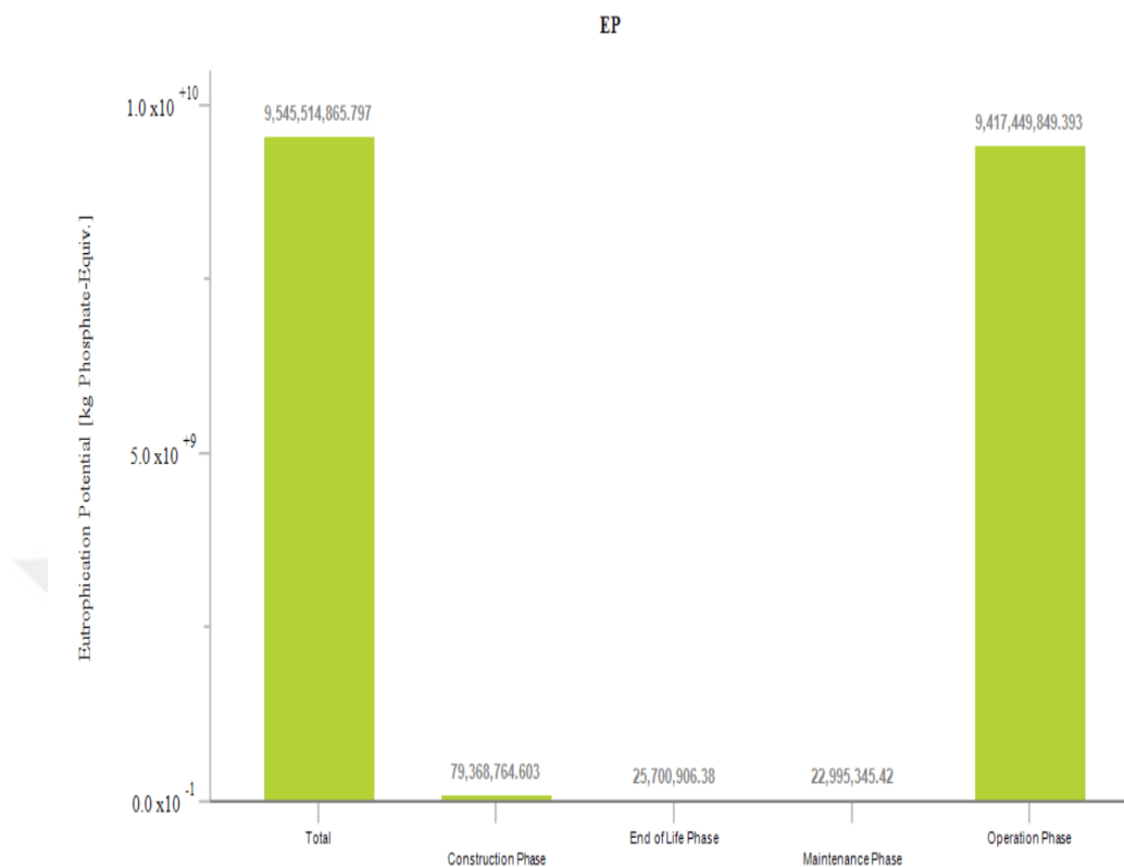
Figure 5.19. Eutrophication Potential of Alternative Case
