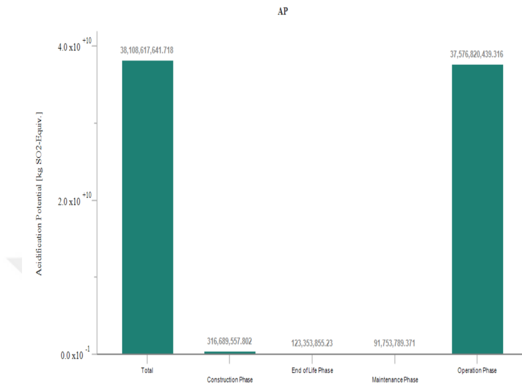
Figure 5.11. Acidification Potential of Base Case
