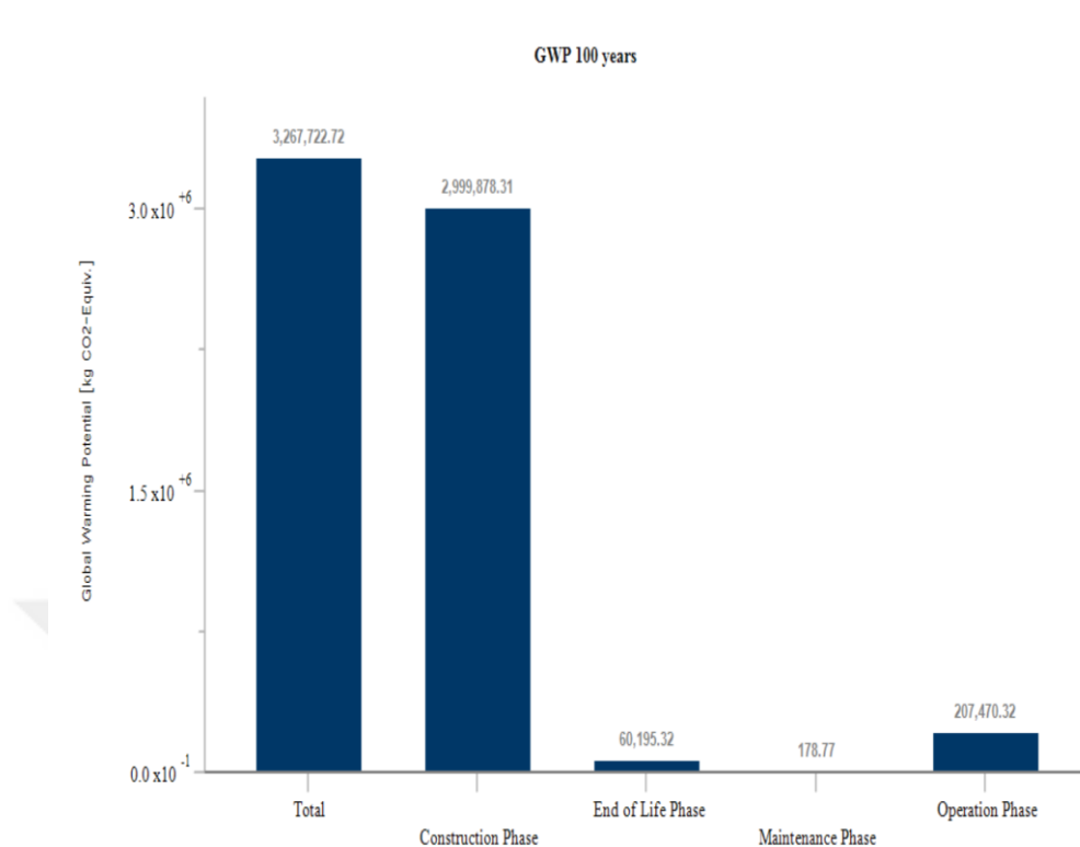
Figure 6.14. Global Warming Potential of Alternative Case
