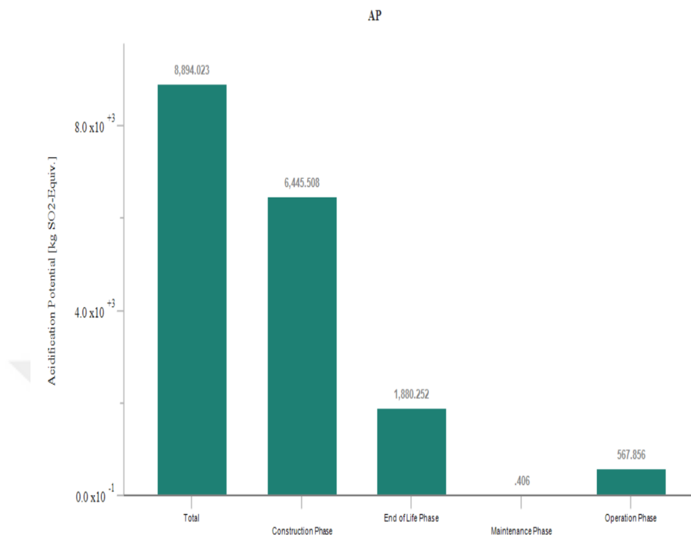
Figure 6.10. Acidification Potential of Base Case
