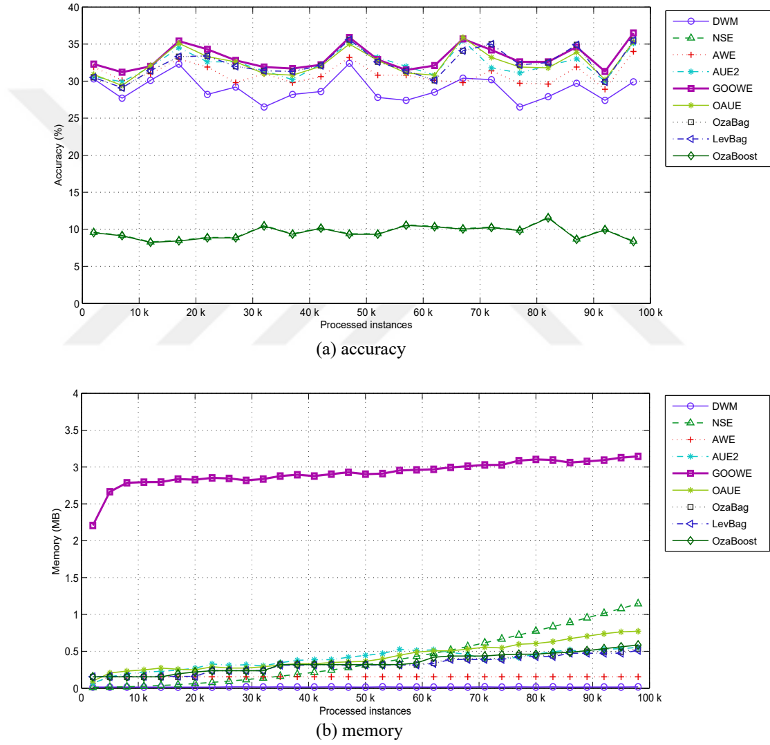
Figure 4.3: LCD example with reoccurring data stream: Classification accuracy and memory consumption for TREE-F dataset.
