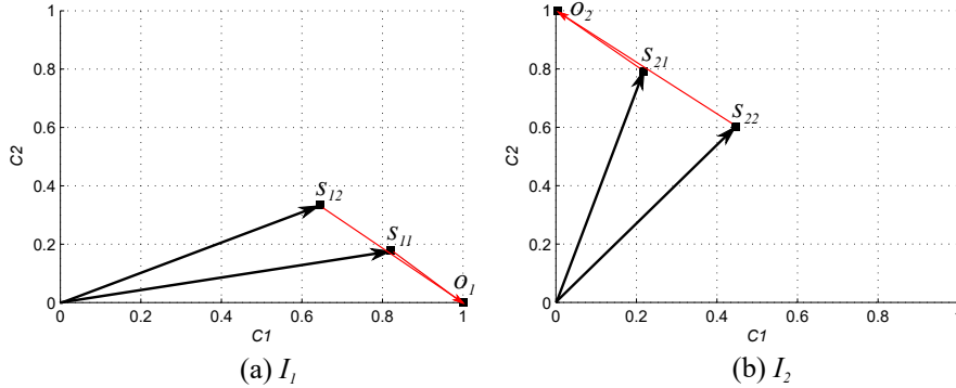
Figure 3.4: Score vectors for window instances of example.
