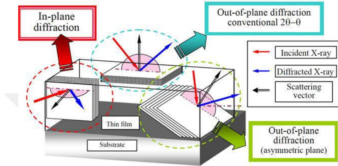
Figure 1.4. Orientation of crystallographic planes in a thin film sample [17]
