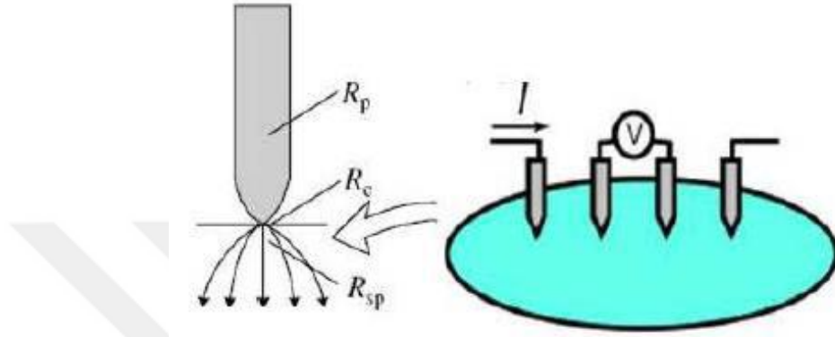
Figure 1.6. Schematic illustration of FPP technique [18]
