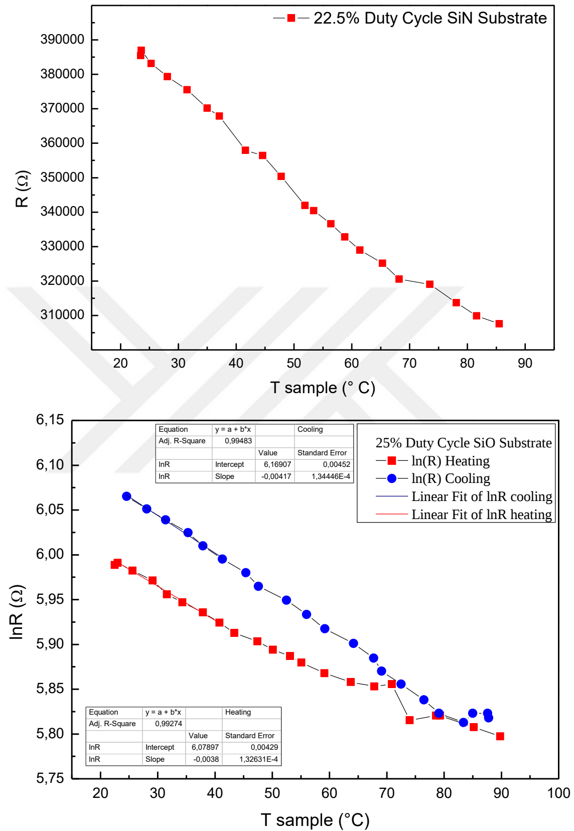
Figure 3.10. (Continued) Change in \ln R and R with respect to temperature for different samples deposited using duty cycle values
