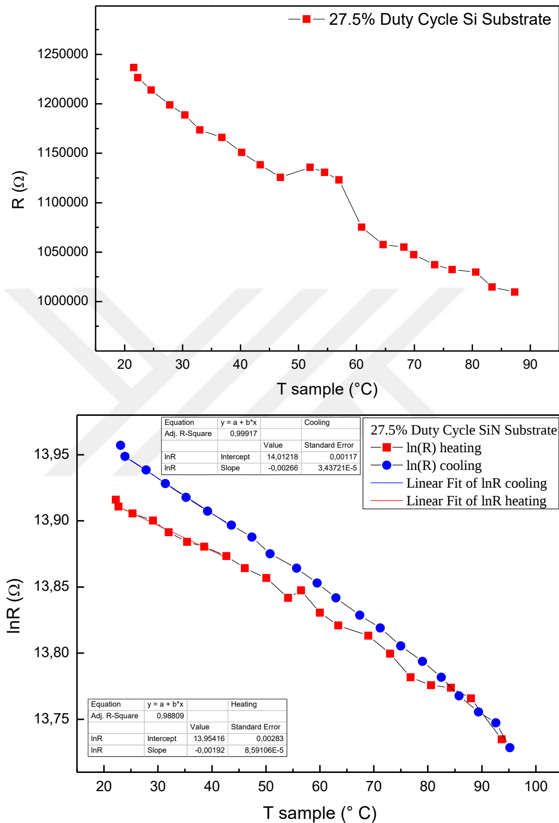
Figure 3.10. (Continued) Change in \ln R and R with respect to temperature for different samples deposited using duty cycle values
