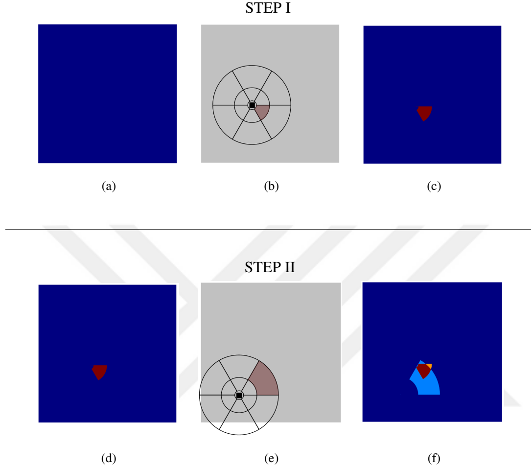
Figure A.1: (a) \mathbf{O} is initialized with zeros. (b) We pick an arbitrary location (i, j) and the 3rd channel of \mathbf{E} . We place the vote field centered at the location (i, j) . Since, we are using the 3rd channel, the relevant region of the vote field is 3 (shown with pink color on \mathbf{E} ). Finally we apply the voting. (c) \mathbf{O} after voting. (d) \mathbf{O} before the voting. (e) To further illustrate the voting process, we pick another location and the 8th channel in \mathbf{E} . We place the vote field centered at the location. The region 8 marks the target area to be voted on. We apply the voting. (f) \mathbf{O} after voting. The colors in \mathbf{O} indicate accumulated vote strength.
