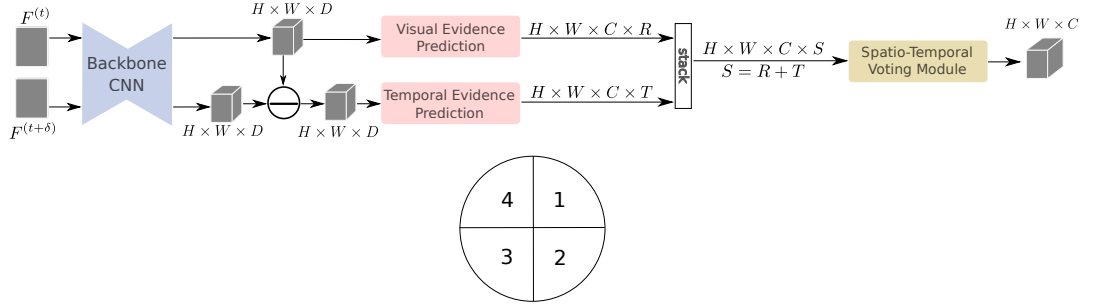
Figure 3.4: (Top) Overall processing pipeline of HoughNet for video object detection. (Bottom) Temporal vote field. Image is taken from our ECCV’20 paper extension [3].
