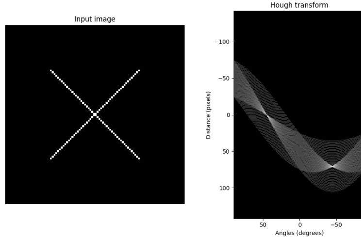
Figure 2.2: An example result of a Hough transform on a raster image containing two lines. Image source: https://scikit-image.org/docs/0.11.x/auto_examples/plot_line_hough_transform.html
