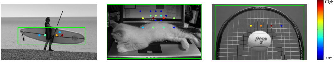
Figure 5.1: Three sample detections by PPDet, from left to right: surfboard, laptop and racket. The colored dots show the locations whose predictions are pooled to generate the final detection shown in the green bounding box. The color denotes the contribution weight. Highest contributions are coming from the objects and not occluders or background areas. Images are from COCO val2017 set. Image is taken from our BMVC’20 paper [24].
