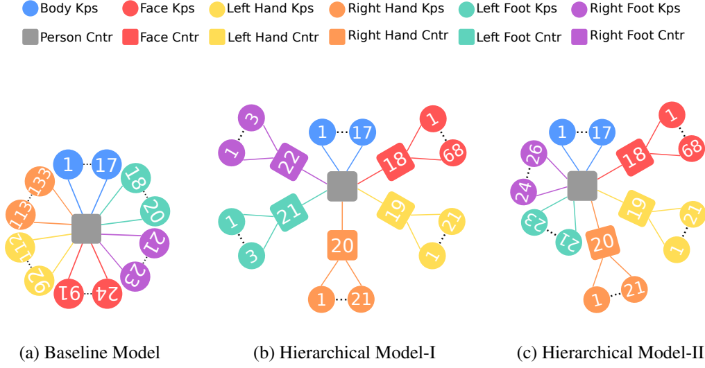
Figure 6.4: Hierarchical representations of whole-body keypoints. (a) Each of 133 whole-body keypoints is defined with an offset to the person box center. (b) Body keypoints and other part centers (i.e. foot, face and hand) are defined with offsets to the person box center. Foot, face and hand keypoints are defined with offsets according to their corresponding part centers. (c) Considering the sparsity of foot keypoint annotations, we define them with their offset values to the person box center. In both Hierarchical Model-I and Hierarchical Model-II, body keypoints are defined with offset values to the person box center. Each face and hand keypoint is defined with an offset to face and hand bounding box centers, respectively. Image is taken from our IMAVIS journal paper [25].
