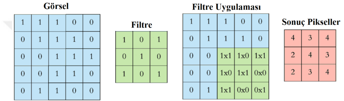
Şekil 3.17. 5 \times 5 görselin 3 \times 3 boyutunda filtrelenmesi ( https://www.freecodecamp.org/news/an-intuitive-guide-to-convolutional-neural-networks-260c2de0a050/ )
