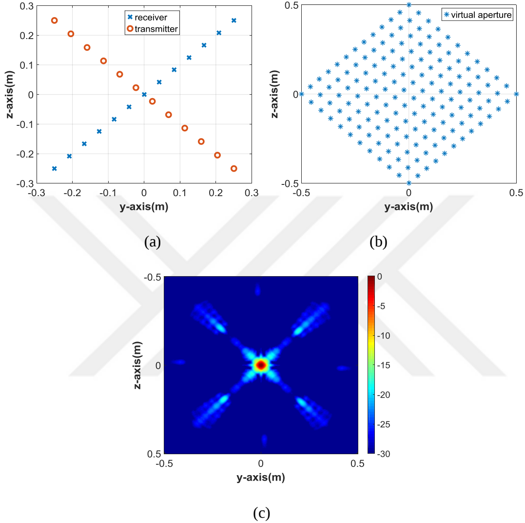
Figure 3.2 (a) Mills Cross array with 13 receivers and 12 transmitters (b) virtual aperture comprised of 156 elements (c) PSF
