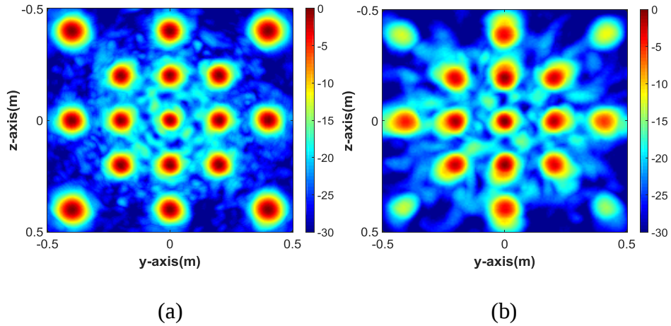
Figure 4.4 Comparison of images obtained for 17 targets located at x=0.5\text{m} (a) simple model (b) rigorous model
