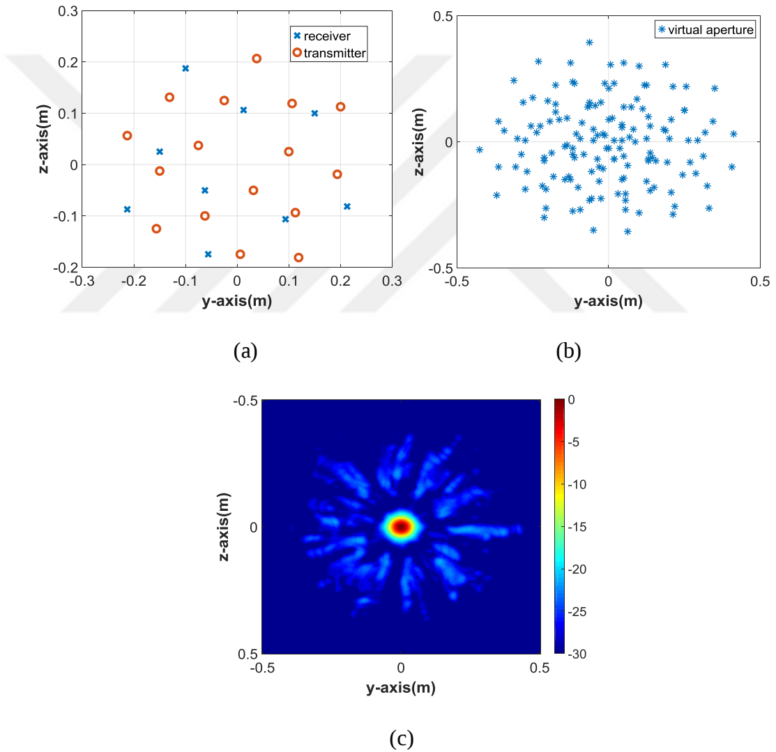
Figure 3.3 (a) Spiral array with 16 receivers and 9 transmitters (b) virtual aperture comprised of 144 elements (c) PSF
