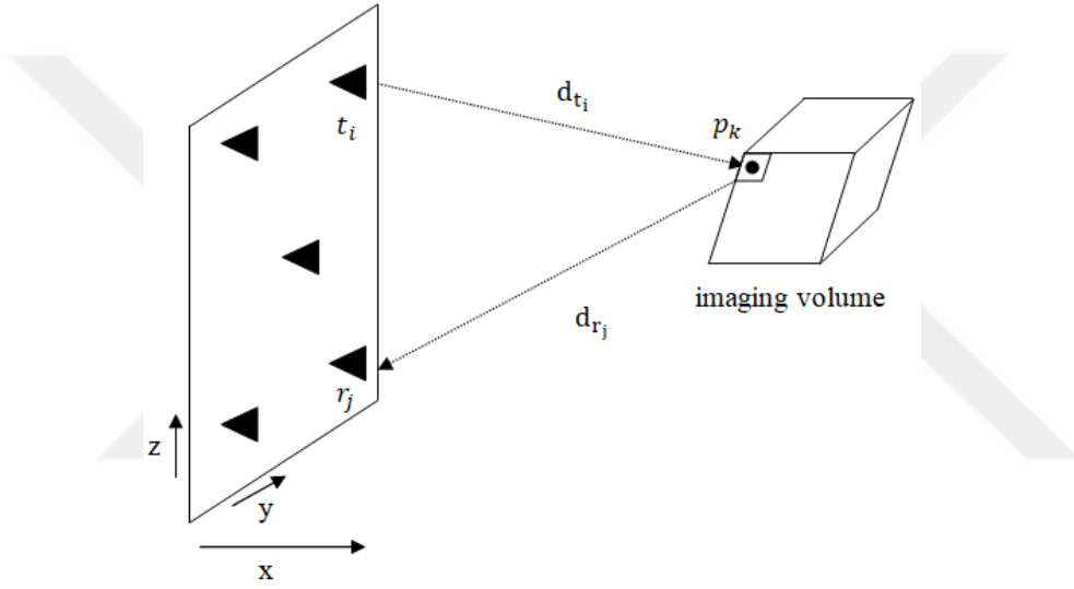
Figure 5.1 Illustration of signal path
