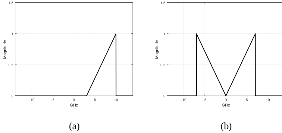
Figure 2.5 Frequency domain signal definition using method II (a) measured signal (b) shifting to baseband and generation of complex conjugate in the negative side
