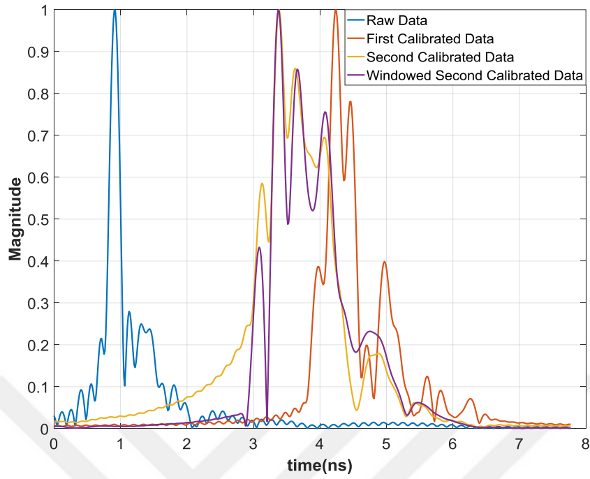
Figure 4.15 Received time domain signals obtained by active antenna pair for rigorous model
