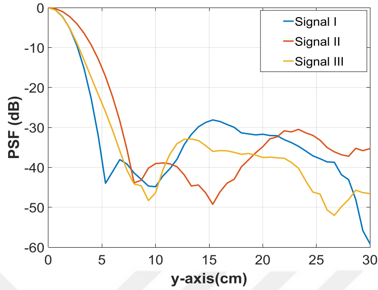
Figure 3.8 Point spread functions for different signal types for z=0
