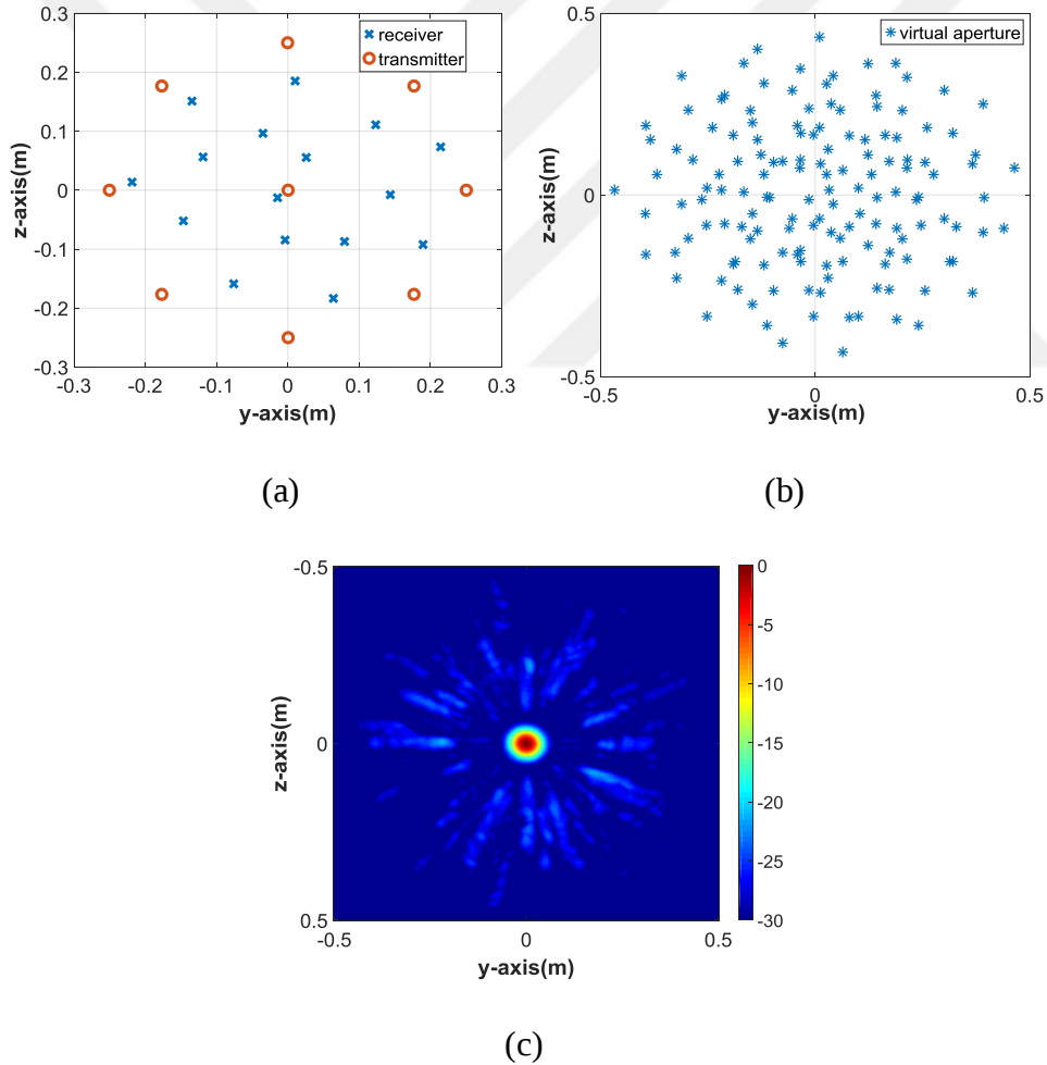
Figure 3.4 (a) Curvilinear array with 16 receivers and 9 transmitters (b) virtual aperture comprised of 144 elements (c) PSF
