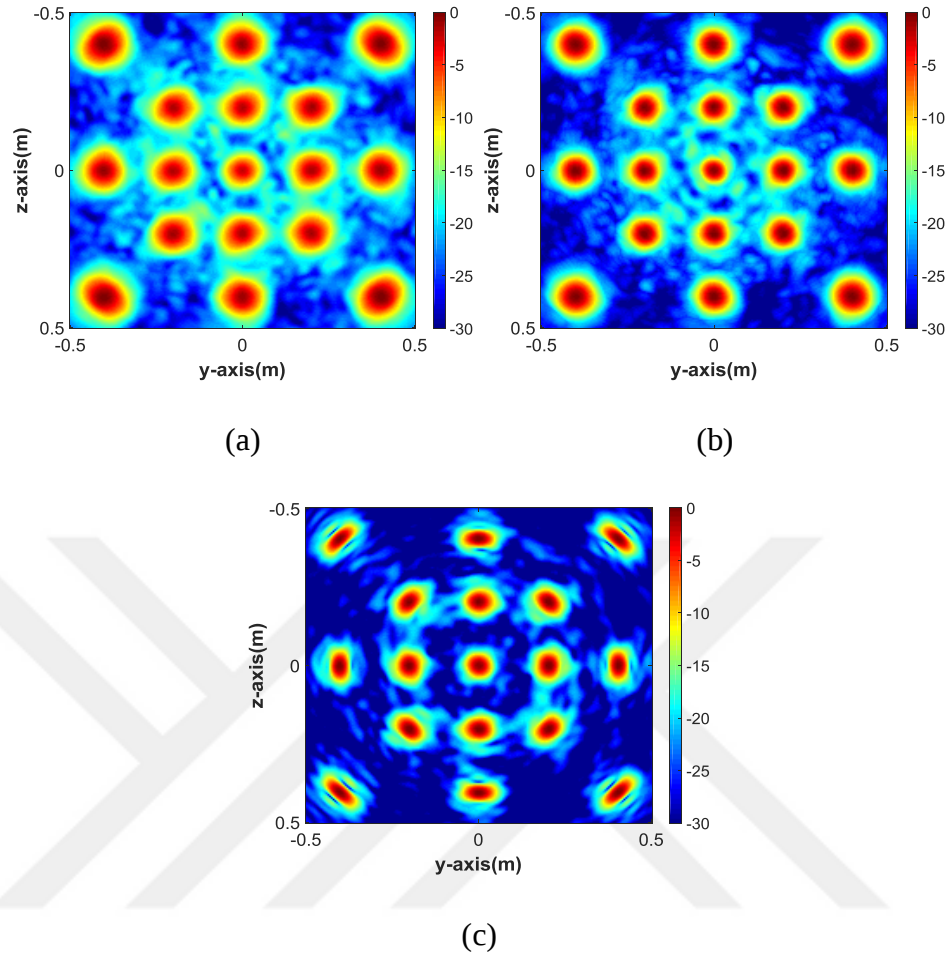
Figure 4.2 Simple model point spread function with 17 targets located at x=0.5\text{m} (a) summation representation (b) maximum representation (c) normal representation
