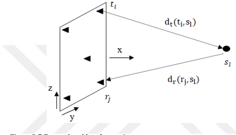
Figure 2.7 Forward problem for a point scatterer
