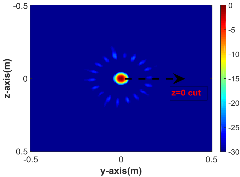
Figure 3.7 Point spread function obtained by the data generated through simple model utilizing signal I
