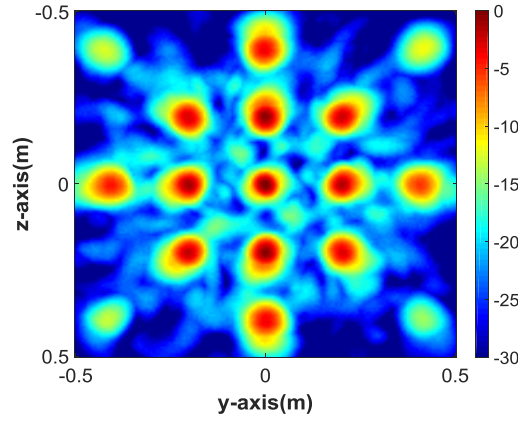
Figure 1.2 Point spread function obtained by data from CST simulation software
