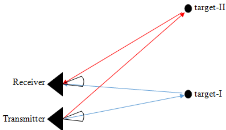
Figure 4.5 Demonstration of different targets affected by radiation pattern
