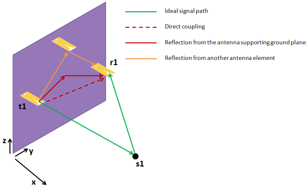
Figure 2.8 Demonstration of rigorous model simulation environment
