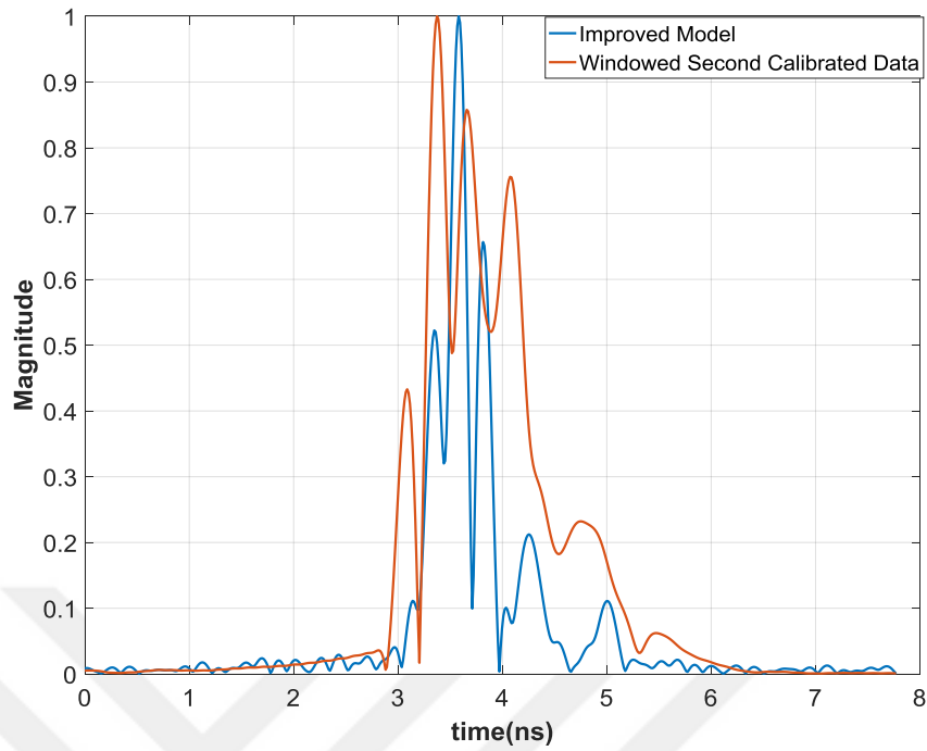
Figure 4.16 Comparison of received time domain signals for improved and rigorous model
