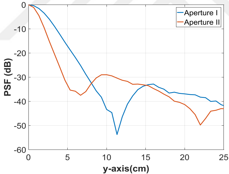
Figure 3.9 Point spread functions for different aperture types at z=0
