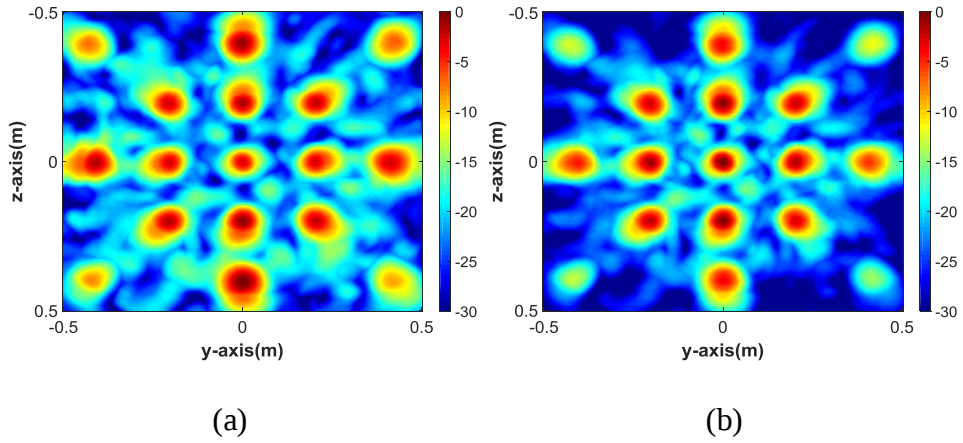
Figure 5.3 Maximum representation of images obtained by two different frequency domain back projection algorithm (a) modified back projection (b) traditional back projection
