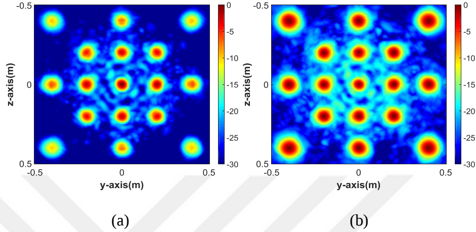
Figure 4.10 Point spread functions by using maximum representation with 17 targets located at x=0.5\text{m} (a) improved model (b) simple model
