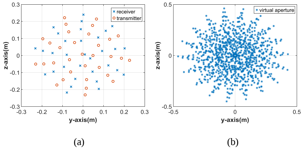
Figure 3.6 Spiral array with 32 transmitters and 32 receivers (a) antenna configuration (b) virtual aperture comprised of 1024 elements
