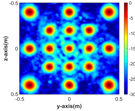
Figure 1.3 Point spread function obtained by data generated through simple model
