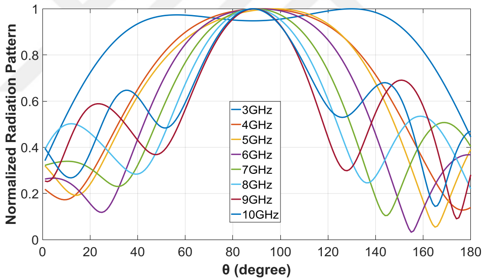
Figure 4.8 Vivaldi antenna H-plane radiation pattern at \phi=0^\circ
