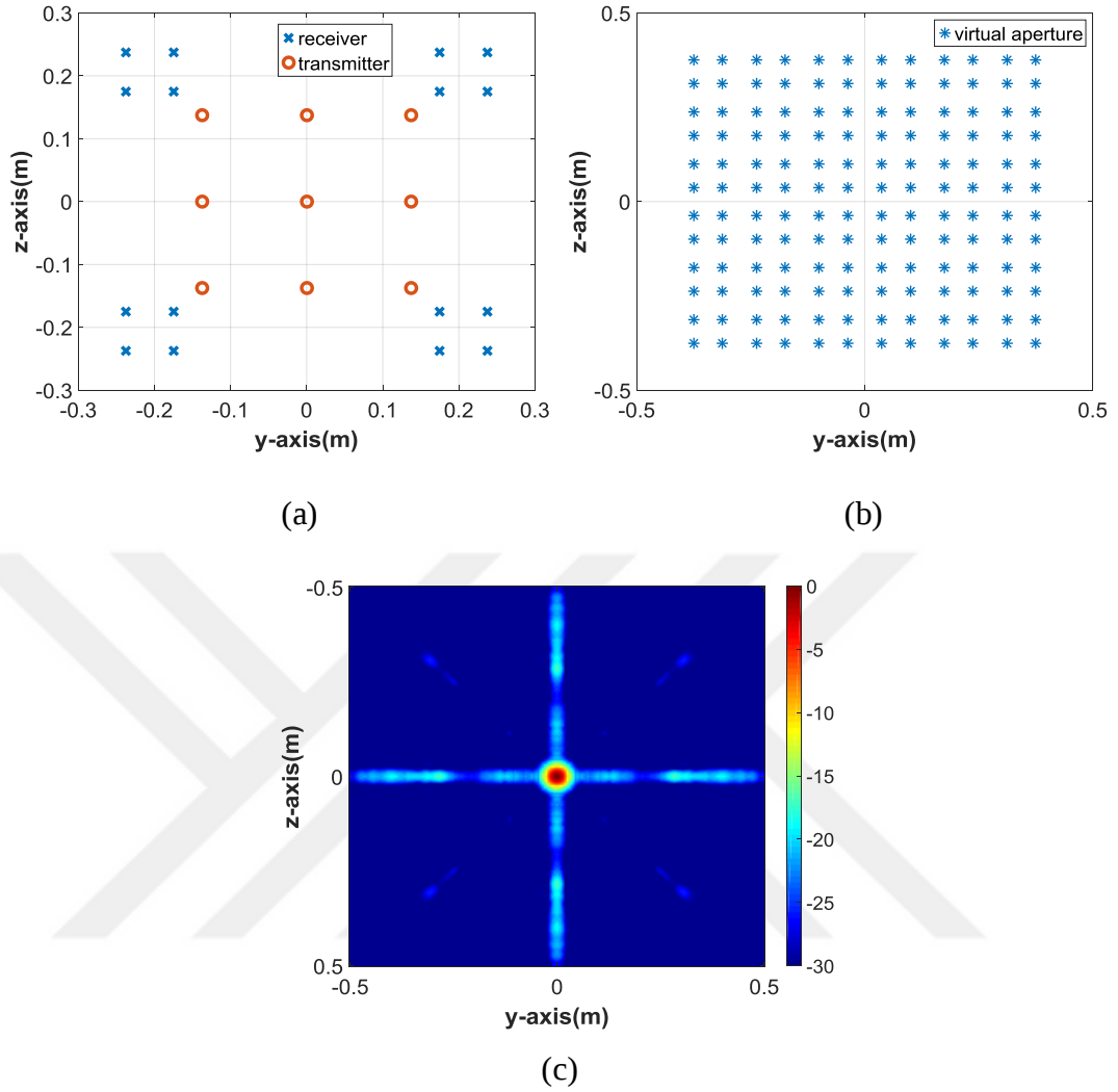
Figure 3.1 (a) Rectangular array with 16 receivers and 9 transmitters (b) virtual aperture comprised of 144 elements (c) PSF
