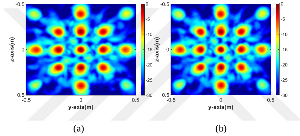
Figure 5.2 Maximum representation of images obtained by back projection algorithm (a) frequency domain (b) time domain
