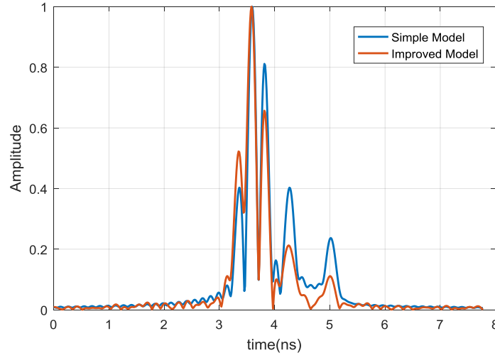
Figure 4.13 Received time domain signal obtained by active antenna pair for simple and improved model
