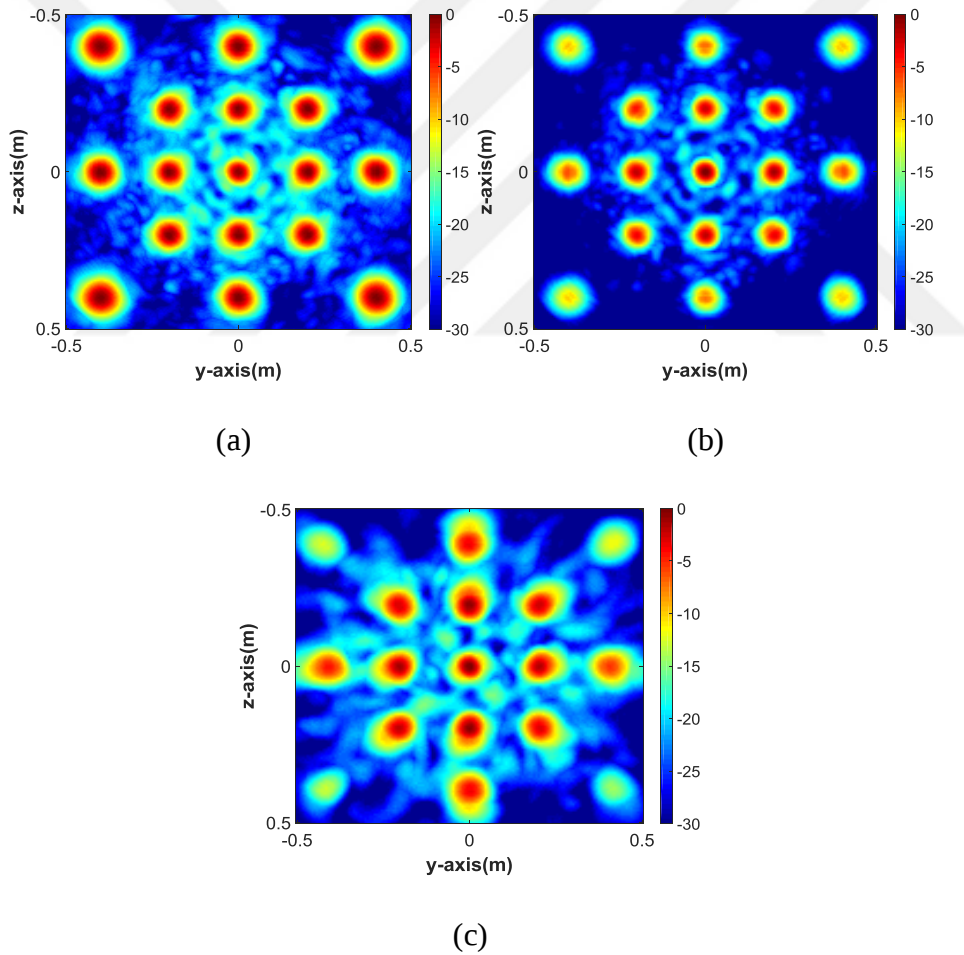
Figure 4.14 Comparison of images obtained for 17 targets located at x=0.5\text{m} by three different models (a) simple model (b) improved model (c) rigorous model
