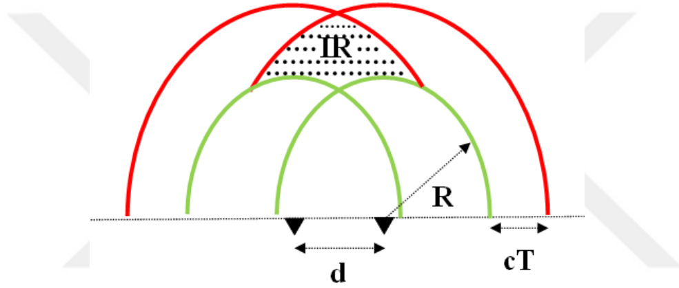
Figure 1.1 Demonstration of IR region
