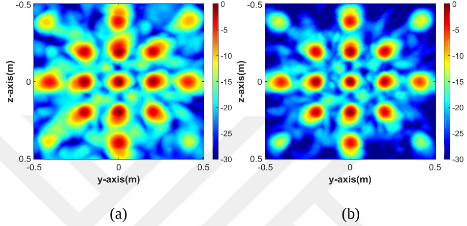
Figure 4.3 Rigorous model point spread functions obtained by using maximum representation with 17 targets located at x=0.5\text{m} (a) without Hamming window (b) with Hamming window
