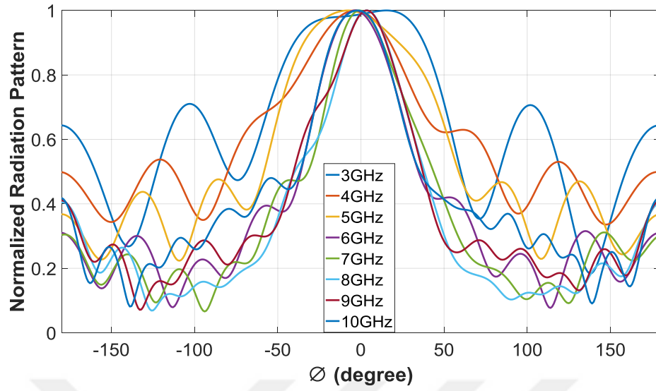
Figure 4.7 Vivaldi antenna E-plane radiation pattern at \theta=90^\circ
