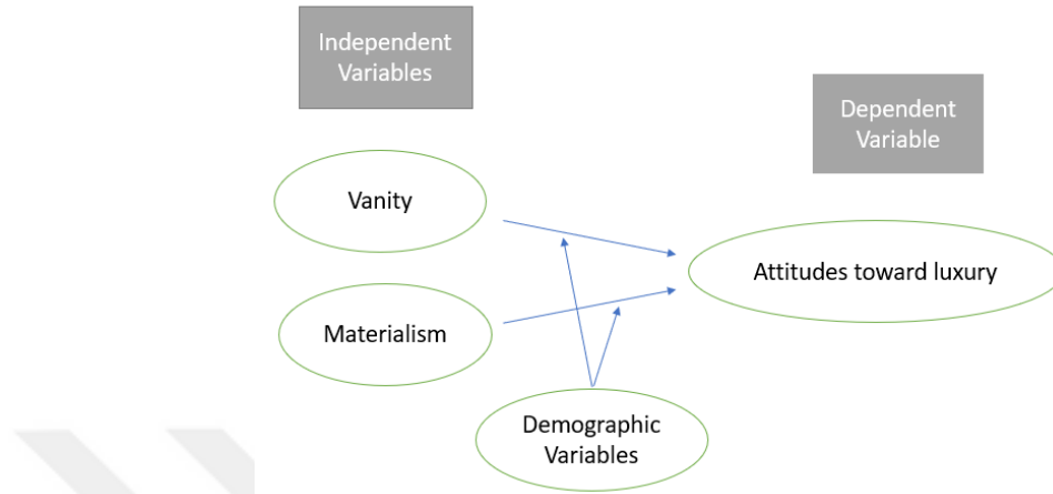
Figure 3. 1. Research model
