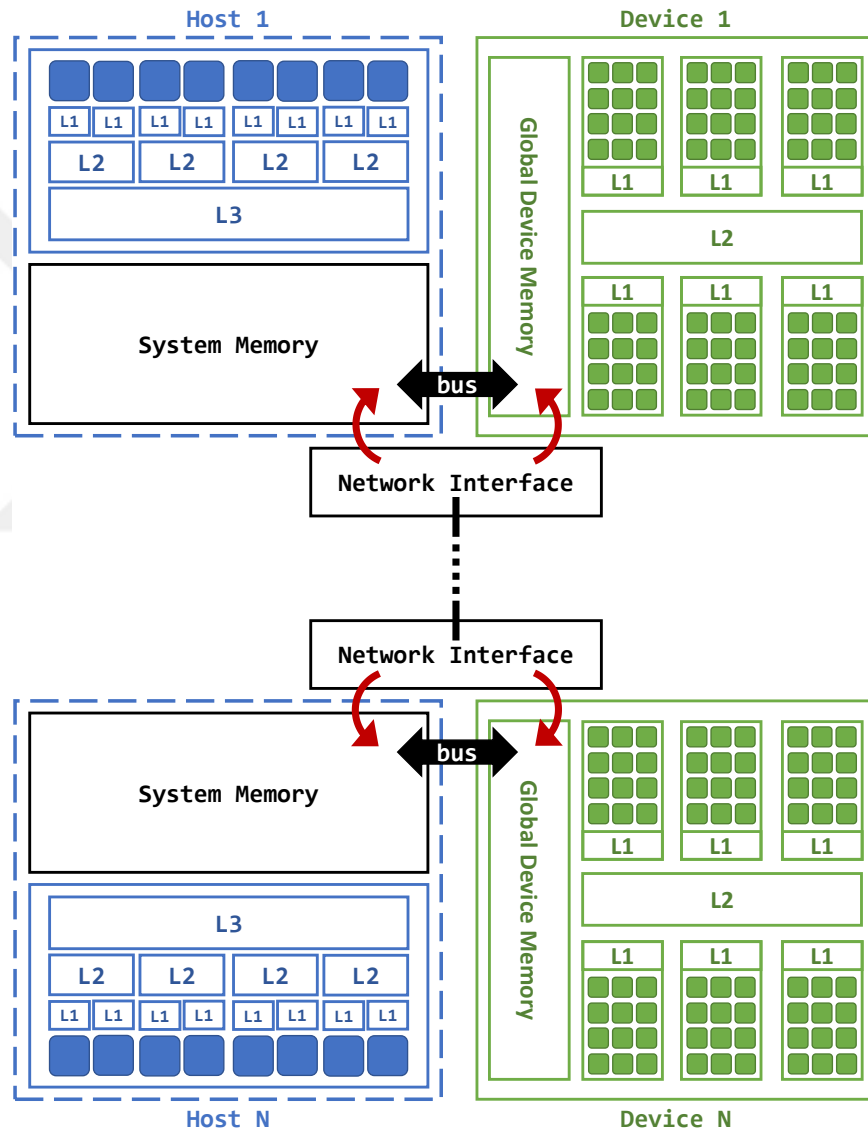
Figure 3.6: GPUDirect RDMA and a compatible network interface allow direct communication from/to GPU memory.
