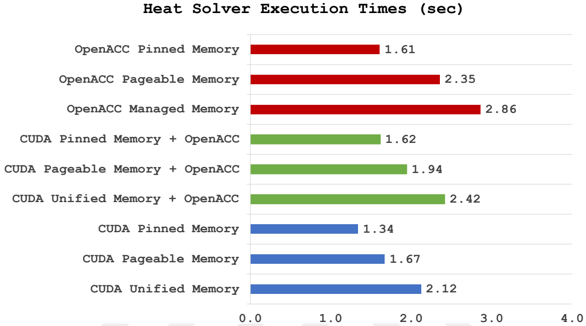
Figure 3.4: Performance of different execution model implementations of heat solver. CUDA + OpenACC indicates implementations that rely on CUDA for memory management and OpenACC for kernel code generation.
