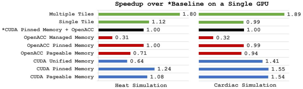
Figure 6.1: Performance comparison of various implementations of Heat and Cardiac . Single and multiple tile versions are based on our programming model.
