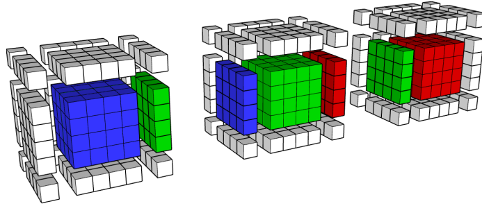
Figure 5.1: Ghost cells from a tile form a ghost zone.
