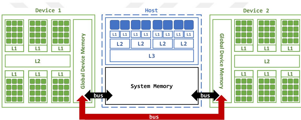
Figure 3.5: GPUDirect P2P Transfer and an interconnect between GPUs allow direct memory transfers between GPUs.
