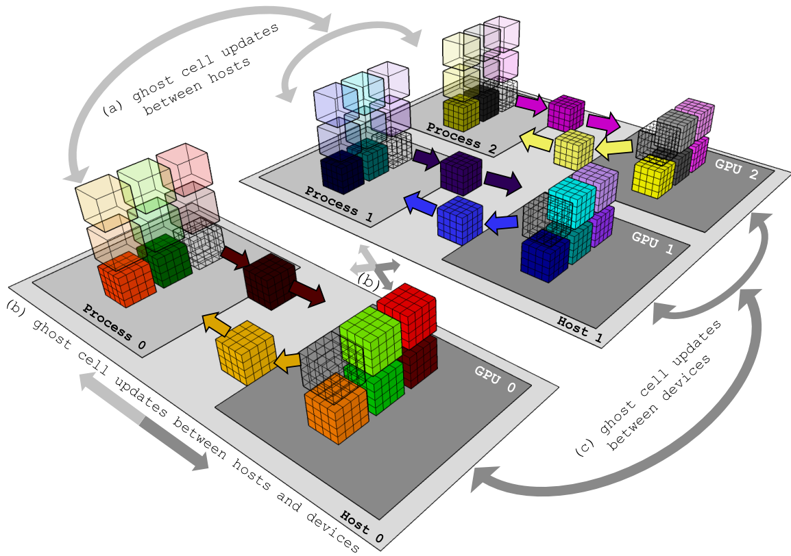
Figure 4.2: Both CPUs and GPUs participate in computing tiles while some tiles are asynchronously being transferred between them.
