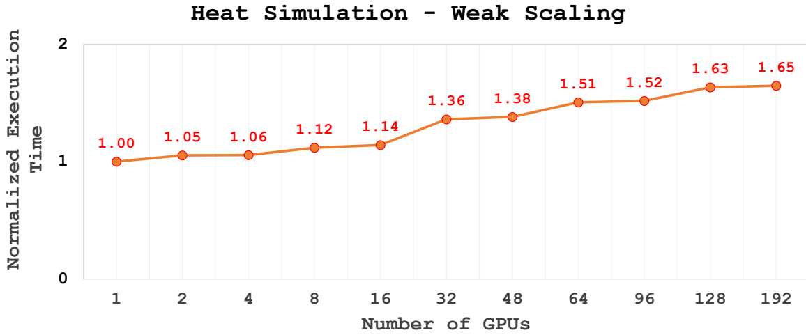
Figure 6.4: Weak scaling study for Heat Simulation
