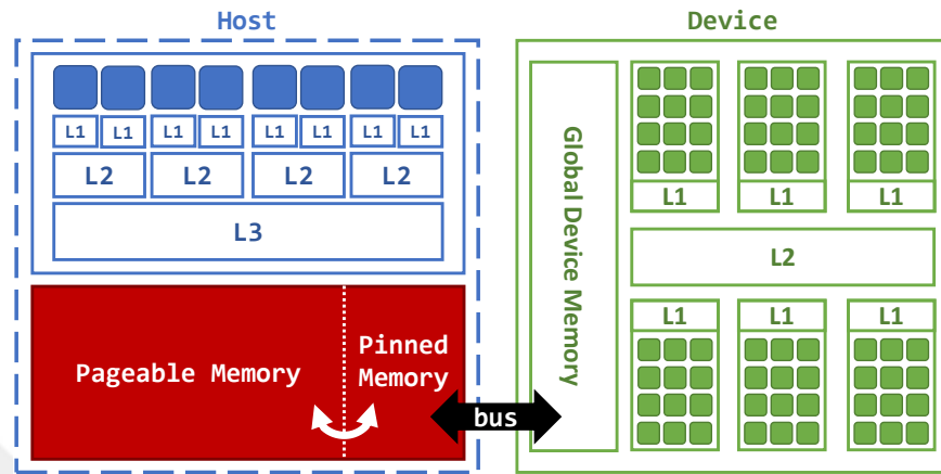
Figure 3.2: In a memory transfer between host and device CUDA implicitly copies from pageable memory to pinned memory or vice versa.
