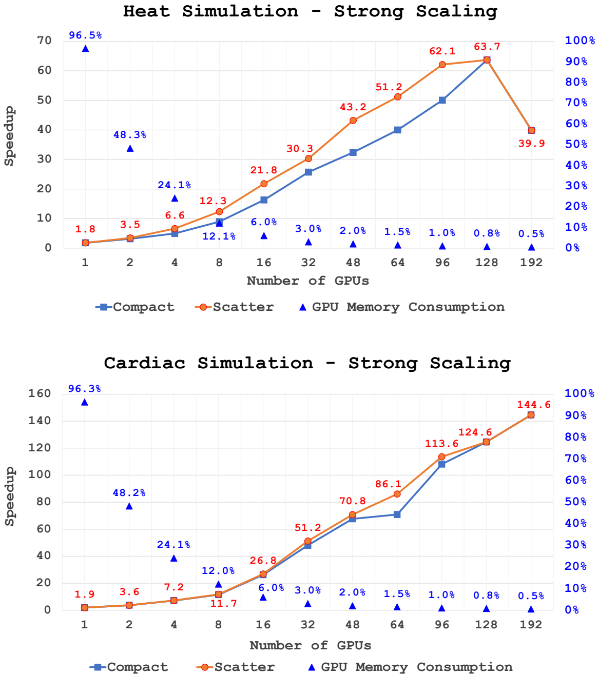
Figure 6.3: Strong scaling studies for Heat and Cardiac simulations.
