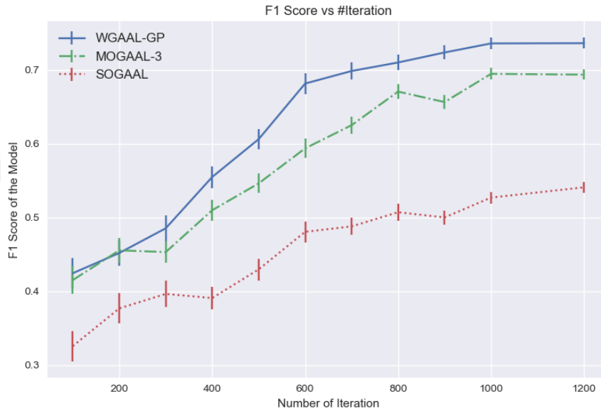
Figure 5.4: F1 scores for GAAL algorithms according to number of training samples
