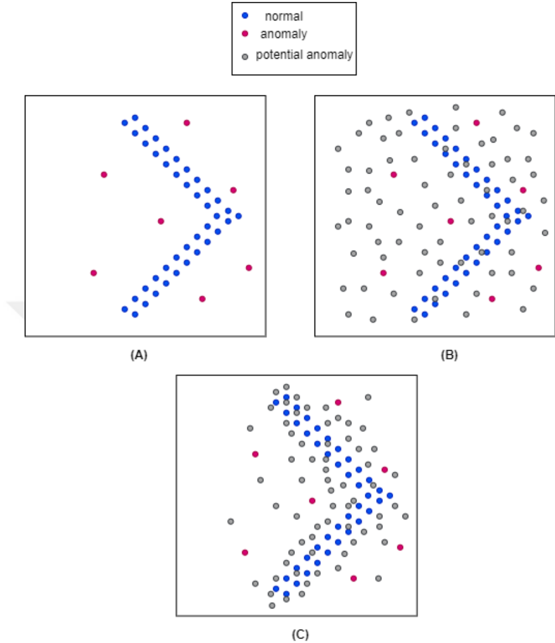
Figure 4.1: A illustrates real data, B illustrates AGPO based generated potential anomaly points, C illustrates GAAL based generated potential anomaly points
