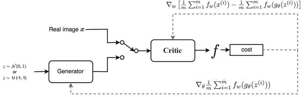
Figure 2.2: WGAN's Structure [35]
