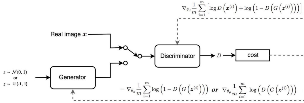
Figure 2.1: GAN's Structure [35]
