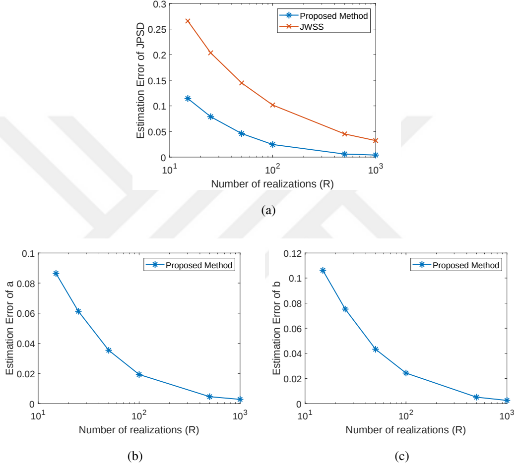
Figure 4.3: (a) JPSD error vs. the number of realizations, (b) Estimation error of a vs. the number of realizations, (c) Estimation error of b vs. the number of realizations
