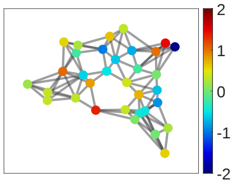
(f) The graph signal at time t = 30
