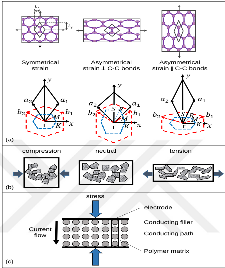
Figure 1. (a) Symmetrical strain distribution, asymmetrical strain distribution perpendicular to C-C bonds, and asymmetrical strain distribution parallel to C-C bonds [57]. (b) Schematic illustration of piezoresistivity of graphene sheets [58]. (c) Schematic illustration of the tunnelling model [59].
