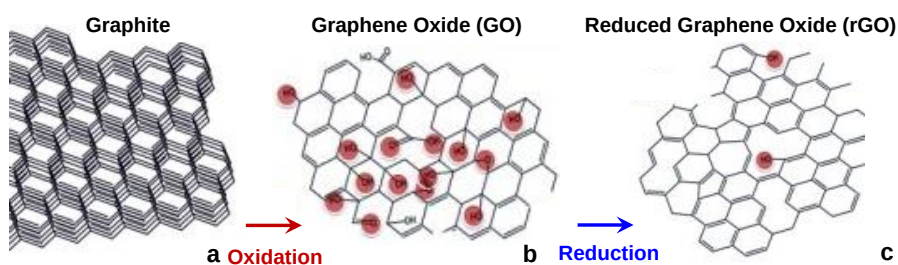
Figure 6. (a, b, c) The schematic diagram of reducing graphene oxide to develop reduced graphene oxide.
