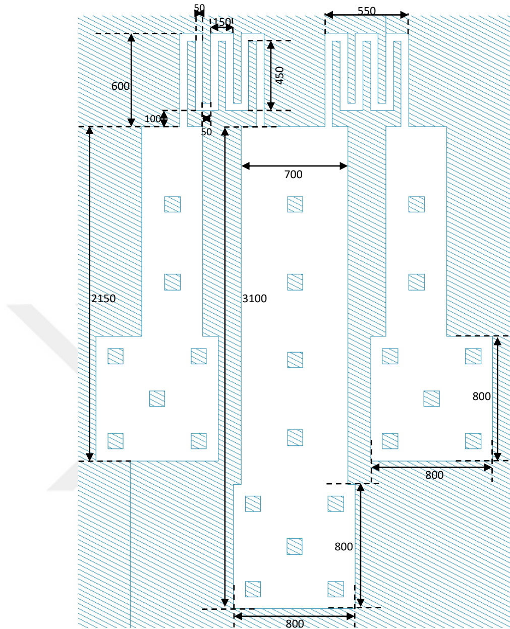
Figure 25. Design of the microcantilever sensor defining the dimensions of the strain gauge shown in the schematic
