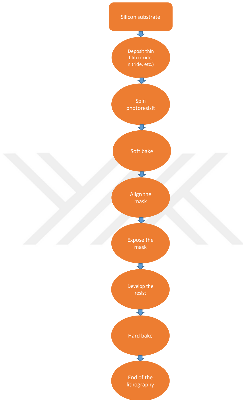
Figure 22. Process flow of lithography
