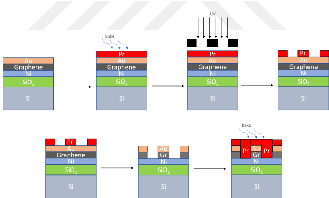
Figure 27. Overall fabrication process flow.
