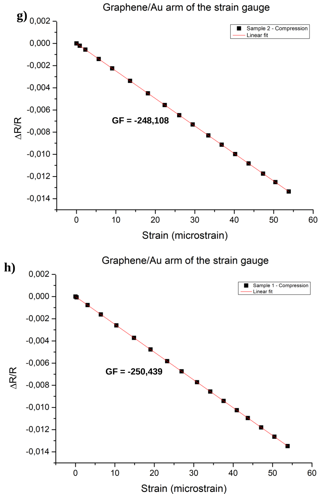
Figure 39. (a-h) Deflection sensitivity of graphene and graphene/Au arm of the strain gauge with respect to changes in strain.
