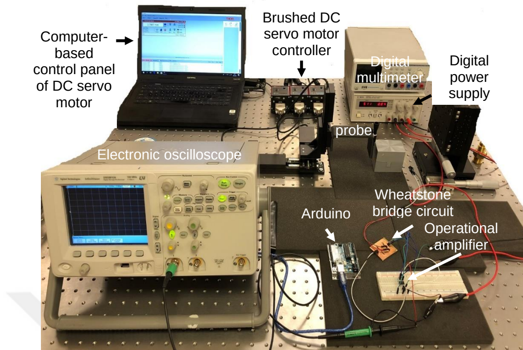
Figure 34. The first experimental setup components for microcantilever gauge factor measurement.
